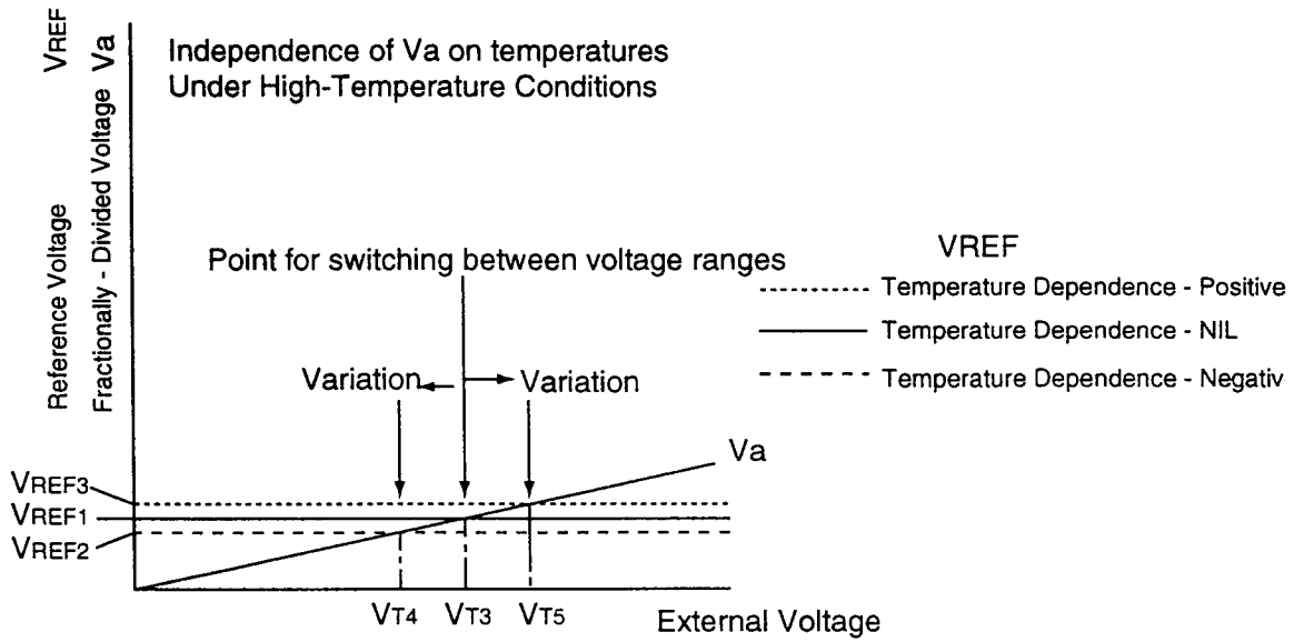
Variation in Point (Boundary Voltage) for switching between voltage ranges with respect to temperatures
