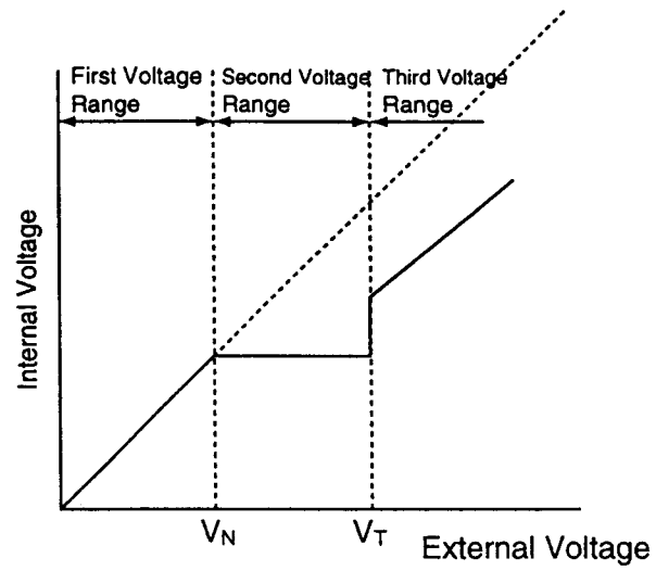
Internal Voltage Characteristics for the External Voltage of a Conventional Internal Voltage Generating Circuit
