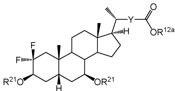
(XXI)
