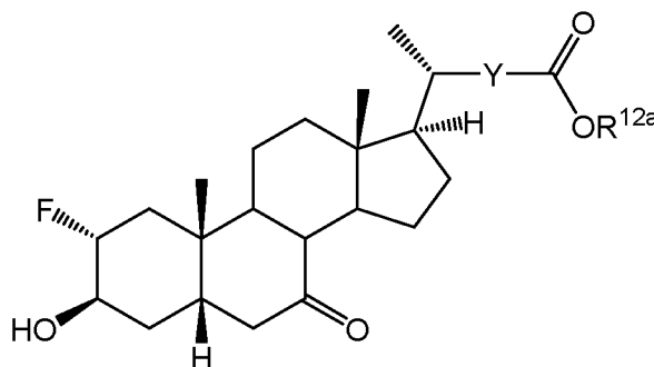
(XIIa)
