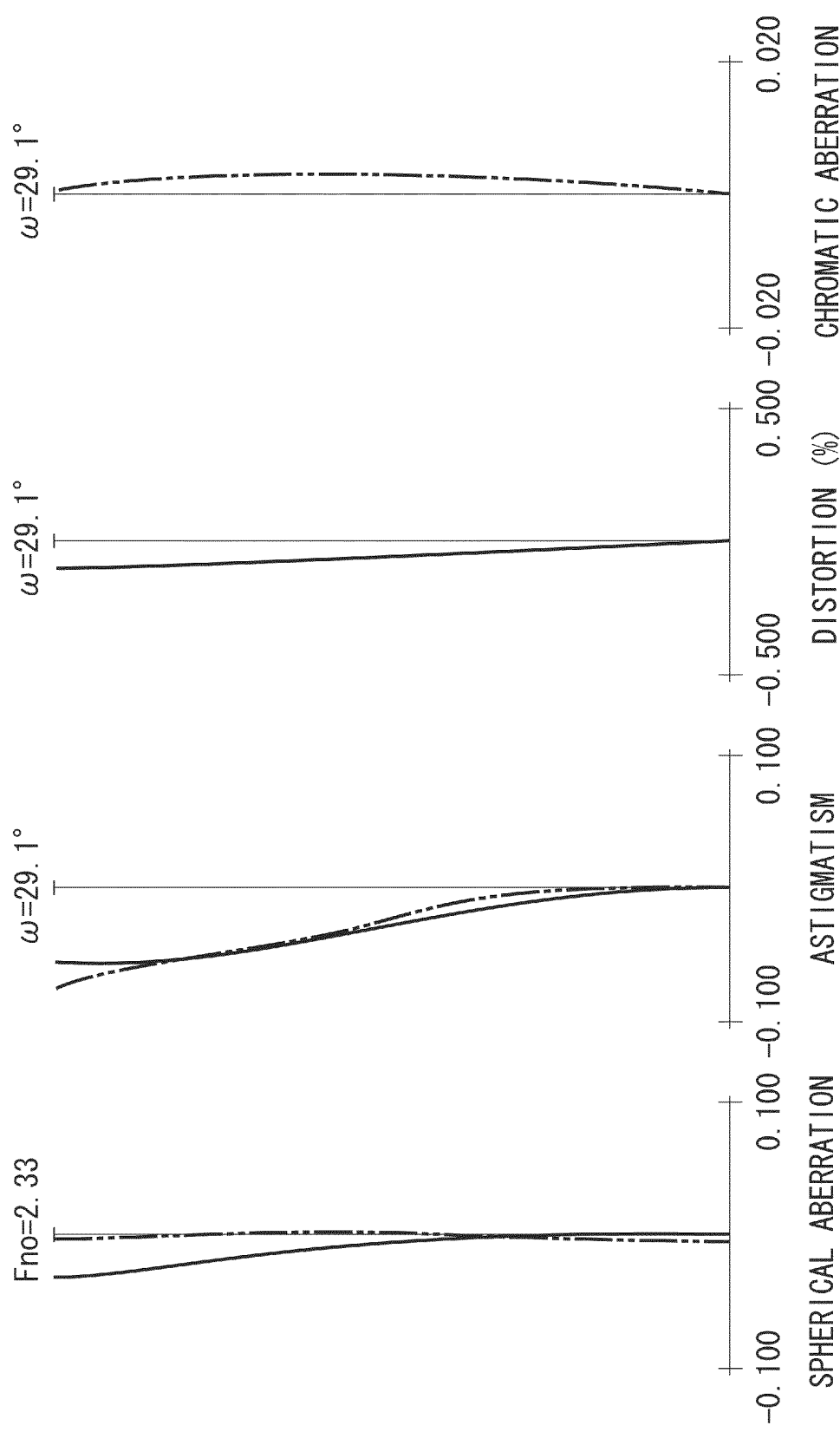
FIG. 2B TELEPHOTO END
