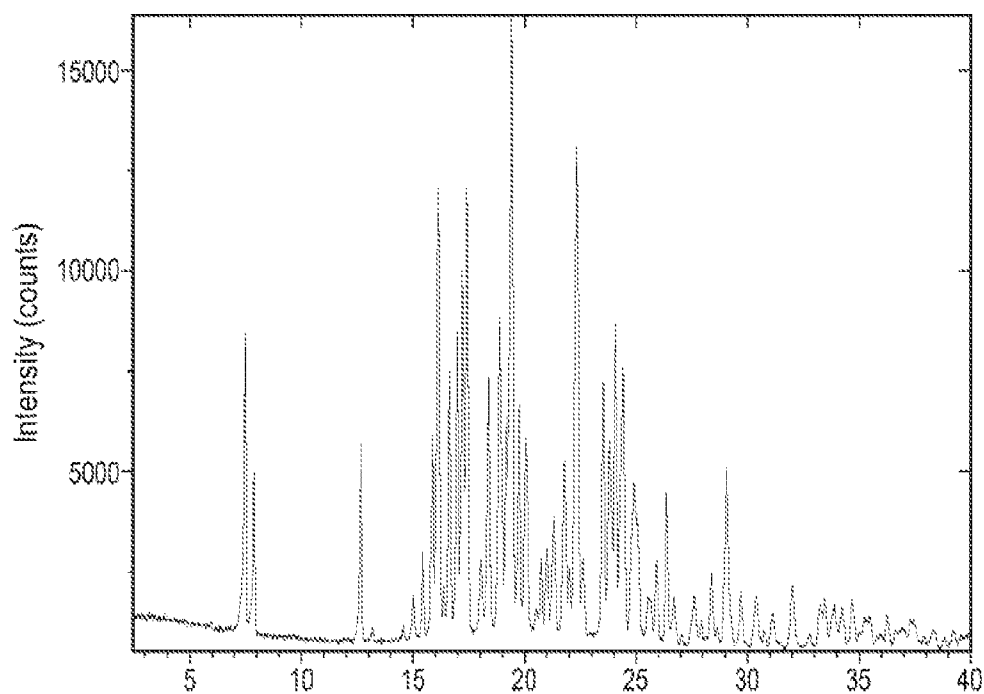
X-ray powder diffraction pattern of CPI-613 Benzathine Material B
