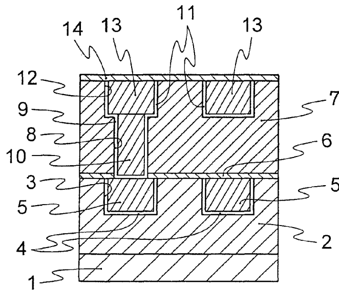
FIG. 5 PRIOR ART
