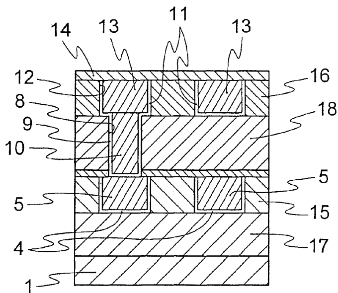
FIG. 6 PRIOR ART
