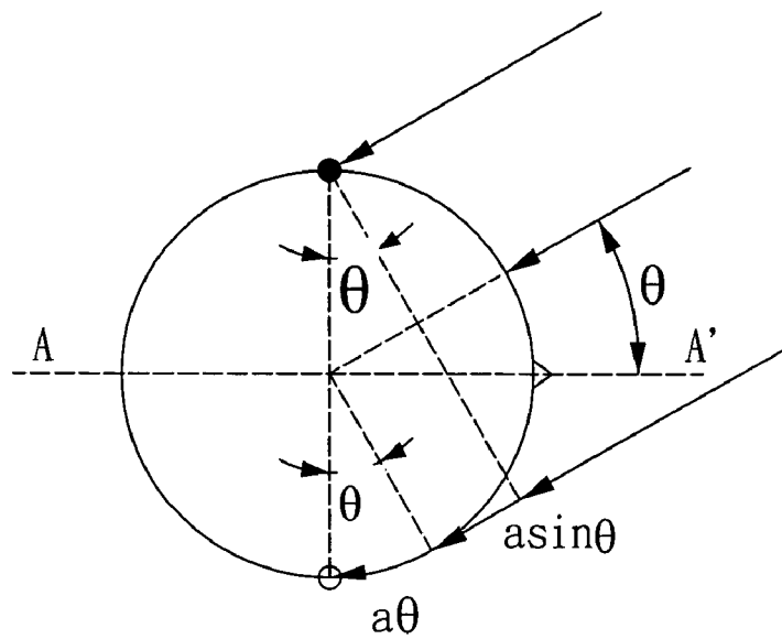
FIG. 2 (PRIOR ART)
