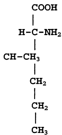
beta-methylnorleucine
