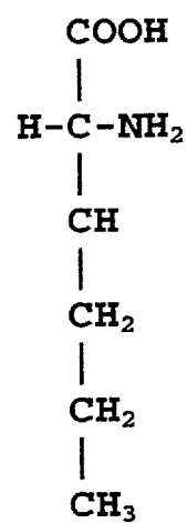
norleucine
