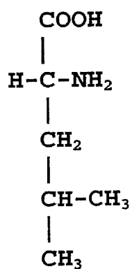
leucine
