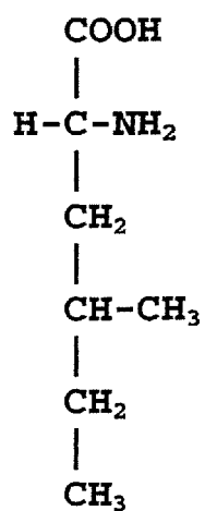
homoisoleucine
