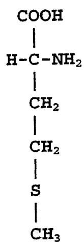
methionine
