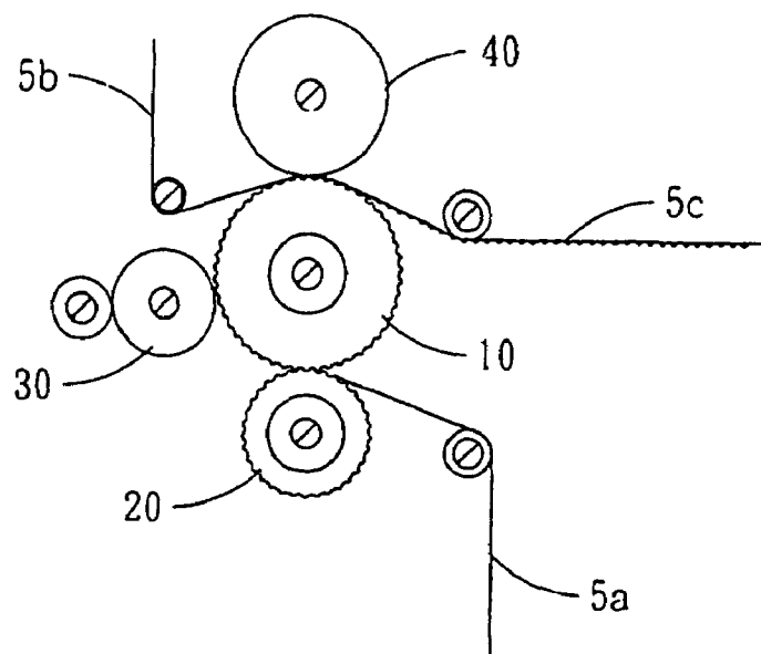
FIG. 1 PRIOR ART
