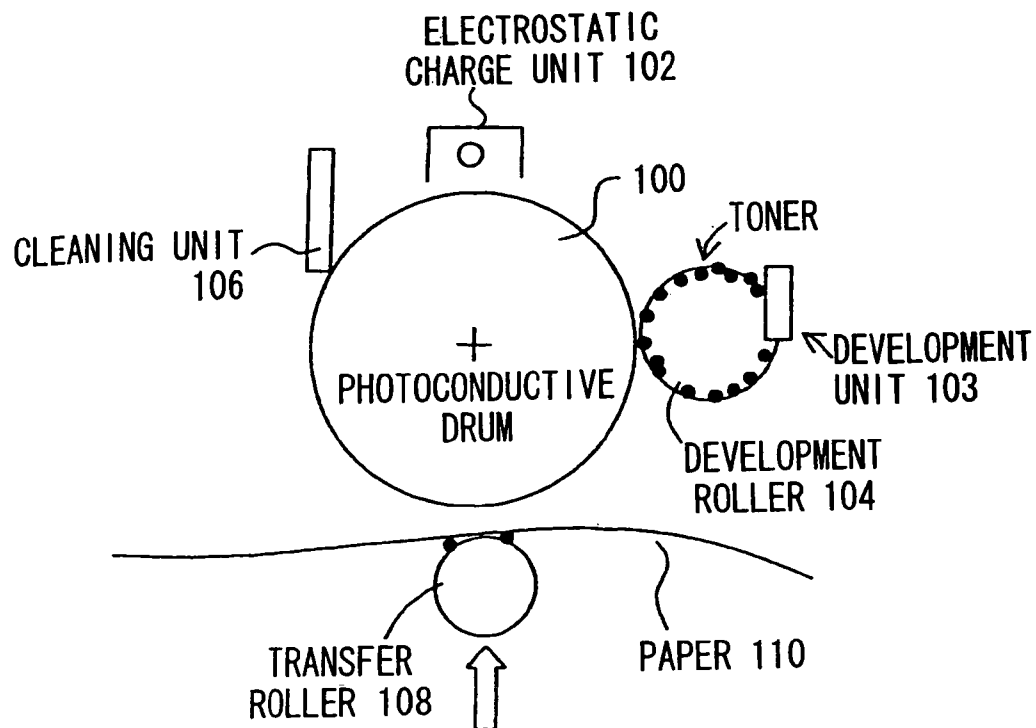
FIG. 32 [PRIOR ART]
