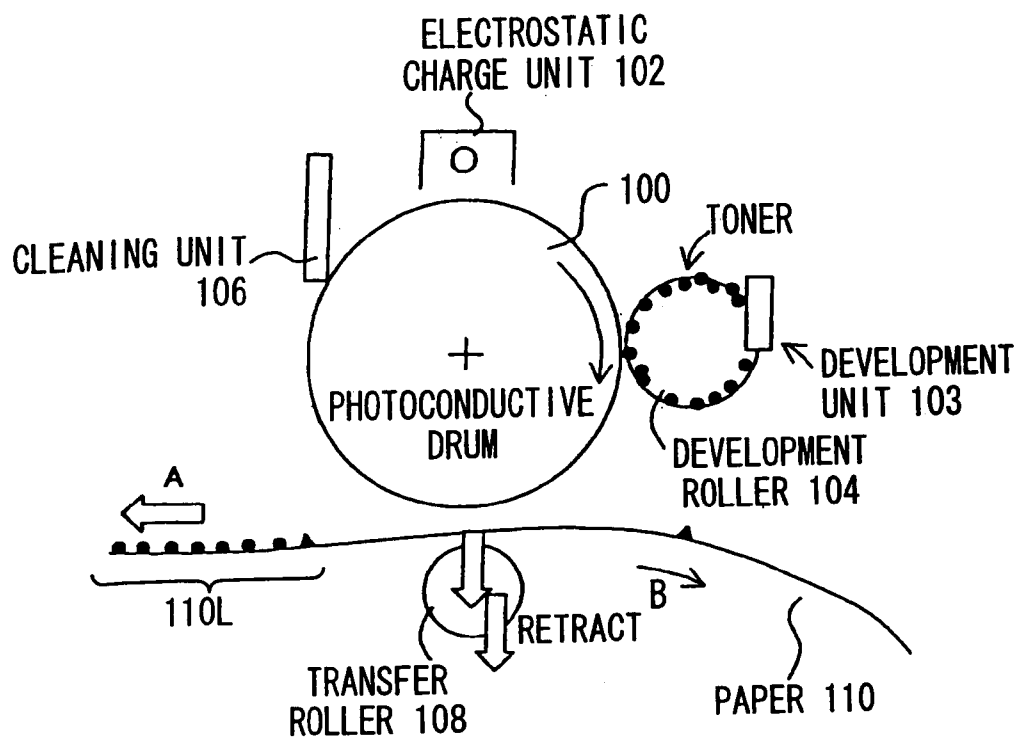
FIG. 31 [PRIOR ART]
