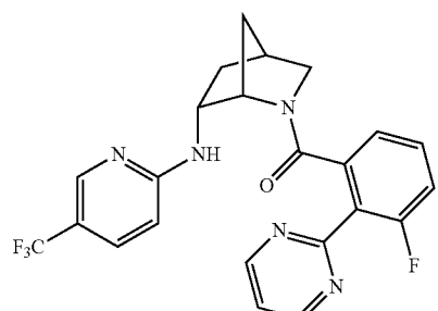
(3-fluoro-2-(pyrimidin-2-yl)phenyl)((1S,4S,6R)-6-((5-(trifluoromethyl)pyridin-2-yl)amino)-2-azabicyclo[2.2.1]heptan-2-yl)methanone
