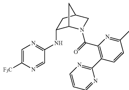
(6-methyl-3-(pyrimidin-2-yl)pyridin-2-yl)((1S,4S,6R)-6-((5-(trifluoromethyl)pyrazin-2-yl)amino)-2-azabicyclo[2.2.1]heptan-2-yl)methanone
