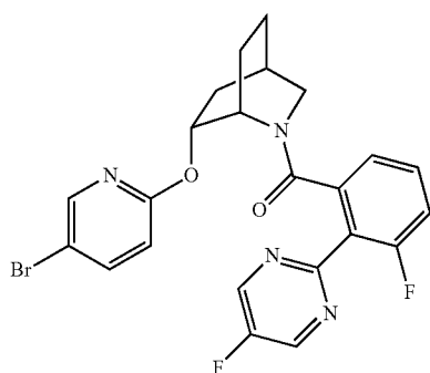
((1S,4R,6R)-6-((5-bromopyridin-2-yl)oxy)-2-azabicyclo[2.2.2]octan-2-yl)(3-fluoro-2-(5-fluoropyrimidin-2-yl)phenyl)methanone,
