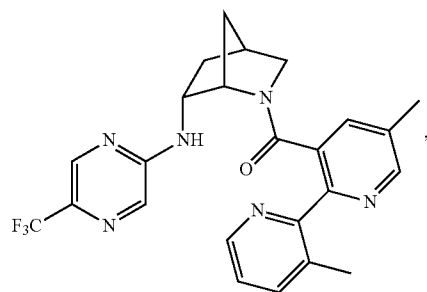
(3,5'-dimethyl-[2,2'-bipyridin]-3-yl)((1S,4S,6R)-6-((5-(trifluoromethyl)pyrazin-2-yl)amino)-2-azabicyclo[2.2.1]heptan-2-yl)methanone
