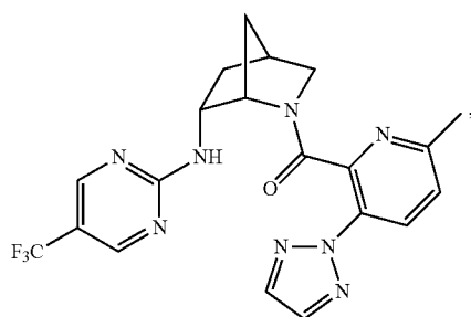
(6-methyl-3-(2H-1,2,3-triazol-2-yl)pyridin-2-yl)((1S,4S,6R)-6-((5-(trifluoromethyl)pyrimidin-2-yl)amino)-2-azabicyclo[2.2.1]heptan-2-yl)methanone
