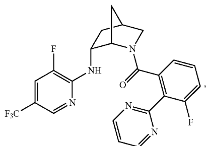
((1S,4S,6R)-6-((3-fluoro-2-(pyrimidin-2-yl)phenyl)((1S,4S,6R)-6-((3-fluoro-5-(trifluoromethyl)pyridin-2-yl)amino)-2-azabicyclo[2.2.1]heptan-2-yl)methanone
