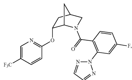
(4-fluoro-2-(2H-1,2,3-triazol-2-yl)phenyl)((1S,4R,6R)-6-((5-(trifluoromethyl)pyridin-2-yl)oxy)-2-azabicyclo[2.2.1]heptan-2-yl)methanone
