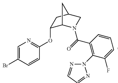
((1S,4R,6R)-6-((5-bromopyridin-2-yl)oxy)-2-azabicyclo[2.2.1]heptan-2-yl)(3-fluoro-2-(2H-1,2,3-triazol-2-yl)phenyl)methanone
