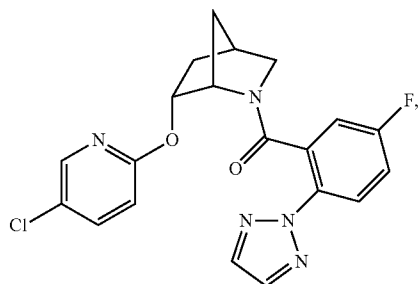
((1S,4R,6R)-6-((5-chloropyridin-2-yl)oxy)-2-azabicyclo[2.2.1]heptan-2-yl)(5-fluoro-2-(2H-1,2,3-triazol-2-yl)phenyl)methanone
