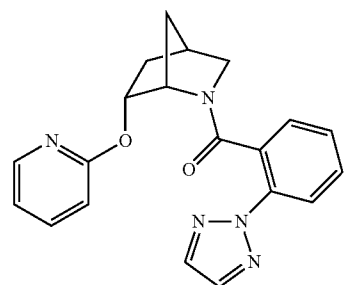
(2-(2H-1,2,3-triazol-2-yl)phenyl)((1S,4R,6R)-6-(pyridin-2-yloxy)-2-azabicyclo[2.2.1]heptan-2-yl)methanone
