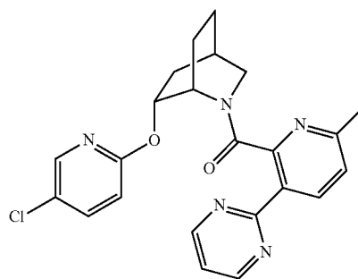
((1S,4R,6R)-6-((5-chloropyridin-2-yl)oxy)-2-azabicyclo[2.2.2]octan-2-yl)(6-methyl-3-(pyrimidin-2-yl)pyridin-2-yl)methanone,
