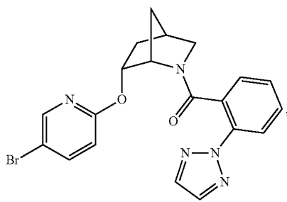
(2-(2H-1,2,3-triazol-2-yl)phenyl)((1S,4R,6R)-6-((5-bromopyridin-2-yl)oxy)-2-azabicyclo[2.2.1]heptan-2-yl)methanone
