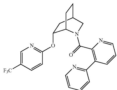
[2,3'-bipyridin]-2'-yl((1S,4R,6R)-6-((5-(trifluoromethyl)pyridin-2-yl)oxy)-2-azabicyclo[2.2.2]octan-2-yl)methanone
