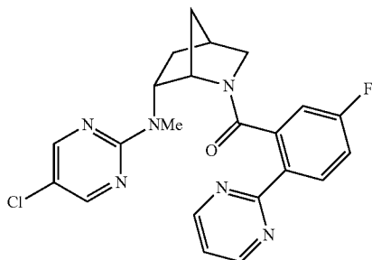
((1S,4S,6R)-6-((5-chloropyrimidin-2-yl)(methyl)amino)-2-azabicyclo[2.2.1]heptan-2-yl)(5-fluoro-2-(pyrimidin-2-yl)phenyl)methanone
