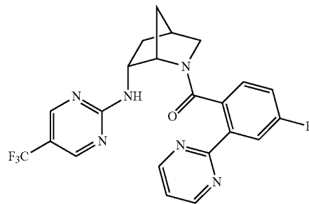
(4-fluoro-2-(pyrimidin-2-yl)phenyl)((1S,4S,6R)-6-((5-(trifluoromethyl)pyrimidin-2-yl)amino)-2-azabicyclo[2.2.1]heptan-2-yl)methanone
