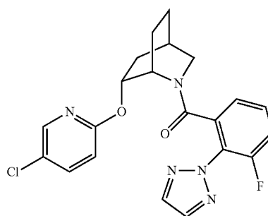
((1S,4R,6R)-6-((5-chloropyridin-2-yl)oxy)-2-azabicyclo[2.2.2]octan-2-yl)(3-fluoro-2-(2H-1,2,3-triazol-2-yl)phenyl)methanone,
