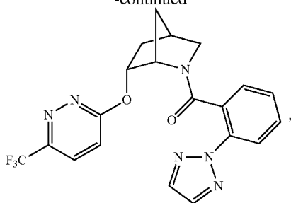
(2-(2H-1,2,3-triazol-2-yl)phenyl)((1S,4R,6R)-6-((6-(trifluoromethyl)pyridazin-3-yl)oxy)-2-azabicyclo[2.2.1]heptan-2-yl)methanone
