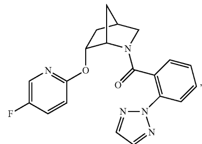
(2-(2H-1,2,3-triazol-2-yl)phenyl)((1S,4R,6R)-6-((5-fluoropyridin-2-yl)oxy)-2-azabicyclo[2.2.1]heptan-2-yl)methanone
