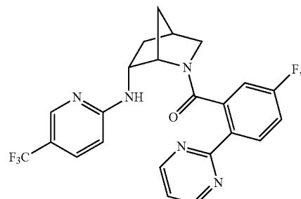
(5-fluoro-2-((pyrimidin-2-yl)phenyl)((1S,4S,6R)-6-((5-(trifluoromethyl)pyridin-2-yl)amino)-2-azabicyclo[2.2.1]heptan-2-yl)methanone
