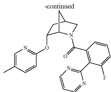
(3-fluoro-2-(pyrimidin-2-yl)phenyl)((1S,4R,6R)-6-((5-methylpyridin-2-yl)oxy)-2-azabicyclo[2.2.1]heptan-2-yl)methanone
