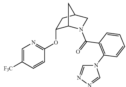
(R/S)-2-(4H-1,2,4-triazol-4-yl)phenyl(6-((5-(trifluoromethyl)pyridin-2-yl)oxy)-2-azabicyclo[2.2.1]heptan-2-yl)methanone
