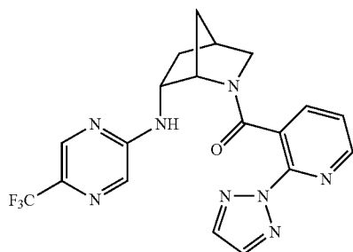
(2-(2H-1,2,3-triazol-2-yl)pyridin-3-yl)((1S,4S,6R)-6-((5-(trifluoromethyl)pyrazin-2-yl)amino)-2-azabicyclo[2.2.1]heptan-2-yl)methanone
