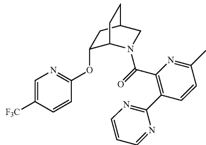
(6-methyl-3-(pyrimidin-2-yl)pyridin-2-yl)((1S,4R,6R)-6-((5-(trifluoromethyl)pyridin-2-yl)oxy)-2-azabicyclo[2.2.2]octan-2-yl)methanone
