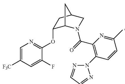
((1S,4R,6R)-6-((3-fluoro-5-(trifluoromethyl)pyridin-2-yl)oxy)-2-azabicyclo[2.2.1]heptan-2-yl)(6-methyl-3-(2H-1,2,3-triazol-2-yl)pyridin-2-yl)methanone
