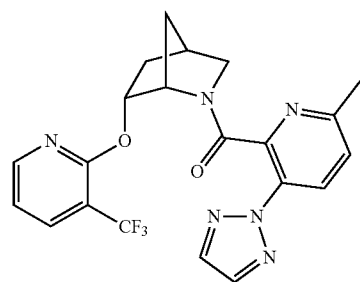
(6-methyl-3-(2H-1,2,3-triazol-2-yl)pyridin-2-yl)((1S,4R,6R)-6-((3-(trifluoromethyl)pyridin-2-yl)oxy)-2-azabicyclo[2.2.1]heptan-2-yl)methanone
