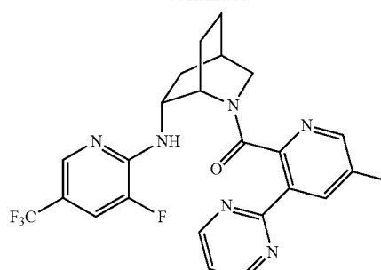
((1S,4R,6R)-6-((3-fluoro-5-(trifluoromethyl)pyridin-2-yl)amino)-2-azabicyclo[2.2.2]octan-2-yl)(5-methyl-3-(pyrimidin-2-yl)pyridin-2-yl)methanone
