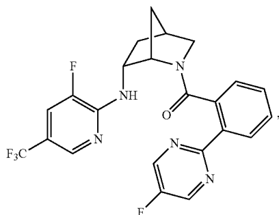
((1S,4S,6R)-6-((3-fluoro-5-(trifluoromethyl)pyridin-2-yl)amino)-2-azabicyclo[2.2.1]heptan-2-yl)(2-(5-fluoropyrimidin-2-yl)phenyl)methanone
