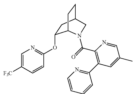
(5'-methyl-[2,3'-bipyridin]-2'-yl)((1S,4R,6R)-6-((5-(trifluoromethyl)pyridin-2-yl)oxy)-2-azabicyclo[2.2.2]octan-2-yl)methanone
