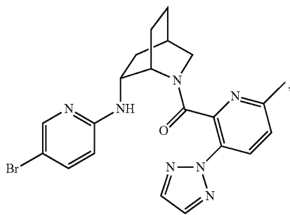
((1S,4R,6R)-6-((5-bromopyridin-2-yl)amino)-2-azabicyclo[2.2.2]octan-2-yl)(6-methyl-3-(2H-1,2,3-triazol-2-yl)pyridin-2-yl)methanone
