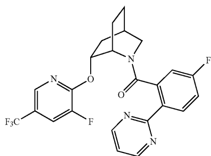
(5-fluoro-2-(pyrimidin-2-yl)phenyl)((1S,4R,6R)-6-((3-fluoro-5-(trifluoromethyl)pyridin-2-yl)oxy)-2-azabicyclo[2.2.2]octan-2-yl)methanone,
