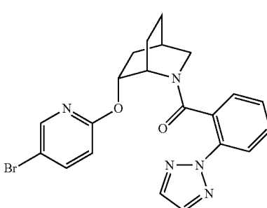
(2-(2H-1,2,3-triazol-2-yl)phenyl)((1S,4R,6R)-6-((5-(bromopyridin-2-yl)oxy)-2-azabicyclo[2.2.2]octan-2-yl)methanone
