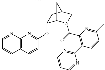
((1S,4R,6R)-6-((1,8-naphthyridin-2-yl)oxy)-2-azabicyclo[2.2.1]heptan-2-yl)-6-methyl-3-(pyrimidin-2-yl)pyridin-2-yl)methanone
