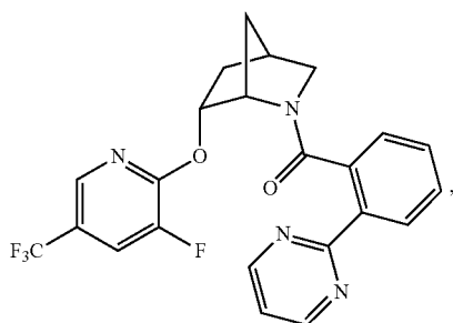
((1S,4R,6R)-6-((3-fluoro-5-(trifluoromethyl)pyridin-2-yl)oxy)-2-azabicyclo[2.2.1]heptan-2-yl)(2-(pyrimidin-2-yl)phenyl)methanone
