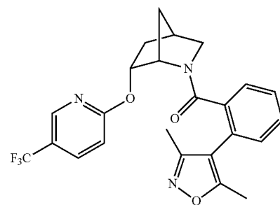
(2-(3,5-dimethylisoxazol-4-yl)phenyl)((1S,4R,6R)-6-((5-(trifluoromethyl)pyridin-2-yl)oxy)-2-azabicyclo[2.2.1]heptan-2-yl)methanone
