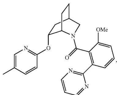
(2-methoxy-6-(pyrimidin-2-yl)phenyl)((1S,4R,6R)-6-((5-methylpyridin-2-yl)oxy)-2-azabicyclo[2.2.2]octan-2-yl)methanone
