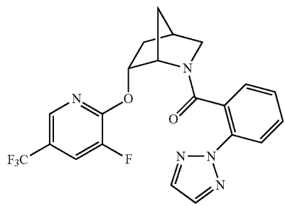
(2-(2H-1,2,3-triazol-2-yl)phenyl)((1S,4R,6R)-6-((3-fluoro-5-(trifluoromethyl)pyridin-2-yl)oxy)-2-azabicyclo[2.2.1]-heptan-2-yl)methanone
