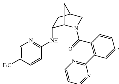
(2-(pyrimidin-2-yl)phenyl)((1S,4S,6R)-6-((5-(trifluoromethyl)pyridin-2-yl)amino)-2-azabicyclo[2.2.1]heptan-2-yl)methanone
