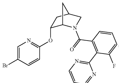
((1S,4R,6R)-6-((5-bromopyridin-2-yl)oxy)-2-azabicyclo[2.2.1]heptan-2-yl)(3-fluoro-2-(pyrimidin-2-yl)phenyl)methanone
