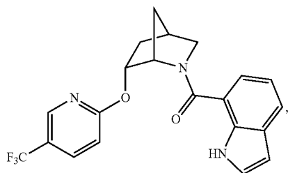
(1H-indol-7-yl)((1S,4R,6R)-6-((5-(trifluoromethyl)pyridin-2-yl)oxy)-2-azabicyclo[2.2.1]heptan-2-yl)methanone
