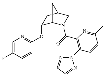
((1S,4R,6R)-6-((5-fluoropyridin-2-yl)oxy)-2-azabicyclo[2.2.1]heptan-2-yl)(6-methyl-3-(2H-1,2,3-triazol-2-yl)pyridin-2-yl)methanone
