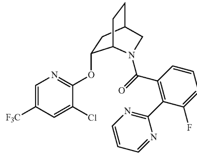
((1S,4R,6R)-6-((3-chloro-5-(trifluoromethyl)pyridin-2-yl)oxy)-2-azabicyclo[2.2.2]octan-2-yl)(3-fluoro-2-(pyrimidin-2-yl)phenyl)methanone
