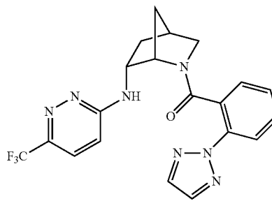
(2-(2H-1,2,3-triazol-2-yl)phenyl)((1S,4S,6R)-6-((6-(trifluoromethyl)pyridazin-3-yl)amino)-2-azabicyclo[2.2.1]heptan-2-yl)methanone
