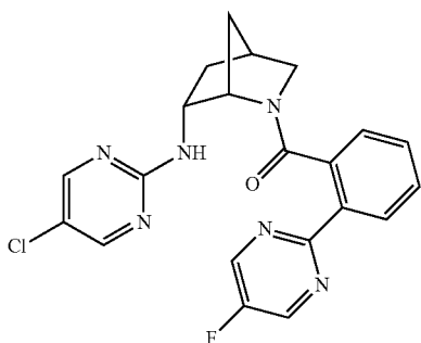
((1S,4S,6R)-6-((5-chloropyrimidin-2-yl)(methyl)amino)-2-azabicyclo[2.2.1]heptan-2-yl)(2-(5-fluoropyrimidin-2-yl)phenyl)methanone
