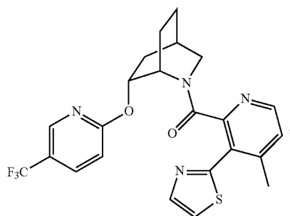
(4-methyl-3-(thiazol-2-yl)pyridin-2-yl)((1S,4R,6R)-6-((5-(trifluoromethyl)pyridin-2-yl)oxy)-2-azabicyclo[2.2.2]octan-2-yl)methanone
