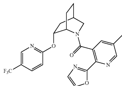
(5-methyl-2-(oxazol-2-yl)pyridin-3-yl)((1S,4R,6R)-6-((5-(trifluoromethyl)pyridin-2-yl)oxy)-2-azabicyclo[2.2.2]octan-2-yl)methanone
