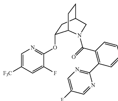
((1S,4R,6R)-6-((3-fluoro-5-(trifluoromethyl)pyridin-2-yl)oxy)-2-azabicyclo[2.2.2]octan-2-yl)(2-(fluoropyrimidin-2-yl)phenyl)methanone,
