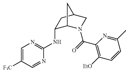
(3-ethoxy-6-methylpyridin-2-yl)((1S,4S,6R)-6-((5-(tri fluoromethyl)pyrimidin-2-yl)amino)-2-azabicyclo[2.2.1]heptan-2-yl)methanone
