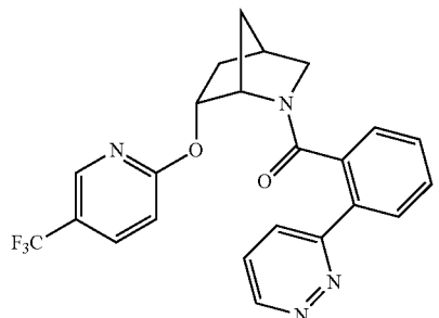
(2-(pyridazin-3-yl)phenyl)((1S,4R,6R)-6-((5-(trifluoromethyl)pyridin-2-yl)oxy)-2-azabicyclo[2.2.1]heptan-2-yl)methanone
