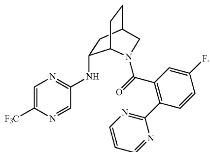
(5-fluoro-2-(pyrimidin-2-yl)phenyl)((1S,4R,6R)-6-((5-(trifluoromethyl)pyrazin-2-yl)amino)-2-azabicyclo[2.2.2]octan-2-yl)methanone
