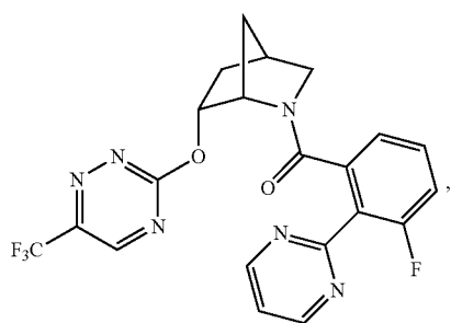
(3-fluoro-2-(pyrimidin-2-yl)phenyl)((1S,4R,6R)-6-((6-(trifluoromethyl)pyridazin-3-yl)oxy)-2-azabicyclo[2.2.1]heptan-2-yl)methanone
