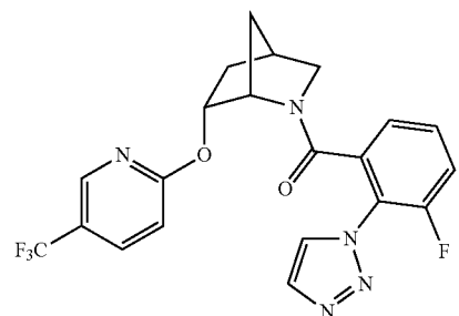
(3-fluoro-2-(1H-1,2,3-triazol-1-yl)phenyl)((1S,4R,6R)-6-((5-(trifluoromethyl)pyridin-2-yl)oxy)-2-azabicyclo[2.2.1]heptan-2-yl)methanone
