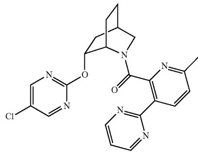
((1S,4R,6R)-6-((5-chloropyrimidin-2-yl)oxy)-2-azabicyclo[2.2.1]heptan-2-yl)(6-methyl-3-(pyrimidin-2-yl)pyridin-2-yl)methanone
