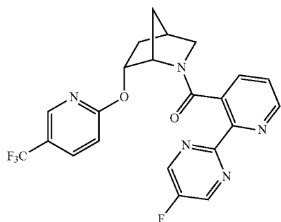
(2-(5-fluoropyrimidin-2-yl)pyridin-3-yl)((1S,4R,6R)-6-((5-(trifluoromethyl)pyridin-2-yl)oxy)-2-azabicyclo[2.2.1]heptan-2-yl)methanone
