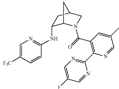
Example 375
