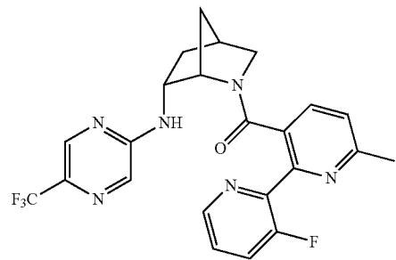
(3'-fluoro-6-methyl-[2,2'-bipyridin]-3-yl)((1S,4S,6R)-6-((5-(trifluoromethyl)pyrazin-2-yl)amino)-2-azabicyclo[2.2.1]heptan-2-yl)methanone,
