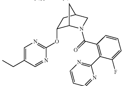
((1S,4R,6R)-6-((5-ethylpyrimidin-2-yl)oxy)-2-azabicyclo[2.2.1]heptan-2-yl)(3-fluoro-2-(pyrimidin-2-yl)phenyl)methanone
