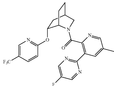
(3-(5-fluoropyrimidin-2-yl)-5-methylpyridin-2-yl)((1S,4R,6R)-6-((5-(trifluoromethyl)pyridin-2-yl)oxy)-2-azabicyclo[2.2.2]octan-2-yl)methanone
