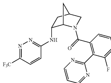
(3-fluoro-2-(pyrimidin-2-yl)phenyl)((1S,4S,6R)-6-((6-(trifluoromethyl)pyridazin-3-yl)amino)-2-azabicyclo[2.2.1]heptan-2-yl)methanone
