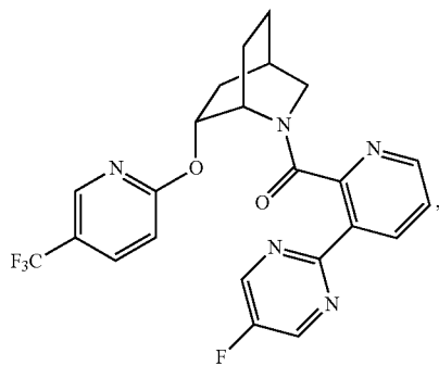
(3-(5-fluoropyrimidin-2-yl)pyridin-2-yl)((1S,4R,6R)-6-((5-(trifluoromethyl)pyridin-2-yl)oxy)-2-azabicyclo[2.2.2]octan-2-yl)methanone
