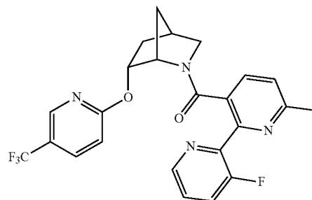
(3-fluoro-6-methyl-[2,2'-bipyridin]-3-yl)((1S,4R,6R)-6-((5-(trifluoromethyl)pyridin-2-yl)oxy)-2-azabicyclo[2.2.1]heptan-2-yl)methanone
