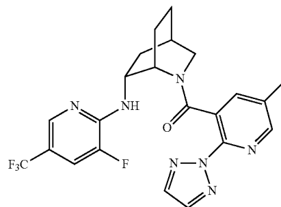
((1S,4R,6R)-6-((3-fluoro-5-(trifluoromethyl)pyridin-2-yl)amino)-2-azabicyclo[2.2.2]octan-2-yl)(5-methyl-2-(2H-1,2,3-triazol-2-yl)pyridin-3-yl)methanone
