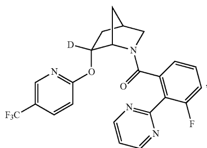
(3-fluoro-2-(pyrimidin-2-yl)phenyl)((1S,4R,6R)-(6- 2 H)-((5-(trifluoromethyl)pyrimidin-2-yl)oxy)-2-azabicyclo[2.2.1]heptan-2-yl)methanone
