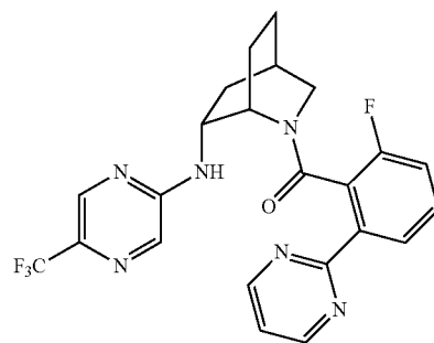
(2-fluoro-6-(pyrimidin-2-yl)phenyl)((1S,4R,6R)-6-((5-(trifluoromethyl)pyrazin-2-yl)amino)-2-azabicyclo[2.2.2]octan-2-yl)methanone
