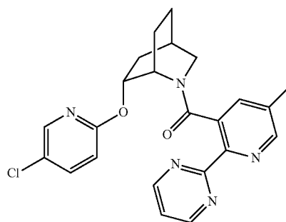
((1S,4R,6R)-6-((5-chloropyridin-2-yl)oxy)-2-azabicyclo[2.2.2]octan-2-yl)(5-methyl-2-(pyrimidin-2-yl)pyridin-2-yl)methanone,
