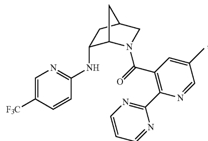
(5-methyl-2-(pyrimidin-2-yl)pyridin-3-yl)((1S,4S,6R)-6-((5-(trifluoromethyl)pyridin-2-yl)amino)-2-azabicyclo[2.2.1]heptan-2-yl)methanone
