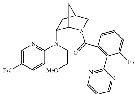
(3-fluoro-2-(pyrimidin-2-yl)phenyl)((1S,4S,6R)-6-((2-methoxyethyl)(5-(trifluoromethyl)pyridin-2-yl)amino)-2-azabicyclo[2.2.1]heptan-2-yl)methanone
