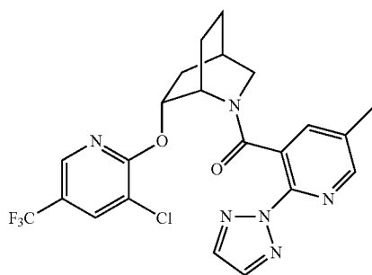
((1S,4R,6R)-6-((3-chloro-5-(trifluoromethyl)pyridin-2-yl)oxy)-2-azabicyclo[2.2.2]octan-2-yl)(5-methyl-2-(2H-1,2,3-triazol-2-yl)pyridin-3-yl)methanone,
