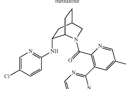
((1S,4R,6R)-6-((5-chloropyridin-2-yl)amino)-2-azabicyclo[2.2.2]octan-2-yl)(5-methyl-3-(pyrimidin-2-yl)pyridin-2-yl)methanone
