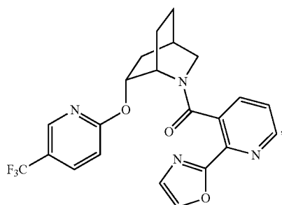
(2-(oxazol-2-yl)pyridin-3-yl)((1S,4R,6R)-6-((5-(trifluoromethyl)pyridin-2-yl)oxy)-2-azabicyclo[2.2.2]octan-2-yl)methanone
