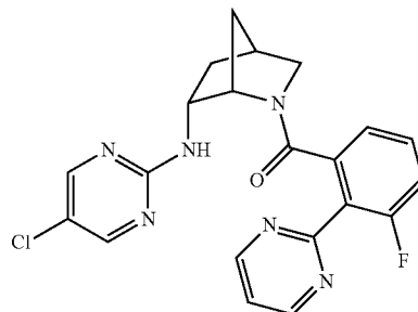
((1S,4S,6R)-6-((5-chloropyrimidin-2-yl)amino)-2-azabicyclo[2.2.1]heptan-2-yl)(3-fluoro-2-(pyrimidin-2-yl)phenyl)methanone
