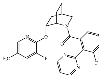
(3-fluoro-2-(pyrimidin-2-yl)phenyl)((1S,4R,6R)-6-((3-fluoro-5-(trifluoromethyl)pyridin-2-yl)oxy)-2-azabicyclo[2.2.2]octan-2-yl)methanone
