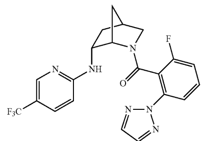
(2-fluoro-6-(2H-1,2,3-triazol-2-yl)phenyl)((1S,4S,6R)-6-((5-(trifluoromethyl)pyridin-2-yl)amino)-2-azabicyclo[2.2.1]heptan-2-yl)methanone
