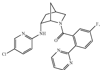
((1S,4S,6R)-6-((5-chloropyridin-2-yl)amino)-2-azabicyclo[2.2.1]heptan-2-yl)(5-fluoro-2-(pyrimidin-2-yl)phenyl)methanone
