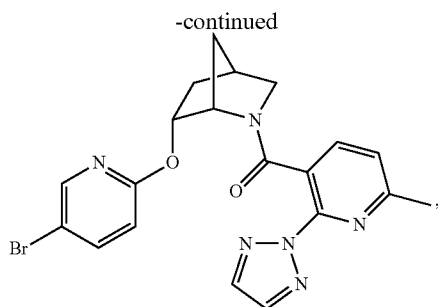
((1S,4R,6R)-6-((5-bromopyridin-2-yl)oxy)-2-azabicyclo[2.2.1]heptan-2-yl)(6-methyl-2-(2H-1,2,3-triazol-2-yl)pyridin-3-yl)methanone
