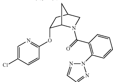
(2-(2H-1,2,3-triazol-2-yl)phenyl)((1S,4R,6R)-6-((5-chloropyridin-2-yl)oxy)-2-azabicyclo[2.2.1]heptan-2-yl)methanone
