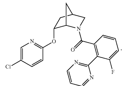
((1S,4R,6R)-6-((5-chloropyridin-2-yl)oxy)-2-azabicyclo[2.2.1]heptan-2-yl)(3-fluoro-2-(pyrimidin-2-yl)phenyl)methanone
