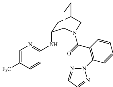
Example 500
