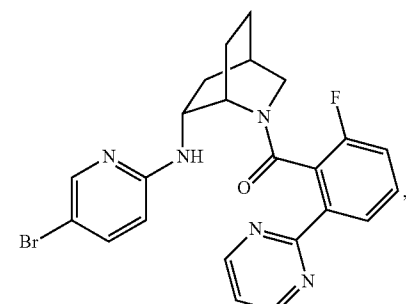
((1S,4R,6R)-6-((5-bromopyridin-2-yl)amino)-2-azabicyclo[2.2.2]octan-2-yl)(2-fluoro-6-(pyrimidin-2-yl)phenyl)methanone
