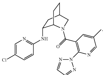
((1S,4R,6R)-6-((5-chloropyridin-2-yl)amino)-2-azabicyclo[2.2.2]octan-2-yl)(5-methyl-2-(2H-1,2,3-triazol-2-yl)pyridin-3-yl)methanone
