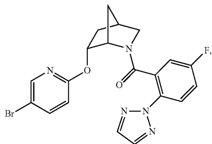
((1S,4R,6R)-6-((5-bromopyridin-2-yl)oxy)-2-azabicyclo[2.2.1]heptan-2-yl)(5-fluoro-2-(2H-1,2,3-triazol-2-yl)phenyl)methanone
