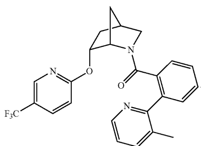
(2-(3-methylpyridin-2-yl)phenyl)((1S,4R,6R)-6-((5-(trifluoromethyl)pyridin-2-yl)oxy)-2-azabicyclo[2.2.1]heptan-2-yl)methanone
