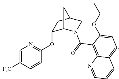
(R/S)-(7-ethoxyisoquinolin-8-yl)(6-((5-(trifluoromethyl)pyridin-2-yl)oxy)-2-azabicyclo[2.2.1]heptan-2-yl)methanone
