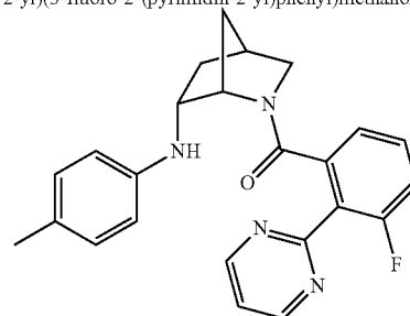
(3-fluoro-2-(pyrimidin-2-yl)phenyl)((1S,4S,6R)-6-p-tolylamino)-2-azabicyclo[2.2.1]heptan-2-yl)methanone
