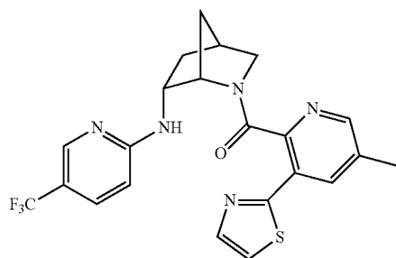
(5-methyl-3-(thiazol-2-yl)pyridin-2-yl)((1S,4S,6R)-6-((5-(trifluoromethyl)pyridin-2-yl)amino)-2-azabicyclo[2.2.1]heptan-2-yl)methanone,
