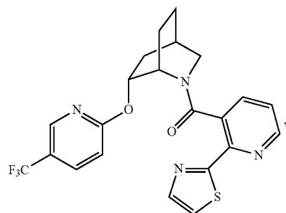
(2-(thiazol-2-yl)pyridin-3-yl)((1S,4R,6R)-6-((5-(trifluoromethyl)pyridin-2-yl)oxy)-2-azabicyclo[2.2.2]octan-2-yl)methanone,
