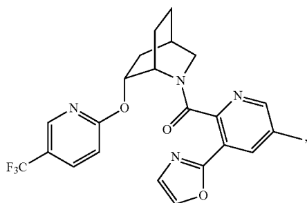
(5-methyl-3-(oxazol-2-yl)pyridin-2-yl)((1S,4R,6R)-6-((5-(trifluoromethyl)pyridin-2-yl)oxy)-2-azabicyclo[2.2.2]octan-2-yl)methanone
