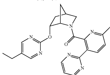
((1S,4R,6R)-6-((5-ethylpyrimidin-2-yl)oxy)-2-azabicyclo[2.2.1]heptan-2-yl)(5-methyl-3-(pyrimidin-2-yl)pyridin-2-yl)methanone
