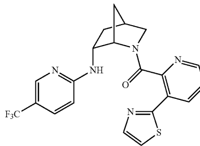
(3-(thiazol-2-yl)pyridin-2-yl)((1S,4S,6R)-6-((5-(trifluoromethyl)pyridin-2-yl)amino)-2-azabicyclo[2.2.1]heptan-2-yl)methanone,
