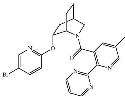
((1S,4R,6R)-6-((5-bromopyridin-2-yl)oxy)-2-azabicyclo[2.2.2]octan-2-yl)(5-methyl-2-(pyrimidin-2-yl)pyridin-3-yl)methanone,
