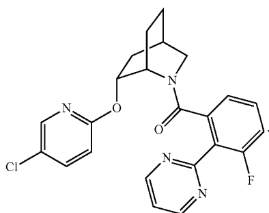
((1S,4R,6R)-6-((5-chloropyridin-2-yl)oxy)-2-azabicyclo[2.2.2]octan-2-yl)(3-fluoro-2-(pyrimidin-2-yl)phenyl)methanone
