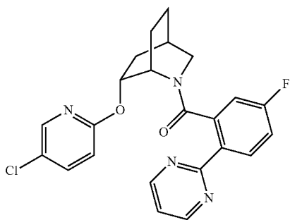
((1S,4R,6R)-6-((5-chloropyridin-2-yl)oxy)-2-azabicyclo[2.2.2]octan-2-yl)(5-fluoro-2-(pyrimidin-2-yl)phenyl)methanone,
