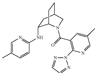
(5-methyl-2-(2H-1,2,3-triazol-2-yl)pyridin-3-yl)((1S,4R,6R)-6-((5-methylpyridin-2-yl)amino)-2-azabicyclo[2.2.2]octan-2-yl)methanone
