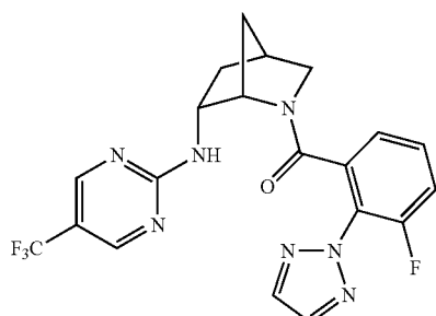
(3-fluoro-2-(2H-1,2,3-triazol-2-yl)phenyl)((1S,4S,6R)-6-((5-(trifluoromethyl)pyrimidin-2-yl)amino)-2-azabicyclo[2.2.1]heptan-2-yl)methanone
