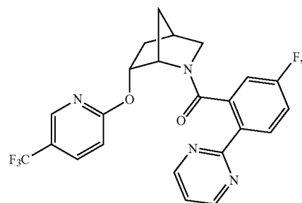
(R/S)-5-fluoro-2-(pyrimidin-2-yl)phenyl(6-((5-(trifluoromethyl)pyridin-2-yl)oxy)-2-azabicyclo[2.2.1]heptan-2-yl)methanone
