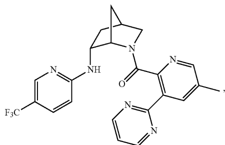
(5-methyl-3-(pyrimidin-2-yl)pyridin-2-yl)((1S,4S,6R)-6-((5-(trifluoromethyl)pyridin-2-yl)amino)-2-azabicyclo[2.2.1]heptan-2-yl)methanone
