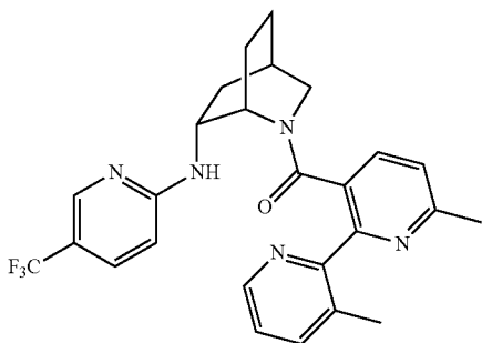
(3,6'-dimethyl-[2,2'-bipyridin]-3-yl)((1S,4R,6R)-6-((5-(trifluoromethyl)pyridin-2-yl)amino)-2-azabicyclo[2.2.2]octan-2-yl)methanone
