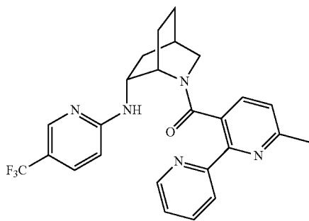
Example 380
