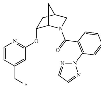
(2-(2H-1,2,3-triazol-2-yl)phenyl)((1S,4R,6R)-6-((5-(fluoromethyl)pyridin-2-yl)oxy)-2-azabicyclo[2.2.1]heptan-2-yl)methanone
