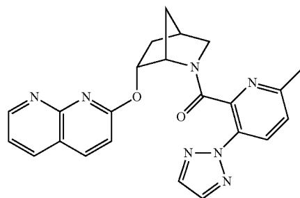
((1S,4R,6R)-6-((1,8-naphthyridin-2-yl)oxy)-2-azabicyclo[2.2.1]heptan-2-yl)(6-methyl-3-(2H-1,2,3-triazol-2-yl)pyridin-2-yl)methanone
