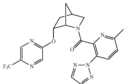
(6-methyl-3-(2H-1,2,3-triazol-2-yl)pyridin-2-yl)((1S,4R,6R)-6-((5-(trifluoromethyl)pyrazin-2-yl)oxy)-2-azabicyclo[2.2.1]heptan-2-yl)methanone
