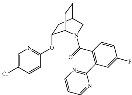
((1S,4R,6R)-6-((5-chloropyridin-2-yl)oxy)-2-azabicyclo[2.2.2]octan-2-yl)(4-fluoro-2-(pyrimidin-2-yl)phenyl)methanone,
