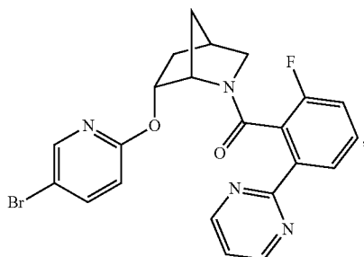
((1S,4R,6R)-6-((5-bromopyridin-2-yl)oxy)-2-azabicyclo[2.2.1]heptan-2-yl)(2-fluoro-6-(pyrimidin-2-yl)phenyl)methanone
