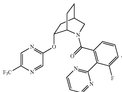
(3-fluoro-2-(pyrimidin-2-yl)phenyl)((1S,4R,6R)-6-((5-(trifluoromethyl)pyrazin-2-yl)oxy)-2-azabicyclo[2.2.2]octan-2-yl)methanone
