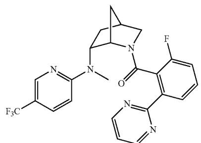
(2-fluoro-6-(pyrimidin-2-yl)phenyl)((1S,4S,6R)-6-(methyl(5-(trifluoromethyl)pyridin-2-yl)amino)-2-azabicyclo[2.2.1]heptan-2-yl)methanone
