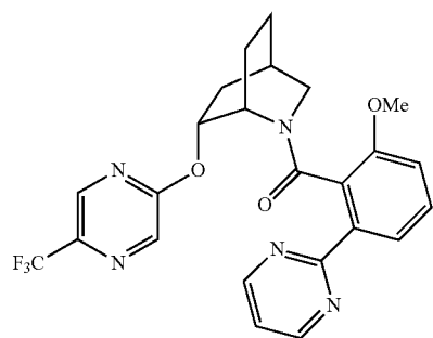
(2-methoxy-6-(pyrimidin-2-yl)phenyl)((1S,4R,6R)-6-((5-(trifluoromethyl)pyrazin-2-yl)oxy)-2-azabicyclo[2.2.2]octan-2-yl)methanone
