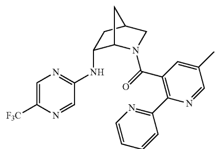
(5-methyl-[2,2'-bipyridin]-3-yl)((1S,4S,6R)-6-((5-(trifluoromethyl)pyrazin-2-yl)amino)-2-azabicyclo[2.2.1]heptan-2-yl)methanone
