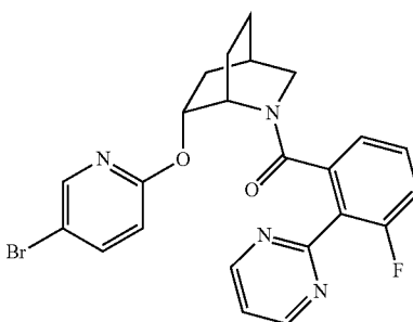
((1S,4R,6R)-6-((5-(bromopyridin-2-yl)oxy)-2-azabicyclo[2.2.2]octan-2-yl)(3-fluoro-2-(pyrimidin-2-yl)phenyl)methanone
