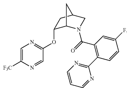
(5-fluoro-2-(pyrimidin-2-yl)phenyl)((1S,4R,6R)-6-((5-(trifluoromethyl)pyrazin-2-yl)oxy)-2-azabicyclo[2.2.1]heptan-2-yl)methanone
