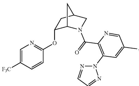
(R/S)-(5-methyl-3-(2H-1,2,3-triazol-2-yl)pyridin-2-yl)(6-((5-(trifluoromethyl)pyridin-2-yl)oxy)-2-azabicyclo[2.2.1]heptan-2-yl)methanone
