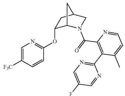
(3-(5-fluoropyrimidin-2-yl)-4-methylpyridin-2-yl)((1S,4R,6R)-6-((5-(trifluoromethyl)pyridin-2-yl)oxy)-2-azabicyclo[2.2.1]heptan-2-yl)methanone
