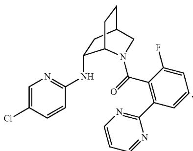
((1S,4R,6R)-6-((5-chloropyridin-2-yl)amino)-2-azabicyclo[2.2.2]octan-2-yl)(2-fluoro-6-(pyrimidin-2-yl)phenyl)methanone
