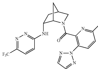
(6-methyl-3-(2H-1,2,3-triazol-2-yl)pyridin-2-yl)((1S,4S,6R)-6-((6-(trifluoromethyl)pyridazin-3-yl)amino)-2-azabicyclo[2.2.1]heptan-2-yl)methanone
