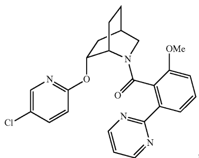
((1S,4R,6R)-6-((5-chloropyridin-2-yl)oxy)-2-azabicyclo[2.2.2]octan-2-yl)(2-methoxy-6-(pyrimidin-2-yl)phenyl)methanone
