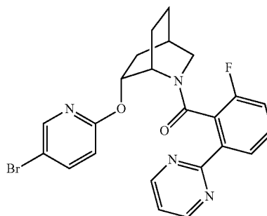
((1S,4R,6R)-6-((5-bromopyridin-2-yl)oxy)-2-azabicyclo[2.2.2]octan-2-yl)(2-fluoro-6-(pyrimidin-2-yl)phenyl)methanone,
