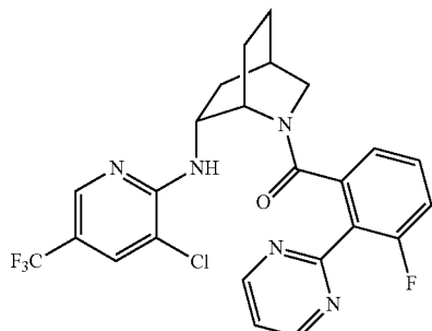
((1S,4R,6R)-6-((3-chloro-5-(trifluoromethyl)pyridin-2-yl)amino)-2-azabicyclo[2.2.2]octan-2-yl)(3-fluoro-2-(pyrimidin-2-yl)phenyl)methanone
