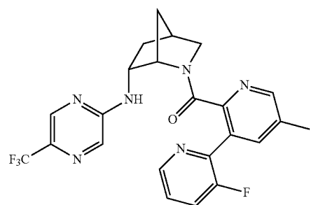
(3-fluoro-5'-methyl-[2,3'-bipyridin]-2'-yl)((1S,4S,6R)-6-((5-(trifluoromethyl)pyrazin-2-yl)amino)-2-azabicyclo[2.2.1]heptan-2-yl)methanone,
