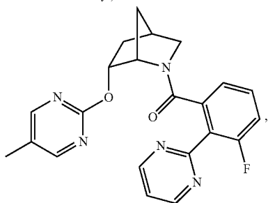
(3-fluoro-2-(pyrimidin-2-yl)phenyl)((1S,4R,6R)-6-((5-methylpyrimidin-2-yl)oxy)-2-azabicyclo[2.2.1]heptan-2-yl)methanone
