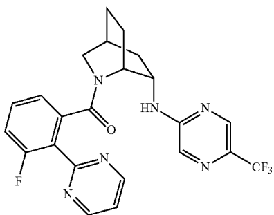
(3-fluoro-2-(pyrimidin-2-yl)phenyl)((1R,4S,6S)-6-((5-(trifluoromethyl)pyrazin-2-yl)amino)-2-azabicyclo[2.2.2]octan-2-yl)methanone
