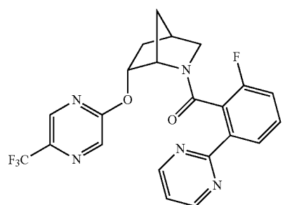
(2-fluoro-6-(pyrimidin-2-yl)phenyl)((1S,4R,6R)-6-((5-(trifluoromethyl)pyrazin-2-yl)oxy)-2-azabicyclo[2.2.1]heptan-2-yl)methanone
