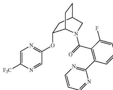
(2-fluoro-6-(pyrimidin-2-yl)phenyl)((1S,4R,6R)-6-((5-(trifluoromethyl)pyrazin-2-yl)oxy)-2-azabicyclo[2.2.2]octan-2-yl)methanone,
