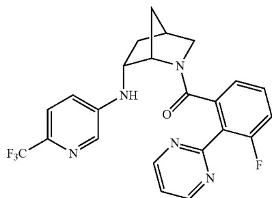
(3-fluoro-2-(pyrimidin-2-yl)phenyl) ((1S,4S,6R)-6-((6-(trifluoromethyl)pyridin-3-yl)amino)-2-azabicyclo[2.2.1]heptan-2-yl)methanone
