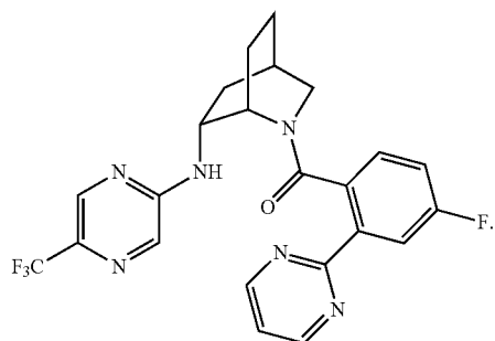
(4-fluoro-2-(pyrimidin-2-yl)phenyl)((1S,4R,6R)-6-((5-(trifluoromethyl)pyrazin-2-yl)amino)-2-azabicyclo[2.2.2]octan-2-yl)methanone
