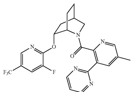
((1S,4R,6R)-6-((3-fluoro-5-(trifluoromethyl)pyridin-2-yl)oxy)-2-azabicyclo[2.2.2]octan-2-yl)(5-methyl-3-(pyrimidin-2-yl)pyridin-2-yl)methanone
