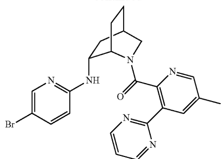
((1S,4R,6R)-6-((5-bromopyridin-2-yl)amino)-2-azabicyclo[2.2.2]octan-2-yl)(5-methyl-3-(pyrimidin-2-yl)pyridin-2-yl)methanone
