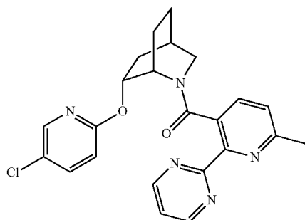
((1S,4R,6R)-6-((5-chloropyridin-2-yl)oxy)-2-azabicyclo[2.2.2]octan-2-yl)(6-methyl-2-(pyrimidin-2-yl)pyridin-3-yl)methanone,
