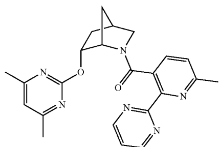
((1S,4R,6R)-6-((4,6-dimethylpyrimidin-2-yl)oxy)-2-azabicyclo[2.2.1]heptan-2-yl)(6-methyl-2-(pyrimidin-2-yl)pyridin-3-yl)methanone
