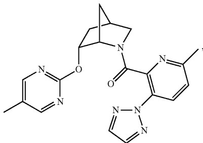
(6-methyl-3-(2H-1,2,3-triazol-2-yl)pyridin-2-yl)((1S,4R,6R)-6-((5-methylpyrimidin-2-yl)oxy)-2-azabicyclo[2.2.1]heptan-2-yl)methanone
