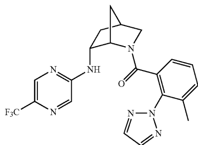
(3-methyl-2-(2H-1,2,3-triazol-2-yl)phenyl)((1S,4S,6R)-6-((5-(trifluoromethyl)pyrazin-2-yl)amino)-2-azabicyclo[2.2.1]heptan-2-yl)methanone
