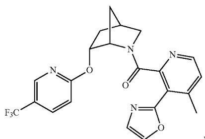
(4-methyl-3-(oxazol-2-yl)pyridin-2-yl)((1S,4R,6R)-6-((5-(trifluoromethyl)pyridin-2-yl)oxy)-2-azabicyclo[2.2.1]heptan-2-yl)methanone
