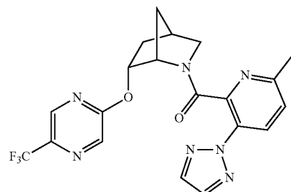
(R/S)-(6-methyl-3-(2H-1,2,3-triazol-2-yl)pyridin-2-yl)(6-((5-(trifluoromethyl)pyrazin-2-yl)oxy)-2-azabicyclo[2.2.1]heptan-2-yl)methanone
