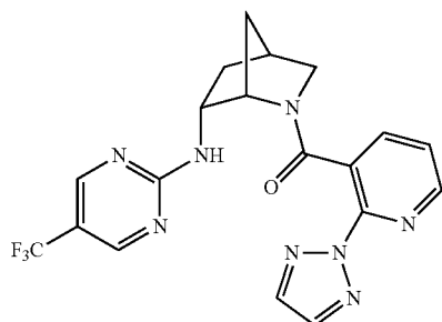
(2-(2H-1,2,3-triazol-2-yl)pyridin-3-yl)((1S,4S,6R)-6-((5-(trifluoromethyl)pyrimidin-2-yl)amino)-2-azabicyclo[2.2.1]heptan-2-yl)methanone
