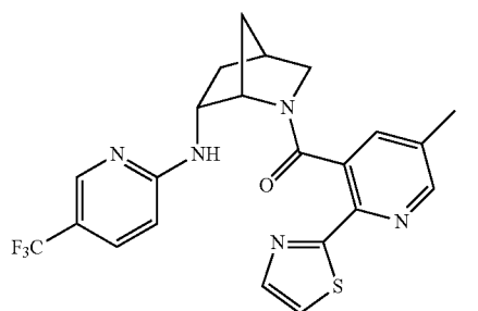
(5-methyl-2-(thiazol-2-yl)pyridin-3-yl)((1S,4S,6R)-6-((5-(trifluoromethyl)pyridin-2-yl)amino)-2-azabicyclo[2.2.1]heptan-2-yl)methanone,
