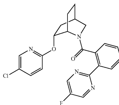
((1S,4R,6R)-6-((5-chloropyridin-2-yl)oxy)-2-azabicyclo[2.2.2]octan-2-yl)(2-(5-fluoropyrimidin-2-yl)phenyl)methanone,
