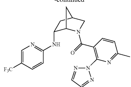
(6-methyl-2-(2H-1,2,3-triazol-2-yl)pyridin-3-yl)((1S,4S,6R)-6-((5-(trifluoromethyl)pyridin-2-yl)amino)-2-azabicyclo[2.2.1]heptan-2-yl)methanone
