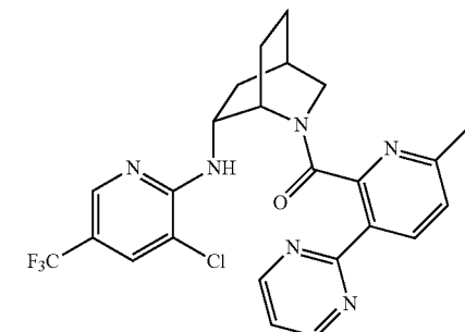
((1S,4R,6R)-6-((3-chloro-5-(trifluoromethyl)pyridin-2-yl)amino-2-azabicyclo[2.2.2]octan-2-yl)(6-methyl-3-(pyrimidin-2-yl)pyridin-2-yl)methanone
