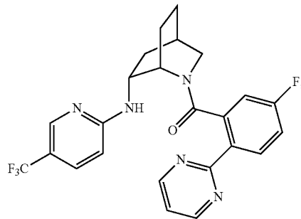
(5-fluoro-2-(pyrimidin-2-yl)phenyl)((1S,4R,6R)-6-((5-(trifluoromethyl)pyridin-2-yl)amino)-2-azabicyclo[2.2.2]octan-2-yl)methanone
