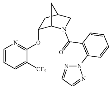
(2-(2H-1,2,3-triazol-2-yl)phenyl)((1S,4R,6R)-6-((3-(trifluoromethyl)pyridin-2-yl)oxy)-2-azabicyclo[2.2.1]heptan-2-yl)methanone
