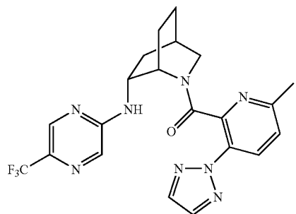
(6-methyl-3-(2H-1,2,3-triazol-2-yl)pyridin-2-yl)((1S,4R,6R)-6-((5-(trifluoromethyl)pyrazin-2-yl)amino)-2-azabicyclo[2.2.2]octan-2-yl)methanone
