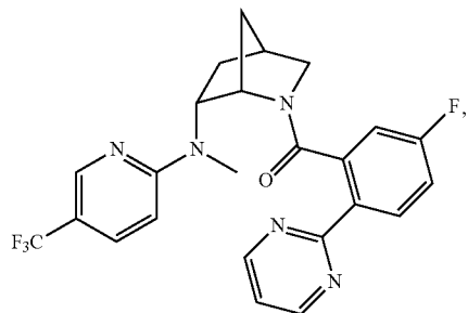
(5-fluoro-2-(pyrimidin-2-yl)phenyl)((1S,4S,6R)-6-(methyl(5-(trifluoromethyl)pyridin-2-yl)amino)-2-azabicyclo[2.2.1]heptan-2-yl)methanone
