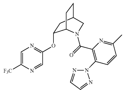
(6-methyl-3-(2H-1,2,3-triazol-2-yl)pyridin-2-yl)((1S,4R,6R)-6-((5-(trifluoromethyl)pyrazin-2-yl)oxy)-2-azabicyclo[2.2.2]octan-2-yl)methanone
