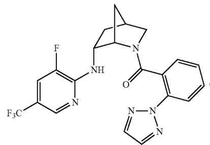
(2-(2H-1,2,3-triazol-2-yl)phenyl)((1S,4S,6R)-6-((3-fluoro-5-(trifluoromethyl)pyridin-2-yl)amino)-2-azabicyclo[2.2.1]heptan-2-yl)methanone
