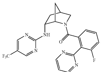
(3-fluoro-2-(pyrimidin-2-yl)phenyl)((1S,4S,6R)-6-((5-(trifluoromethyl)pyrimidin-2-yl)amino)-2-azabicyclo[2.2.1]heptan-2-yl)methanone
