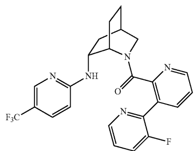
(3-fluoro-[2,3'-bipyridin]-2'-yl)((1S,4R,6R)-6-((5-(trifluoromethyl)pyridin-2-yl)amino)-2-azabicyclo[2.2.2]octan-2-yl)methanone
