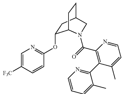
(3,4'-dimethyl-[2,3'-bipyridin]-2'-yl)((1S,4R,6R)-6-((5-(trifluoromethyl)pyridin-2-yl)oxy)-2-azabicyclo[2.2.2]octan-2-yl)methanone
