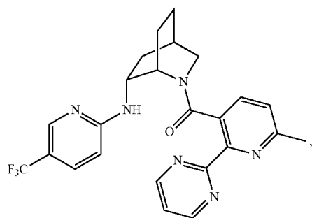
(6-methyl-2-(pyrimidin-2-yl)pyridin-3-yl)((1S,4R,6R)-6-((5-(trifluoromethyl)pyridin-2-yl)amino)-2-azabicyclo[2.2.2]octan-2-yl)methanone
