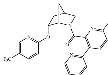
(6'-methyl-[2,3'-bipyridin]-2'-yl)((1S,4R,6R)-6-((5-(trifluoromethyl)pyridin-2-yl)oxy)-2-azabicyclo[2.2.1]heptan-2-yl)methanone
