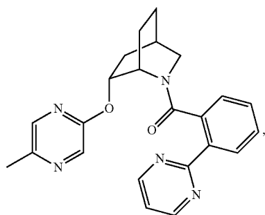
((1S,4R,6R)-6-((5-methylpyrazin-2-yl)oxy)-2-azabicyclo[2.2.2]octan-2-yl)(2-(pyrimidin-2-yl)phenyl)methanone
