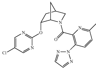
((1S,4R,6R)-6-((5-chloropyrimidin-2-yl)oxy)-2-azabicyclo[2.2.1]heptan-2-yl)(6-methyl-3-(2H-1,2,3-triazol-2-yl)pyridin-2-yl)methanone
