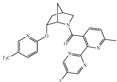
(2-(5-fluoropyrimidin-2-yl)-6-methylpyridin-3-yl)((1S,4R,6R)-6-((5-(trifluoromethyl)pyridin-2-yl)oxy)-2-azabicyclo[2.2.1]heptan-2-yl)methanone
