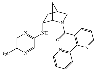
[2,2'-bipyridin]-3-yl((1S,4S,6R)-6-((5-(trifluoromethyl)pyrazin-2-yl)amino)-2-azabicyclo[2.2.1]heptan-2-yl)methanone
