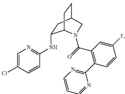
((1S,4R,6R)-6-((5-chloropyridin-2-yl)amino)-2-azabicyclo[2.2.2]octan-2-yl)(5-fluoro-2-(pyrimidin-2-yl)phenyl)methanone
