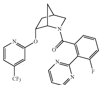
(3-fluoro-2-(pyrimidin-2-yl)phenyl)((1S,4R,6R)-6-((4-(trifluoromethyl)pyridin-2-yl)oxy)-2-azabicyclo[2.2.1]-heptan-2-yl)methanone
