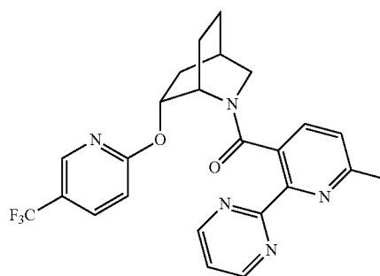
(6-methyl-2-(pyrimidin-2-yl)pyridin-3-yl)((1S,4R,6R)-6-((5-(trifluoromethyl)pyridin-2-yl)oxy)-2-azabicyclo[2.2.2]octan-2-yl)methanone,
