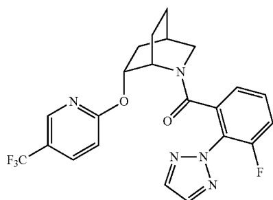
(R/S)-(3-fluoro-2-(2H-1,2,3-triazol-2-yl)phenyl) (6-((5-(trifluoromethyl)pyridin-2-yl)oxy)-2-azabicyclo[2.2.2]octan-2-yl)methanone
