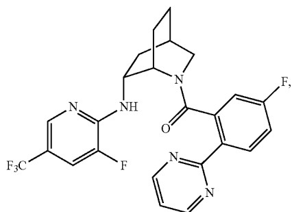
(5-fluoro-2-(pyrimidin-2-yl)phenyl)((1S,4R,6R)-6-((3-fluoro-5-(trifluoromethyl)pyridin-2-yl)amino)-2-azabicyclo[2.2.2]octan-2-yl)methanone
