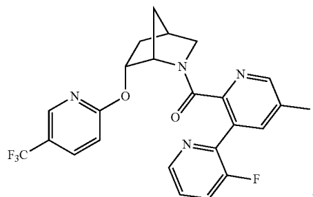
(3-fluoro-5'-methyl-[2,3'-bipyridin]-2'-yl)((1S,4R,6R)-6-((5-(trifluoromethyl)pyridin-2-yl)oxy)-2-azabicyclo[2.2.1]heptan-2-yl)methanone
