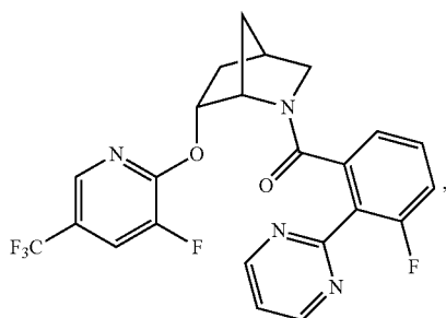
(3-fluoro-2-(pyrimidin-2-yl)phenyl)((1S,4R,6R)-6-((3-fluoro-5-(trifluoromethyl)pyridin-2-yl)oxy)-2-azabicyclo[2.2.1]heptan-2-yl)methanone
