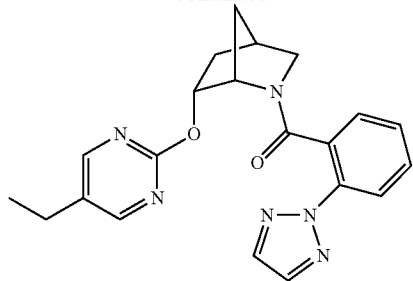
(2-(2H-1,2,3-triazol-2-yl)phenyl)((1S,4R,6R)-6-((5-ethylpyrimidin-2-yl)oxy)-2-azabicyclo[2.2.1]heptan-2-yl)methanone
