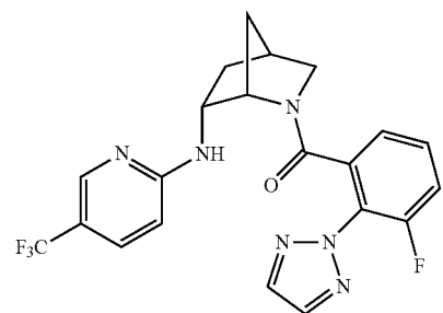
(3-fluoro-2-(2H-1,2,3-triazol-2-yl)phenyl)((1S,4S,6R)-6-((5-(trifluoromethyl)pyridin-2-yl)amino)-2-azabicyclo[2.2.1]heptan-2-yl)methanone
