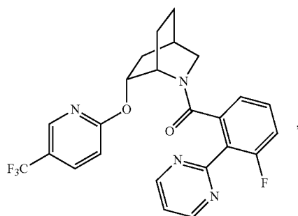
(3-fluoro-2-(pyrimidin-2-yl)phenyl)((1S,4R,6R)-6-((5-(trifluoromethyl)pyridin-2-yl)oxy)-2-azabicyclo[2.2.2]octan-2-yl)methanone
