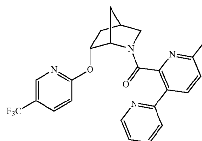
(5-methyl-[2,2'-bipyridin]-3-yl)((1S,4R,6R)-6-((5-(trifluoromethyl)pyridin-2-yl)oxy)-2-azabicyclo[2.2.1]heptan-2-yl)methanone
