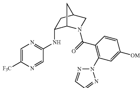
(4-methoxy-2-(2H-1,2,3-triazol-2-yl)phenyl)((1S,4S,6R)-6-((5-(trifluoromethyl)pyrazin-2-yl)amino)-2-azabicyclo[2.2.1]heptan-2-yl)methanone
