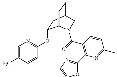
(6-methyl-2-(oxazol-2-yl)pyridin-3-yl)((1S,4R,6R)-6-((5-(trifluoromethyl)pyridin-2-yl)oxy)-2-azabicyclo[2.2.2]octan-2-yl)methanone
