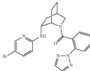
Example 533
