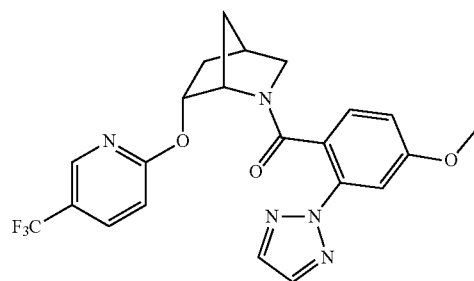
(R/S)-(4-methoxy-2-(2H-1,2,3-triazol-2-yl)phenyl)(6-((5-(trifluoromethyl)pyridin-2-yl)oxy)-2-azabicyclo[2.2.1]heptan-2-yl)methanone
