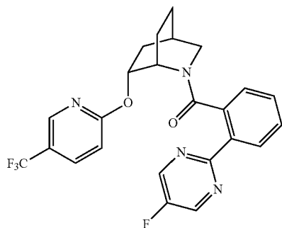
(2-(5-fluoropyrimidin-2-yl)phenyl)((1S,4R,6R)-6-((5-(trifluoromethyl)pyridin-2-yl)oxy)-2-azabicyclo[2.2.2]octan-2-yl)methanone
