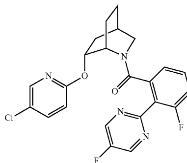
((1S,4R,6R)-6-((5-chloropyridin-2-yl)oxy)-2-azabicyclo[2.2.2]octan-2-yl)(4-fluoro-2-(pyrimidin-2-yl)phenyl)methanone,
