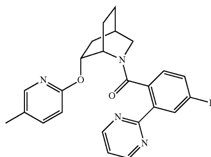
(4-fluoro-2-(pyrimidin-2-yl-phenyl)((1S,4R,6R)-6-((5-methylpyridin-2-yl)oxy)-2-azabicyclo[2.2.2]octan-2-yl)methanone,
