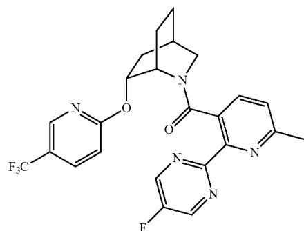
(2-(5-fluoropyrimidin-2-yl)-6-methylpyridin-3-yl)((1S,4R,6R)-6-((5-(trifluoromethyl)pyridin-2-yl)oxy)-2-azabicyclo[2.2.2]octan-2-yl)methanone
