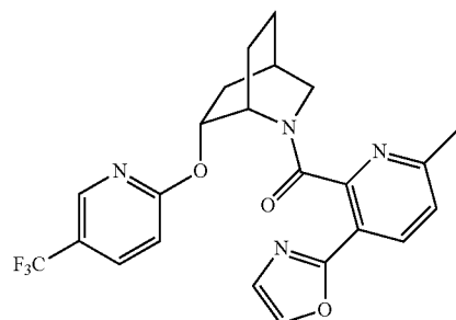
(6-methyl-3-(oxazol-2-yl)pyridin-2-yl)((1S,4R,6R)-6-((5-(trifluoromethyl)pyridin-2-yl)oxy)-2-azabicyclo[2.2.2]octan-2-yl)methanone
