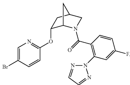
((1S,4R,6R)-6-((5-bromopyridin-2-yl)oxy)-2-azabicyclo[2.2.1]heptan-2-yl)(4-fluoro-2-(2H-1,2,3-triazol-2-yl)phenyl)methanone
