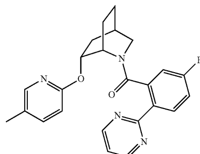
(5-fluoro-2-(pyrimidin-2-yl-phenyl)((1S,4R,6R)-6-((5-methylpyridin-2-yl)oxy)-2-azabicyclo[2.2.2]octan-2-yl)methanone,
