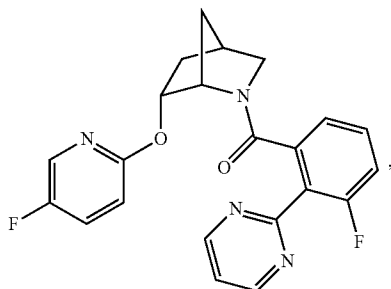
(3-fluoro-2-(pyrimidin-2-yl)phenyl)((1S,4R,6R)-6-((5-fluoropyridin-2-yl)oxy)-2-azabicyclo[2.2.1]heptan-2-yl)methanone
