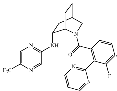
(3-fluoro-2-(pyrimidin-2-yl)phenyl)((1S,4R,6R)-6-((5-(trifluoromethyl)pyrazin-2-yl)amino)-2-azabicyclo[2.2.2]octan-2-yl)methanone
