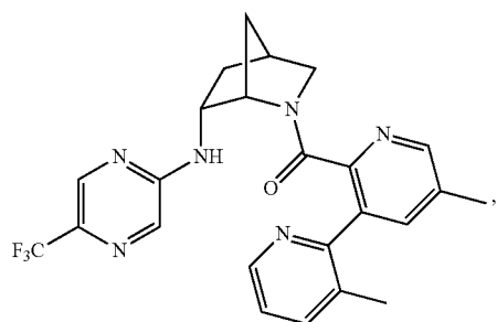
(3,5'-dimethyl-[2,3'-bipyridin]-2'-yl)((1S,4S,6R)-6-((5-(trifluoromethyl)pyrazin-2-yl)amino)-2-azabicyclo[2.2.1]heptan-2-yl)methanone
