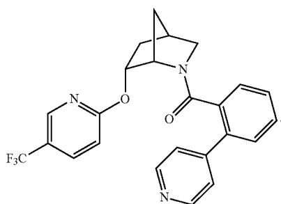
(2-(pyridin-4-yl)phenyl)((1S,4R,6R)-6-((5-(trifluoromethyl)pyridin-2-yl)oxy)-2-azabicyclo[2.2.1]heptan-2-yl)methanone
