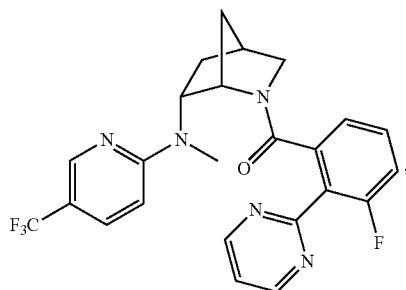
(3-fluoro-1-(pyrimidin-2-yl)phenyl)((1S,4S,6R)-6-(methyl(5-(trifluoromethyl)pyridin-2-yl)amino)-2-azabicyclo[2.2.1]heptan-2-yl)methanone
