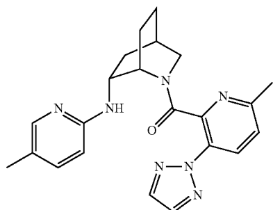
(6-methyl-3-(2H-1,2,3-triazol-2-yl)pyridin-2-yl)((1S,4R,6R)-6-((5-methylpyridin-2-yl)amino)-2-azabicyclo[2.2.2]octan-2-yl)methanone
