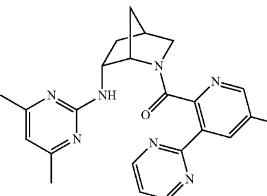
((1S,4S,6R)-6-((4,6-dimethylpyrimidin-2-yl)amino)-2-azabicyclo[2.2.1]heptan-2-yl)(5-methyl-3-(pyrimidin-2-yl)pyridin-2-yl)methanone,
