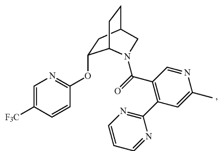
(6-methyl-4-(pyrimidin-2-yl)pyridin-3-yl)((1S,4R,6R)-6-((5-trifluoromethyl)pyridin-2-yl)oxy)-2-azabicyclo[2.2.2]octan-2-yl)methanone
