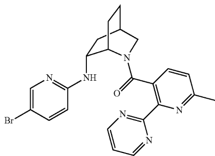
((1S,4R,6R)-6-((5-bromopyridin-2-yl)amino)-2-azabicyclo[2.2.2]octan-2-yl)(6-methyl-2-(pyrimidin-2-yl)pyridin-3-yl)methanone
