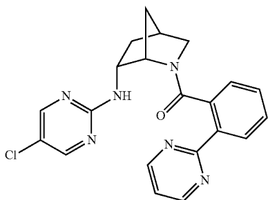
((1S,4S,6R)-6-((5-chloropyrimidin-2-yl)amino)-2-azabicyclo[2.2.1]heptan-2-yl)(2-(pyrimidin-2-yl)phenyl)methanone
