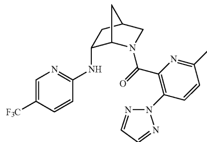
(6-methyl-3-(2H-1,2,3-triazol-2-yl)pyridin-2-yl)((1S,4S,6R)-6-((5-(trifluoromethyl)pyridin-2-yl)amino)-2-azabicyclo[2.2.1]heptan-2-yl)methanone
