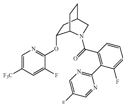
(3-fluoro-2-(fluoropyrimidin-2-yl)phenyl)((1S,4R,6R)-6-((3-fluoro-5-(trifluoromethyl)pyridin-2-yl)oxy)-2-azabicyclo[2.2.2]octan-2-yl)methanone.
