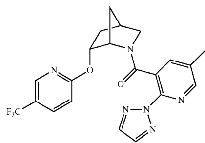
(5-methyl-2-(2H-1,2,3-triazol-2-yl)pyridin-3-yl)((1S,4R,6R)-6-((5-(trifluoromethyl)pyridin-2-yl)oxy)-2-azabicyclo[2.2.1]heptan-2-yl)methanone
