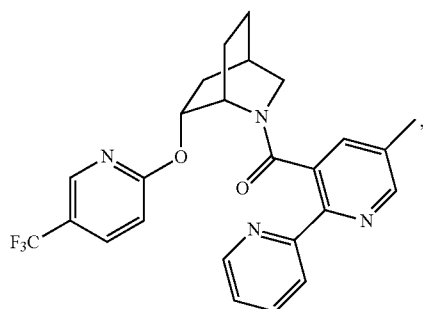
(5-methyl-[2,2'-bipyridin]-3-yl)((1S,4R,6R)-6-((5-(trifluoromethyl)pyridin-2-yl)oxy)-2-azabicyclo[2.2.2]octan-2-yl)methanone
