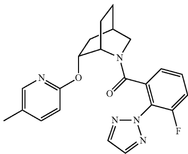
(6-fluoro-2-(2H-1,2,3-triazol-2-yl)phenyl)((1S,4R,6R)-6-((5-methylpyridin-2-yl)oxy)-2-azabicyclo[2.2.2]octan-2-yl)methanone,
