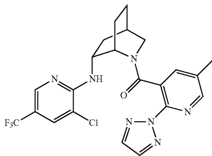
((1S,4R,6R)-6-((3-chloro-5-(trifluoromethyl)pyridin-2-yl)amino-2-azabicyclo[2.2.2]octan-2-yl)(5-methyl-2-(2H-1,2,3-triazol-2-yl)pyridin-3-yl)methanone
