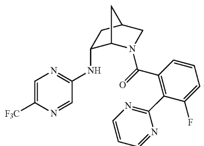
(3-fluoro-2-(pyrimidin-2-yl)phenyl)((1S,4S,6R)-6-((5-(trifluoromethyl)pyrazin-2-yl)amino)-2-azabicyclo[2.2.1]heptan-2-yl)methanone
