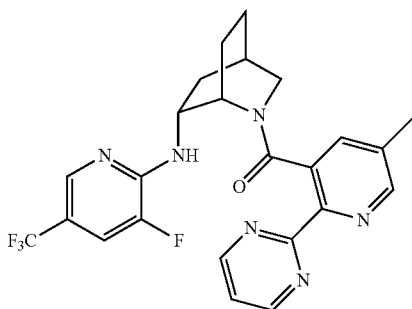
Example 536
