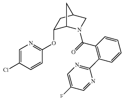
((1S,4R,6R)-6-((5-chloropyridin-2-yl)oxy)-2-azabicyclo[2.2.1]heptan-2-yl)(2-(5-fluoropyrimidin-2-yl)phenyl)methanone
