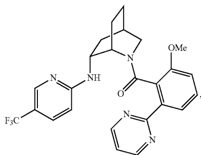
(2-methoxy-6-(pyrimidin-2-yl)phenyl)((1S,4R,6R)-6-((5-(trifluoromethyl)pyridin-2-yl)amino)-2-azabicyclo[2.2.2]octan-2-yl)methanone
