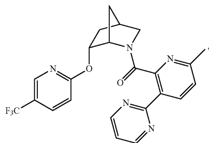
(6-methyl-3-(pyrimidin-2-yl)pyridin-2-yl)((1S,4R,6R)-6-((5-(trifluoromethyl)pyridin-2-yl)oxy)-2-azabicyclo[2.2.1]-heptan-2-yl)methanone
