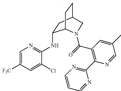
((1S,4R,6R)-6-((3-chloro-5-(trifluoromethyl)pyridin-2-yl)amino-2-azabicyclo[2.2.2]octan-2-yl)(5-methyl-2-(pyrimidin-2-yl)pyridin-3-yl)methanone
