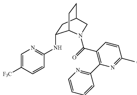
(6-methyl-[2,2'-bipyridin]-3-yl)((1S,4R,6R)-6-((5-(trifluoromethyl)pyridin-2-yl)amino)-2-azabicyclo[2.2.2]octan-2-yl)methanone
