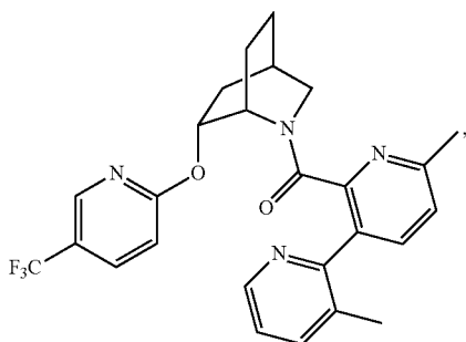
(3,6'-dimethyl-[2,3'-bipyridin]-2'-yl)((1S,4R,6R)-6-((5-(trifluoromethyl)pyridin-2-yl)oxy)-2-azabicyclo[2.2.2]octan-2-yl)methanone
