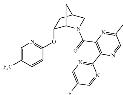
(2-(5-fluoropyrimidin-2-yl)-5-methylpyridin-3-yl)((1S,4R,6R)-6-((5-(trifluoromethyl)pyridin-2-yl)oxy)-2-azabicyclo[2.2.1]heptan-2-yl)methanone
