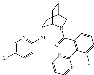
((1S,4R,6R)-6-((5-bromopyridin-2-yl)amino)-2-azabicyclo[2.2.2]octan-2-yl)(3-fluoro-2-(pyrimidin-2-yl)phenyl)methanone
