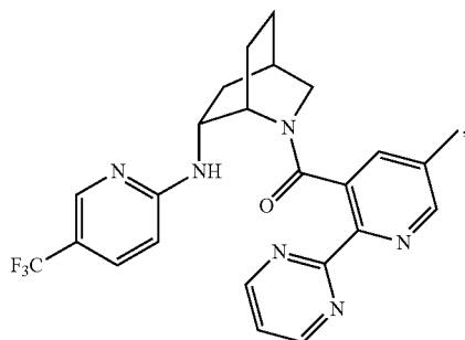
(5-methyl-2-(pyrimidin-2-yl)pyridin-3-yl)((1S,4R,6R)-6-((5-(trifluoromethyl)pyridin-2-yl)amino)-2-azabicyclo[2.2.2]octan-2-yl)methanone
