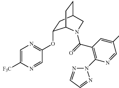
Example 420
