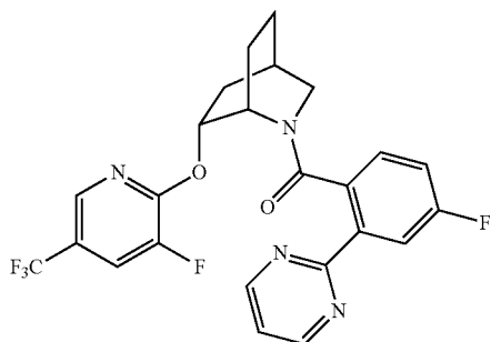
(4-fluoro-2-(pyrimidin-2-yl)phenyl)((1S,4R,6R)-6-((3-fluoro-5-(trifluoromethyl)pyridin-2-yl)oxy)-2-azabicyclo[2.2.2]octan-2-yl)methanone,
