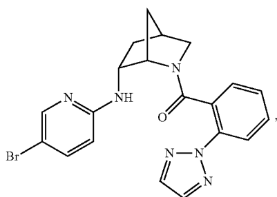
(2-(2H-1,2,3-triazol-2-yl)phenyl)((1S,4S,6R)-6-((5-bromopyridin-2-yl)amino)-2-azabicyclo[2.2.1]heptan-2-yl)methanone
