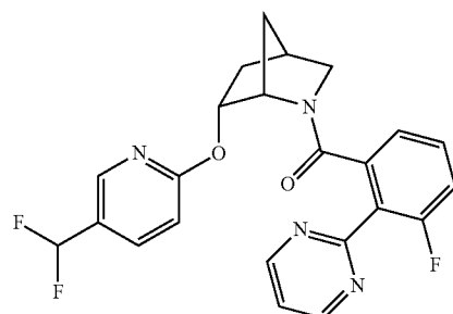
((1S,4R,6R)-6-((5-(difluoromethyl)pyridin-2-yl)oxy)-2-azabicyclo[2.2.1]heptan-2-yl)(3-fluoro-2-(pyrimidin-2-yl)phenyl)methanone
