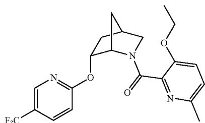
(3-ethoxy-6-methylpyridin-2-yl)((1S,4R,6R)-6-((5-(trifluoromethyl)pyridin-2-yl)oxy)-2-azabicyclo[2.2.1]heptan-2-yl)methanone
