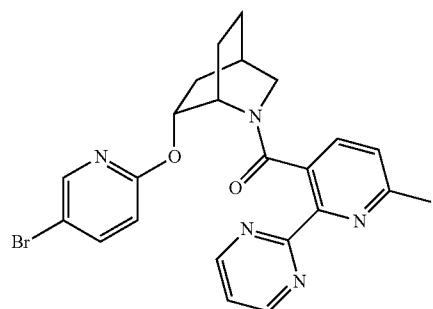
((1S,4R,6R)-6-((5-bromopyridin-2-yl)oxy)-2-azabicyclo[2.2.2]octan-2-yl)(6-methyl-2-(pyrimidin-2-yl)pyridin-3-yl)methanone
