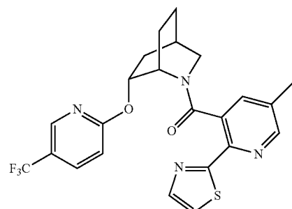
(5-methyl-2-(thiazol-2-yl)pyridin-3-yl)((1S,4R,6R)-6-((5-(trifluoromethyl)pyridin-2-yl)oxy)-2-azabicyclo[2.2.2]octan-2-yl)methanone,
