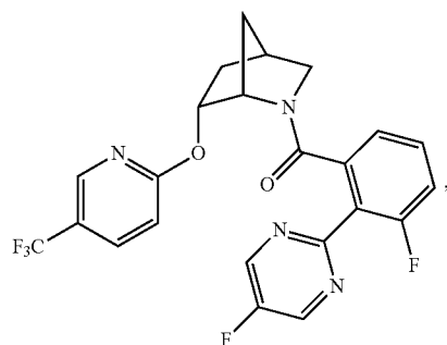
(3-fluoro-2-(5-fluoropyrimidin-2-yl)phenyl)((1S,4R,6R)-6-((5-(trifluoromethyl)pyridin-2-yl)oxy)-2-azabicyclo[2.2.1]heptan-2-yl)methanone
