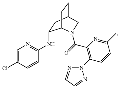
((1S,4R,6R)-6-((5-chloropyridin-2-yl)amino)-2-azabicyclo[2.2.2]octan-2-yl)(6-methyl-3-(2H-1,2,3-triazol-2-yl)pyridin-2-yl)methanone
