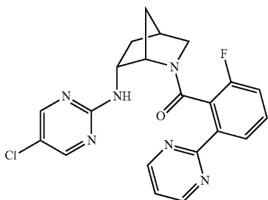
((1S,4S,6R)-6-((5-chloropyrimidin-2-yl)amino)-2-azabicyclo[2.2.1]heptan-2-yl)(2-fluoro-6-(pyrimidin-2-yl)phenyl)methanone
