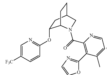
(4-methyl-3-(oxazol-2-yl)pyridin-2-yl)((1S,4R,6R)-6-((5-(trifluoromethyl)pyridin-2-yl)oxy)-2-azabicyclo[2.2.2]octan-2-yl)methanone
