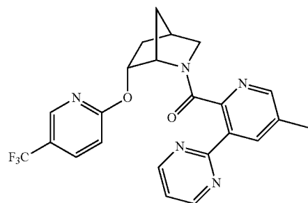
(5-methyl-3-(pyrimidin-2-yl)pyridin-2-yl)((1S,4R,6R)-6-((5-(trifluoromethyl)pyridin-2-yl)oxy)-2-azabicyclo[2.2.1]heptan-2-yl)methanone
