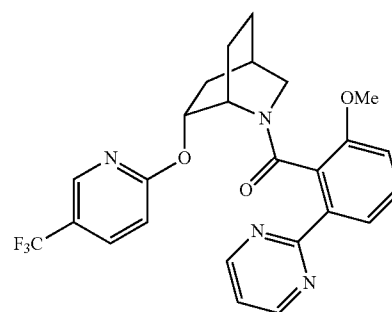
(2-methoxy-6-(pyrimidin-2-yl)phenyl)-((1S,4R,6R)-6-((5-(trifluoromethyl)pyridin-2-yl)oxy)-2-azabicyclo[2.2.2]octan-2-yl)methanone
