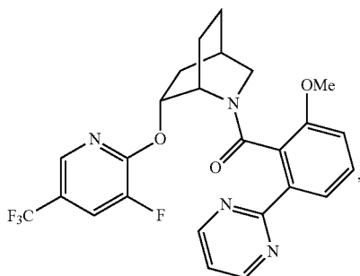
((1S,4R,6R)-6-((3-fluoro-5-(trifluoromethyl)pyridin-2-yl)oxy)-2-azabicyclo[2.2.2]octan-2-yl)(2-methoxy-6-(pyrimidin-2-yl)phenyl)methanone
