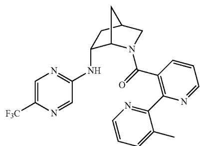
(3'-methyl-[2,2'-bipyridin]-3-yl)((1S,4S,6R)-6-((5-(trifluoromethyl)pyrazin-2-yl)amino)-2-azabicyclo[2.2.1]heptan-2-yl)methanone,
