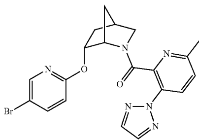
((1S,4R,6R)-6-((5-bromopyridin-2-yl)oxy)-2-azabicyclo[2.2.1]heptan-2-yl)(6-methyl-3-(2H-1,2,3-triazol-2-yl)pyridin-2-yl)methanone
