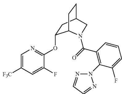
(3-fluoro-2-(2H-1,2,3-triazol-2-yl)phenyl)((1S,4R,6R)-6-((3-fluoro-5-(trifluoromethyl)pyridin-2-yl)oxy)-2-azabicyclo[2.2.2]octan-2-yl)methanone,
