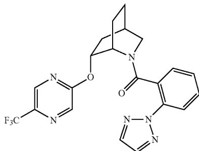
Example 428
