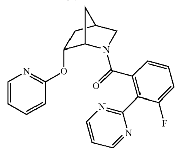
(3-fluoro-2-(pyrimidin-2-yl)phenyl)((1S,4R,6R)-6-(pyridin-2-yloxy)-2-azabicyclo[2.2.1]heptan-2-yl)methanone
