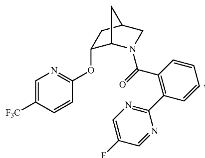
(2-(5-fluoropyrimidin-2-yl)phenyl)((1S,4R,6R)-6-((5-(trifluoromethyl)pyridin-2-yl)oxy)-2-azabicyclo[2.2.1]heptan-2-yl)methanone
