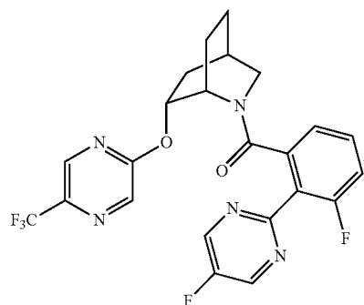
(3-fluoro-2-(5-fluoropyrimidin-2-yl)phenyl)((1S,4R,6R)-6-((5-(trifluoromethyl)pyrazin-2-yl)oxy)-2-azabicyclo[2.2.2]octan-2-yl)methanone
