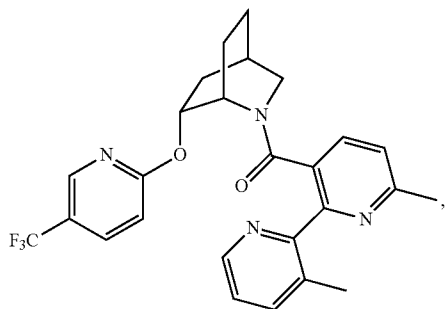
(3,6'-dimethyl-[2,2'-bipyridin]-3-yl)((1S,4R,6R)-6-((5-(trifluoromethyl)pyridin-2-yl)oxy)-2-azabicyclo[2.2.2]octan-2-yl)methanone
