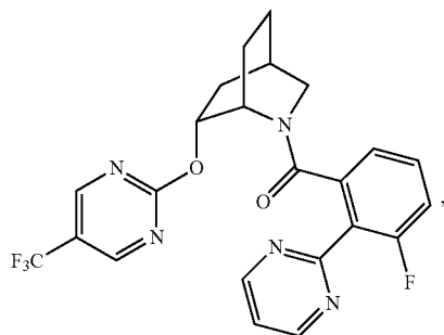
(3-fluoro-2-(pyrimidin-2-yl)phenyl)((1S,4R,6R)-6-((5-(trifluoromethyl)pyrimidin-2-yl)oxy)-2-azabicyclo[2.2.2]octan-2-yl)methanone
