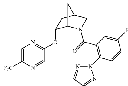
(5-fluoro-2-(2H-1,2,3-triazol-2-yl)phenyl)((1S,4R,6R)-6-((5-(trifluoromethyl)pyrazin-2-yl)oxy)-2-azabicyclo[2.2.1]heptan-2-yl)methanone
