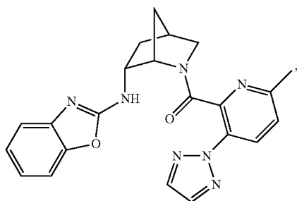
((1S,4S,6R)-6-(benzo[d]oxazol-2-ylamino)-2-azabicyclo[2.2.1]heptan-2-yl)(6-methyl-3-(2H-1,2,3-triazol-2-yl)pyridin-2-yl)methanone
