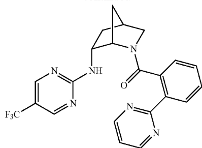
(2-(pyrimidin-2-yl)phenyl)((1S,4S,6R)-6-((5-(tri fluoromethyl)pyrimidin-2-yl)amino)-2-azabicyclo[2.2.1]heptan-2-yl)methanone
