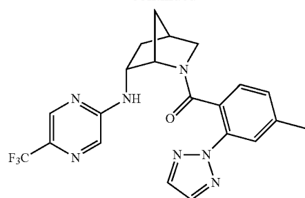
(4-methyl-2-(2H-1,2,3-triazol-2-yl)phenyl)((1S,4S,6R)-6-((5-(trifluoromethyl)pyrazin-2-yl)amino)-2-azabicyclo[2.2.1]heptan-2-yl)methanone
