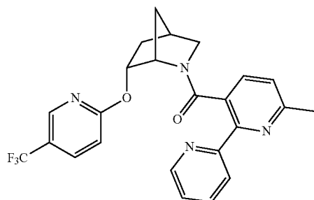
(6'-methyl-[2,2'-bipyridin]-3-yl)((1S,4R,6R)-6-((5-(trifluoromethyl)pyridin-2-yl)oxy)-2-azabicyclo[2.2.1]heptan-2-yl)methanone
