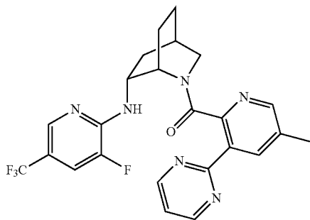
Example 559
