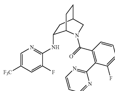
(3-fluoro-2-(pyrimidin-2-yl)phenyl)((1S,4R,6R)-6-((3-fluoro-5-(trifluoromethyl)pyridin-2-yl)amino)-2-azabicyclo[2.2.2]octan-2-yl)methanone
