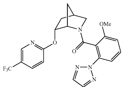
(2-Methoxy-6-(2H-1,2,3-triazol-2-yl)phenyl)((1S,4R,6R)-6-((5-(trifluoromethyl)pyridin-2-yl)oxy)-2-azabicyclo[2.2.1]heptan-2-yl)methanone
