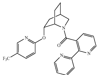
[2,2'-bipyridin]-3-yl((1S,4R,6R)-6-((5-(trifluoromethyl)pyridin-2-yl)oxy)-2-azabicyclo[2.2.2]octan-2-yl)methanone
