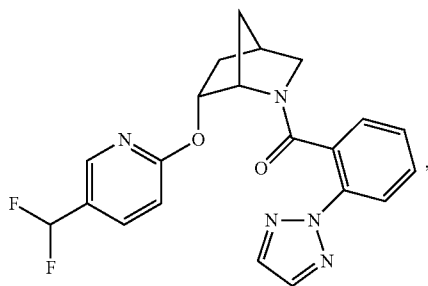
(2-(2H-1,2,3-triazol-2-yl)phenyl)((1S,4R,6R)-6-((5-(difluoromethyl)pyridin-2-yl)oxy)-2-azabicyclo[2.2.1]heptan-2-yl)methanone
