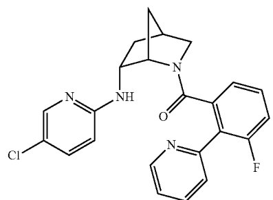
((1S,4S,6R)-6-((5-chloropyridin-2-yl)amino)-2-azabicyclo[2.2.1]heptan-2-yl)(3-fluoro-2-(pyrimidin-2-yl)phenyl)methanone
