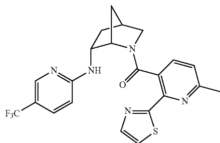
(6-methyl-2-(thiazol-2-yl)pyridin-3-yl)((1S,4S,6R)-6-((5-(trifluoromethyl)pyridin-2-yl)amino)-2-azabicyclo[2.2.1]heptan-2-yl)methanone,
