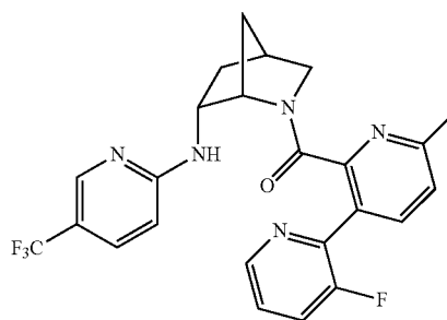
Example 395
