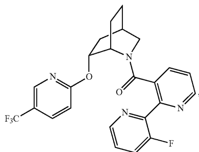
(3'-fluoro-[2,2'-bipyridin]-3-yl)((1S,4R,6R)-6-((5-(trifluoromethyl)pyridin-2-yl)oxy)-2-azabicyclo[2.2.2]octan-2-yl)methanone
