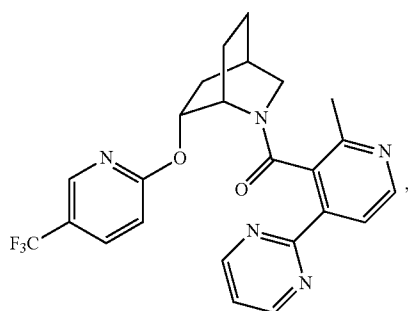
(2-methyl-4-(pyrimidin-2-yl)pyridin-3-yl)((1S,4R,6R)-6-((5-trifluoromethyl)pyridin-2-yl)oxy)-2-azabicyclo[2.2.2]octan-2-yl)methanone
