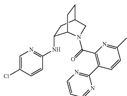
((1S,4R,6R)-6-((5-chloropyridin-2-yl)amino)-2-azabicyclo[2.2.2]octan-2-yl)(6-methyl-2-(pyrimidin-2-yl)pyridin-2-yl)methanone
