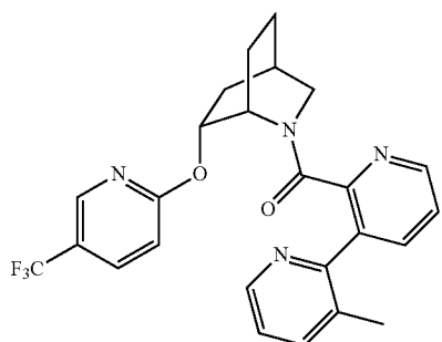
(3-methyl-[2,3'-bipyridin]-2'-yl)((1S,4R,6R)-6-((5-(trifluoromethyl)pyridin-2-yl)oxy)-2-azabicyclo[2.2.2]octan-2-yl)methanone
