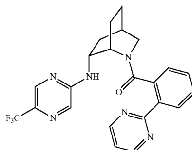
(2-(pyrimidin-2-yl)phenyl)((1S,4R,6R)-6-((5-(trifluoromethyl)pyrazin-2-yl)amino)-2-azabicyclo[2.2.2]octan-2-yl)methanone
