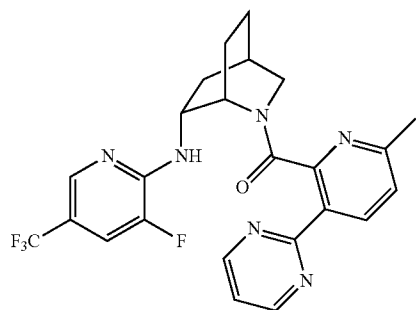
((1S,4R,6R)-6-((3-fluoro-5-(trifluoromethyl)pyridin-2-yl)amino)-2-azabicyclo[2.2.2]octan-2-yl)(6-methyl-3-(pyrimidin-2-yl)pyridin-2-yl)methanone
