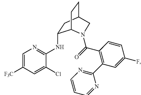
((1S,4R,6R)-6-((3-chloro-5-(trifluoromethyl)pyridin-2-yl)amino-2-azabicyclo[2.2.2]octan-2-yl)(4-fluoro-2-(pyrimidin-2-yl)phenyl)methanone
