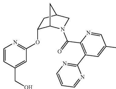
((1S,4R,6R)-6-((5-(hydroxymethyl)pyridin-2-yl)oxy)-2-azabicyclo[2.2.1]heptan-2-yl)(5-methyl-3-(pyrimidin-2-yl)pyridin-2-yl)methanone
