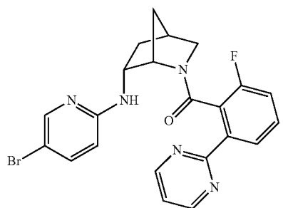
((1S,4S,6R)-6-((5-bromopyridin-2-yl)amino)-2-azabicyclo[2.2.1]heptan-2-yl)(2-fluoro-6-(pyrimidin-2-yl)phenyl)methanone
