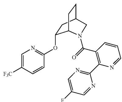
(2-(5-fluoropyrimidin-2-yl)pyridin-3-yl)((1S,4R,6R)-6-((5-(trifluoromethyl)pyridin-2-yl)oxy)-2-azabicyclo[2.2.2]octan-2-yl)methanone
