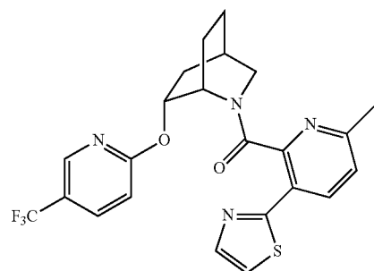
(6-methyl-3-(thiazol-2-yl)pyridin-2-yl)((1S,4R,6R)-6-((5-(trifluoromethyl)pyridin-2-yl)oxy)-2-azabicyclo[2.2.2]octan-2-yl)methanone
