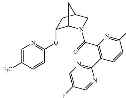
Example 323
