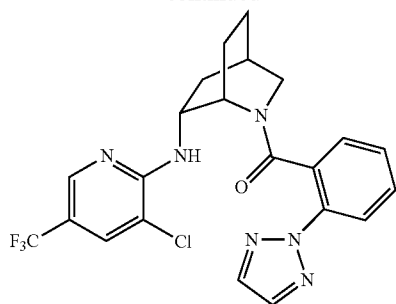
(2-(2H-1,2,3-triazol-2-yl)phenyl)((1S,4R,6R)-6-((3-chloro-5-(trifluoromethyl)pyridin-2-yl)amino)-2-azabicyclo[2.2.2]octan-2-yl)methanone
