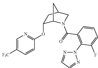
(3-fluoro-2-(2H-1,2,3-triazol-2-yl)phenyl)((1S,4R,6R)-6-((5-(trifluoromethyl)pyridin-2-yl)oxy)-2-azabicyclo[2.2.1]heptan-2-yl)methanone
