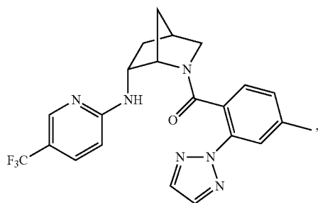
(4-methyl-2-(2H-1,2,3-triazol-2-yl)phenyl)((1S,4S,6R)-6-((5-(trifluoromethyl)pyridin-2-yl)amino)-2-azabicyclo[2.2.1]heptan-2-yl)methanone
