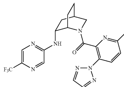
(R/S)-(6-methyl-3-(2H-1,2,3-triazol-2-yl)pyridin-2-yl) (6-((5-(trifluoromethyl)pyrazin-2-yl)amino)-2-azabicyclo[2.2.2]octan-2-yl)methanone
