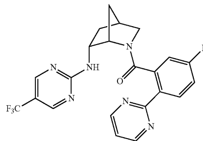
(5-fluoro-2-(pyrimidin-2-yl)phenyl)((1S,4S,6R)-6-((5-(trifluoromethyl)pyrimidin-2-yl)amino)-2-azabicyclo[2.2.1]heptan-2-yl)methanone
