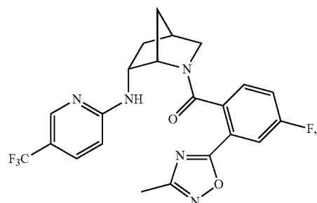
(4-fluoro-2-(3-methyl-1,2,4-oxadiazol-5-yl)phenyl)((1S,4R,6R)-6-((5-(trifluoromethyl)pyridin-2-yl)oxy)-2-azabicyclo[2.2.1]heptan-2-yl)methanone
