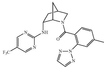
(4-methyl-2-(2H-1,2,3-triazol-2-yl)phenyl)((1S,4S,6R)-6-((5-(trifluoromethyl)pyrimidin-2-yl)amino)-2-azabicyclo[2.2.1]heptan-2-yl)methanone
