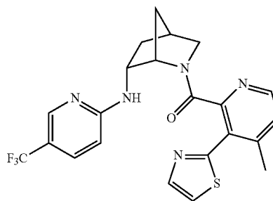
(4-methyl-3-(thiazol-2-yl)pyridin-2-yl)((1S,4S,6R)-6-((5-(trifluoromethyl)pyridin-2-yl)amino)-2-azabicyclo[2.2.1]heptan-2-yl)methanone,
