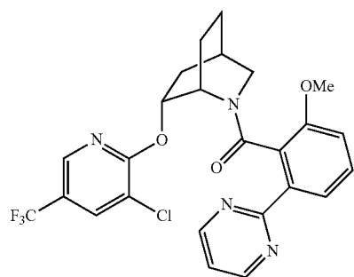
((1S,4R,6R)-6-((3-chloro-5-(trifluoromethyl)pyridin-2-yl)oxy)-2-azabicyclo[2.2.2]octan-2-yl)(2-methoxy-6-(pyrimidin-2-yl)phenyl)methanone
