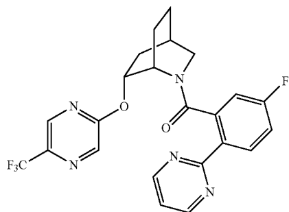
(5-fluoro-2-(pyrimidin-2-yl)phenyl)((1S,4R,6R)-6-((5-(trifluoromethyl)pyrazin-2-yl)oxy)-2-azabicyclo[2.2.2]octan-2-yl)methanone,
