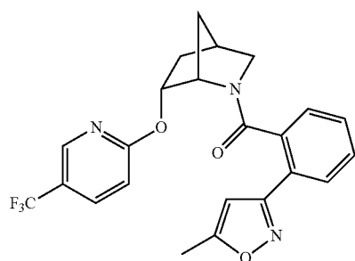
(2-(5-methylisoxazol-3-yl)phenyl)((1S,4R,6R)-6-((5-(trifluoromethyl)pyridin-2-yl)oxy)-2-azabicyclo[2.2.1]heptan-2-yl)methanone
