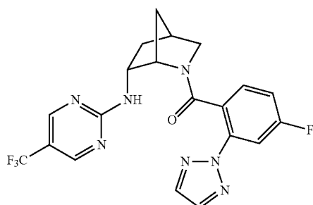
(4-fluoro-2-(2H-1,2,3-triazol-2-yl)phenyl)((1S,4S,6R)-6-((5-(trifluoromethyl)pyrimidin-2-yl)amino)-2-azabicyclo[2.2.1]heptan-2-yl)methanone
