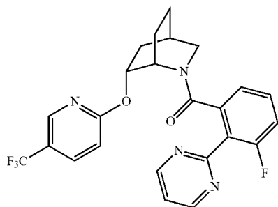
(R/S)-(3-fluoro-2-(pyrimidin-2-yl)phenyl) (6-((5-(trifluoromethyl)pyridin-2-yl)oxy)-2-azabicyclo[2.2.2]octan-2-yl)methanone
