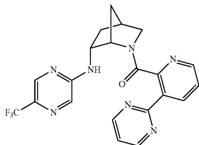
(3-(pyrimidin-2-yl)pyridin-2-yl)((1S,4S,6R)-6-((5-(trifluoromethyl)pyrazin-2-yl)amino)-2-azabicyclo[2.2.1]heptan-2-yl)methanone
