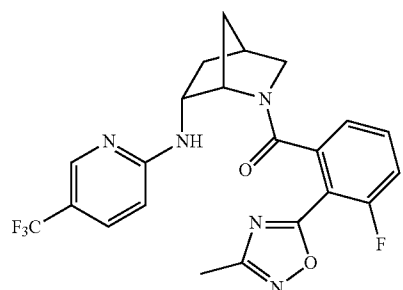
(3-fluoro-2-(3-methyl-1,2,4-oxadiazol-5-yl)phenyl)((1S,4S,6R)-6-((5-(trifluoromethyl)pyridin-2-yl)amino)-2-azabicyclo[2.2.1]heptan-2-yl)methanone
