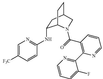
(3'-fluoro-[2,2'-bipyridin]-3-yl)((1S,4R,6R)-6-((5-(trifluoromethyl)pyridin-2-yl)amino)-2-azabicyclo[2.2.2]octan-2-yl)methanone
