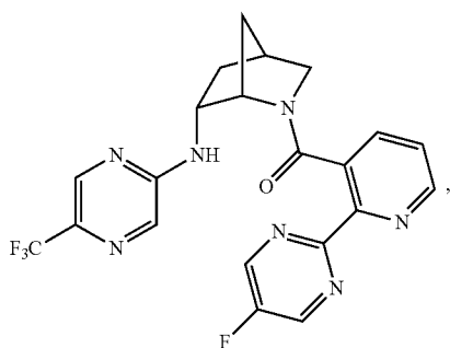
(2-(5-fluoropyrimidin-2-yl)pyridin-3-yl)((1S,4S,6R)-6-((5-(trifluoromethyl)pyrazin-2-yl)amino)-2-azabicyclo[2.2.1]heptan-2-yl)methanone
