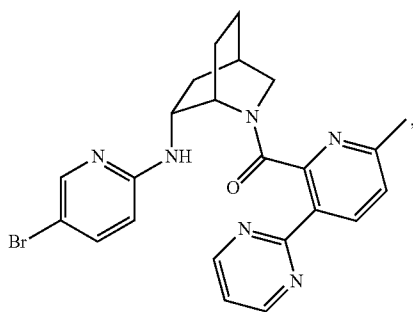
((1S,4R,6R)-6-((5-bromopyridin-2-yl)amino)-2-azabicyclo[2.2.2]octan-2-yl)(6-methyl-3-(pyrimidin-2-yl)pyridin-2-yl)methanone
