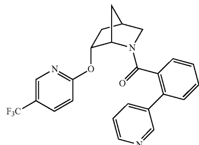
(2-(pyridin-3-yl)phenyl)((1S,4R,6R)-6-((5-(trifluoromethyl)pyridin-2-yl)oxy)-2-azabicyclo[2.2.1]heptan-2-yl)methanone
