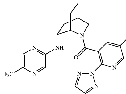
(5-methyl-2-(2H-1,2,3-triazol-2-yl)pyridin-3-yl)-((1S,4R,6R)-6-((5-(trifluoromethyl)pyrazin-2-yl)amino)-2-azabicyclo[2.2.2]octan-2-yl)methanone
