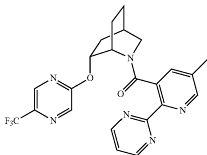
(5-methyl-2-(pyrimidin-2-yl)pyridin-3-yl)((1S,4R,6R)-6-((5-(trifluoromethyl)pyrazin-2-yl)oxy)-2-azabicyclo[2.2.2]octan-2-yl)methanone,
