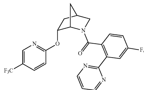
(R/S)-4-fluoro-2-(pyrimidin-2-yl)phenyl(6-((5-(trifluoromethyl)pyridin-2-yl)oxy)-2-azabicyclo[2.2.1]heptan-2-yl)methanone
