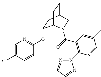
((1S,4R,6R)-6-((5-chloropyridin-2-yl)oxy)-2-azabicyclo[2.2.2]octan-2-yl)(5-methyl-2-(2H-1,2,3-triazol-2-yl)pyridin-3-yl)methanone,
