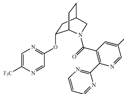
(6-methyl-2-(pyrimidin-2-yl)pyridin-3-yl)((1S,4R,6R)-6-((5-(trifluoromethyl)pyrazin-2-yl)oxy)-2-azabicyclo[2.2.2]octan-2-yl)methanone,
