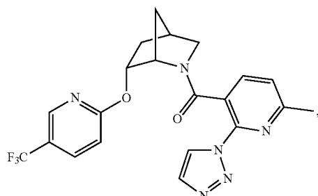
(6-methyl-2-(1H-1,2,3-triazol-1-yl)pyridin-3-yl)((1S,4R,6R)-6-((5-(trifluoromethyl)pyridin-2-yl)oxy)-2-azabicyclo[2.2.1]heptan-2-yl)methanone
