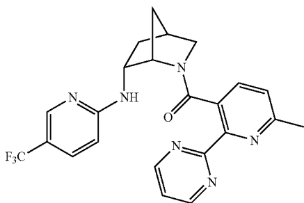
(6-methyl-2-(pyrimidin-2-yl)pyridin-3-yl)((1S,4S,6R)-6-((5-(trifluoromethyl)pyridin-2-yl)amino)-2-azabicyclo[2.2.1]heptan-2-yl)methanone,
