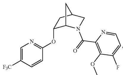
(3-fluoro-2-methoxyphenyl)((1S,4R,6R)-6-((5-(trifluoromethyl)pyridin-2-yl)oxy)-2-azabicyclo[2.2.1]heptan-2-yl)methanone
