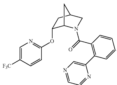
(2-(pyrazin-2-yl)phenyl)((1S,4R,6R)-6-((5-(trifluoromethyl)pyridin-2-yl)oxy)-2-azabicyclo[2.2.1]heptan-2-yl)methanone
