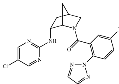
((1S,4S,6R)-6-((5-chloropyrimidin-2-yl)amino)-2-azabicyclo[2.2.1]heptan-2-yl)(5-fluoro-2-(2H-1,2,3-triazol-2-yl)phenyl)methanone
