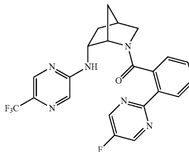
(2-(5-fluoropyrimidin-2-yl)phenyl)((1S,4S,6R)-6-((5-(trifluoromethyl)pyrazin-2-yl)amino)-2-azabicyclo[2.2.1]heptan-2-yl)methanone
