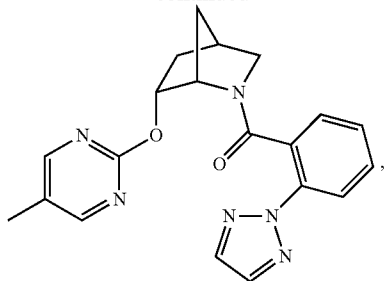
(2-(2H-1,2,3-triazol-2-yl)phenyl)((1S,4R,6R)-6-((5-methylpyrimidin-2-yl)oxy)-2-azabicyclo[2.2.1]heptan-2-yl)methanone
