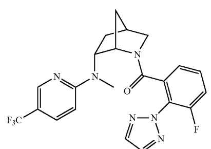
(3-fluoro-2-(2H-1,2,3-triazol-2-yl)phenyl)((1S,4S,6R)-6-methyl(5-(trifluoromethyl)pyridin-2-yl)amino)-2-azabicyclo[2.2.1]heptan-2-yl)methanone
