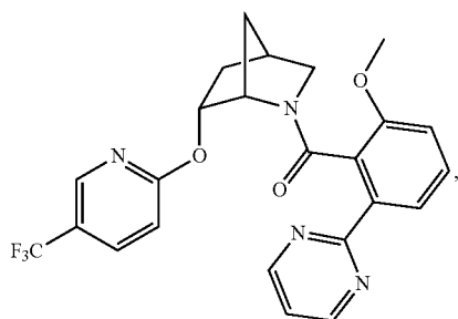
(2-methoxy-6-(pyrimidin-2-yl)phenyl)((1S,4R,6R)-6-((5-(trifluoromethyl)pyridin-2-yl)oxy)-2-azabicyclo[2.2.1]heptan-2-yl)methanone
