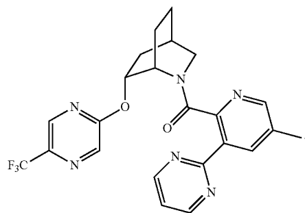
(5-methyl-3-(pyrimidin-2-yl)pyridin-2-yl)((1S,4R,6R)-6-((5-(trifluoromethyl)pyrazin-2-yl)oxy)-2-azabicyclo[2.2.2]octan-2-yl)methanone
