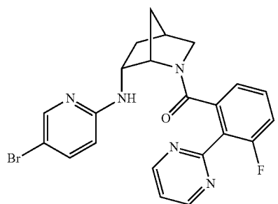
((1S,4S,6R)-6-((5-bromopyridin-2-yl)amino)-2-azabicyclo[2.2.1]heptan-2-yl)(3-fluoro-2-(pyrimidin-2-yl)phenyl)methanone
