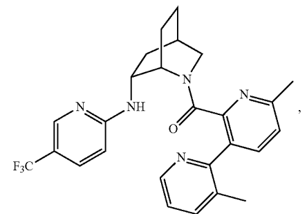
(3,6'-dimethyl-[2,3'-bipyridin]-2'-yl)((1S,4R,6R)-6-((5-(trifluoromethyl)pyridin-2-yl)amino)-2-azabicyclo[2.2.2]octan-2-yl)methanone
