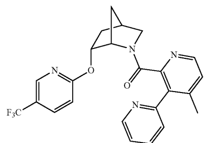
(4'-methyl-[2,3'-bipyridin]-2'-yl)((1S,4R,6R)-6-((5-(trifluoromethyl)pyridin-2-yl)oxy)-2-azabicyclo[2.2.1]heptan-2-yl)methanone
