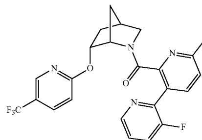
(3-fluoro-6-methyl-[2,2'-bipyridin]-3-yl)((1S,4R,6R)-6-((5-(trifluoromethyl)pyridin-2-yl)oxy)-2-azabicyclo[2.2.1]heptan-2-yl)methanone
