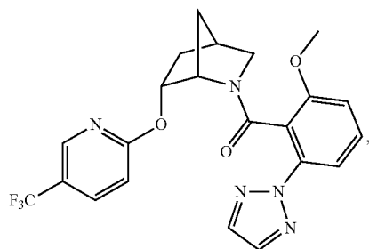
(R/S)-2-methoxy-6-(2H-1,2,3-triazol-2-yl)phenyl(6-((5-(trifluoromethyl)pyridin-2-yl)oxy)-2-azabicyclo[2.2.1]heptan-2-yl)methanone
