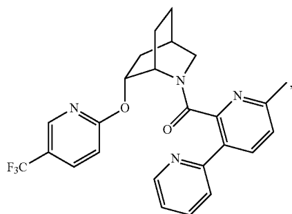
(6'-methyl-[2,3'-bipyridin]-2'-yl)((1S,4R,6R)-6-((5-(trifluoromethyl)pyridin-2-yl)oxy)-2-azabicyclo[2.2.2]octan-2-yl)methanone
