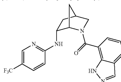
(1H-indazol-7-yl)((1S,4S,6R)-6-((5-(trifluoromethyl)pyridin-2-yl)amino)-2-azabicyclo[2.2.1]heptan-2-yl)methanone
