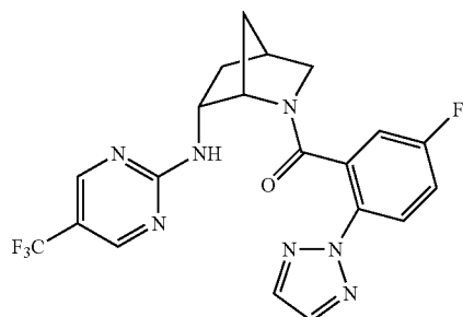
(5-fluoro-2-(2H-1,2,3-triazol-2-yl)phenyl)((1S,4S,6R)-6-((5-(trifluoromethyl)pyrimidin-2-yl)amino)-2-azabicyclo[2.2.1]heptan-2-yl)methanone
