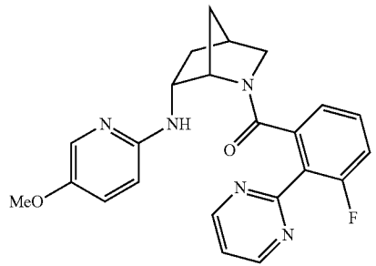
(3-fluoro-2-(pyrimidin-2-yl)phenyl)((1S,4S,6R)-6-((5-methoxypyridin-2-yl)amino)-2-azabicyclo[2.2.1]heptan-2-yl)methanone
