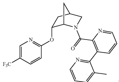
(3',4-dimethyl-[2,3'-bipyridin]-2'-yl)((1S,4R,6R)-6-((5-(trifluoromethyl)pyridin-2-yl)oxy)-2-azabicyclo[2.2.1]heptan-2-yl)methanone
