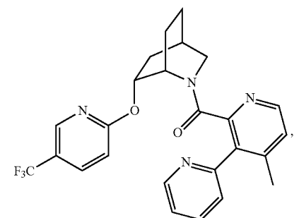
(4'-methyl-[2,3'-bipyridin]-2'-yl)((1S,4R,6R)-6-((5-(trifluoromethyl)pyridin-2-yl)oxy)-2-azabicyclo[2.2.2]octan-2-yl)methanone
