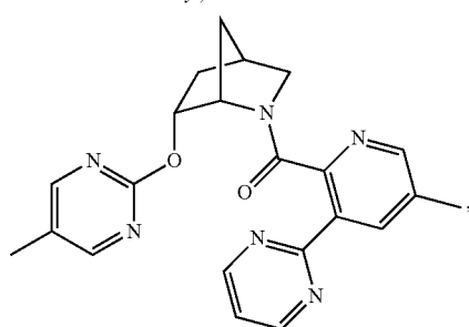
(5-methyl-3-(pyrimidin-2-yl)pyridin-2-yl)((1S,4R,6R)-6-((5-methylpyrimidin-2-yl)oxy)-2-azabicyclo[2.2.1]heptan-2-yl)methanone
