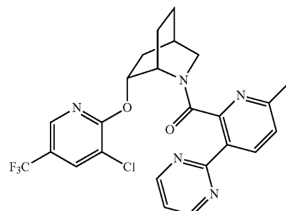
((1S,4R,6R)-6-((3-chloro-5-(trifluoromethyl)pyridin-2-yl)oxy)-2-azabicyclo[2.2.2]octan-2-yl)(6-methyl-3-(pyrimidin-2-yl)pyridin-2-yl)methanone,
