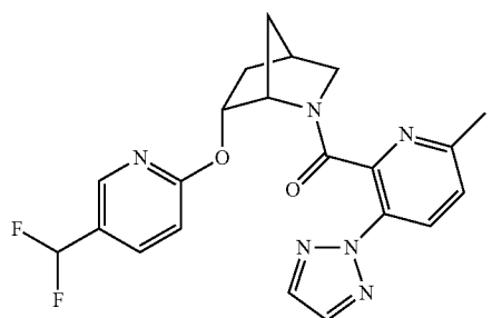
((1S,4R,6R)-6-((5-(difluoromethyl)pyridin-2-yl)oxy)-2-azabicyclo[2.2.1]heptan-2-yl)(6-methyl-3-(2H-1,2,3-triazol-2-yl)pyridin-2-yl)methanone
