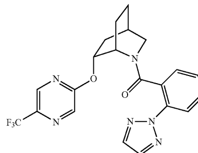
(2-(2H-1,2,3-triazol-2-yl)phenyl)((1S,4R,6R)-6-((5-(trifluoromethyl)pyrazin-2-yl)oxy)-2-azabicyclo[2.2.2]octan-2-yl)methanone,
