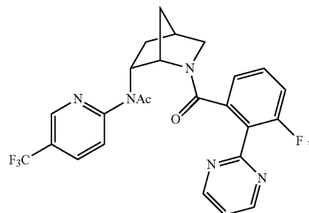
N-((1S,4S,6R)-2-(3-fluoro-2-(pyrimidin-2-yl)benzoyl)-2-azabicyclo[2.2.1]heptan-6-yl)-N-(5-(trifluoromethyl)pyridin-2-yl)acetamide
