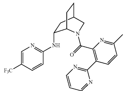
(6-methyl-3-(pyrimidin-2-yl)pyridin-2-yl)((1S,4R,6R)-6-((5-(trifluoromethyl)pyridin-2-yl)amino)-2-azabicyclo[2.2.2]octan-2-yl)methanone
