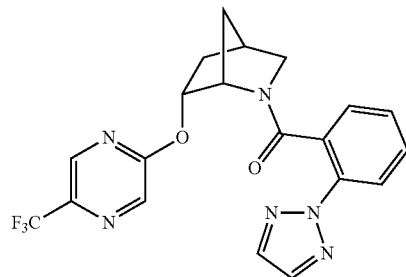
(R/S)-(2-(2H-1,2,3-triazol-2-yl)phenyl)(6-((5-(trifluoromethyl)pyrazin-2-yl)oxy)-2-azabicyclo[2.2.1]heptan-2-yl)methanone
