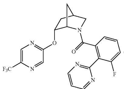
(3-fluoro-2-(pyrimidin-2-yl)phenyl)((1S,4R,6R)-6-((5-(trifluoromethyl)pyrazin-2-yl)oxy)-2-azabicyclo[2.2.1]heptan-2-yl)methanone
