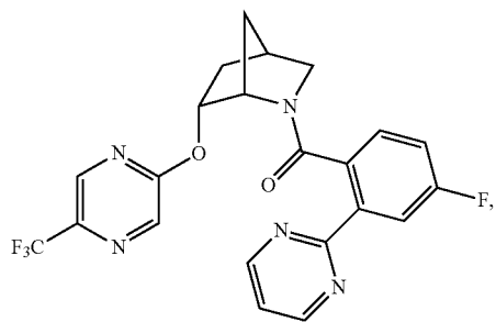
(4-fluoro-2-(pyrimidin-2-yl)phenyl)((1S,4R,6R)-6-((5-(trifluoromethyl)pyrazin-2-yl)oxy)-2-azabicyclo[2.2.1]heptan-2-yl)methanone
