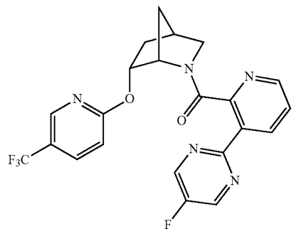
(3-(5-fluoropyrimidin-2-yl)pyridin-2-yl)((1S,4R,6R)-6-((5-(trifluoromethyl)pyridin-2-yl)oxy)-2-azabicyclo[2.2.1]heptan-2-yl)methanone
