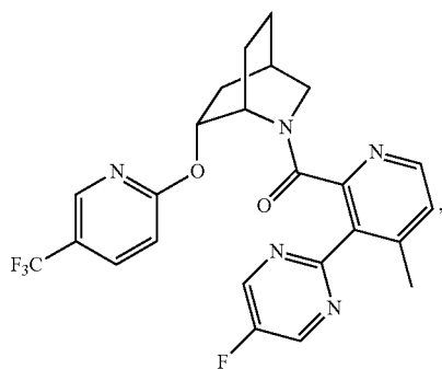
(3-(5-fluoropyrimidin-2-yl)-4-methylpyridin-2-yl)((1S,4R,6R)-6-((5-(trifluoromethyl)pyridin-2-yl)oxy)-2-azabicyclo[2.2.2]octan-2-yl)methanone
