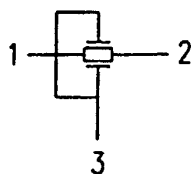
TRANSMISSION GATE STYLE SWITCH (S)
