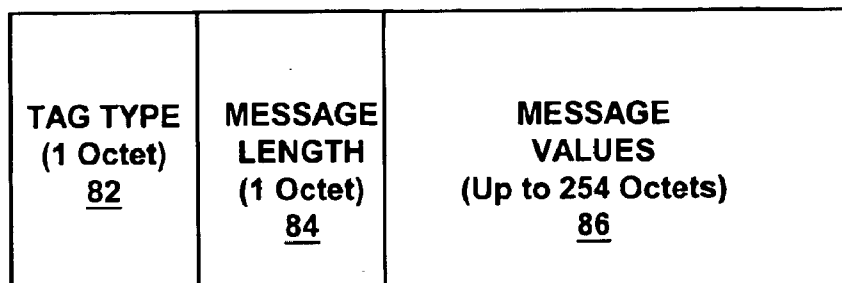
LOCATION-AWARE MESSAGE LAYOUT
