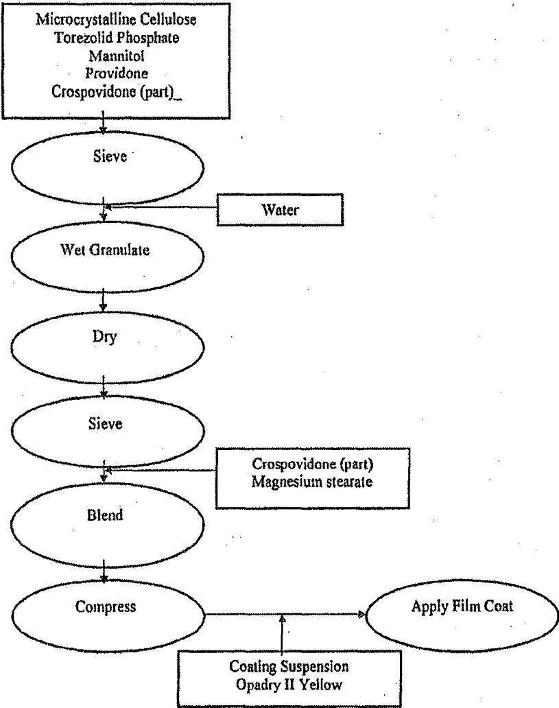
Torezolid Phosphate Tablet, 200 mg, Manufacturing Process Schematic
