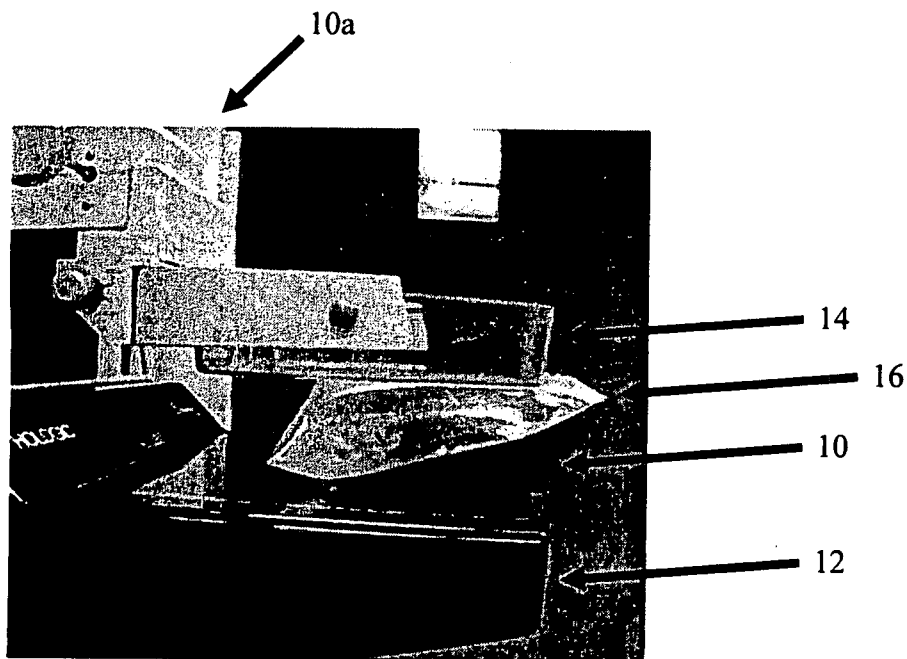
Figure 1 Air pillow side view
