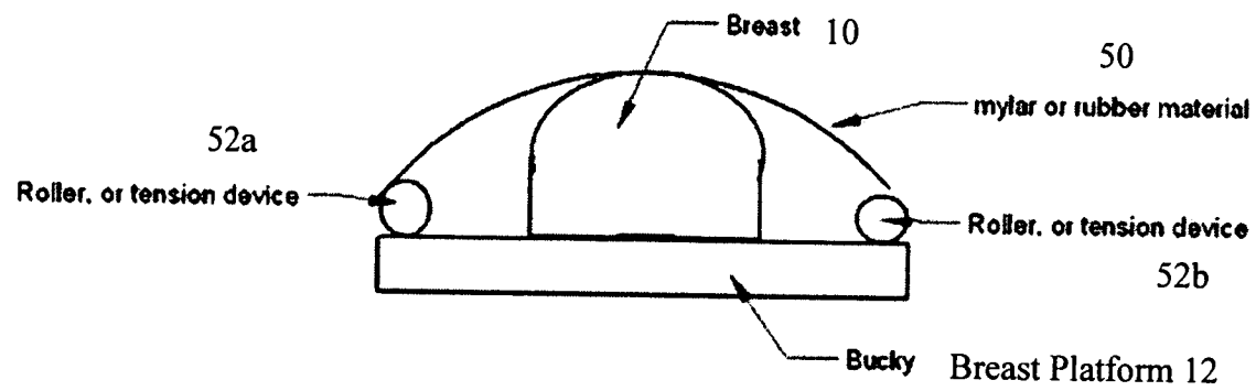
Figure 9 Compression system utilizing material stretched between two rods or rollers fastened to lower breast platform or Bucky
