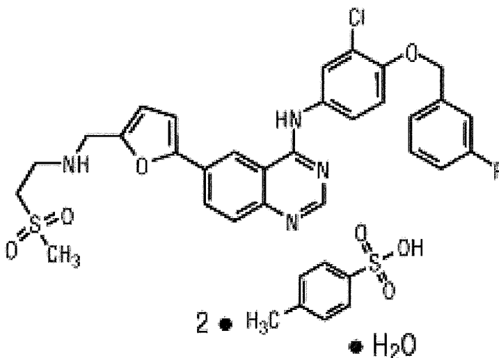
Lapatinib
