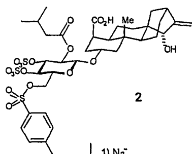
Reaction Scheme 1
