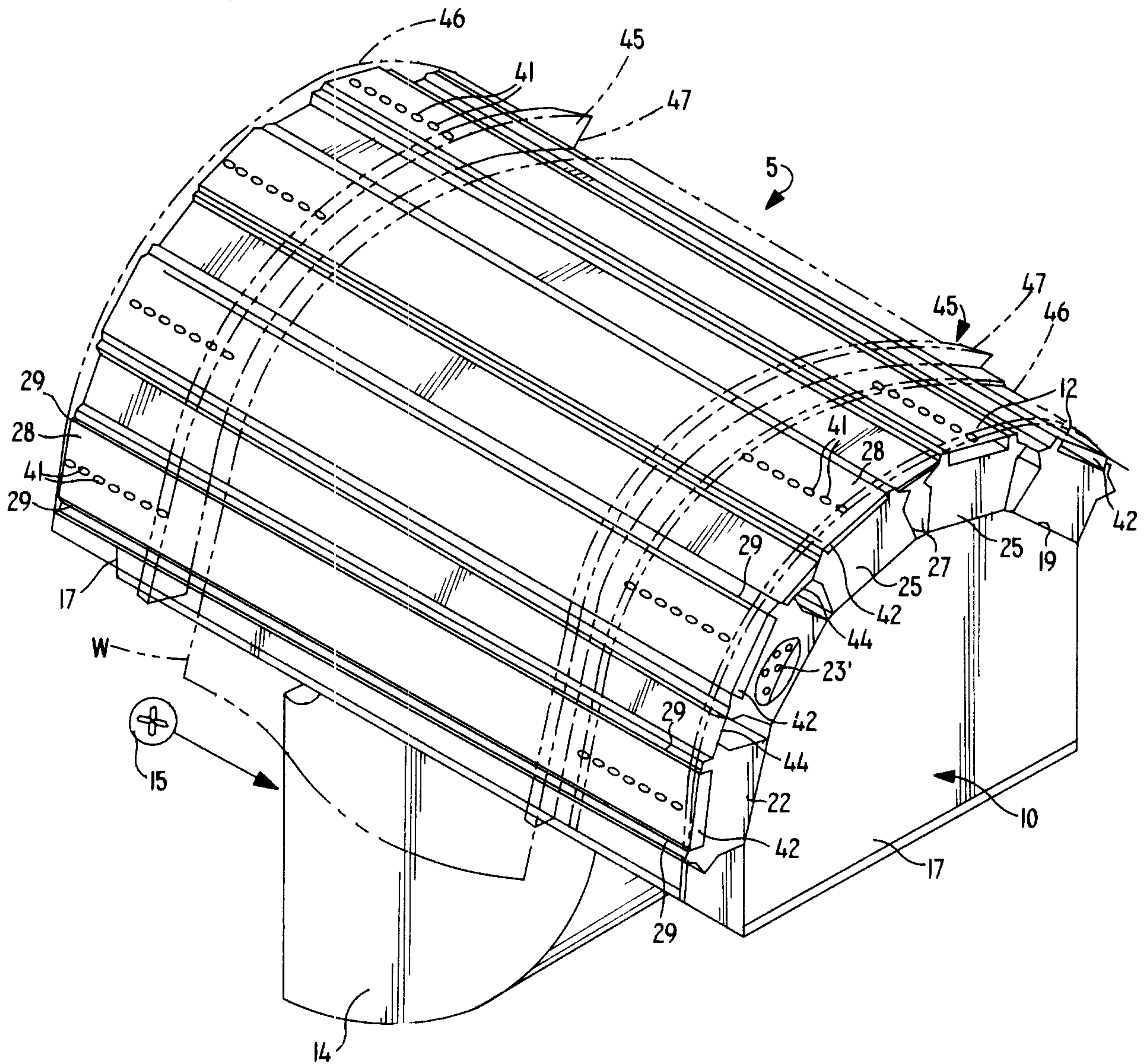
FIG. 1 (PRIOR ART)
