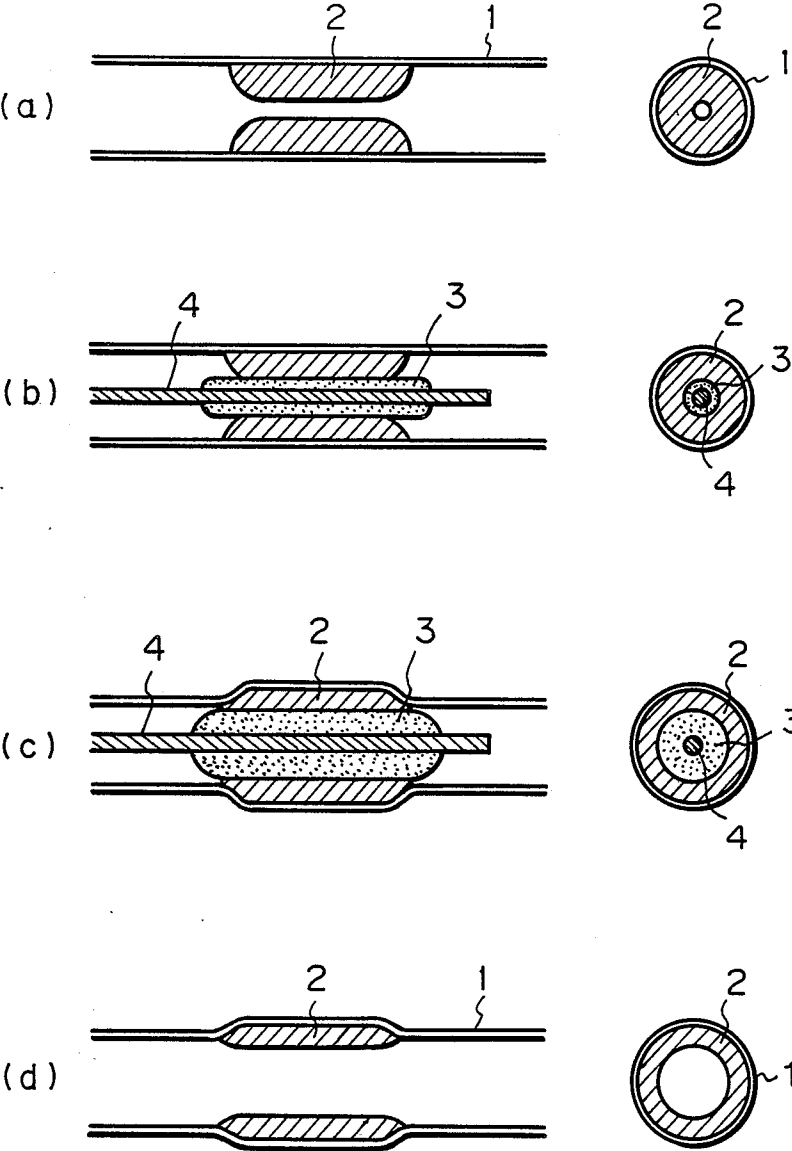
Fig. 9 PRIOR ART
