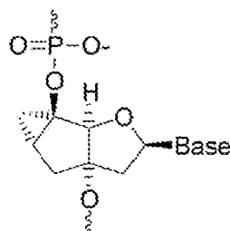
tricyclo-DNA
