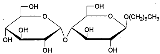
n-Decyl- \beta -D-maltoside
