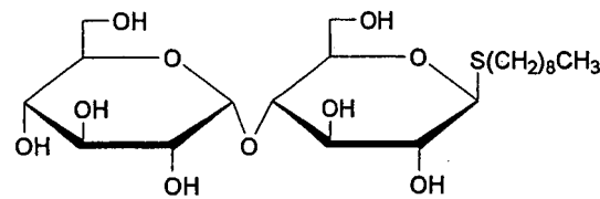
n-Nonyl- \beta -D-thiomaltoside
