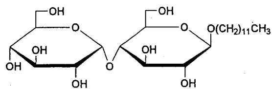
n-Dodecyl- \beta -D-maltoside
