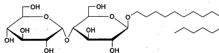
n-Hexadecyl- \beta -D-maltoside
