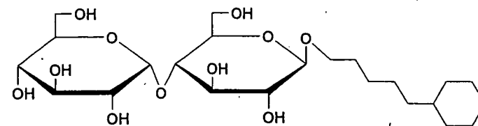
5-Cyclohexylpentyl- \beta -D-maltoside
