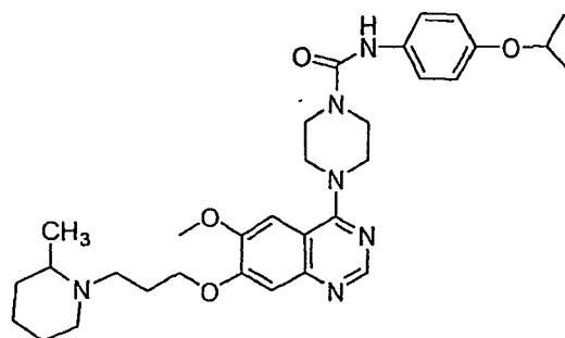
(4-{6-methoxy-7-[3-(4-methylpiperidyl)propoxy]quinazolin-4-yl}piperazinyl)-N-[4-(methylethoxy)phenyl]carboxamide
