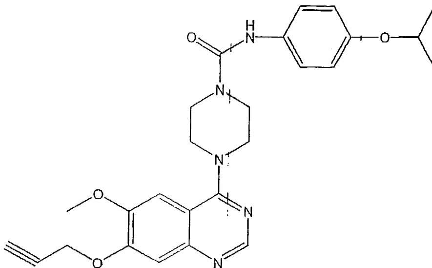
[4-(6-methoxy-7-prop-2-ynyloxyquinazolin-4-yl)piperazinyl]-N-(4-isopropoxyphenyl)carboxamide
