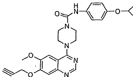
[4-(6-methoxy-7-prop-2-enyloxyquinazolin-4-yl)piperazinyl]-N-(4-naphthyloxyphenyl)carboxamide
