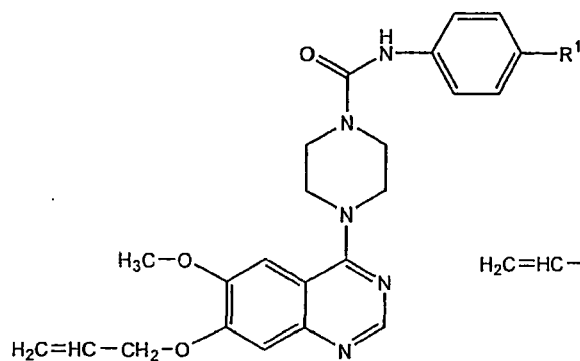
Formula I(c)
