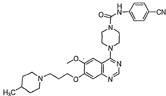
{4-[7-(2-hydroxy-3-piperidyl)propoxy]-6-methoxyquinazolin-4-yl}piperazinyl-N-[4-(methylethoxy)phenyl]carboxamide
