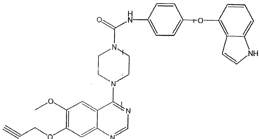
[4-(6-methoxy-7-prop-2-ynoxyquinazolin-4-yl)piperazinyl]-N-(4-phenoxyphenyl)carboxamide
