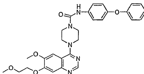
{4-[6-methoxy-7-(2-methoxyethoxy)quinazolin-4-yl]piperazinyl}-N-[4-(methylethoxy)phenyl]carboxamide
