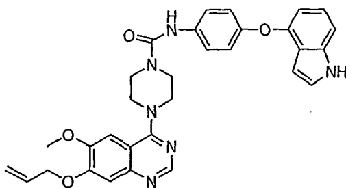
[4-(6-methoxy-7-prop-2-enyloxyquinazolin-4-yl)piperazinyl]-N-(4-phenoxyphenyl)carboxamide
