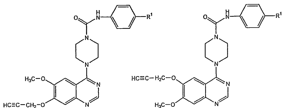
Formula I(f)
