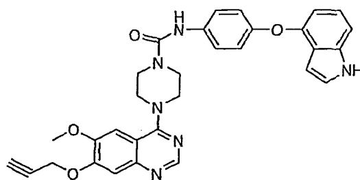
[4-(6-methoxy-7-prop-2-ynyloxyquinazolin-4-yl)piperazinyl]-N-(4-phenoxyphenyl)carboxamide
