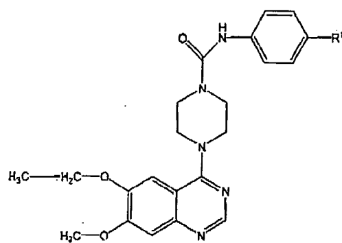
Formula I(b)
