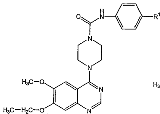
Formula I(a)
