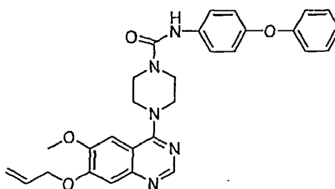
N-(4-cyanophenyl)[4-(6-methoxy-7-prop-2-enyloxyquinazolin-4-yl)piperazinyl]carboxamide
