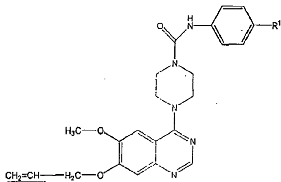
Formula I(c)
