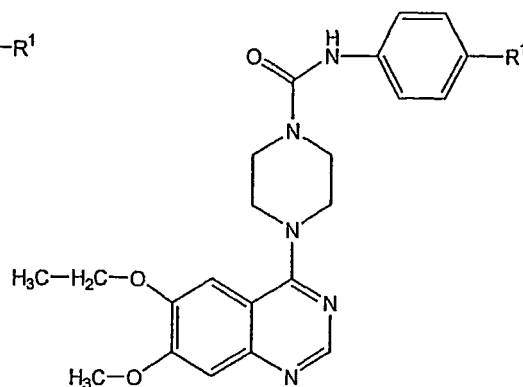
Formula I(b)
