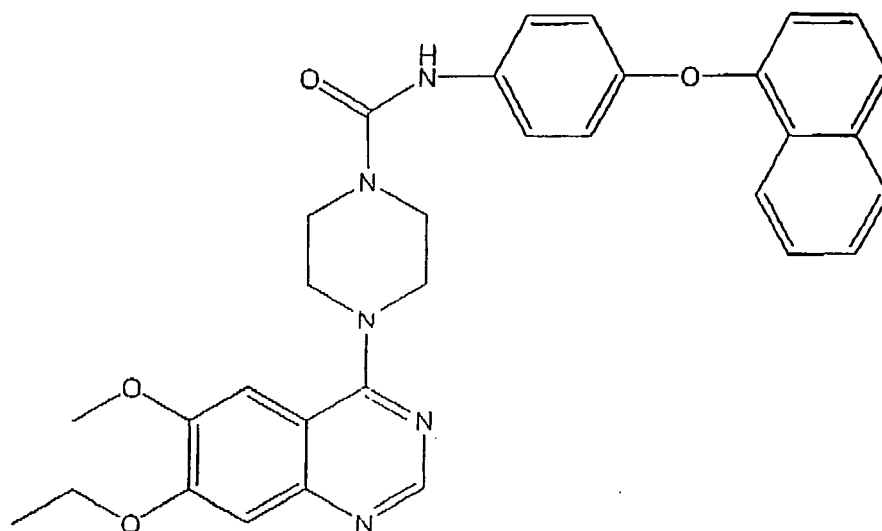
[4-(7-ethoxy-6-methoxyquinazolin-4-yl)piperazinyl]-N-(4-yloxyphenyl)carboxamide
