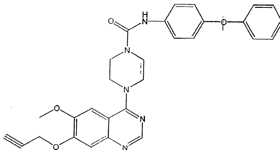
[4-(6-methoxy-7-prop-2-ynoxyquinazolin-4-yl)piperazinyl]-N-(4-phenoxyphenyl)carboxamide
