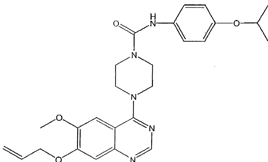
[4-(6-methoxy-7-prop-2-enyloxyquinazolin-4-yl)piperazinyl]-N-(4-naphthyloxyphenyl)carboxamide
