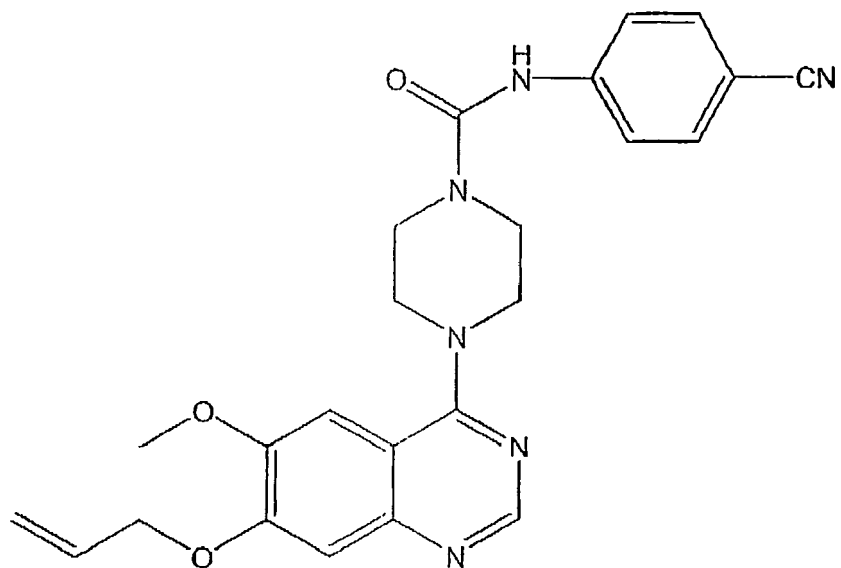
[4-(6-methoxy-7-prop-2-enyloxyquinazolin-4-yl)piperazinyl]-N-[4-(methylethoxy)phenyl]carboxamide
