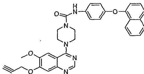
N-(4-indol-4-yloxyphenyl)[4-(6-methoxy-7-prop-2-ynyloxy quinazolin-4-yl)piperazinyl]carboxamide
