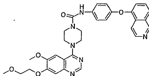
{4-[6-methoxy-7-(2-methoxyethoxy)quinazolin-4-yl]piperazinyl}-N-(4-phenoxyphenyl)carboxamide
