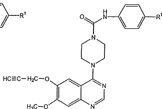
Formula I(f)
