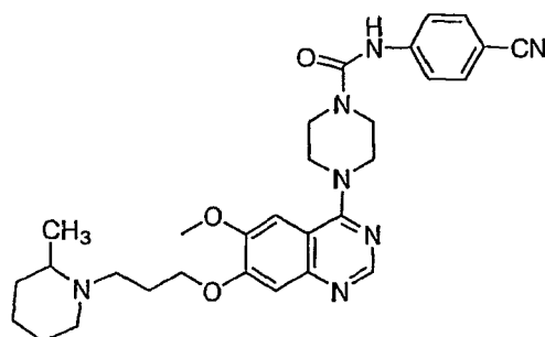
N-(4-cyanophenyl)(4-{6-methoxy-7-[3-(4-methylpiperidyl)propoxy]quinazolin-4-yl}piperazinyl)carboxamide
