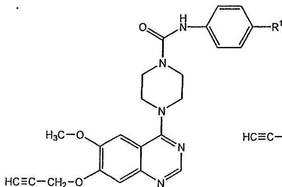
Formula I(e)
