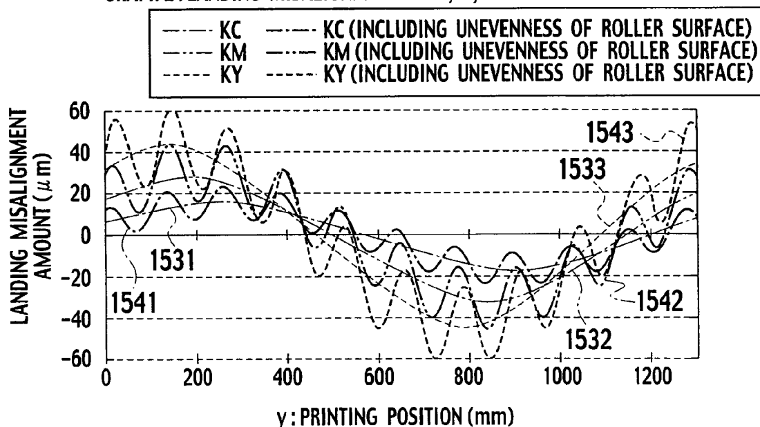
GRAPH 2: LANDING MISALIGNMENT OF C, M, Y AGAINST K
