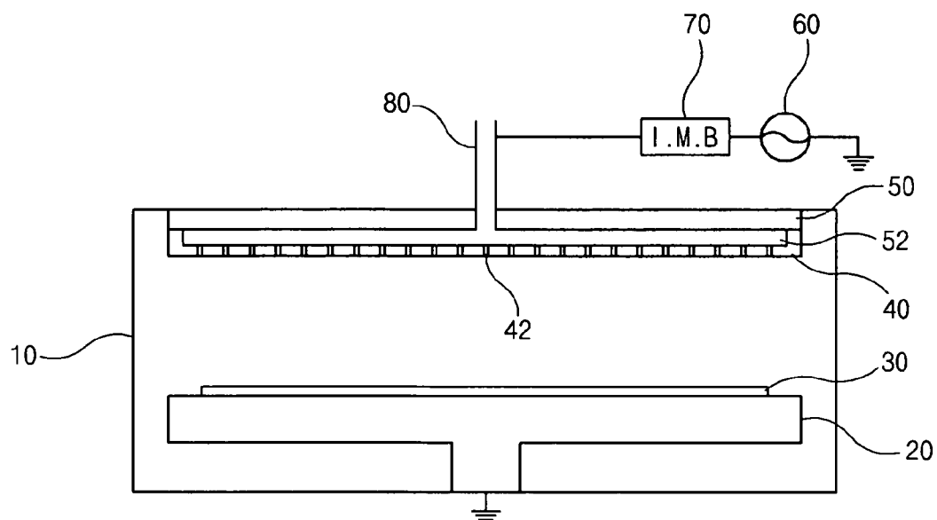
FIG. 1 RELATED ART
