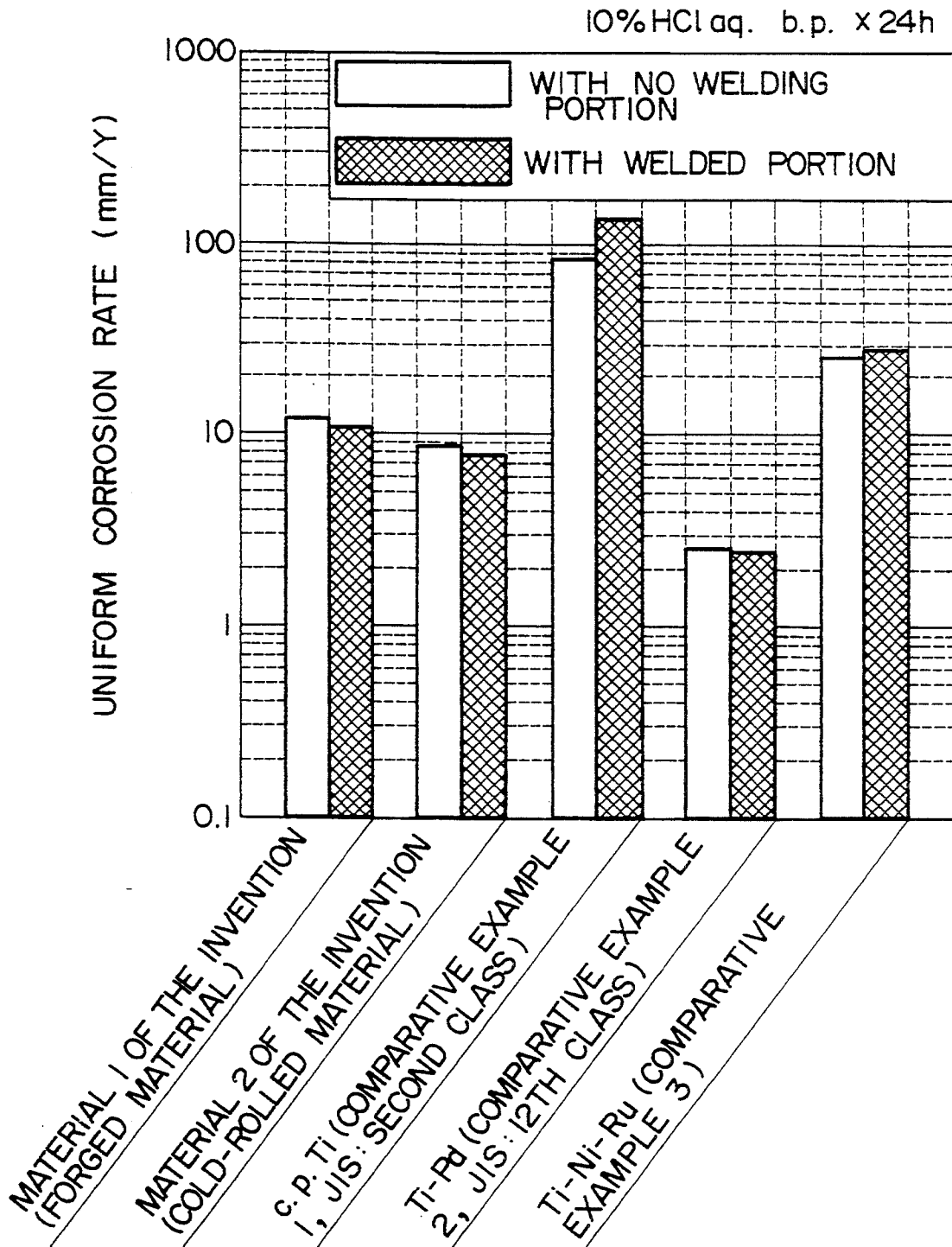
UNIFORM CORROSION RATE OF SIMULATED WELDED SPECIMEN
