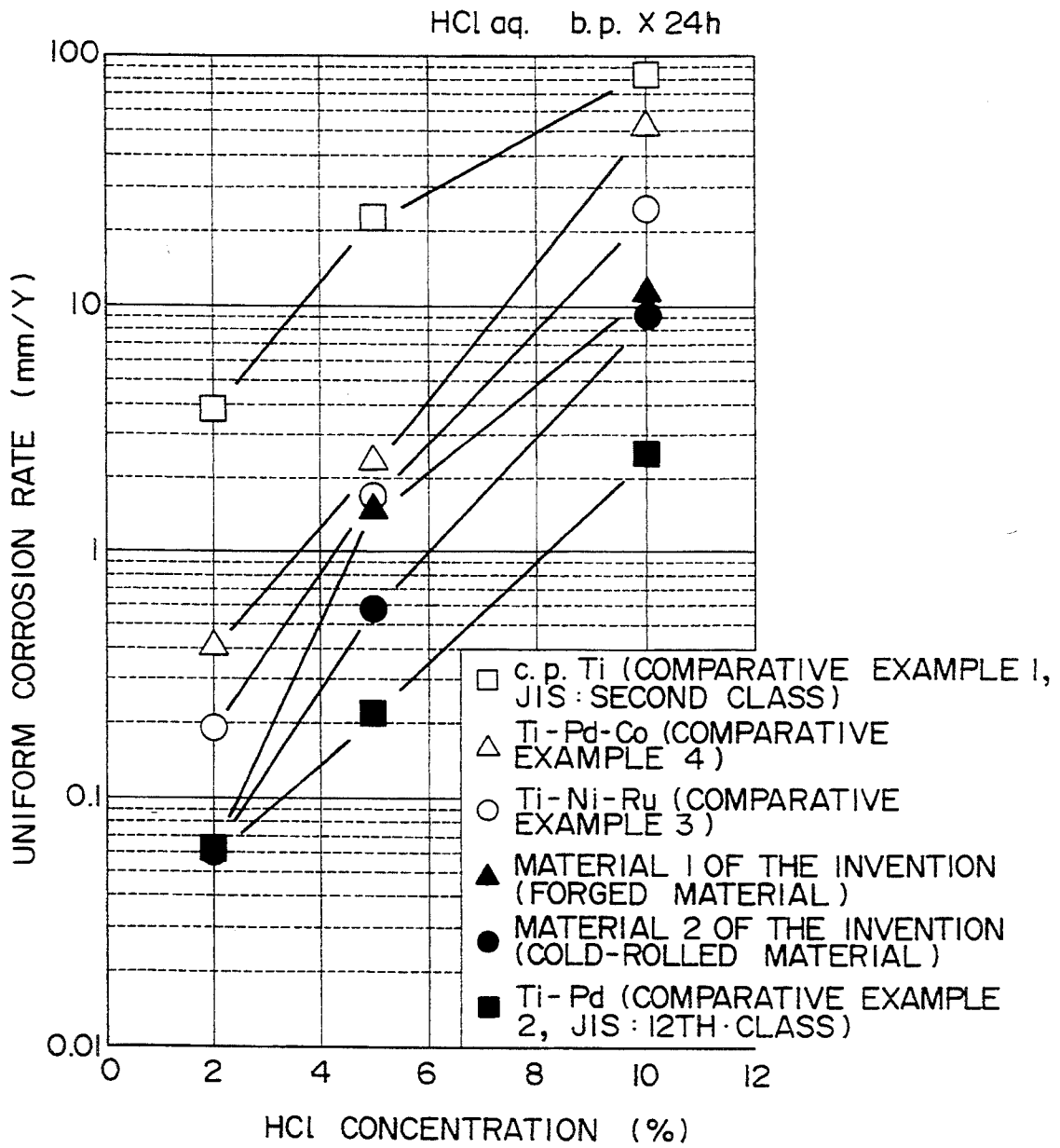
UNIFORM CORROSION RATE IN BOILING HCl
