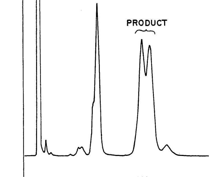
GLC PROFILE FOR EXAMPLE VII .
