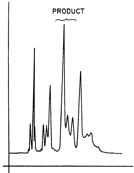
FIG.16 GLC PROFILE FOR EXAMPLE VI .
