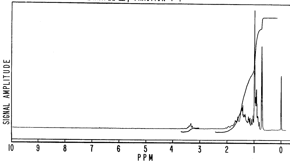
NMR SPECTRUM FOR EXAMPLE V, FRACTION 7 .
