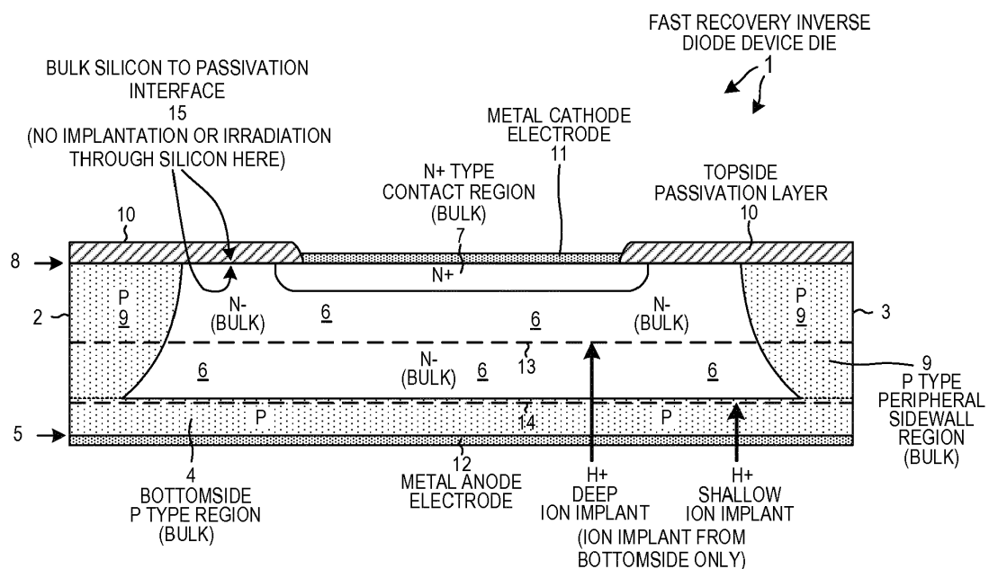
FAST RECOVERY INVERSE DIODE FIG. 1
