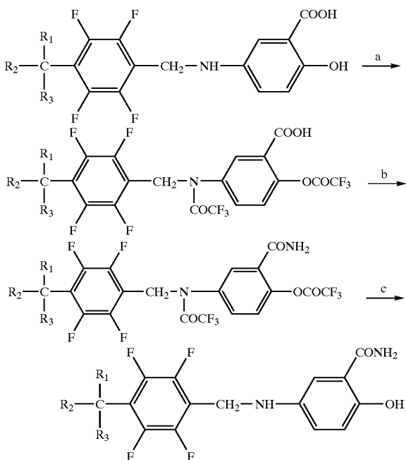
&lt;Reaction scheme 2&gt;
