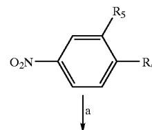
<Reaction scheme 1>
