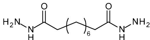
Sebacic acid dihydrazide
