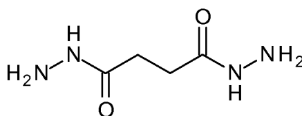
Succinic dihydrazide (SDH)
