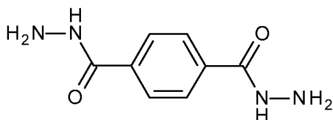
Isophthalic Dihydrazide (IDH)
