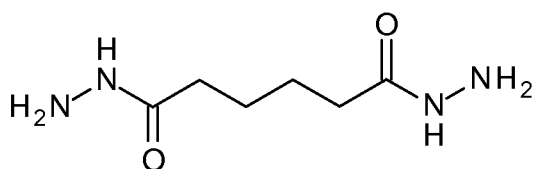
Adipic dihydrazide (ADH)
