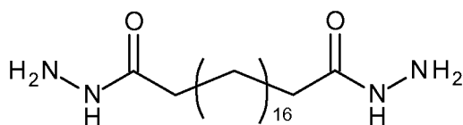
Icosanedioic acid dihydrazide
