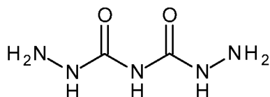
Imidodicarboxylic acid dihydrazide
