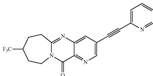
Example 3.9 3-(pyridin-2-ylethynyl)-8-(trifluoromethyl)-7,8,9,10-tetrahydropyrido[3',2':4,5]pyrimido[1,2-a]azepin-12(6H)-one
