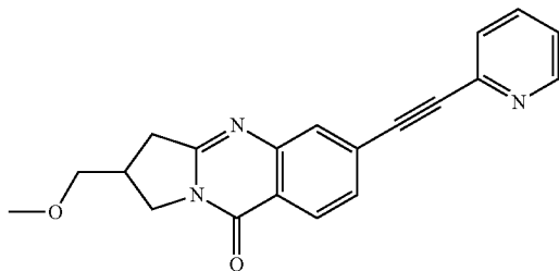
Example 1.1 2-(methoxymethyl)-6-(pyridin-2-ylethynyl)-2,3-dihydropyrrolo[2,1-b]quinazolin-9(1H)-one
