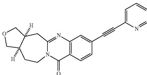
Example 3.32a 7-(pyridin-2-ylethynyl)-1,3a,4,12,13,13a-hexahydrofuro[3',4':4,5]azepino[2,1-b]quinazolin-10(3H)-one
