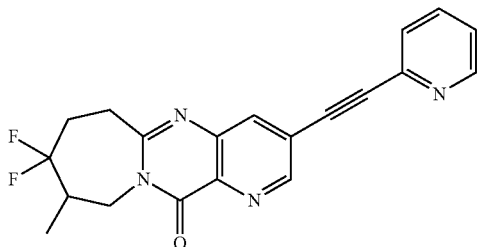
8,8-difluoro-9-methyl-3-(pyridin-2-ylethynyl)-7,8,9,10-tetrahydropyrido[3',2':4,5]pyrimido[1,2-a]azepin-12(6H)-one Example 3.31
