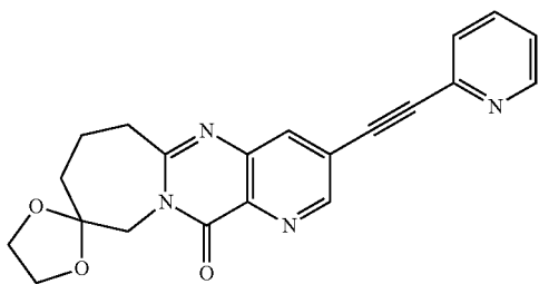
Example 3.29 3'-(pyridin-2-ylethynyl)-7',8'- dihydro-6'H- spiro[[1,3]dioxolane-2,9'- pyrido[3',2':4,5]pyrimido[1,2- a]azepin]-12'(10'H)-one
