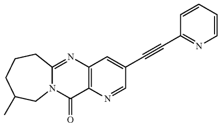
Example 3.28 9-methyl-3-(pyridin-2-ylethynyl)-7,8,9,10-tetrahydropyrido[3',2':4,5]pyrimido[1,2-a]azepin-12(6H)-one
