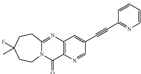
Example 3.10 8-fluoro-8-methyl-3-(pyridin-2-ylethynyl)-7,8,9,10-tetrahydropyrido[3',2':4,5]pyrimido[1,2-a]azepin-12(6H)-one
