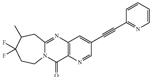
8,8-difluoro-7-methyl-3-(pyridin-2-ylethynyl)-7,8,9,10-tetrahydropyrido[3',2':4,5]pyrimido[1,2-a]azepin-12(6H)-one
