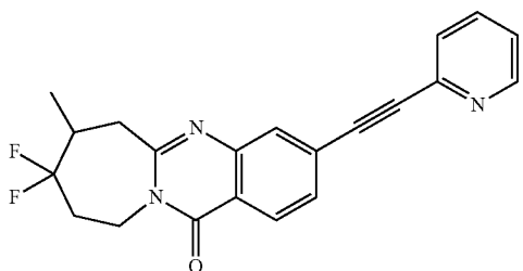
Example 3.30a 8,8-difluoro-7-methyl-3-(pyridin- 2-ylethynyl)-7,8,9,10- tetrahydroazepino[2,1- b]quinazolin-12(6H)-one
