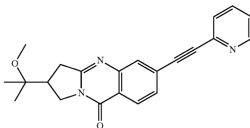
Example 1.4 2-(2-methoxypropan-2-yl)-6-(pyridin-2-ylethynyl)-2,3-dihydropyrrolo[2,1-b]quinazolin-9(1H)-one
