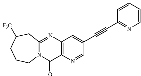
Example 3.8 3-(pyridin-2-ylethynyl)-7-(trifluoromethyl)-7,8,9,10-tetrahydropyrido[3',2':4,5]pyrimido[1,2-a]azepin-12(6H)-one
