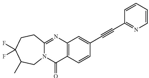
Example 3.30b 8,8-difluoro-9-methyl-3-(pyridin- 2-ylethynyl)-7,8,9,10- tetrahydroazepino[2,1- b]quinazolin-12(6H)-one
