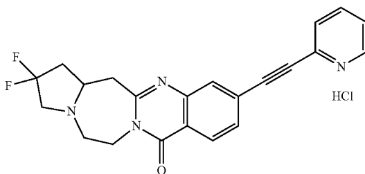
Example 3.33b 2,2-difluoro-11-(pyridin-2- ylethynyl)-2,3,5,6,14,14a- hexahydropyrrolo[1',2':4,5][1,4]di- azepino[7,1-b]quinazolin-8(1H)- one
