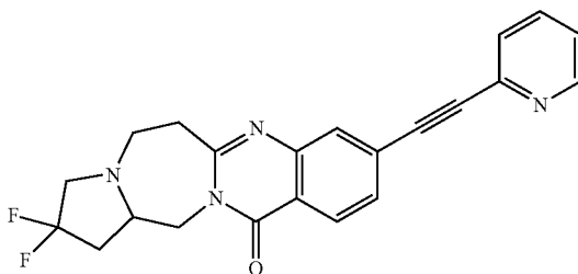
Example 3.33a 2,2-difluoro-9-(pyridin-2- ylethynyl)-2,3,5,6,14,14a- hexahydropyrrolo[2',1':3,4][1,4]di- azepino[7,1-b]quinazolin- 12(1H)-one
