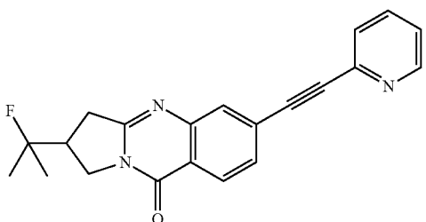
Example 1.3 2-(2-fluoropropan-2-yl)-6-(pyridin-2-ylethynyl)-2,3-dihydropyrrolo[2,1-b]quinazolin-9(1H)-one
