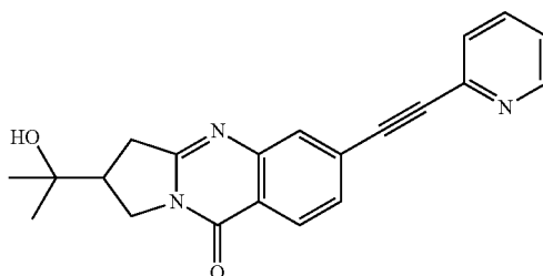
Example 1.2 2-(2-hydroxypropan-2-yl)-6-(pyridin-2-ylethynyl)-2,3-dihydropyrrolo[2,1-b]quinazolin-9(1H)-one
