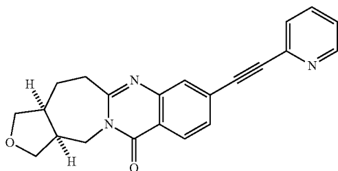
9-(pyridin-2-ylethynyl)- 1,3a,4,12,13,13a- hexahydrofuro[3',4':5,6]azepino[2,1- b]quinazolin-6(3H)-one Example 3.32b
