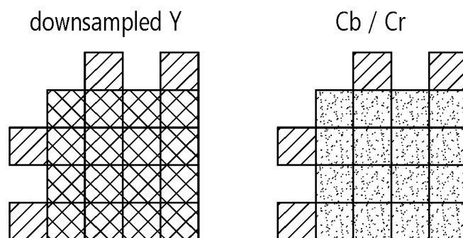
proposed reference subsampling method
