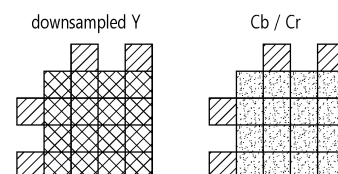
proposed reference subsampling method
