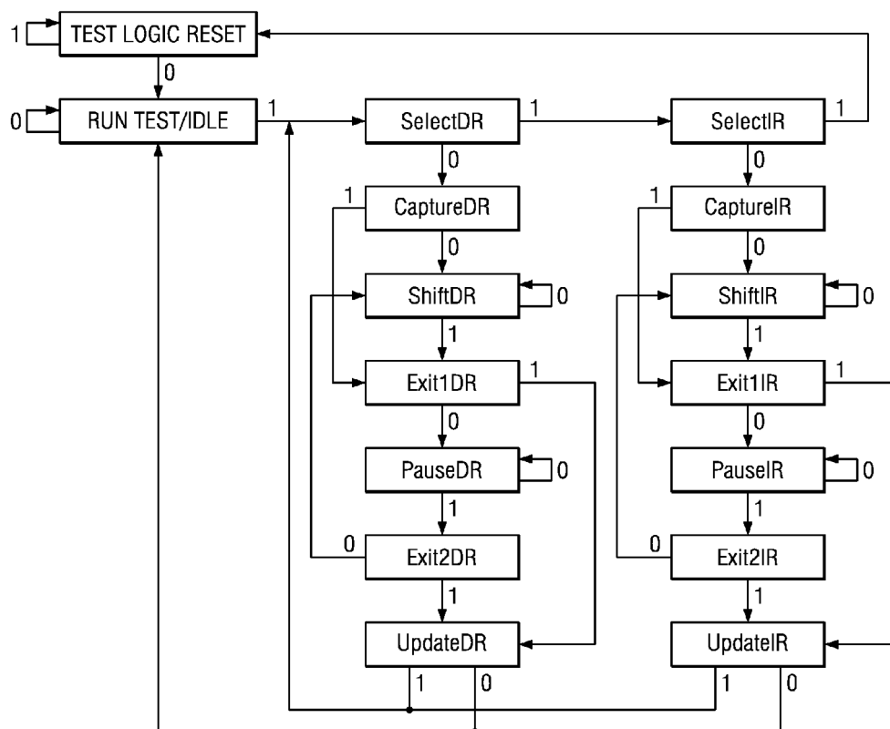
FIG. 3 (PRIOR ART)
