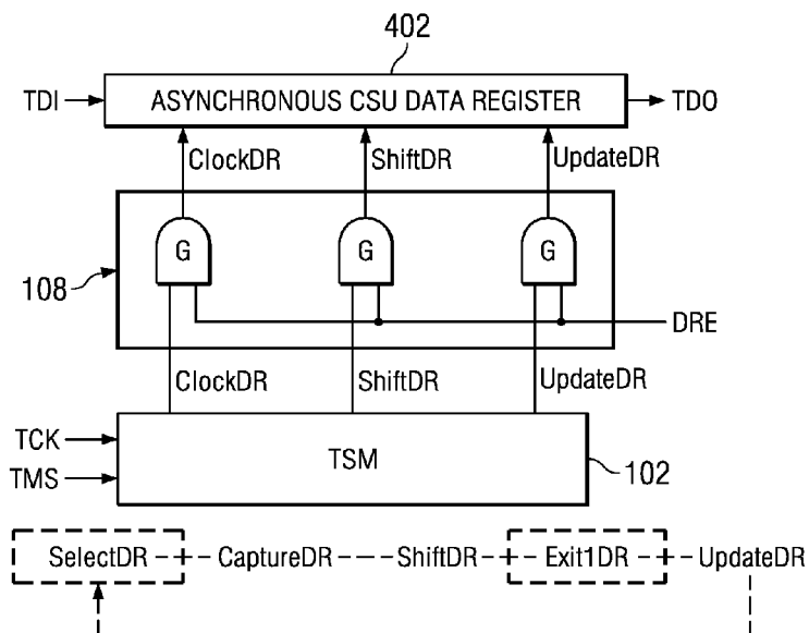
FIG. 4 (PRIOR ART)
