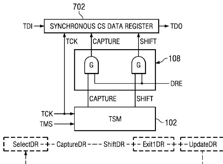
FIG. 7 (PRIOR ART)
