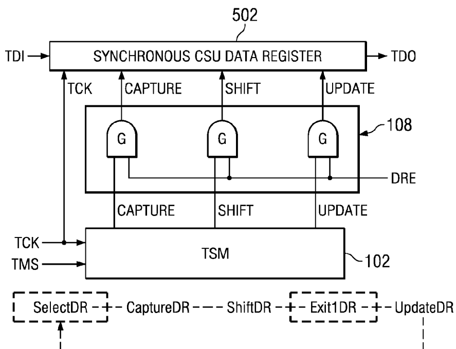
FIG. 5 (PRIOR ART)
