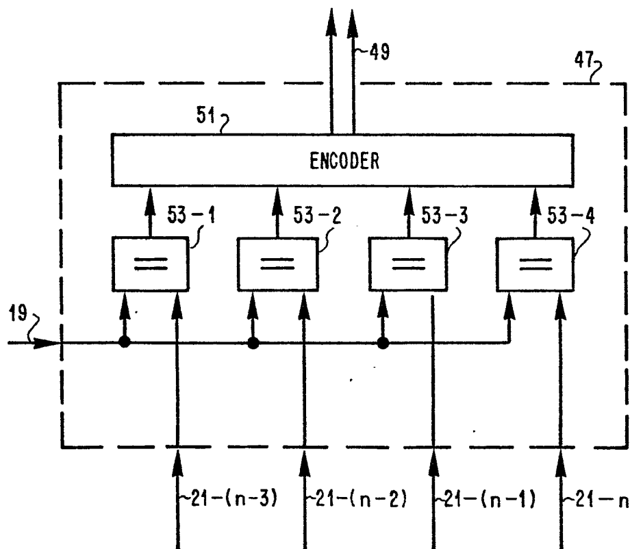
FIG. 7 DELAY LENGTH ENCODER
