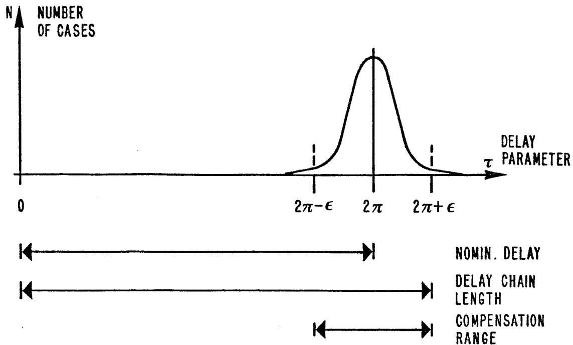
FIG. 6 PROPAGATION DELAY DISTRIBUTION
