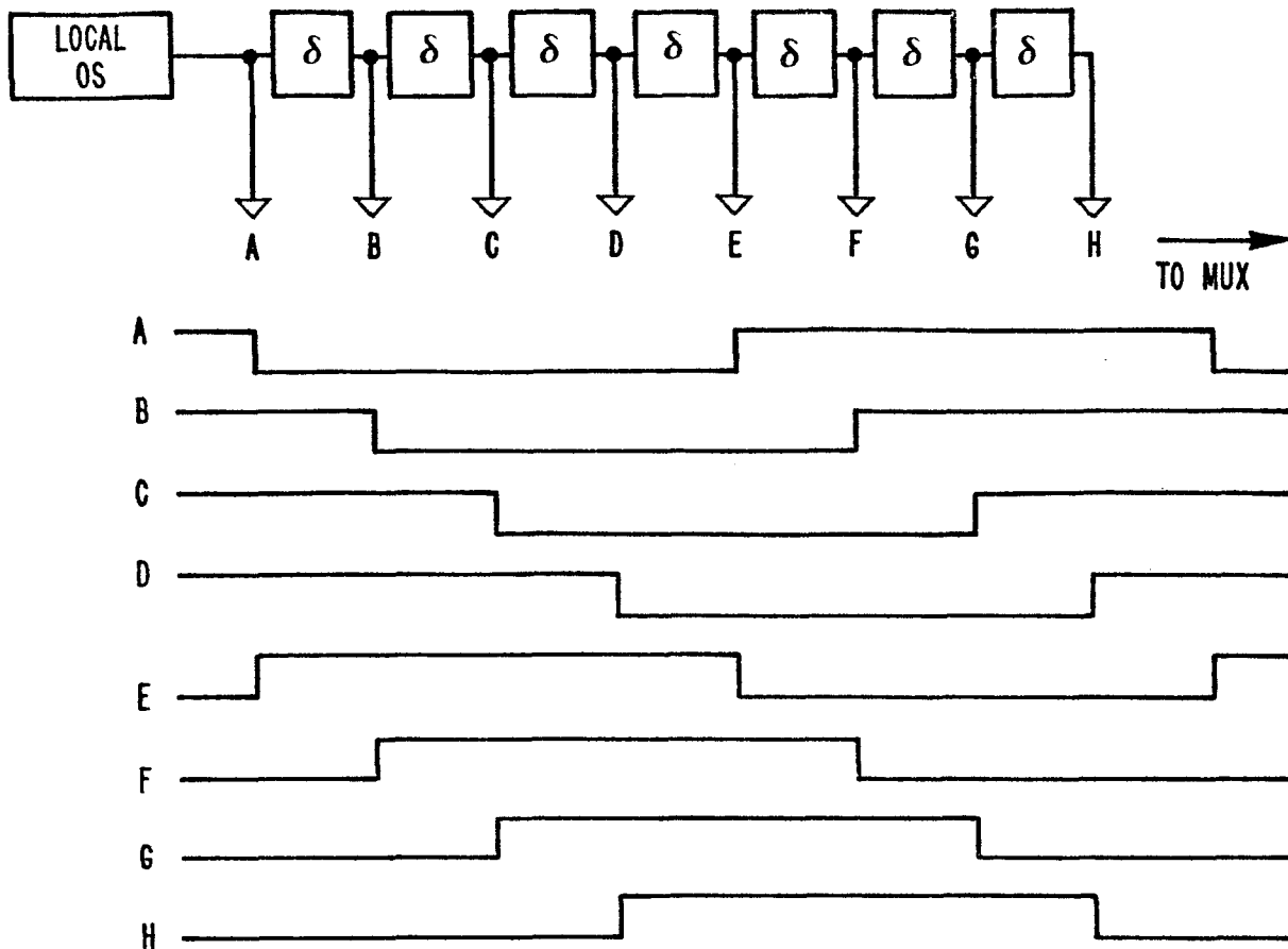
FIG. 3 DELAY CHAIN - PHASE SHIFTING
