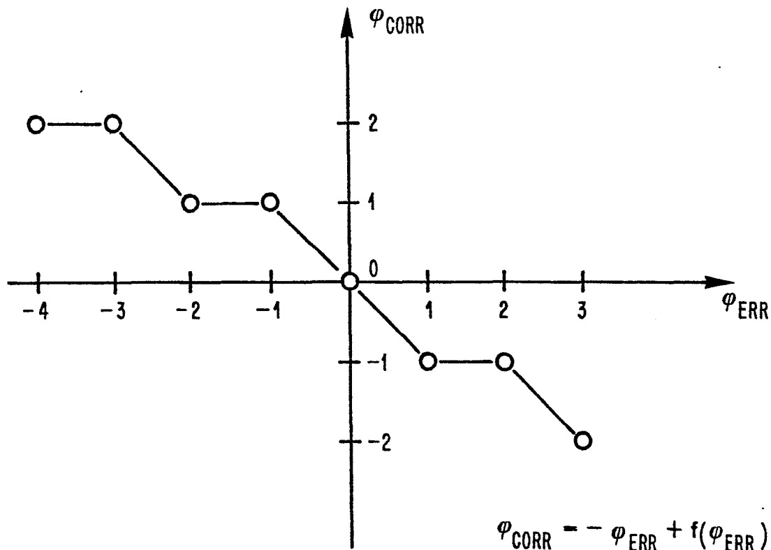
FIG. 4 PHASE CORRECTION FUNCTION
