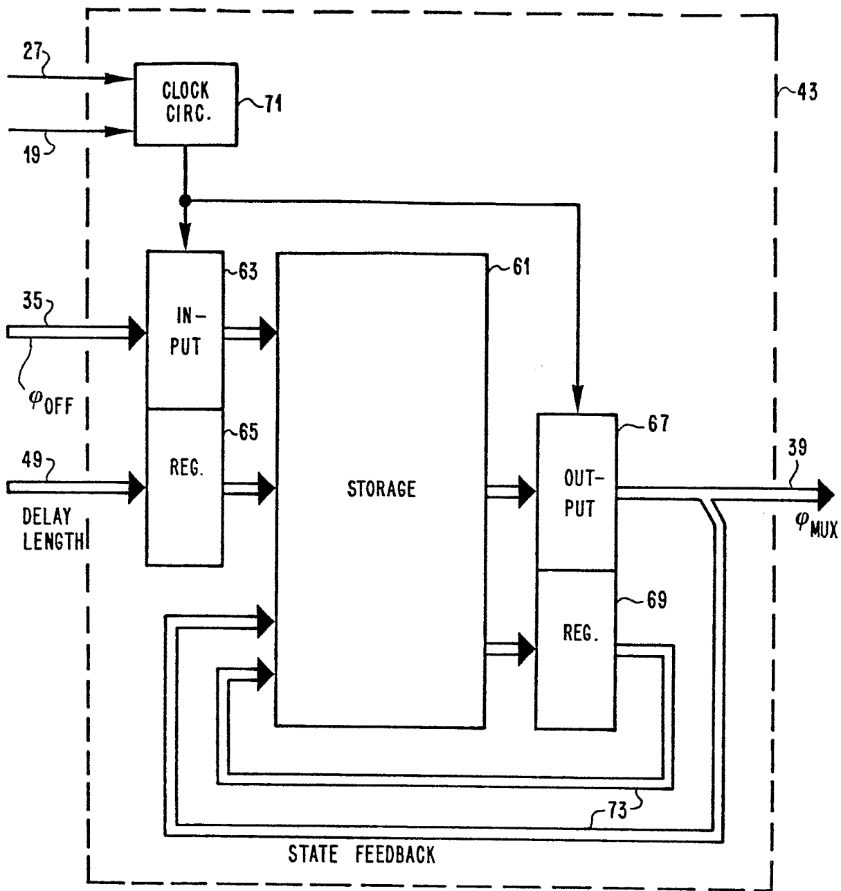
FIG. 8 PROCESSOR
