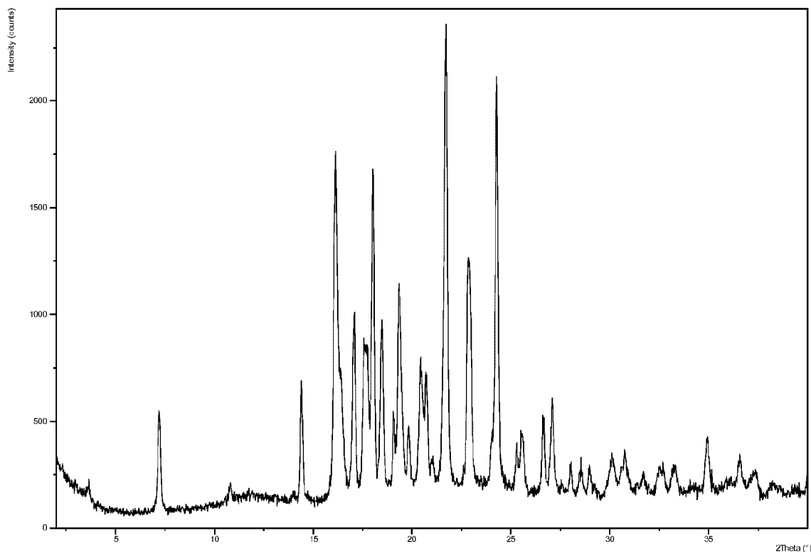
Figure 1: XRPD spectrum for compound of Formula (I)
