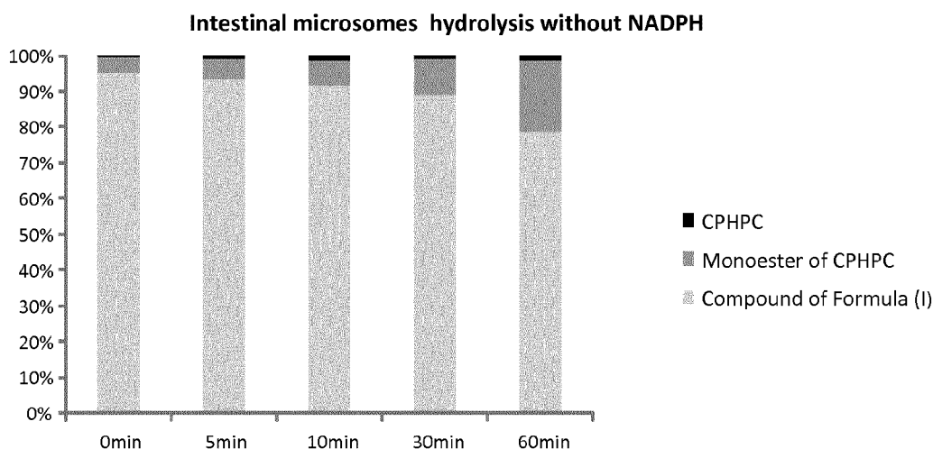
Figure 3: In vitro Intestinal Microsomal Stability of Compound of Formula (I) in human microsomes. "0/5/10/30/60min" refers to the time (in minutes) that the sample was taken from the mixture for analysis.
