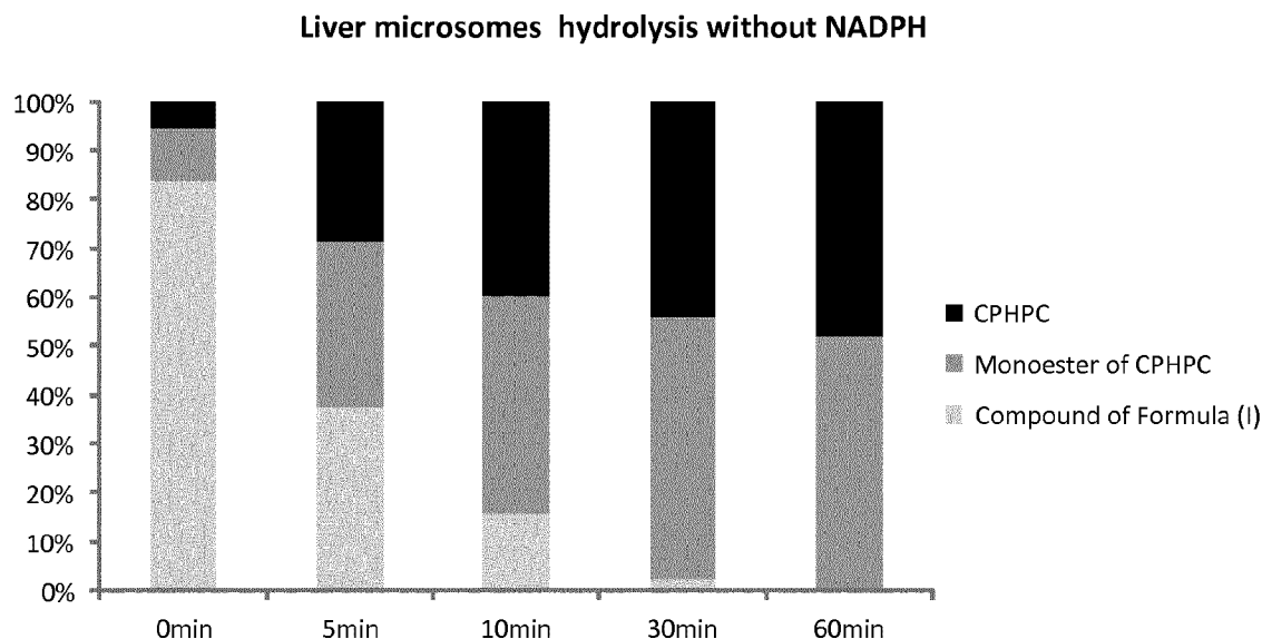
5 Figure 5: In vitro Liver microsomal stability of compound of Formula (I) in human liver microsomes. "0/5/10/30/60min" refers to the time (in minutes) that the sample was taken from the mixture for analysis.
