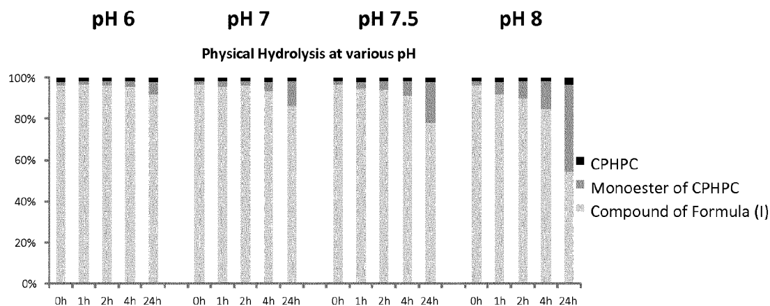
Figure 2: In vitro physical hydrolysis of compound of Formula (I) in phosphate buffered saline at pH6, 7, 7.5 and 8
