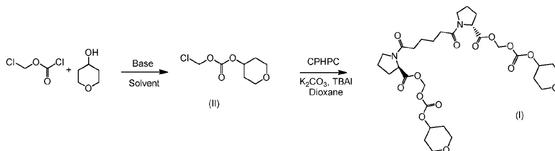
Reaction Scheme 1
