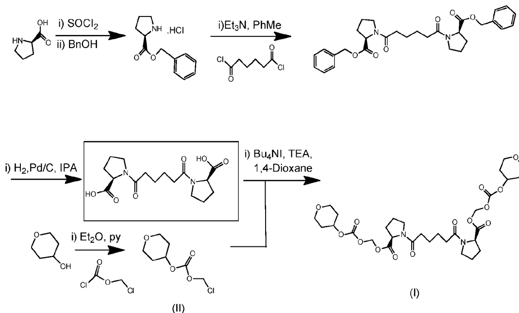
Reaction Scheme 2
