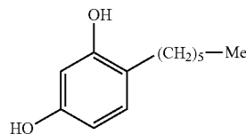
4-hexyl resorcinol
