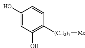
4-octylresorcinol
