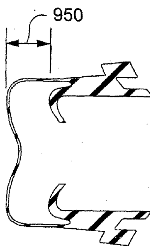
Fig. 95C SECTION B-B
