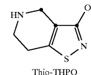
Thio-THPO
