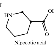
Nipecotic acid
