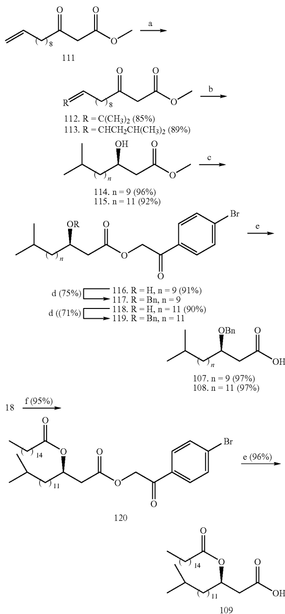
Scheme 8.
