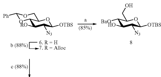
Scheme 1 a
