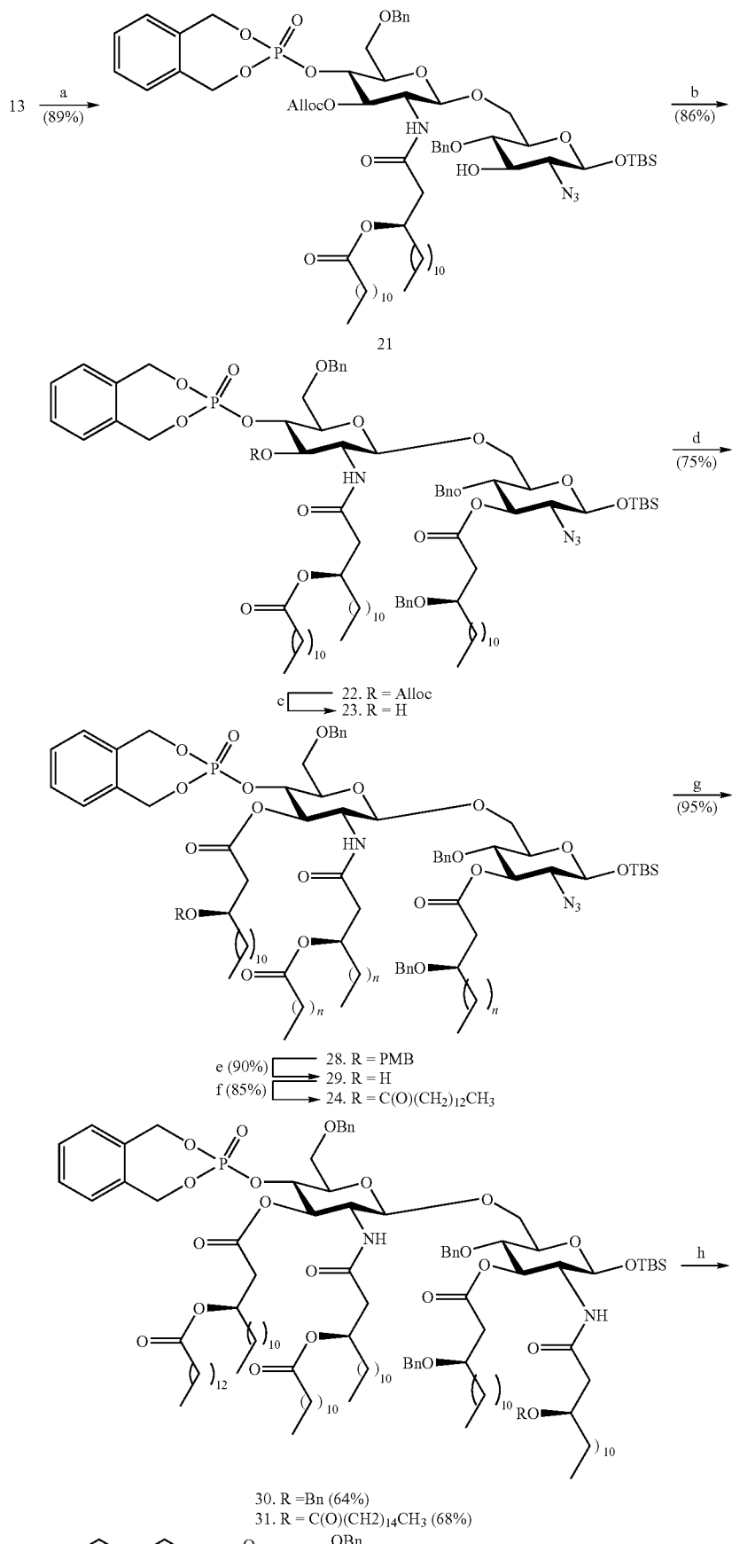
Scheme 2 a
