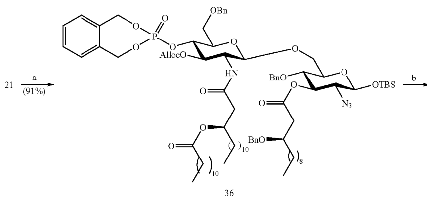
Scheme 3 a
