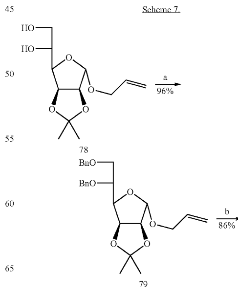
Scheme 7.
