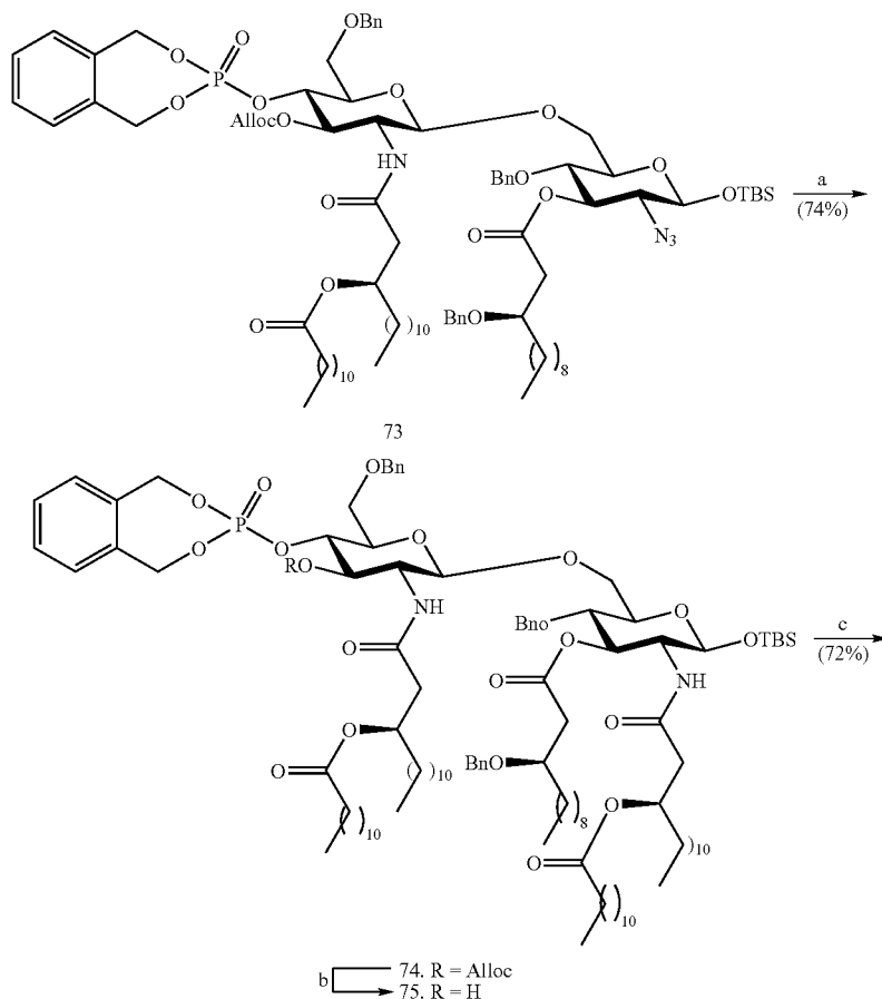
Scheme 6.
