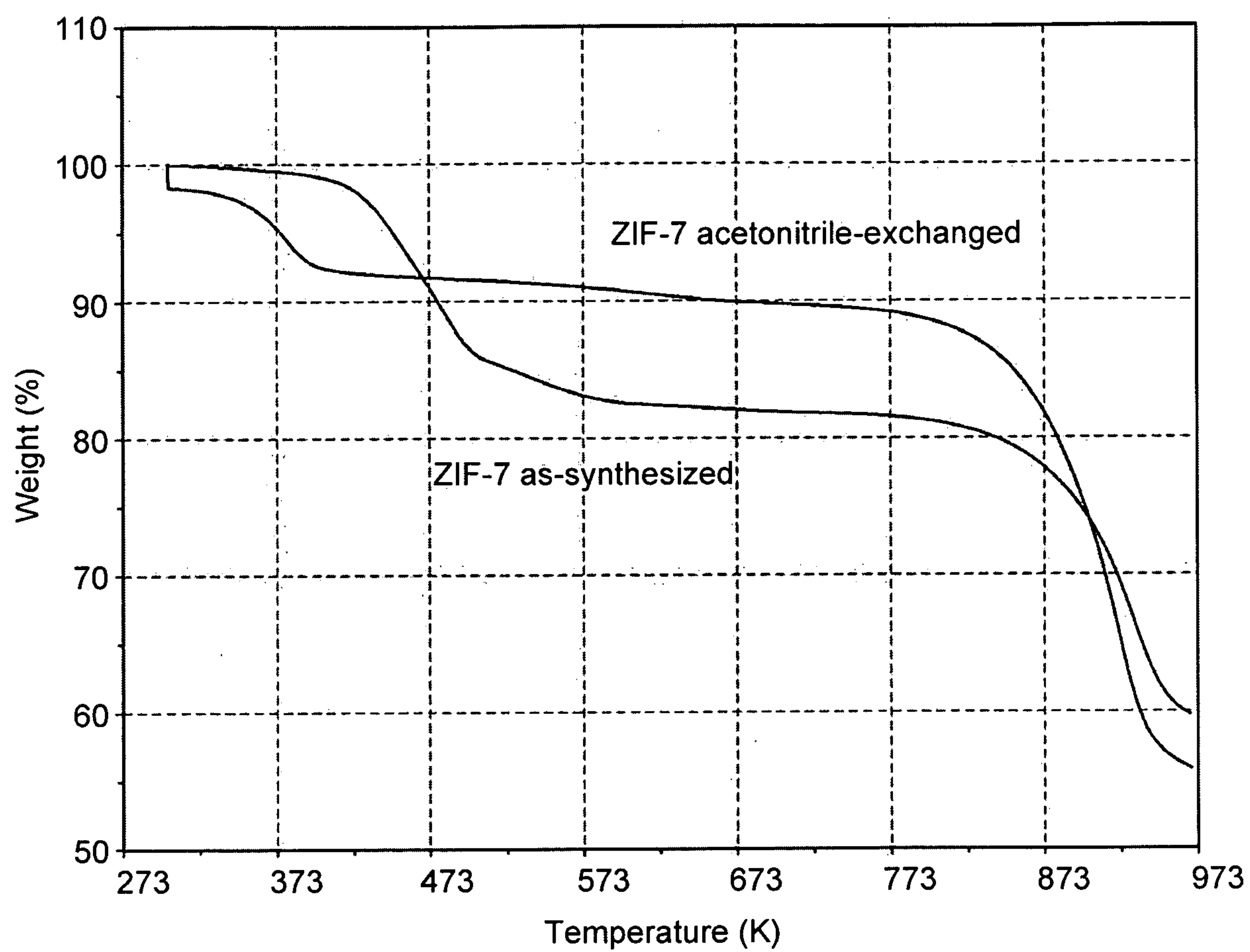
Thermogravimetric Analyses of ZIF-7
