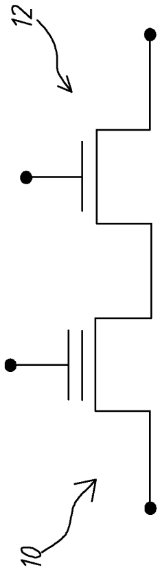
Fig. 1 (Prior Art)
