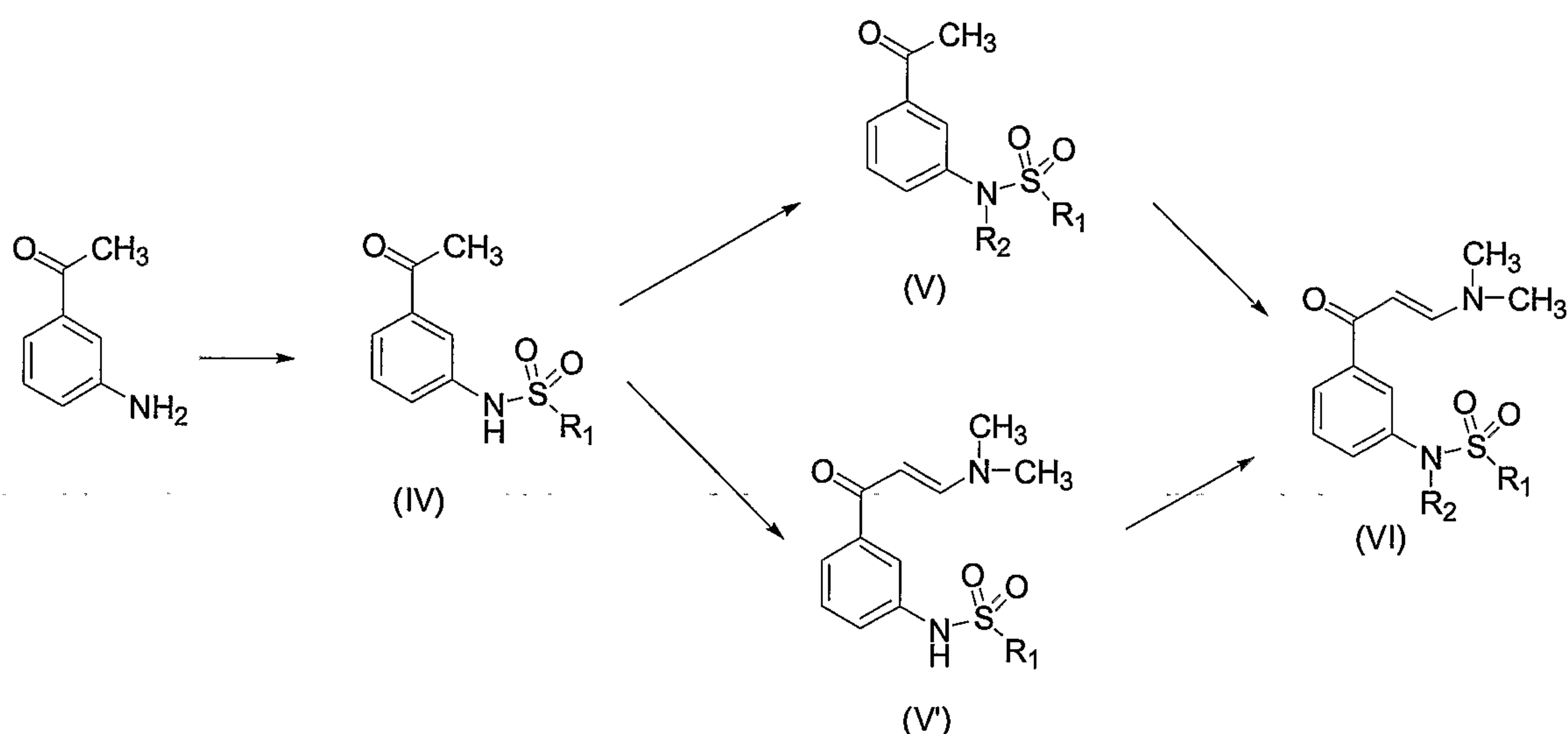
Scheme 2
