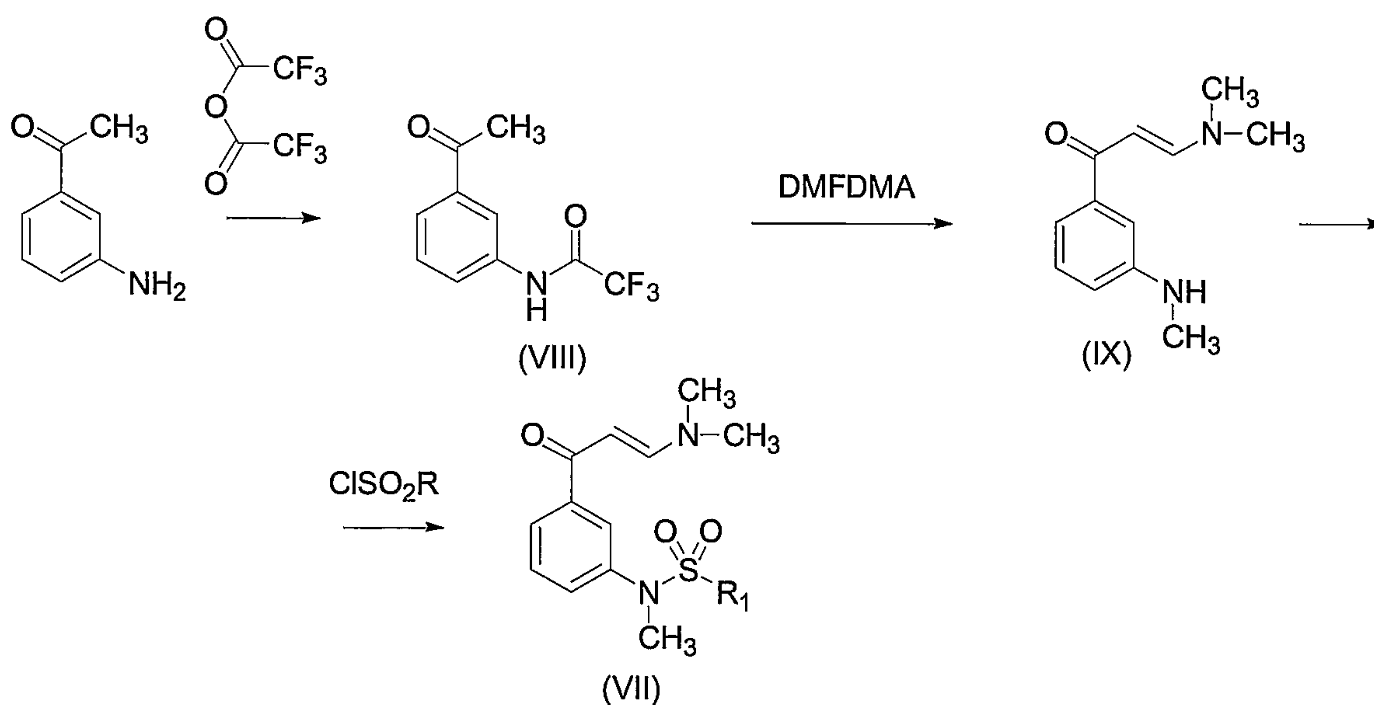
Scheme 4
