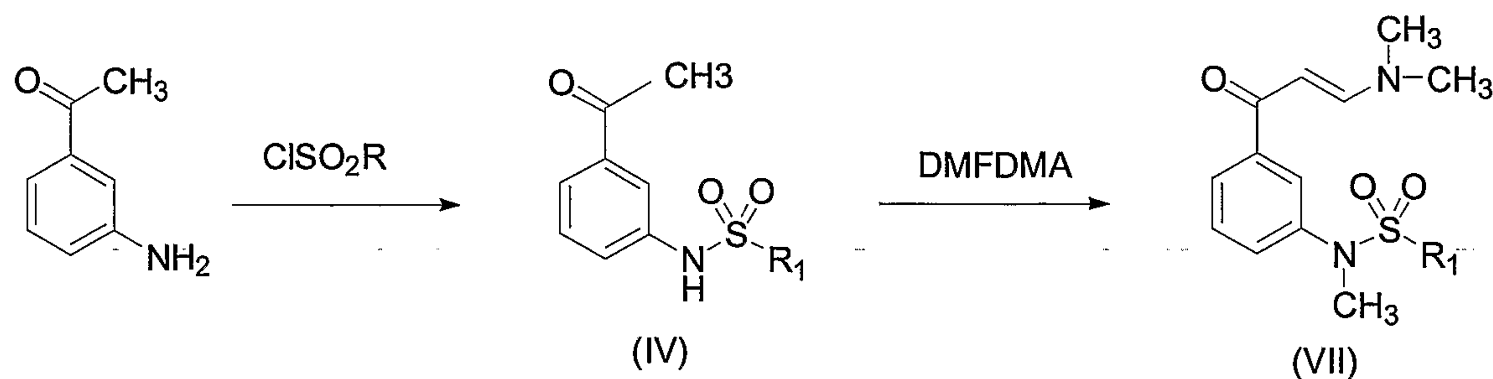
Scheme 3
