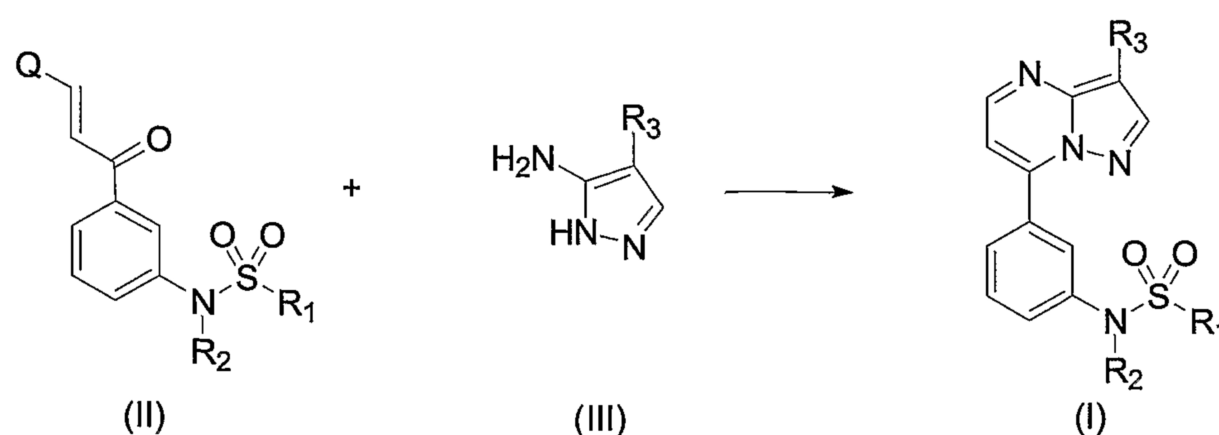
Scheme 1
