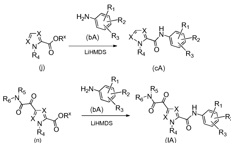
Scheme 3A
