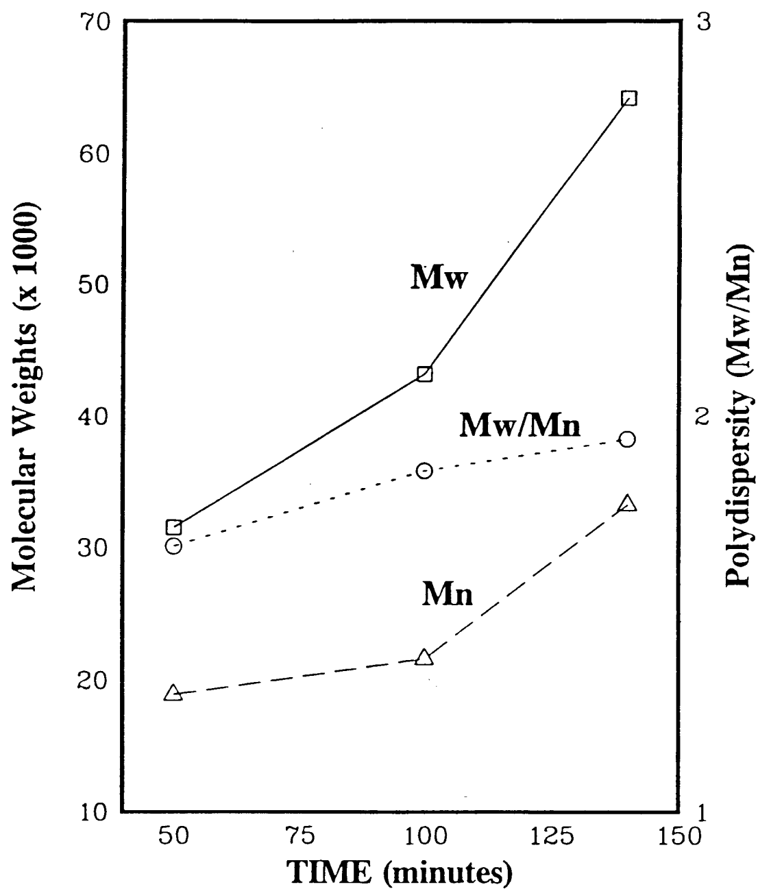
FIGURE 2 VCM Polymerization Using Iodoform Mw, Mn and Polydispersity vs. Time
