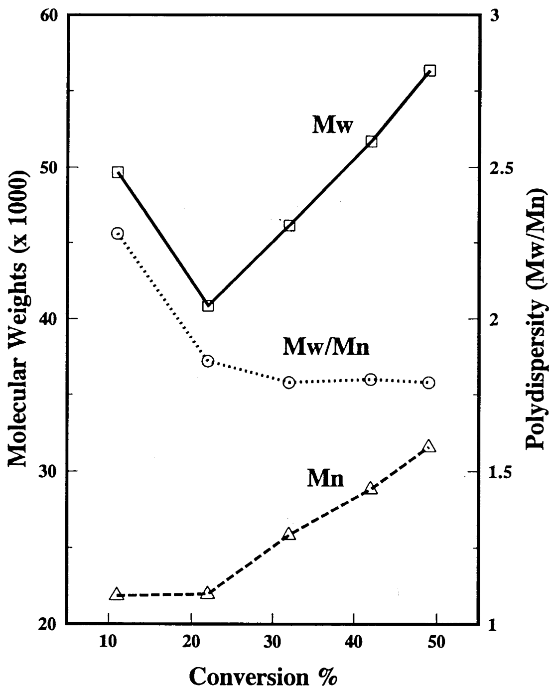
FIGURE 1 VCM Polymerization Using 1-Chloro-1-iodoethane Mw, Mn and Polydispersity vs. Conversion
