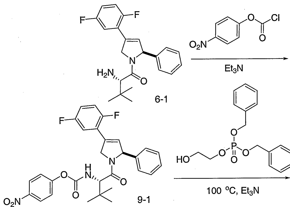
SCHEME 9 (continued)
