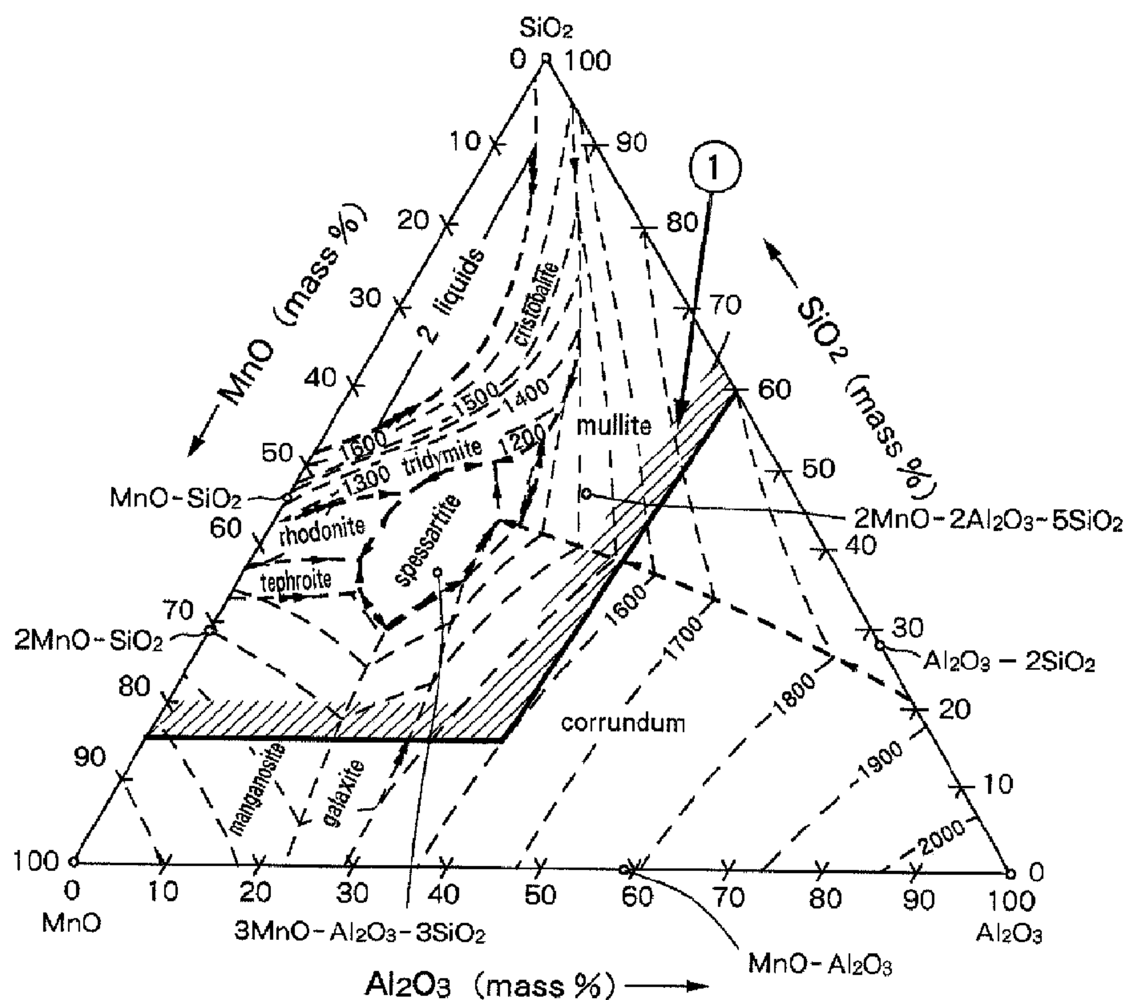
a MnO-SiO 2 -Al 2 O 3 phase diagram
