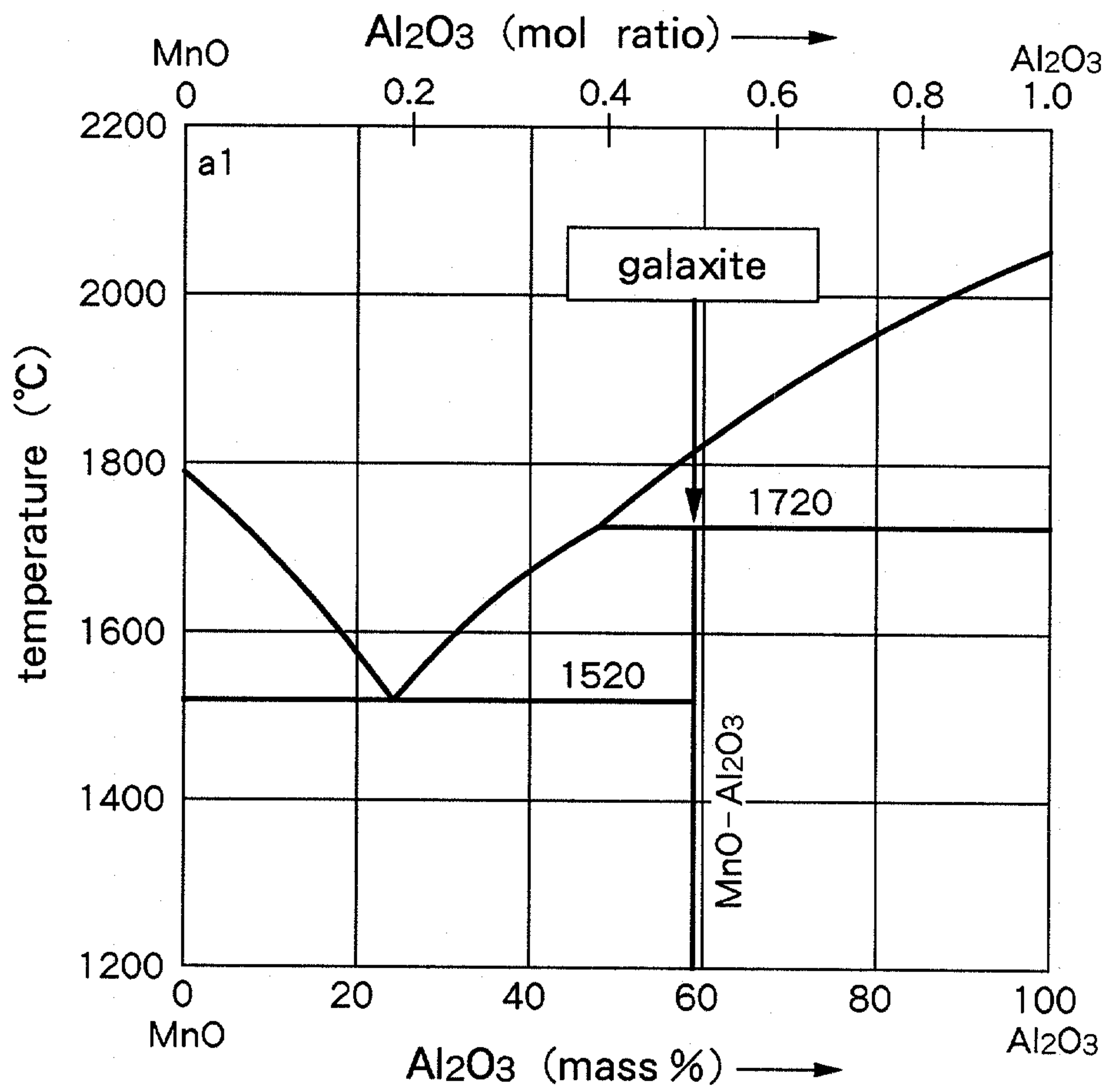
A MnO-Al 2 O 3 PHASE DIAGRAM
