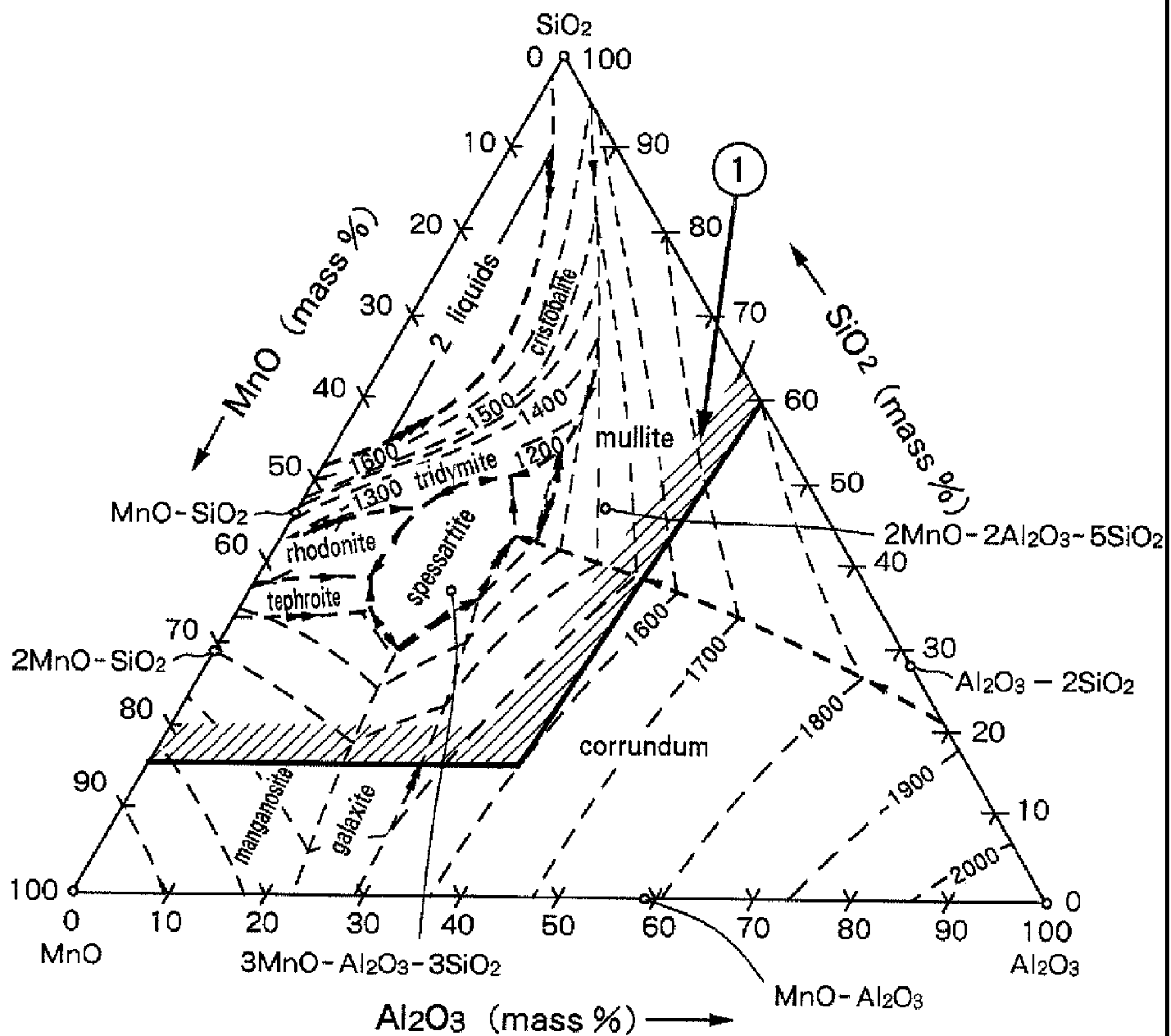
a \text{MnO}-\text{SiO}_2-\text{Al}_2\text{O}_3 phase diagram
