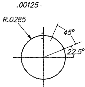
SECTION B-B SCALE 30:1
