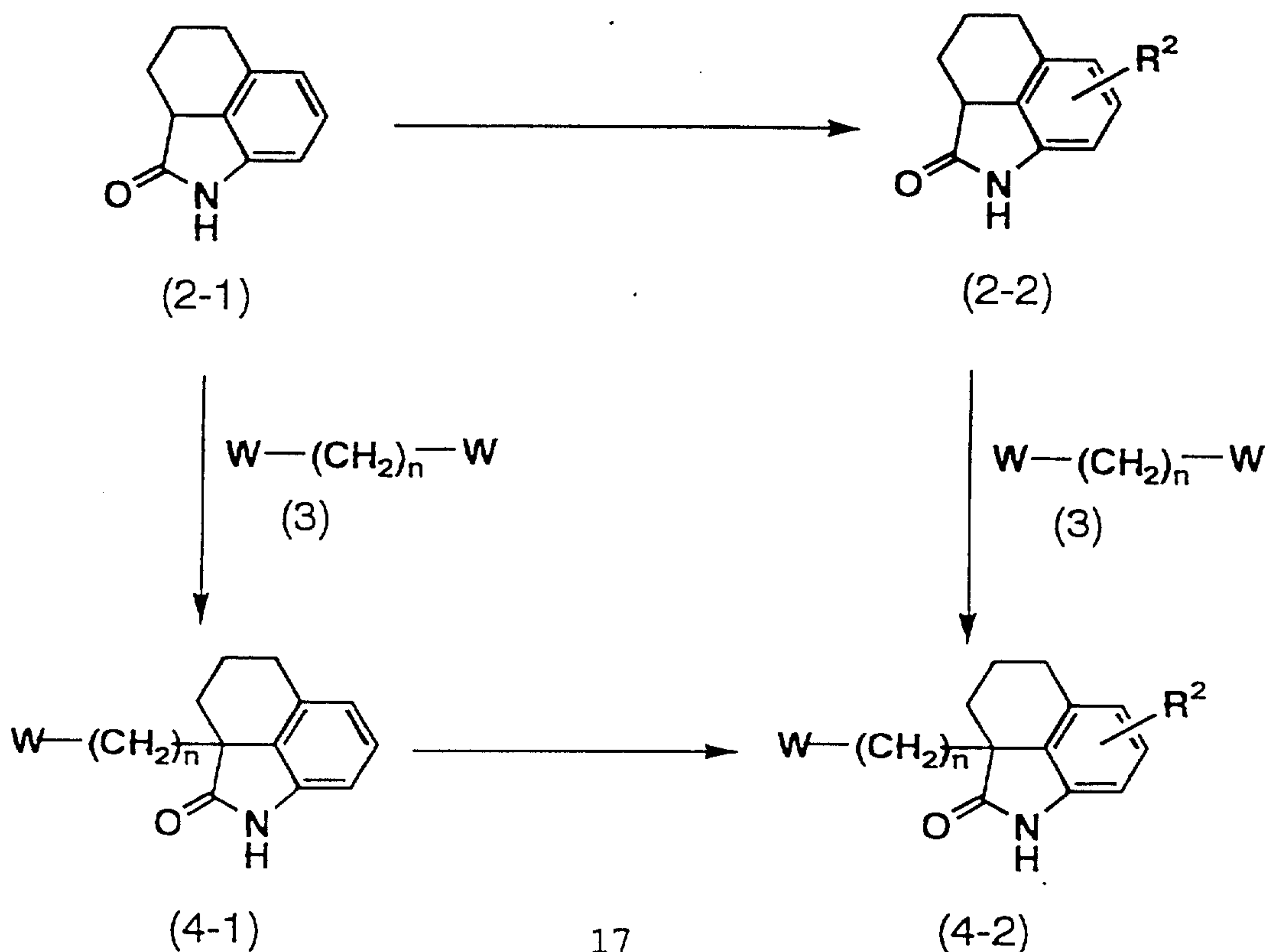
Reaction Formula 2
