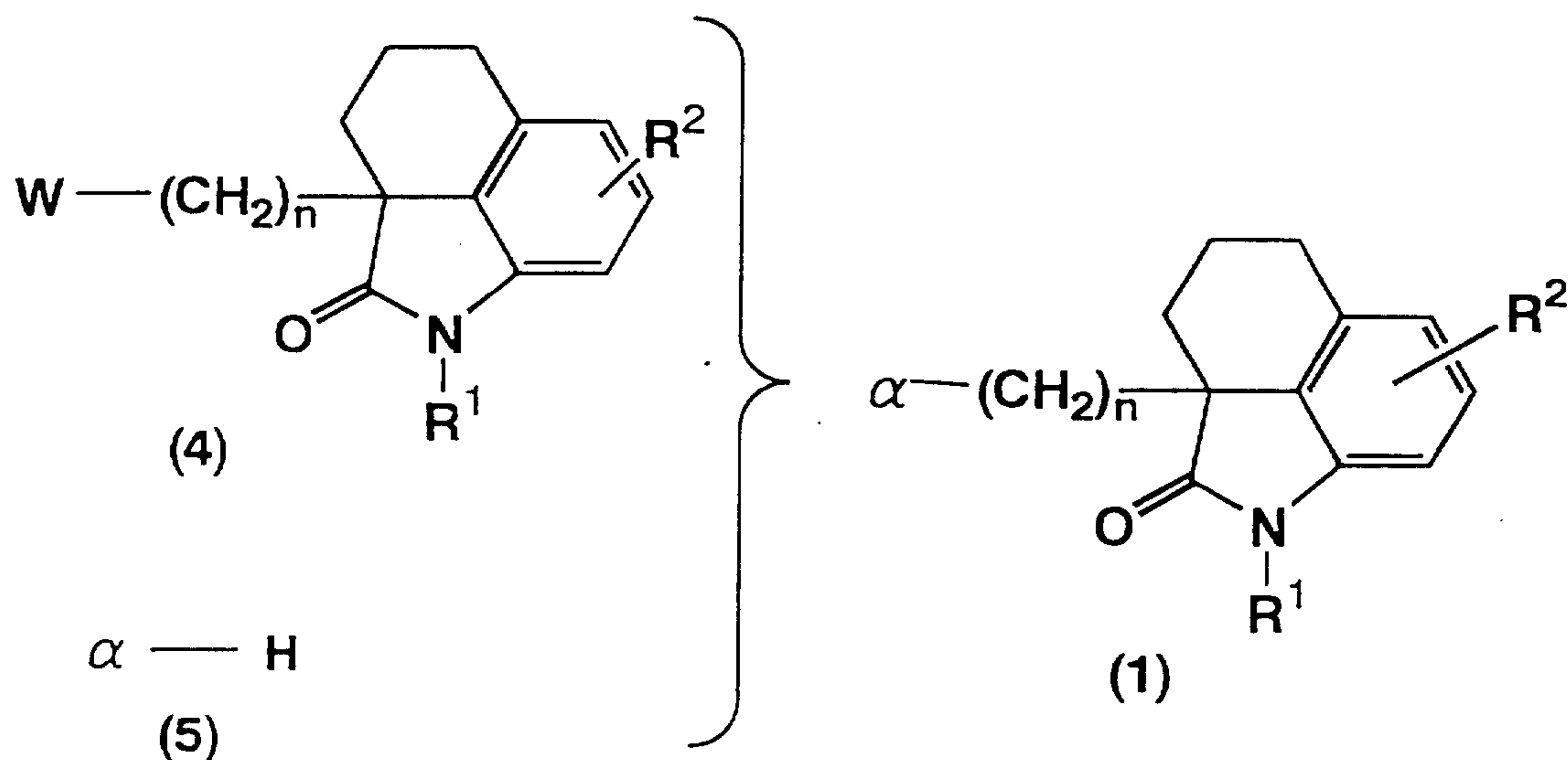
Reaction Formula 1
