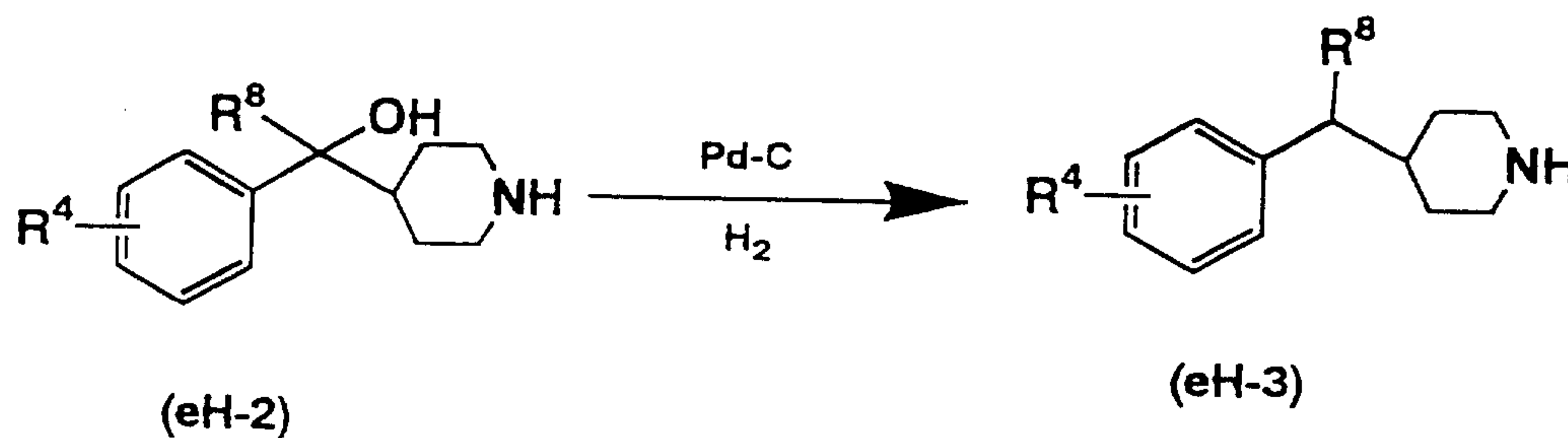
Reaction Formula 16
