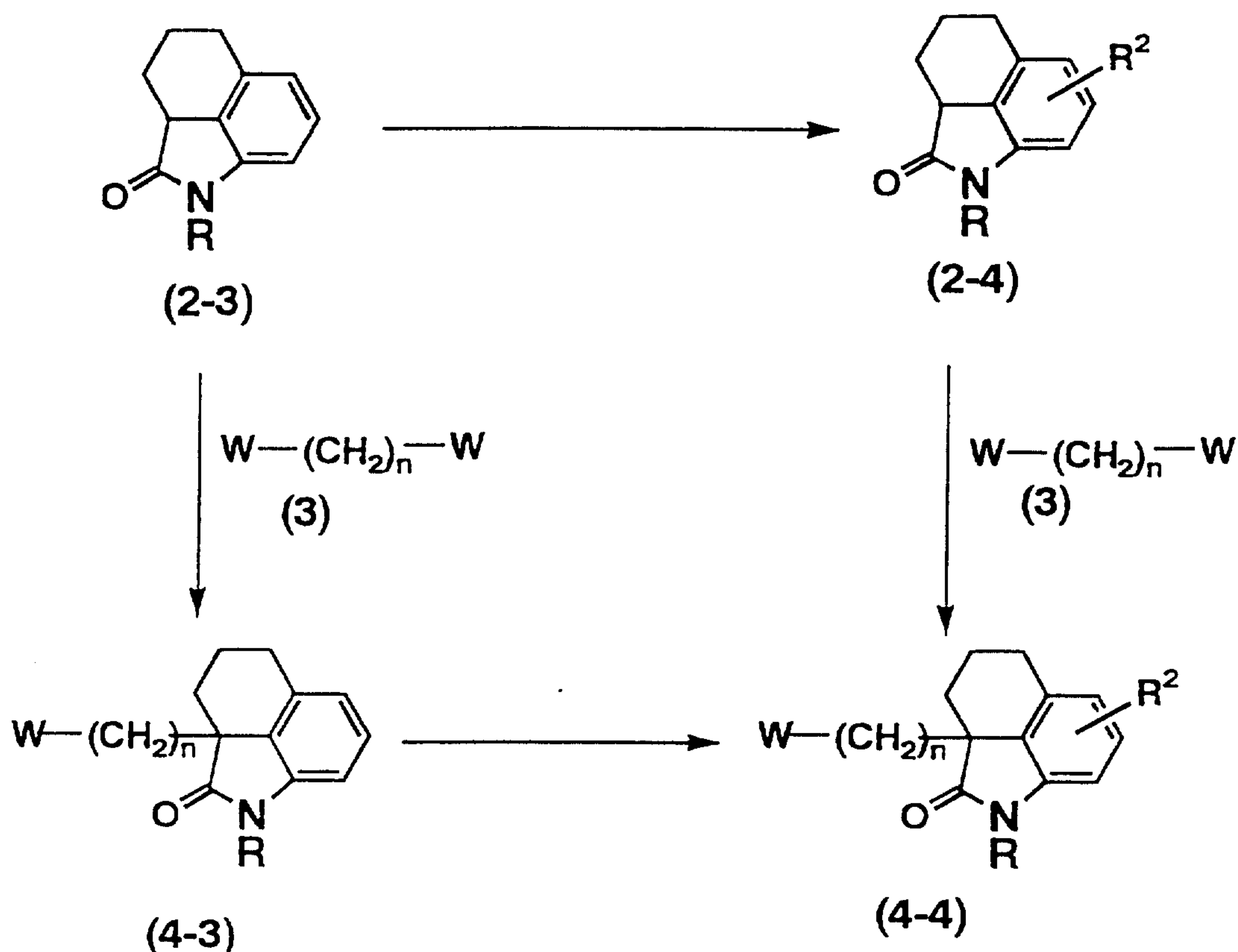
Reaction Formula 3
