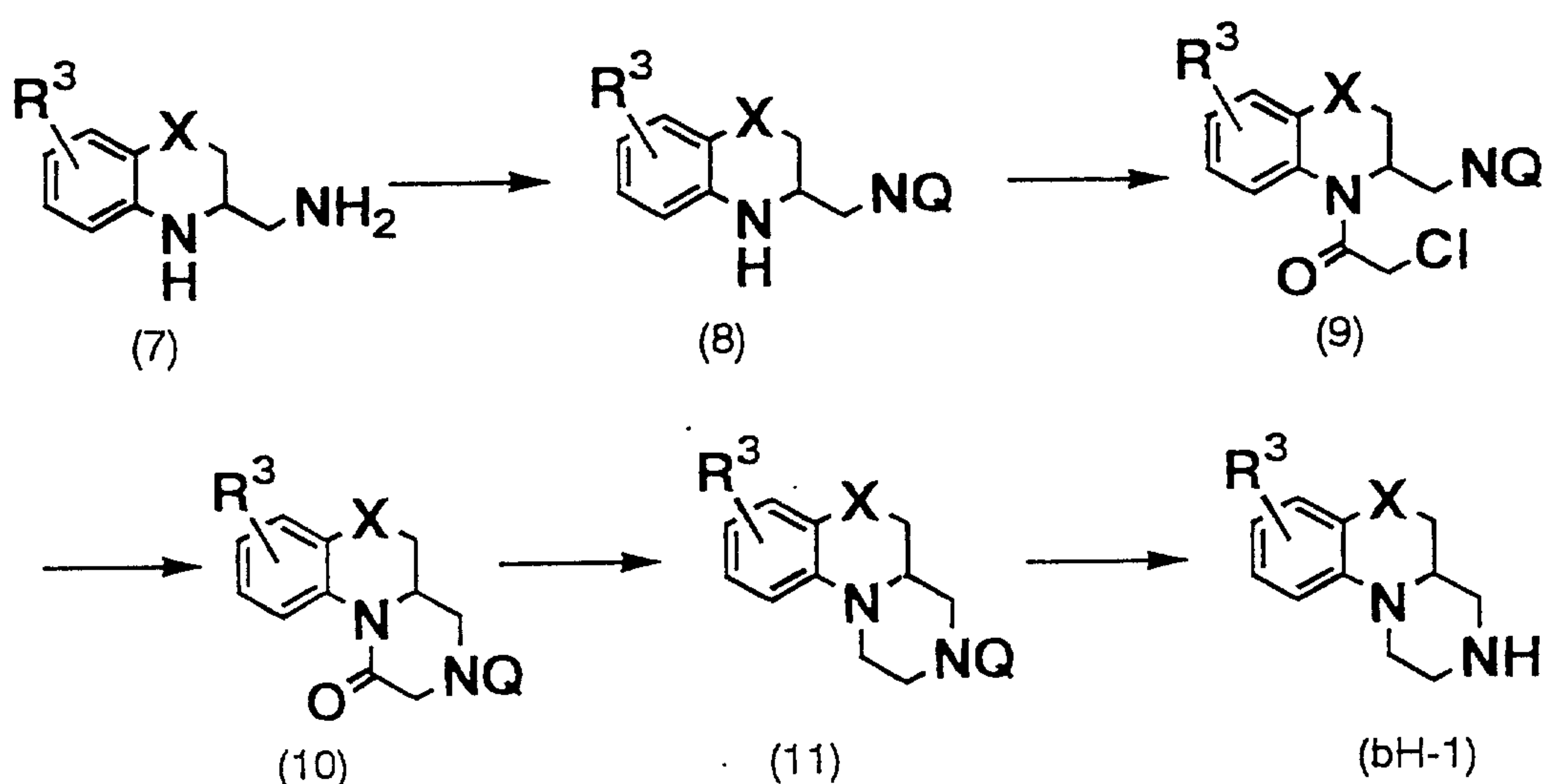
Reaction Formula 4
