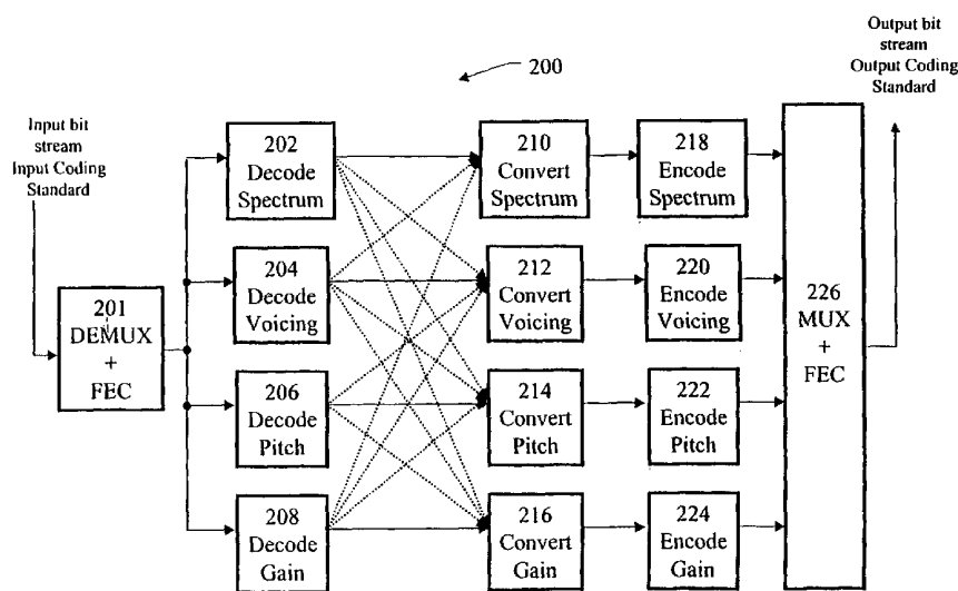
Universal Transcoder
