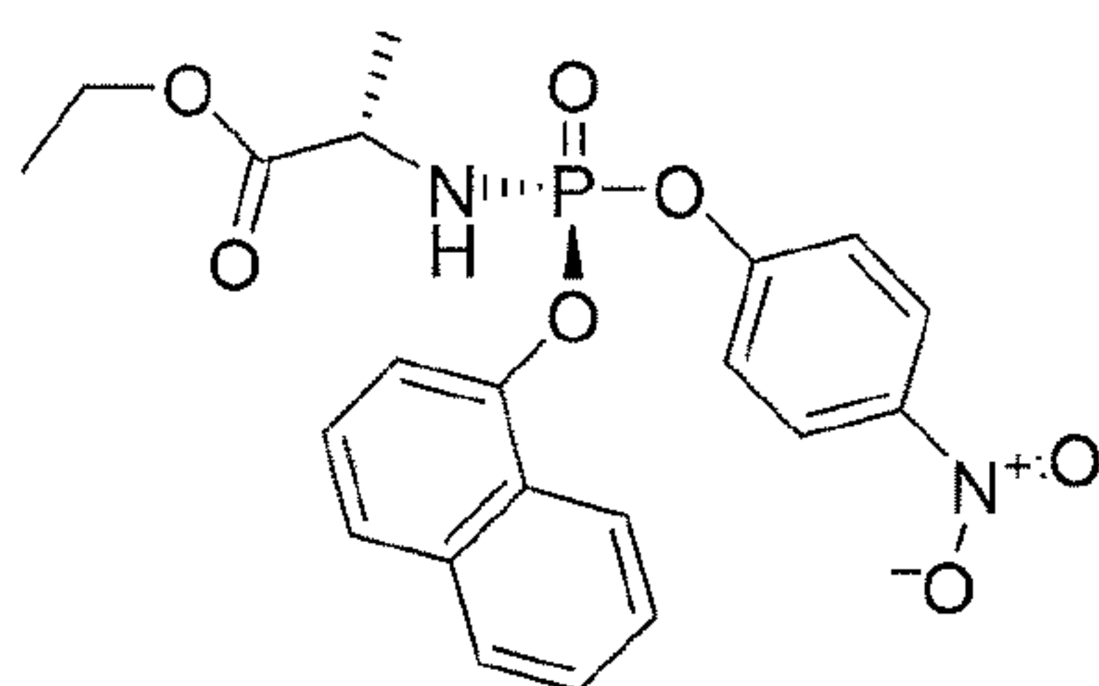
Compound 21
