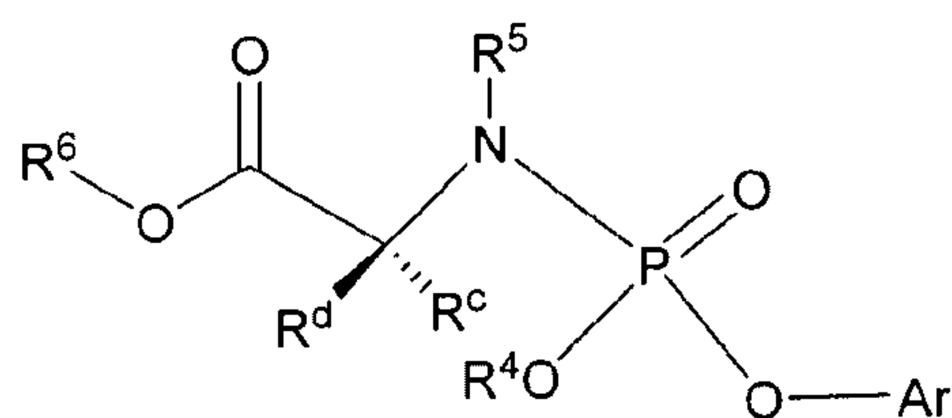
Formula VIII
