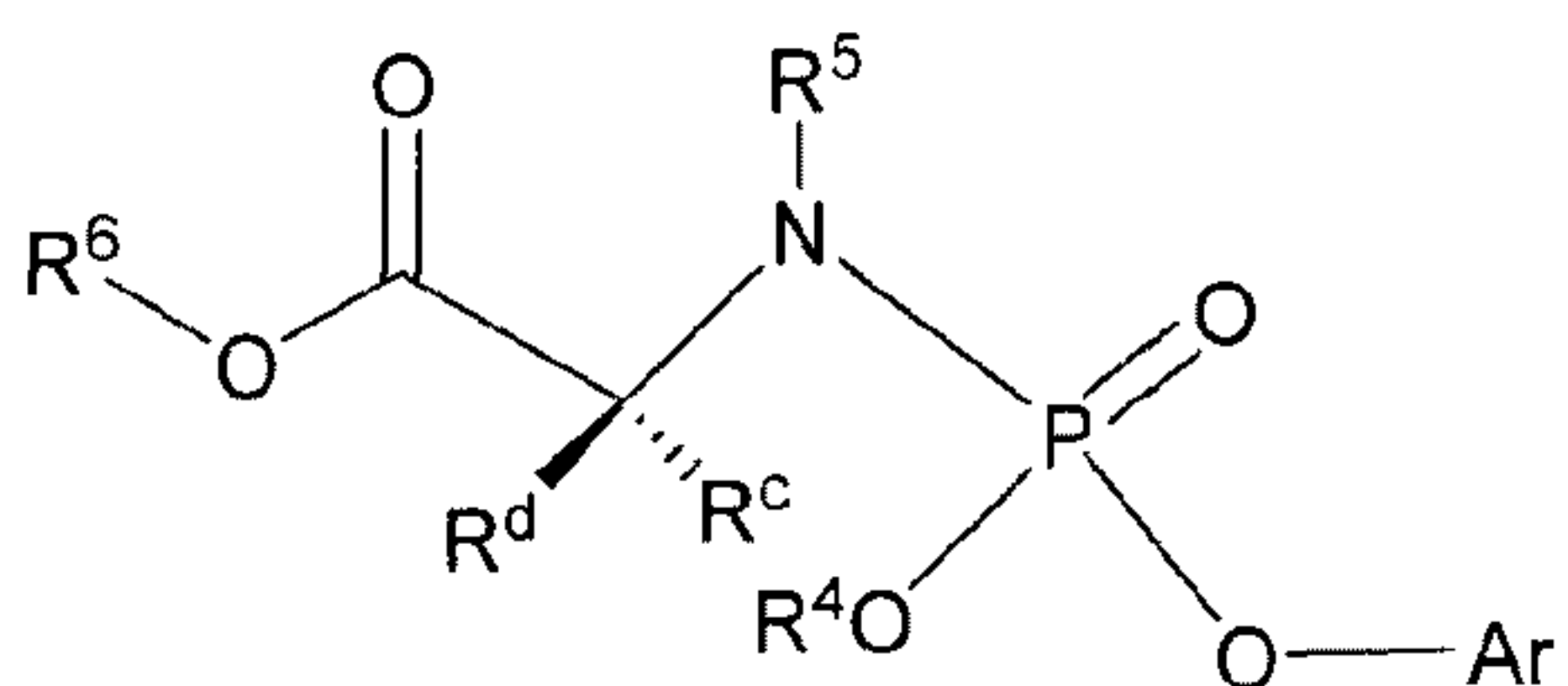
Formula VIII
