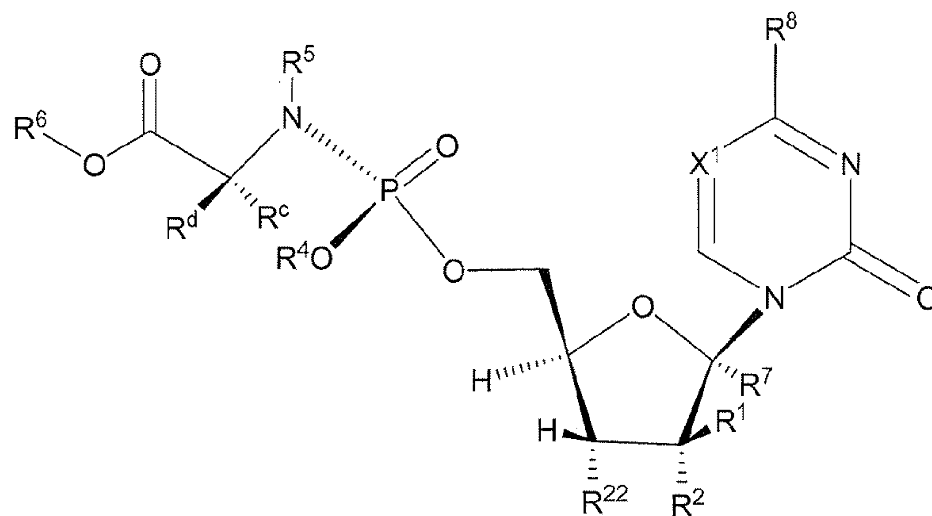
Formula XIIIa
