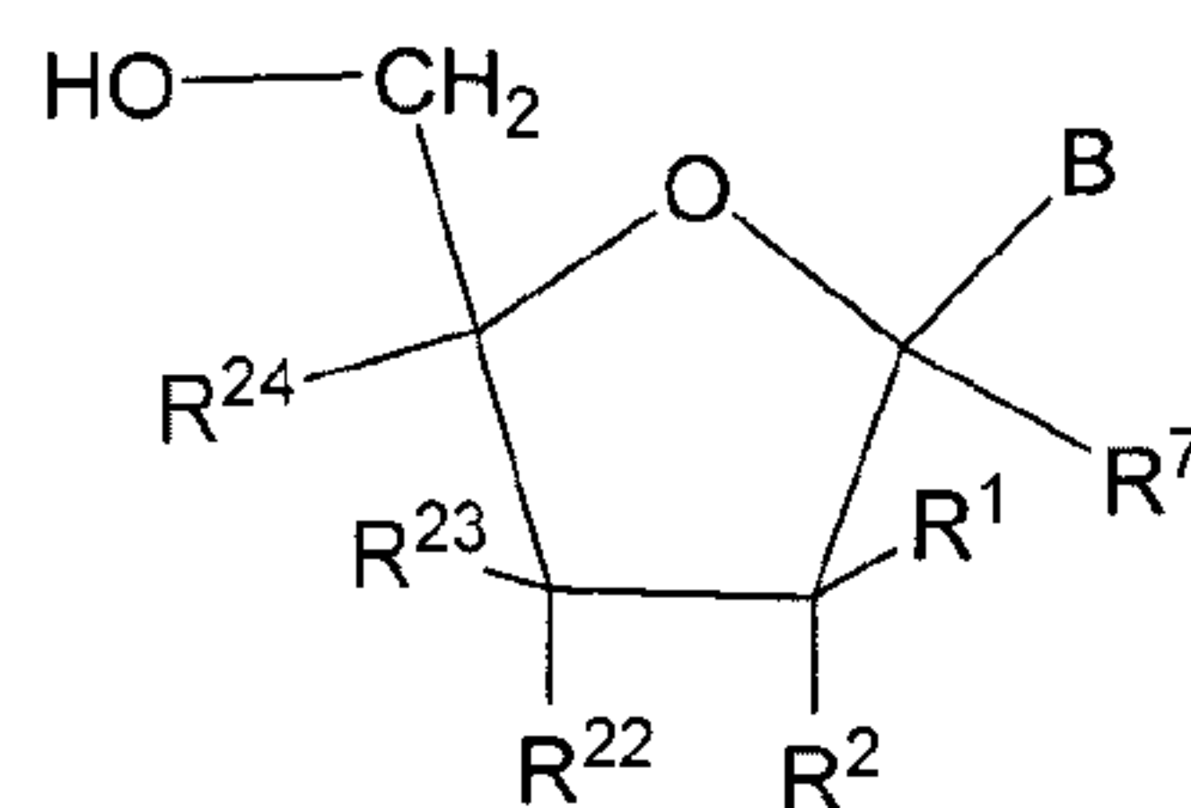
Formula II
