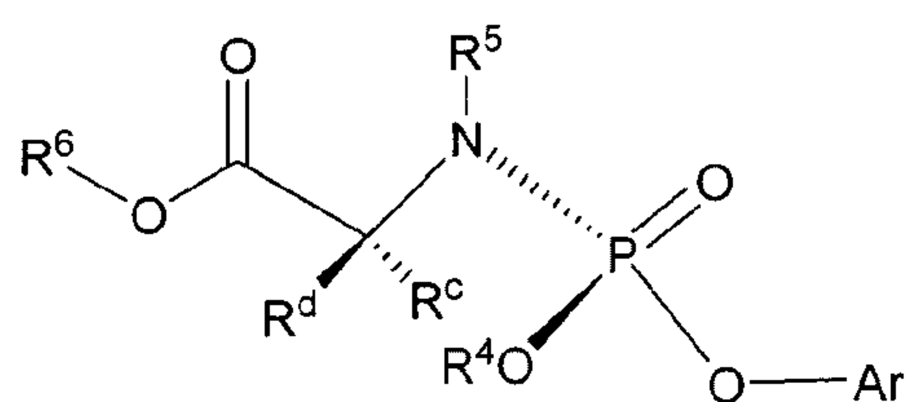
Formula IIIb
