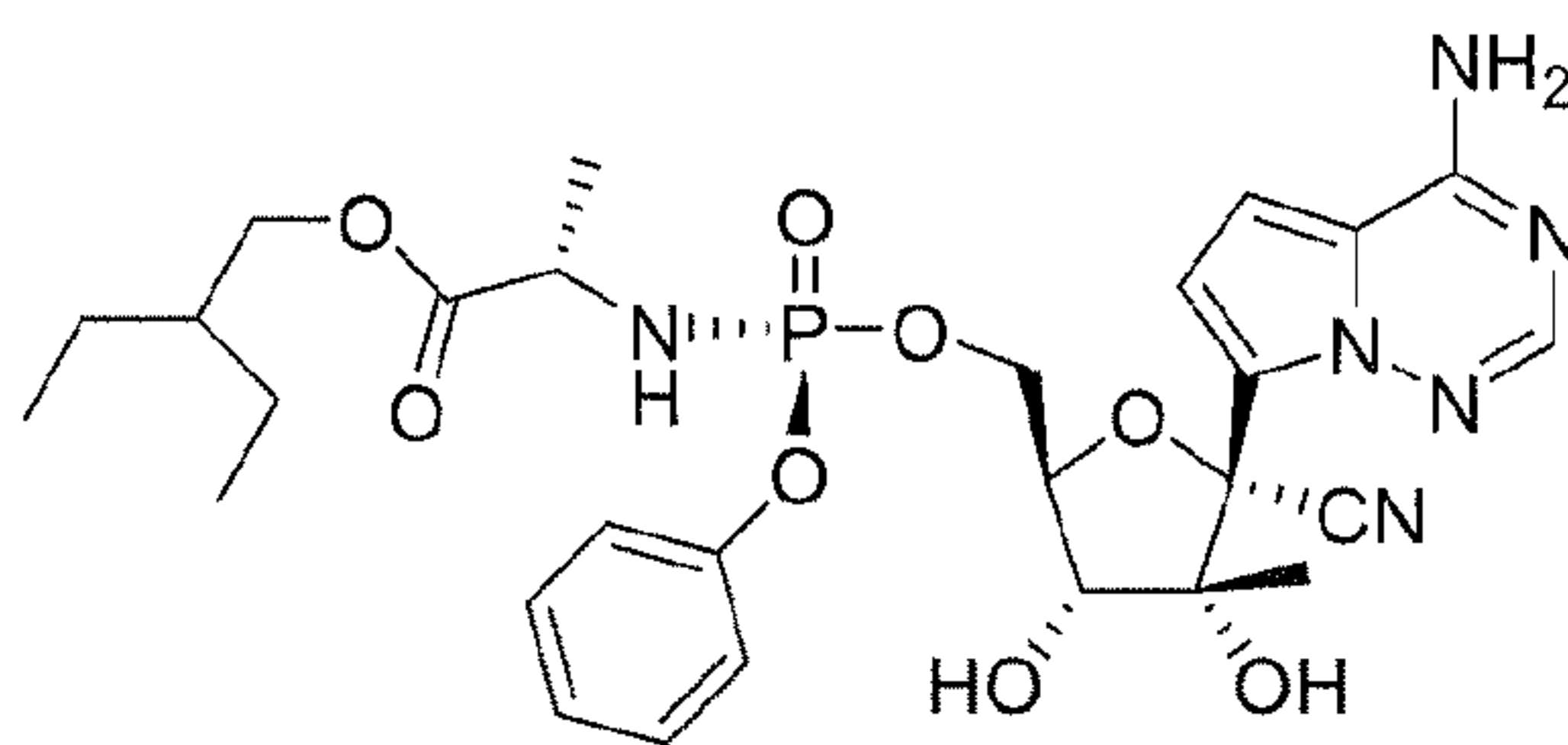
Compound 26
