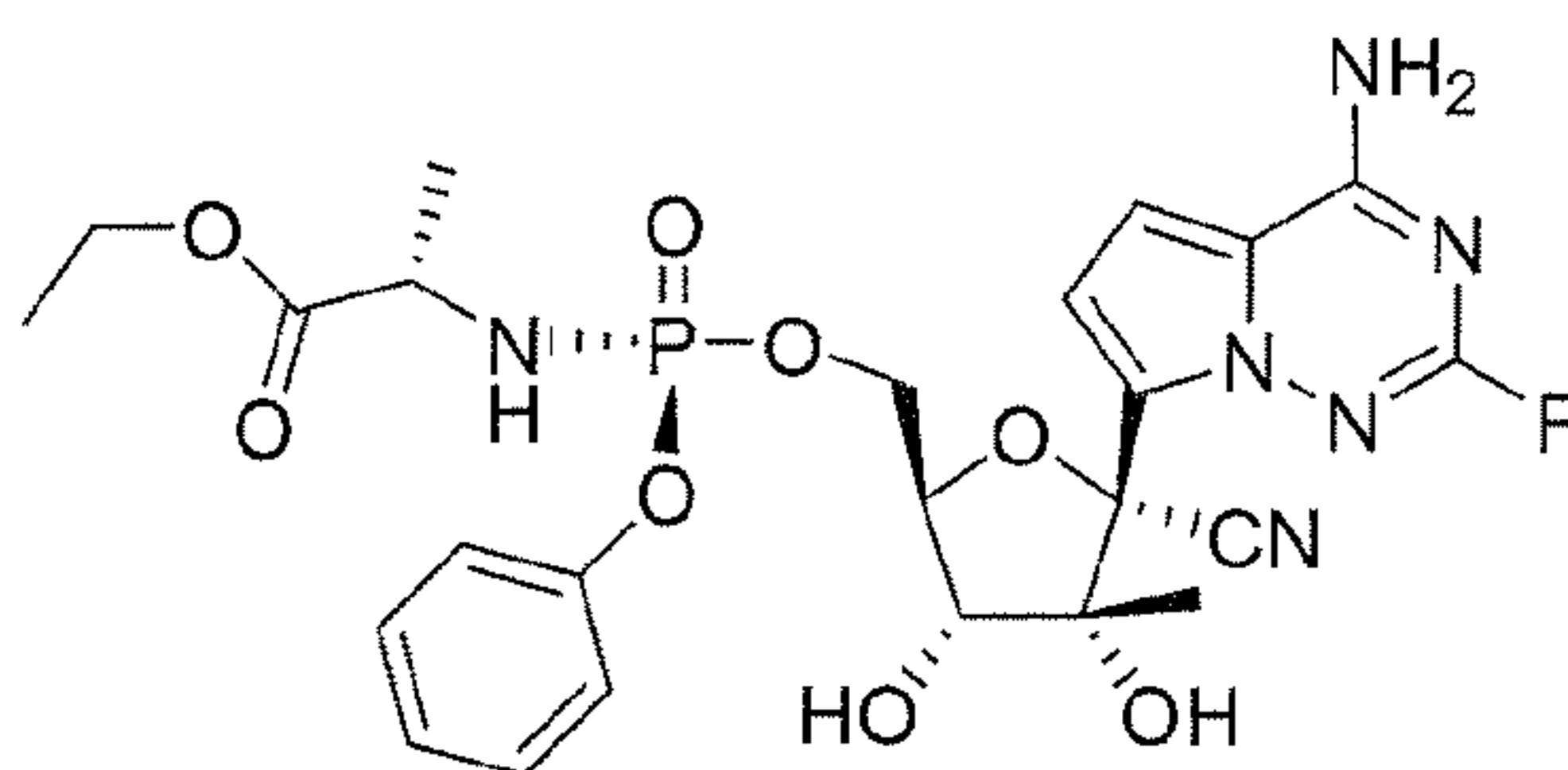
Compound 31
