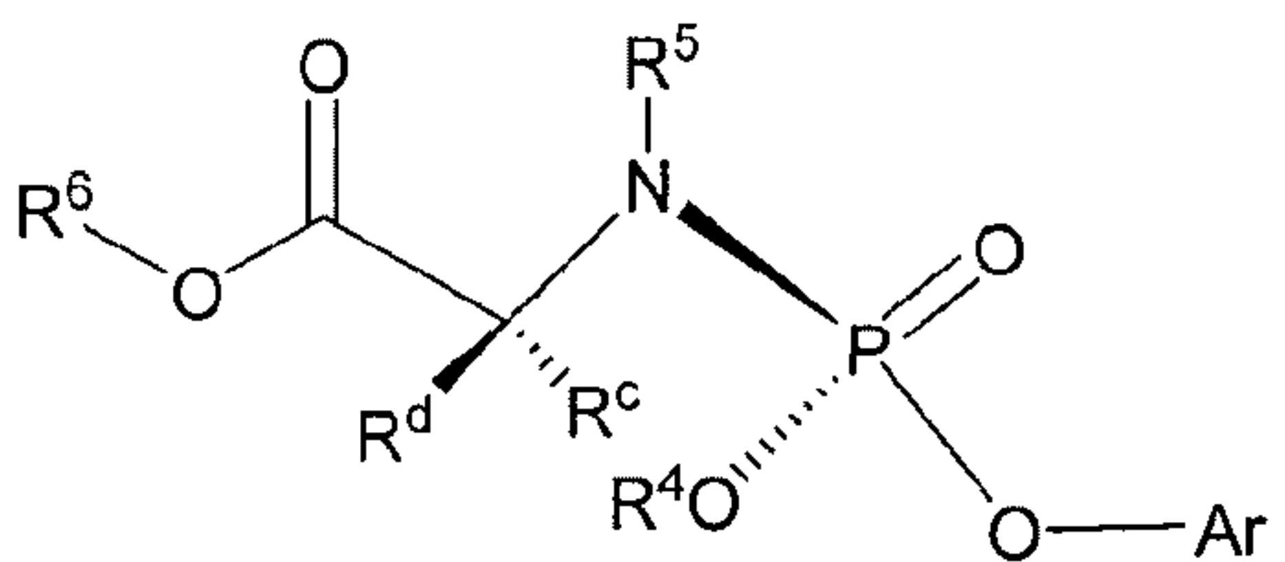
Formula IIIa
