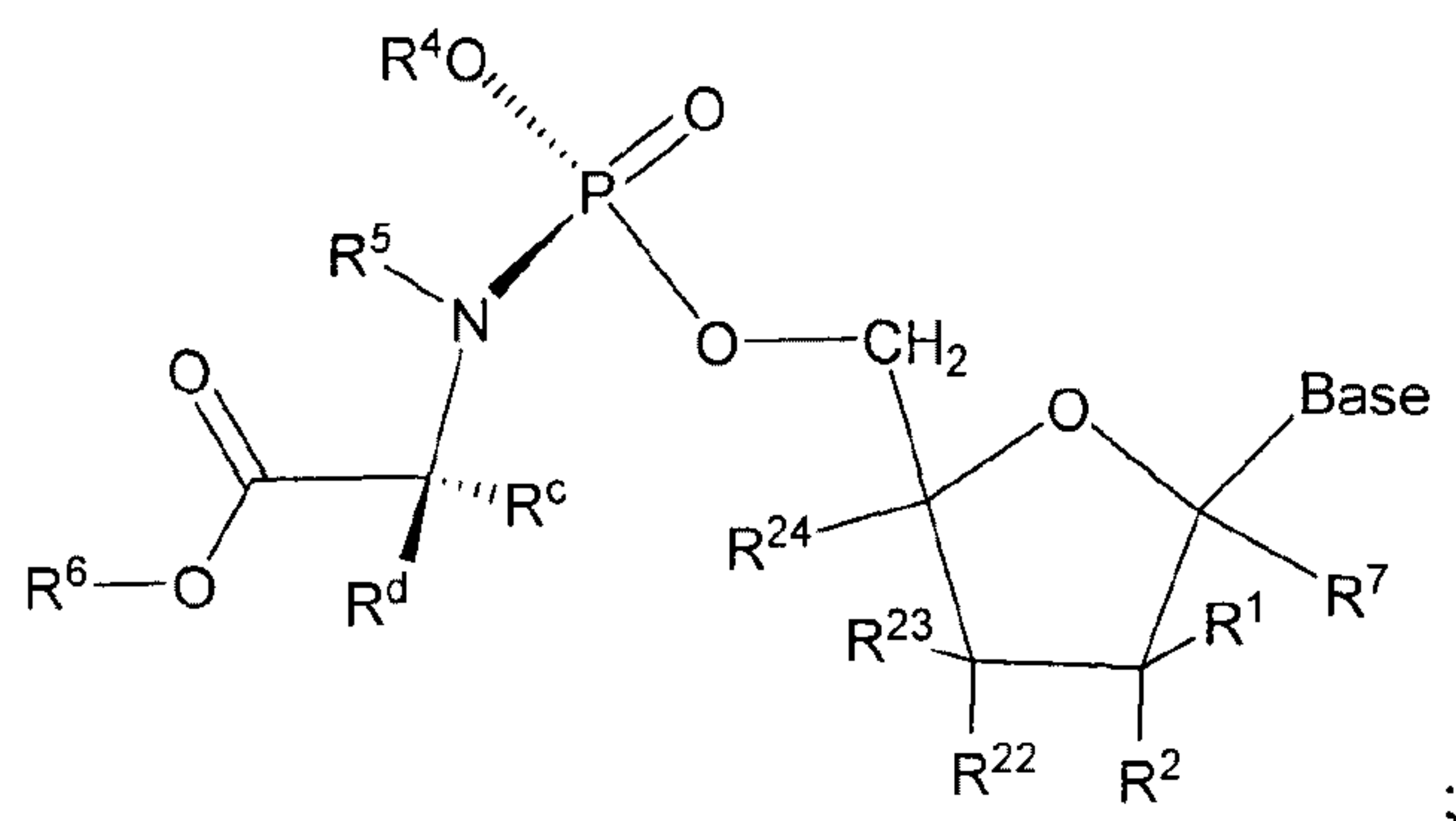
Formula Ib
