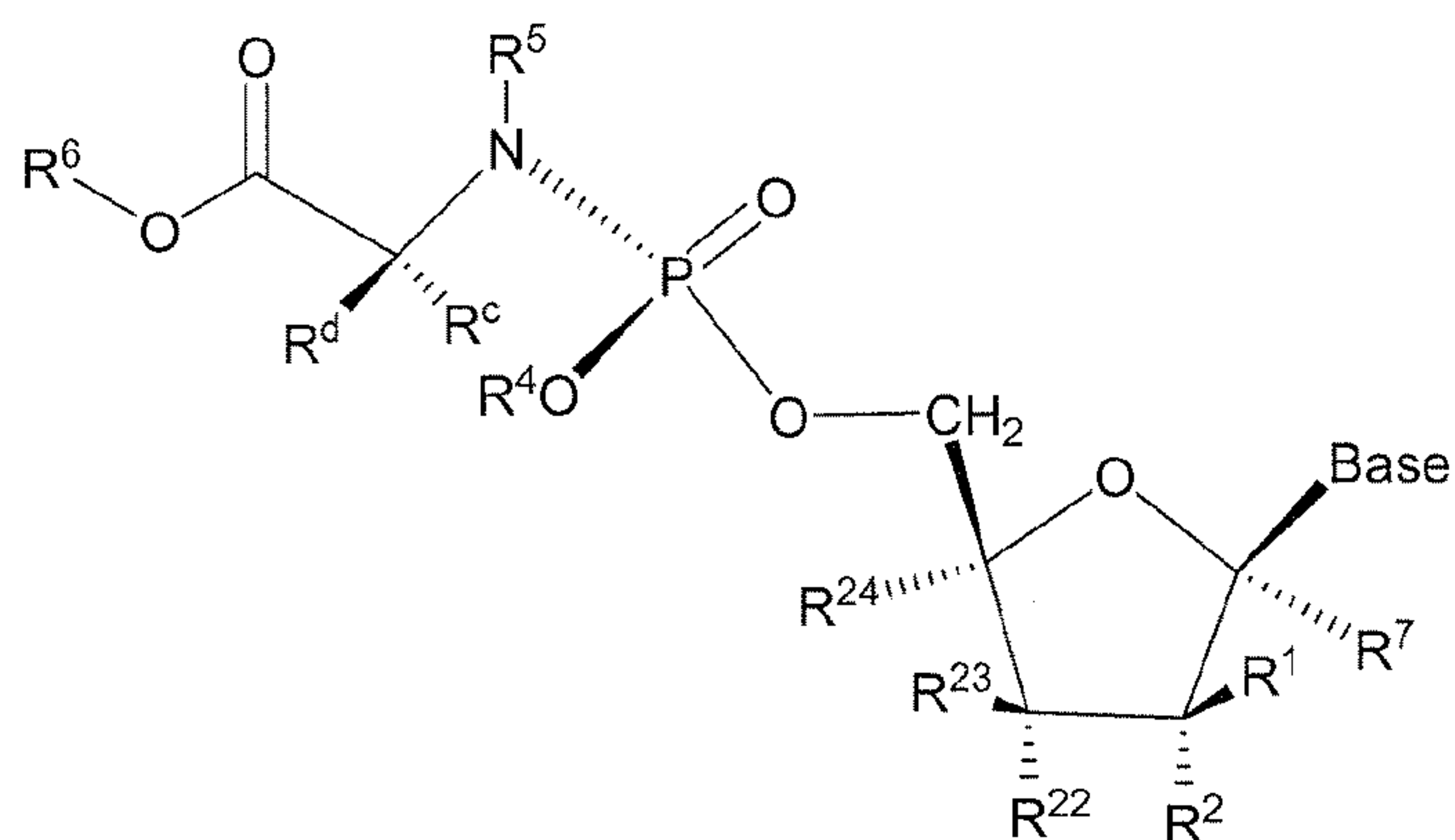
Formula IVa
