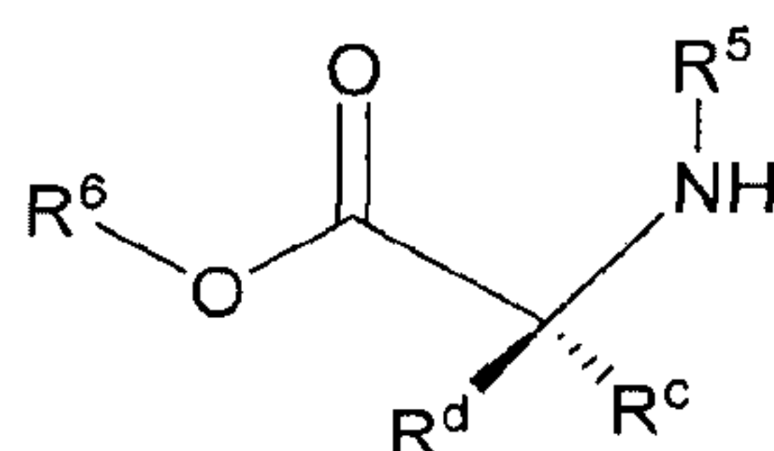
Formula IX
