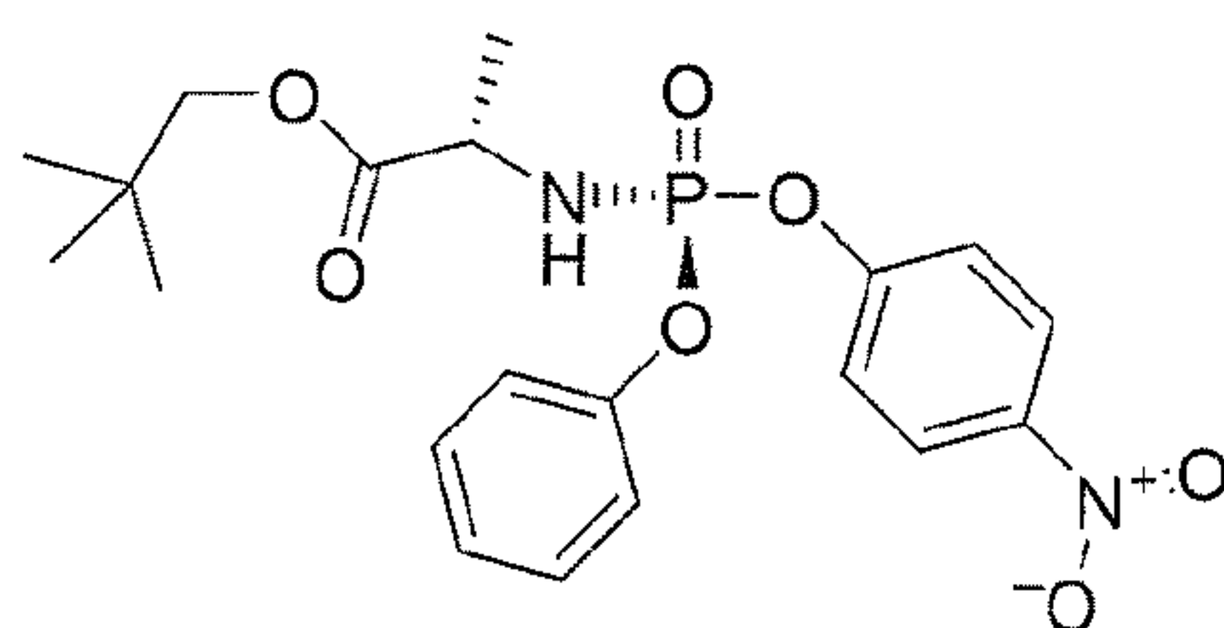
Compound 24
