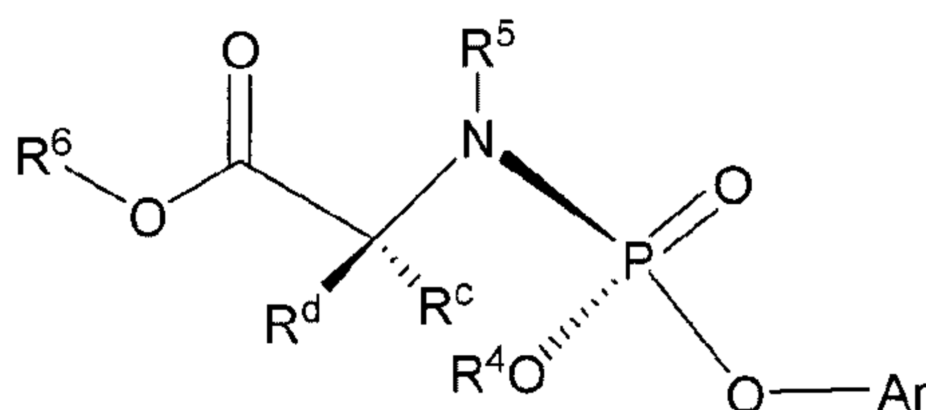
Formula IIIa
