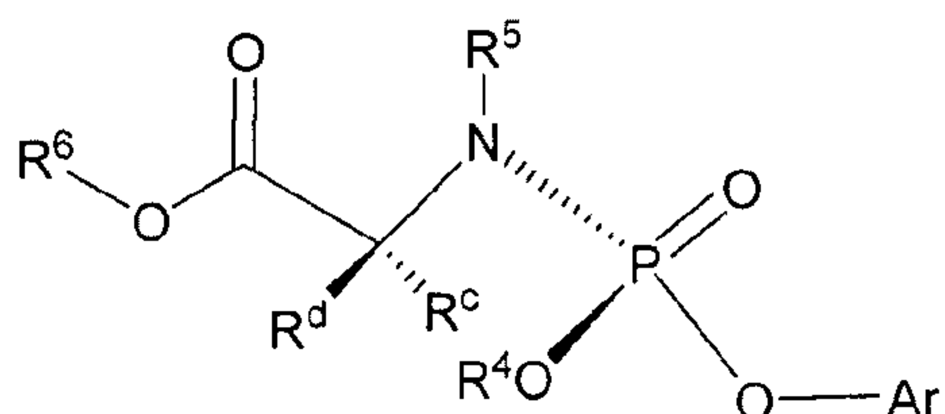
Formula IIIb
