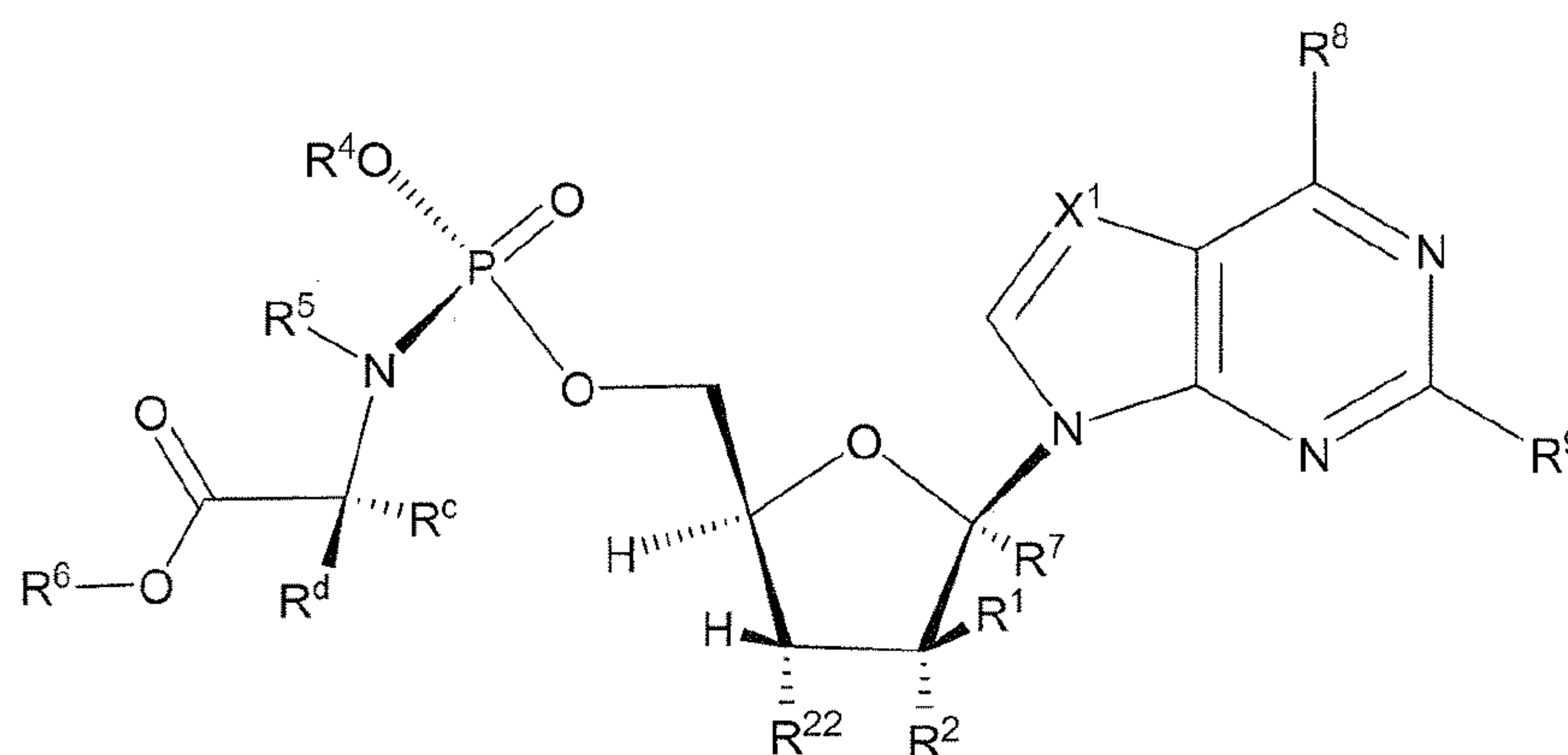
Formula XIb
