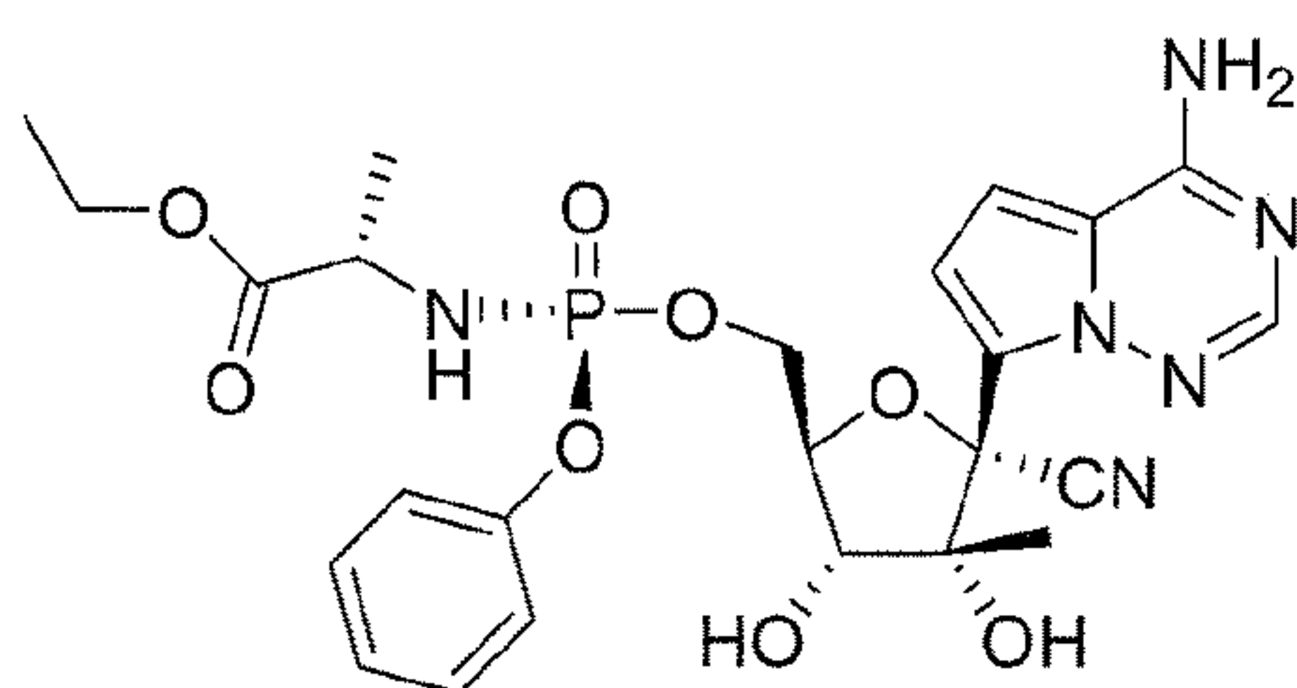
Compound 25
