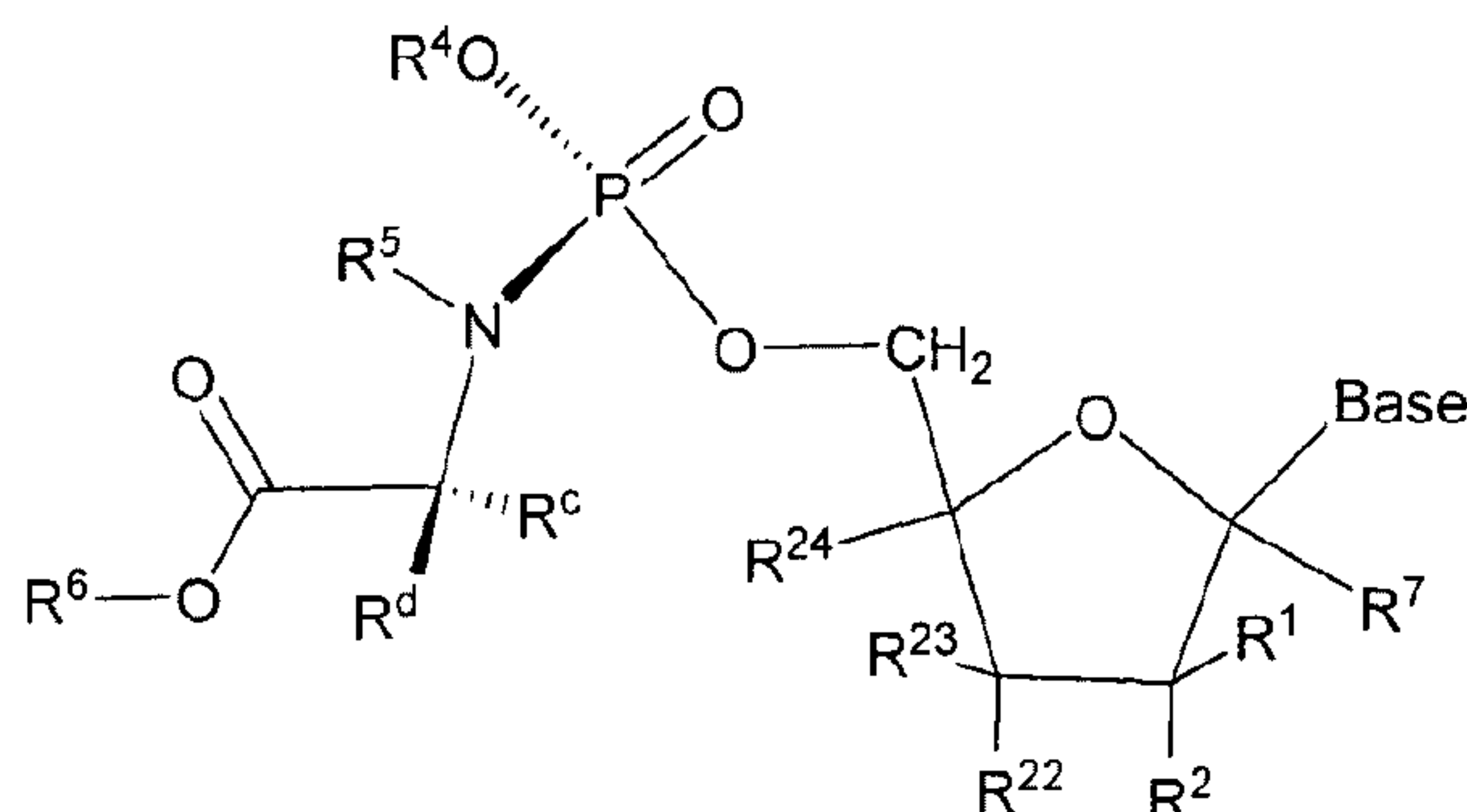
Formula Ib
