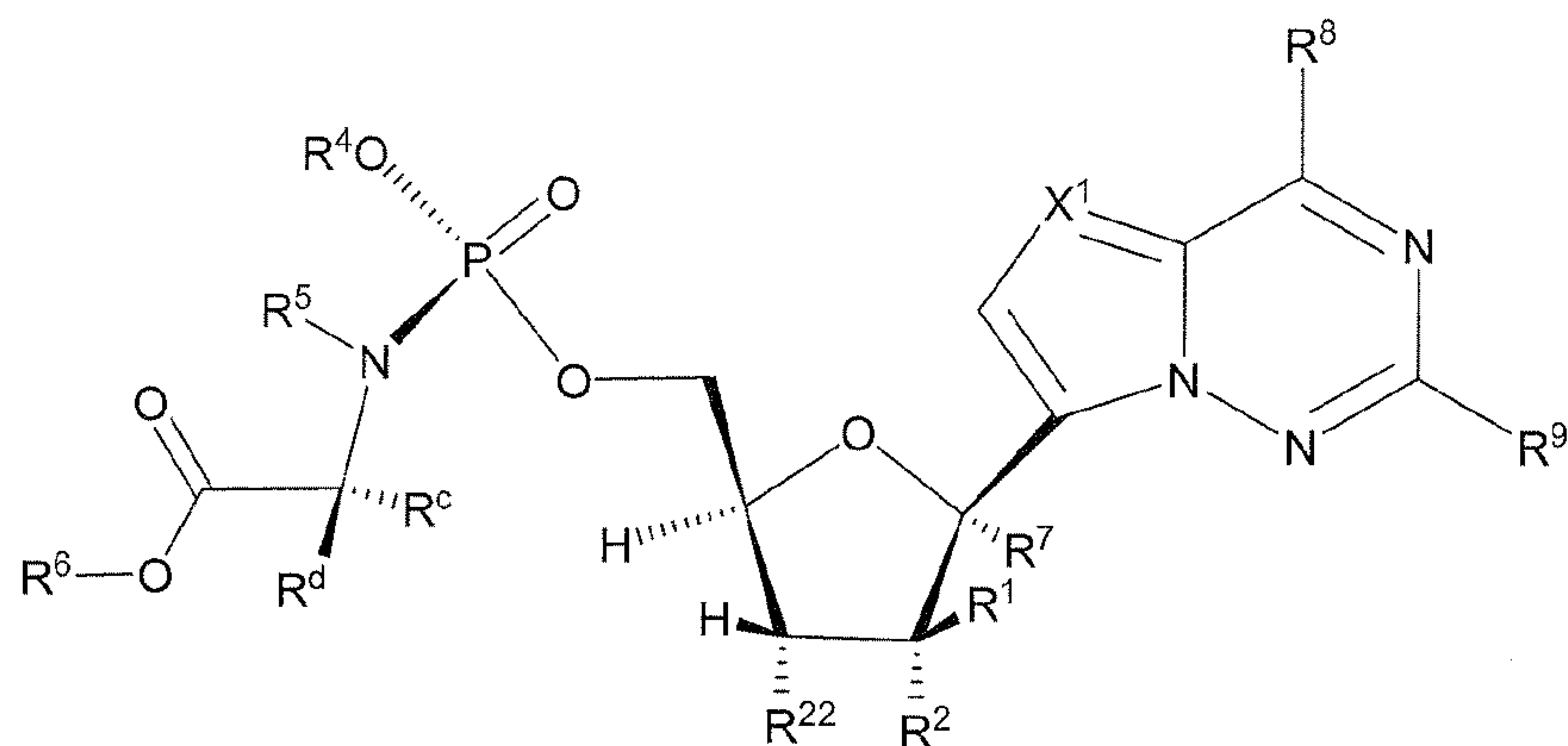
Formula VIb
