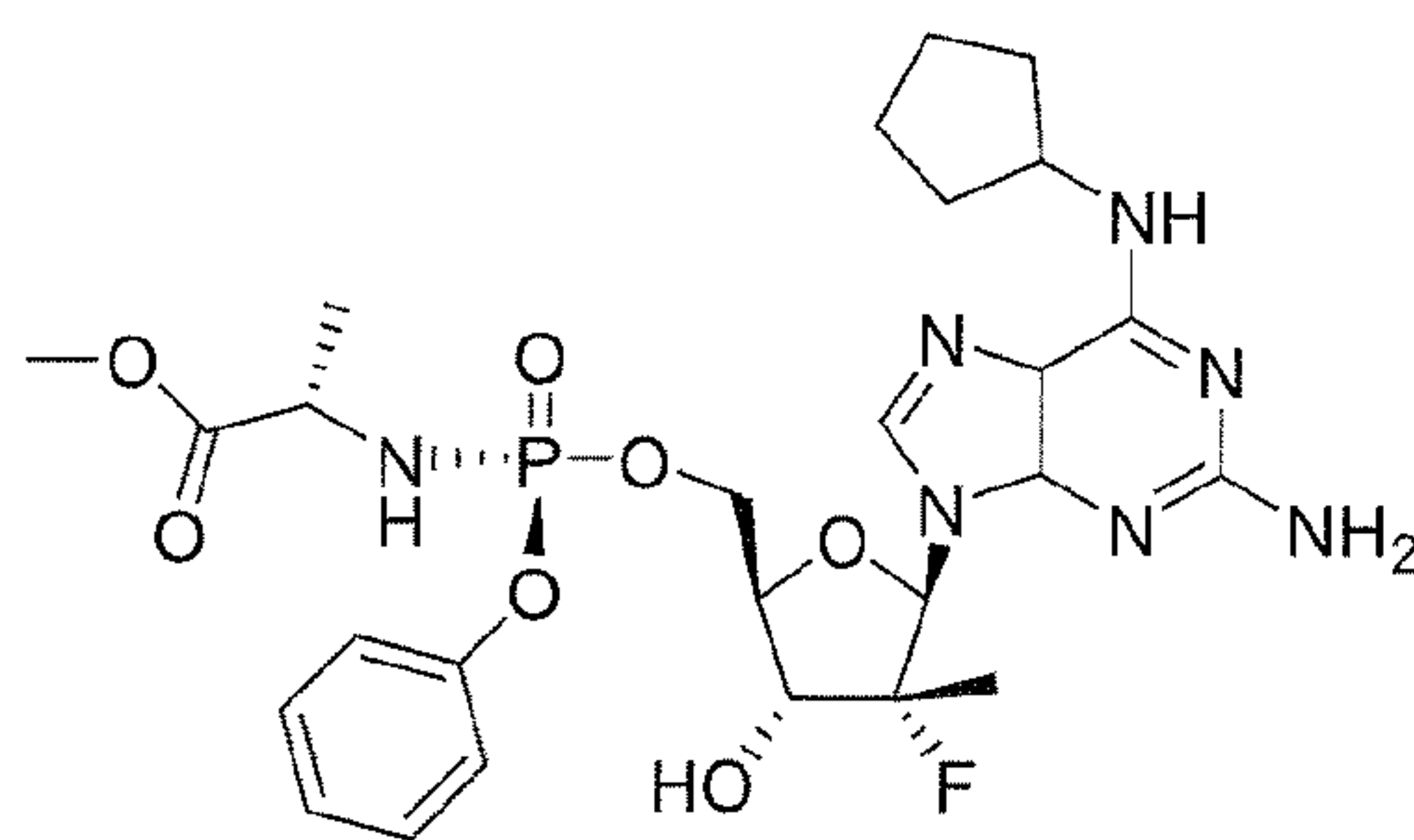
Compound 37
