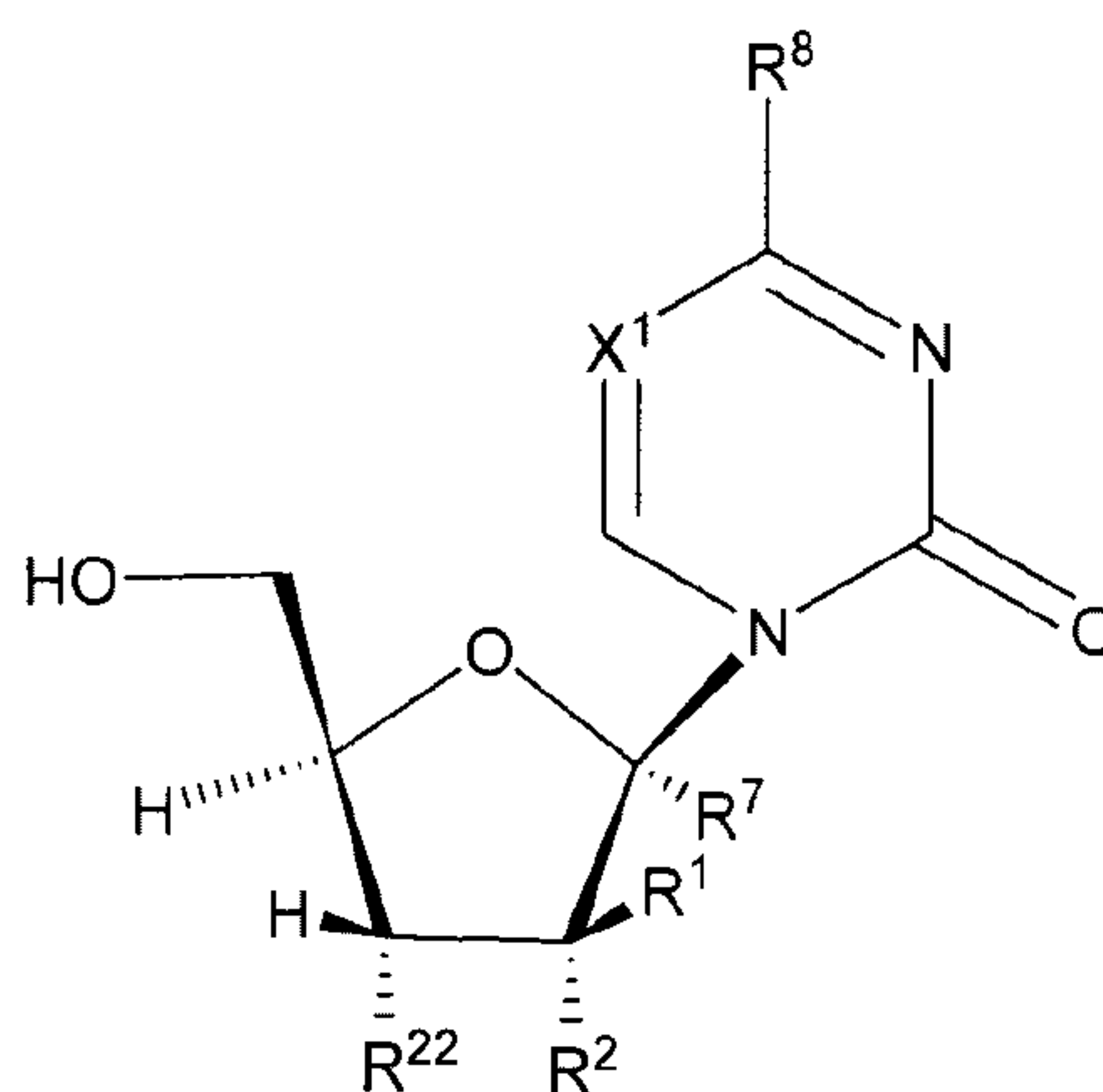
Formula XIV
