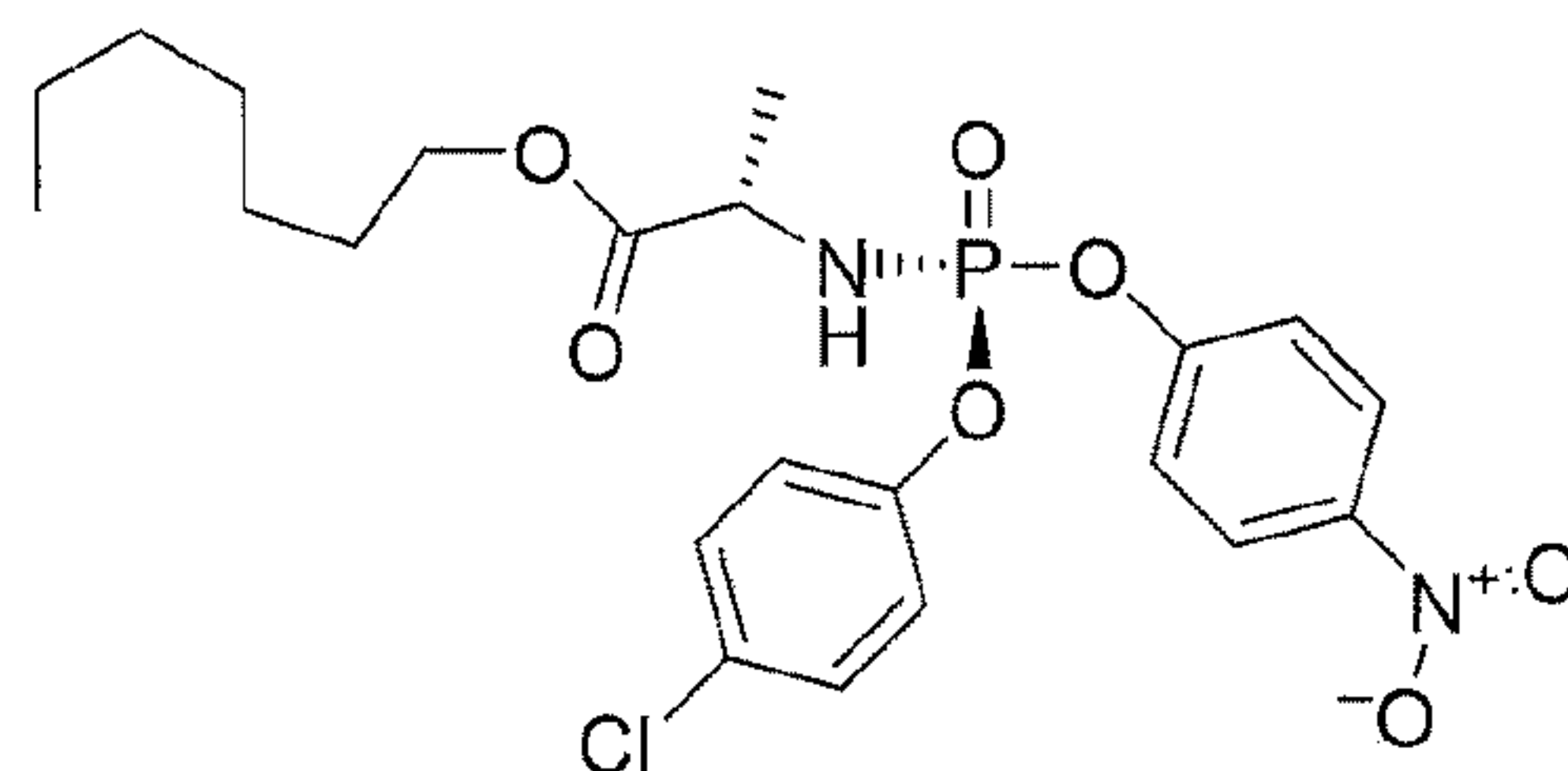
Compound 19
