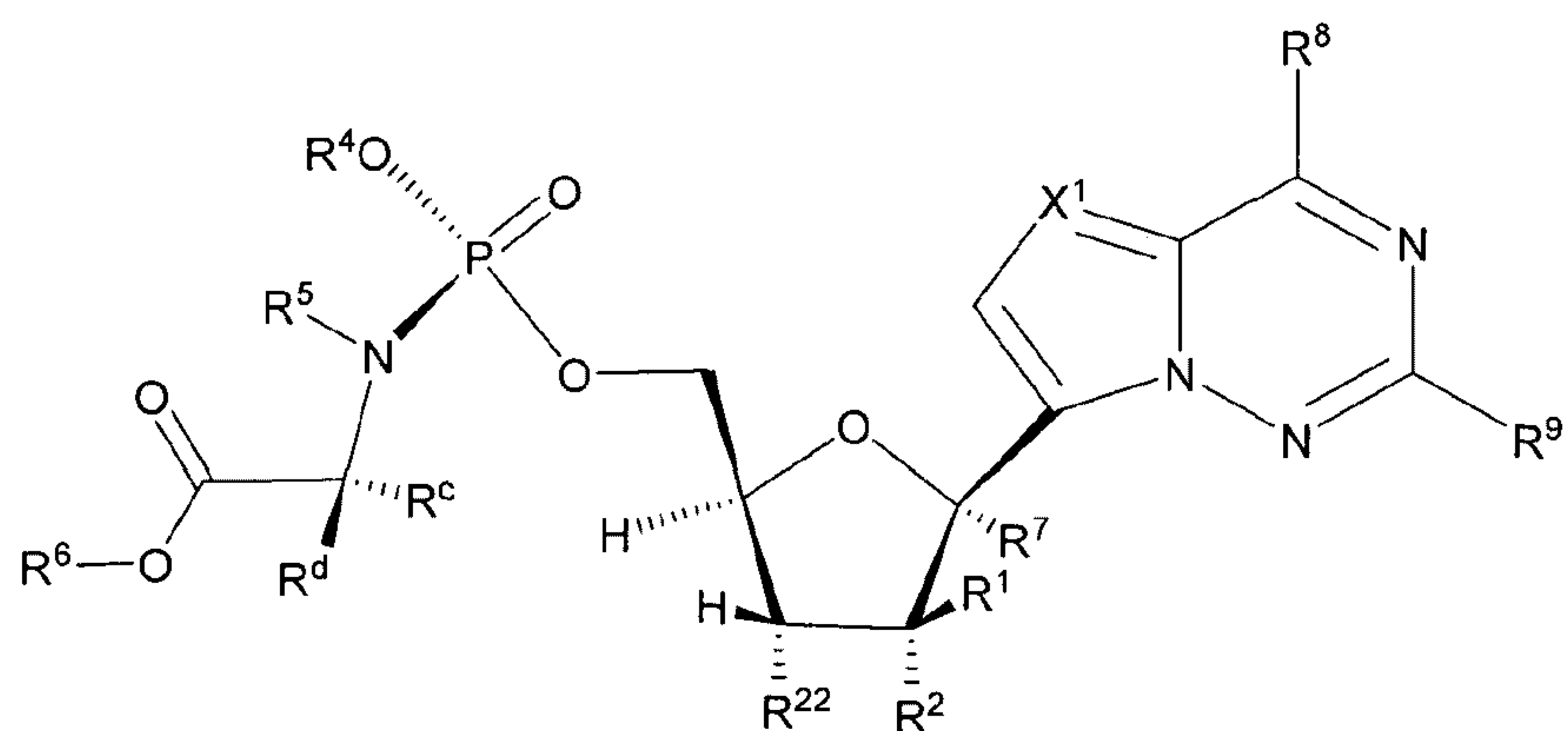
Formula VIb
