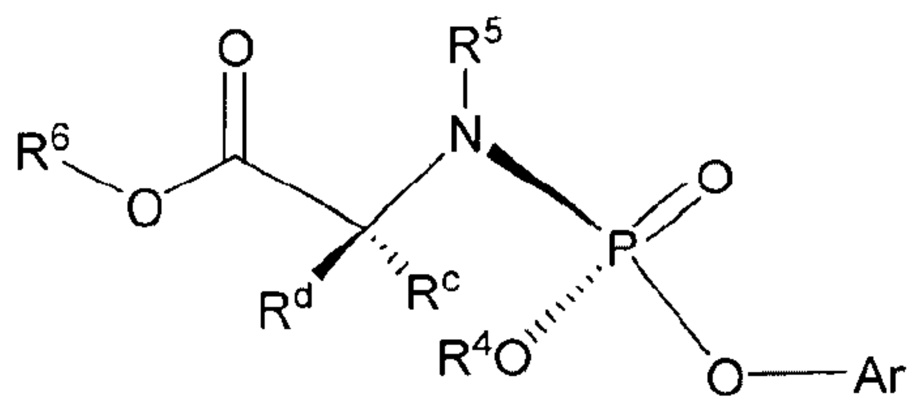
Formula IIIa
