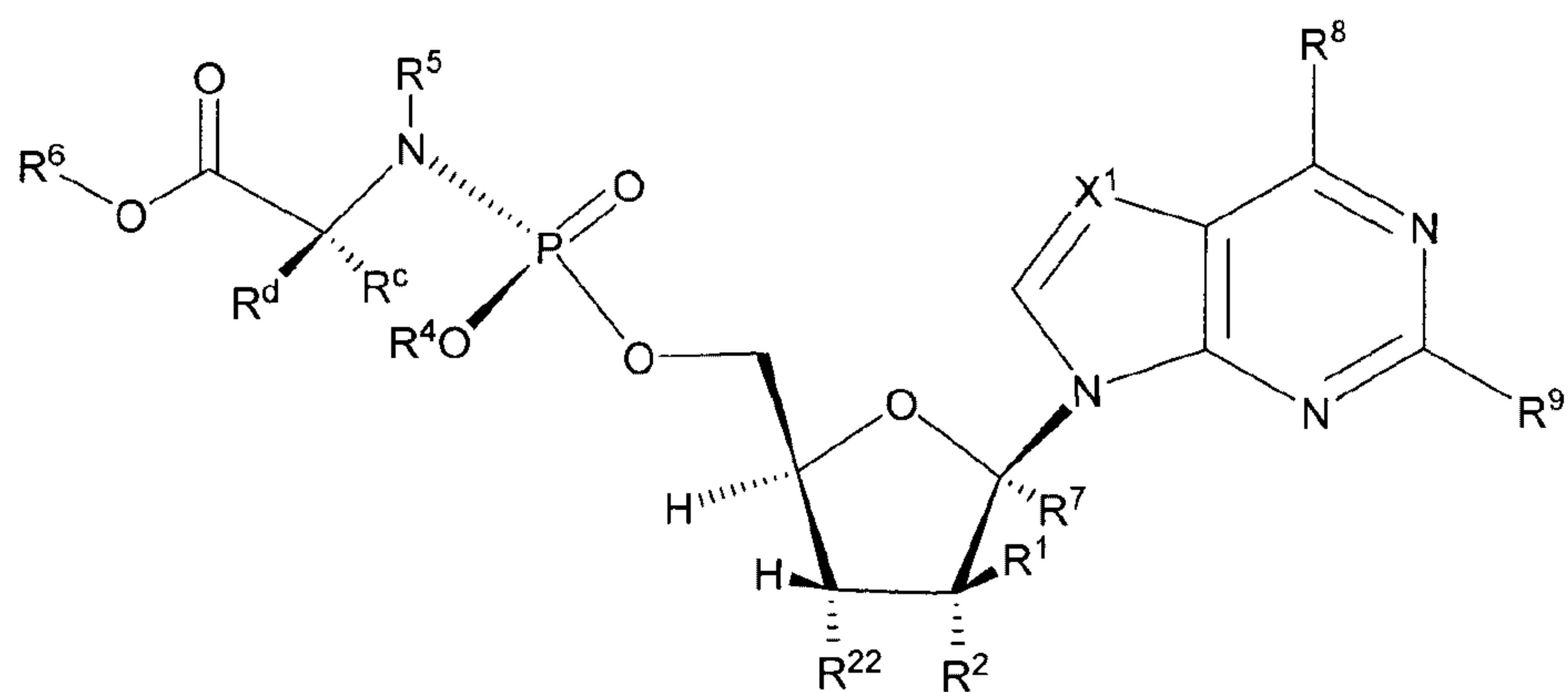
Formula XIa
