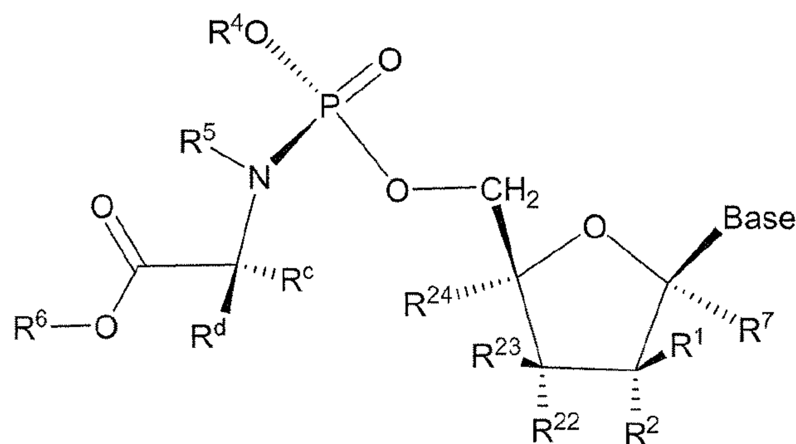
Formula IVb
