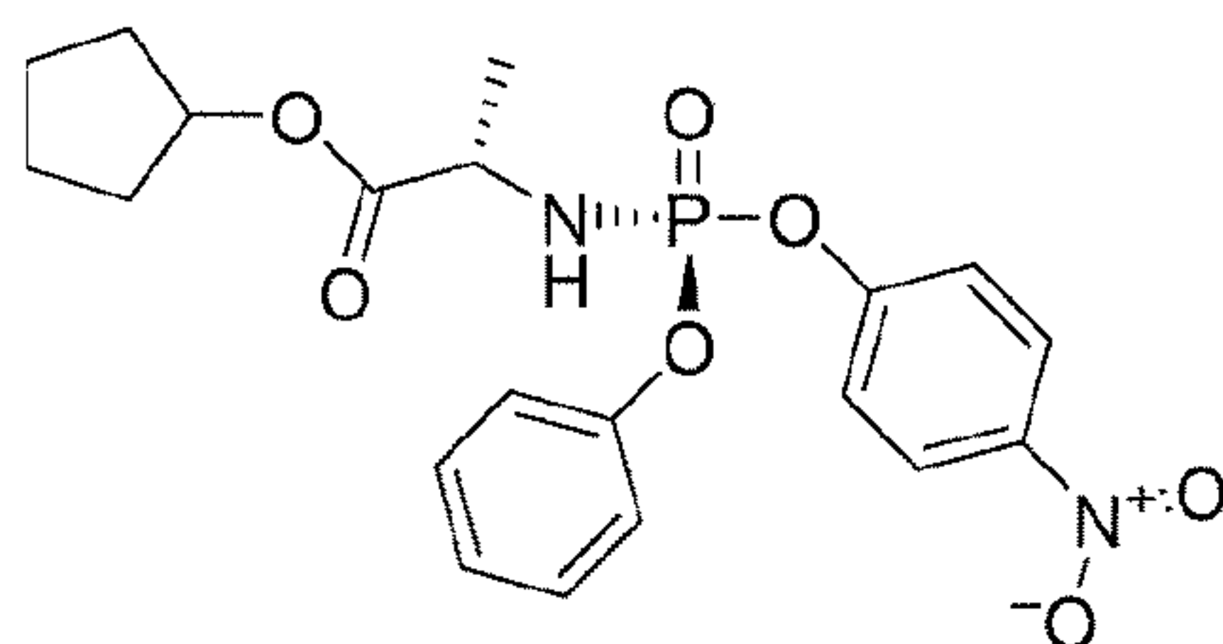
Compound 17
