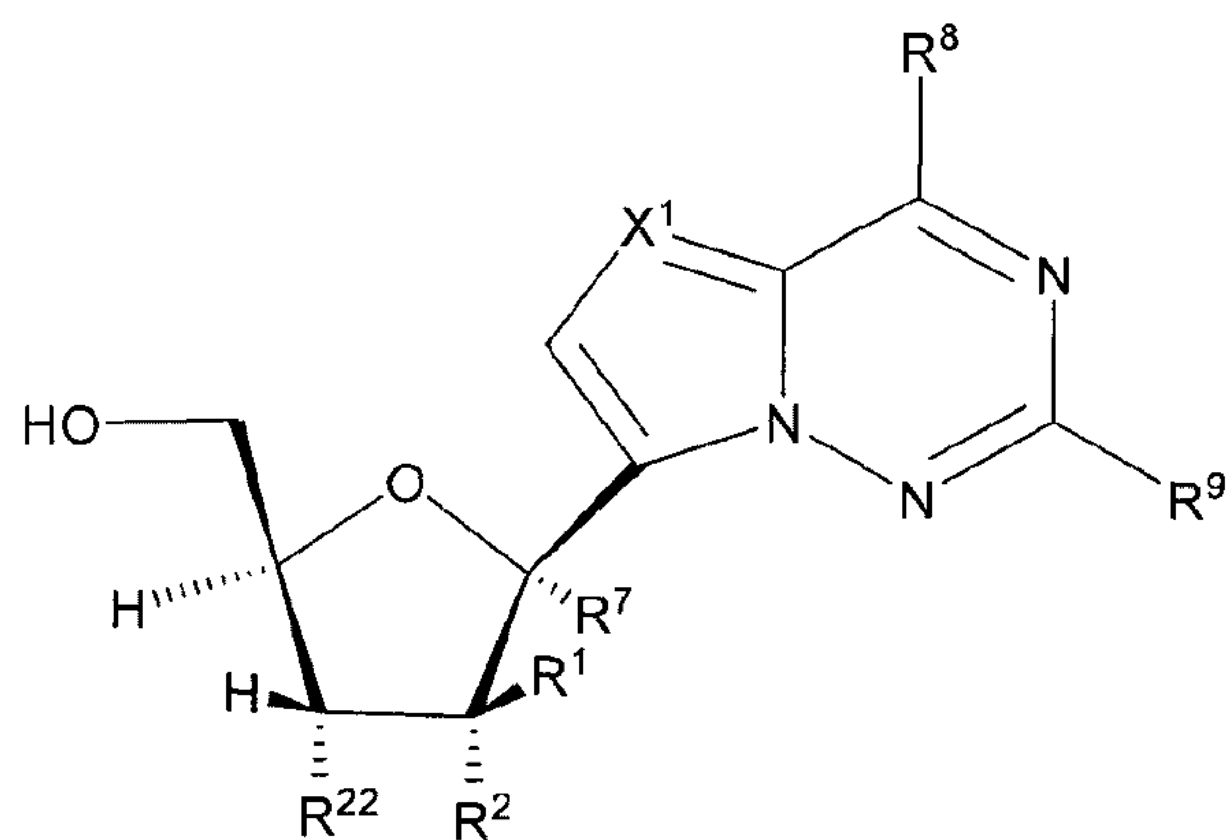
Formula VII
