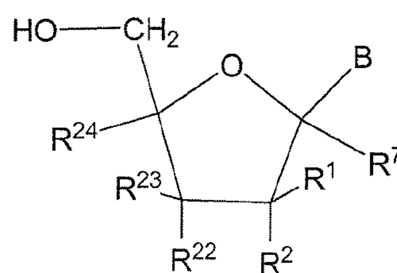
Formula II
