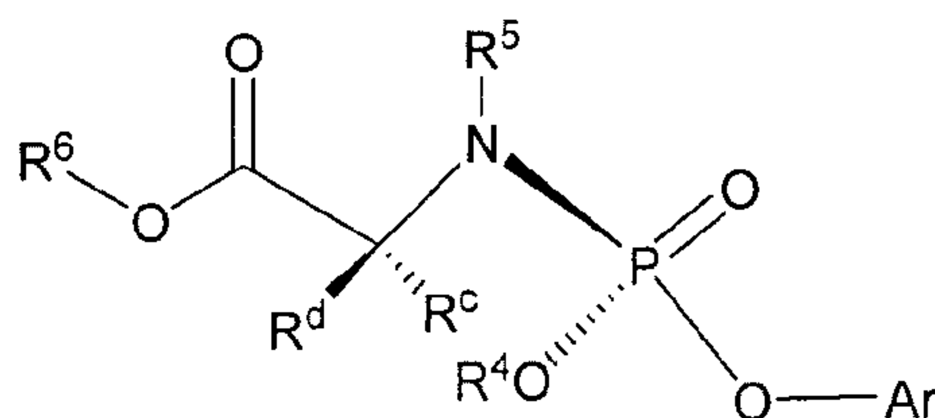
Formula IIIa
