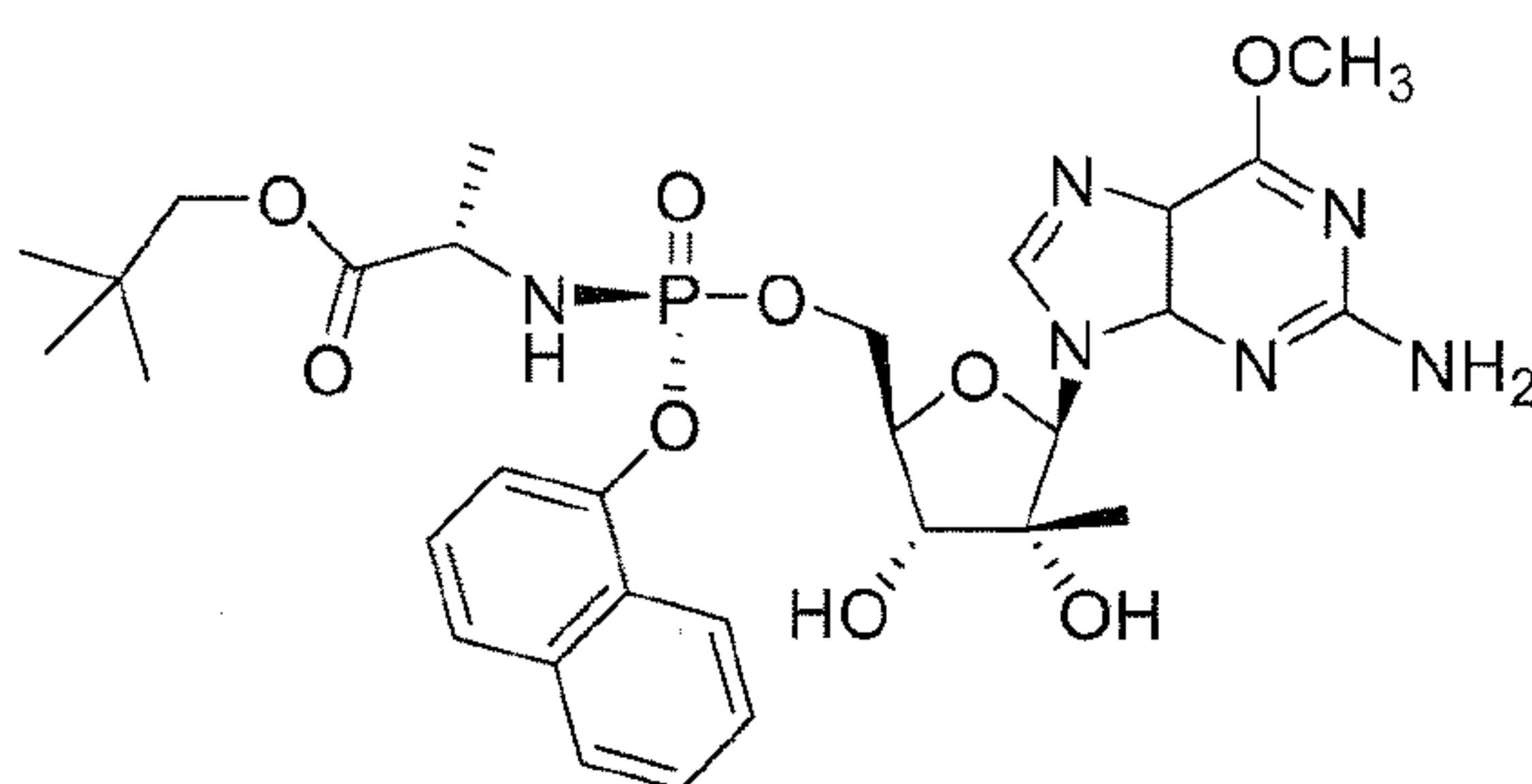
Compound 36
