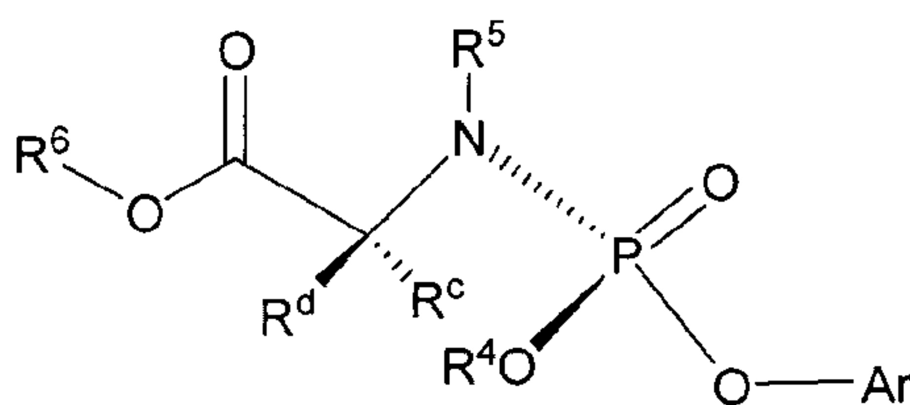
Formula IIIb
