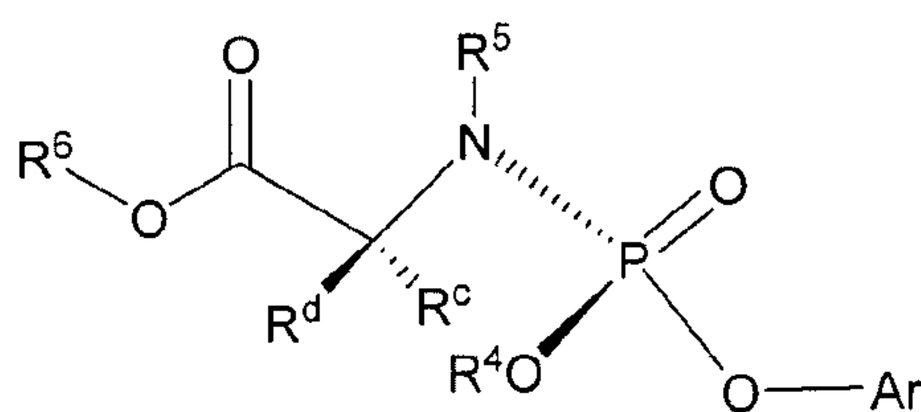
Formula IIIb
