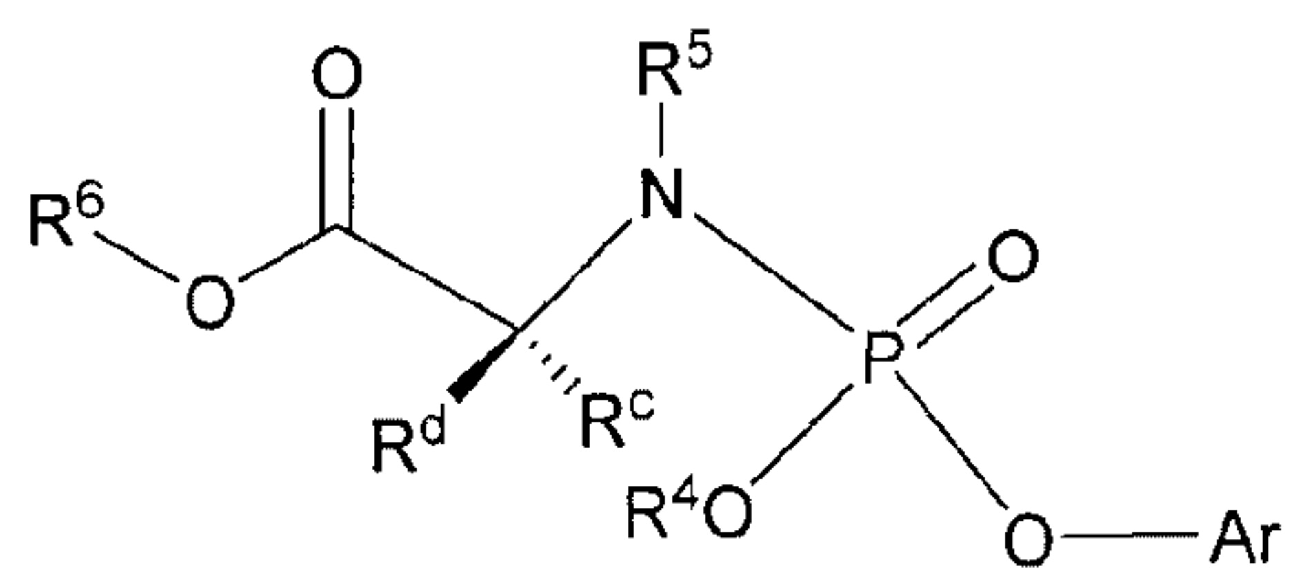
Formula VIII
