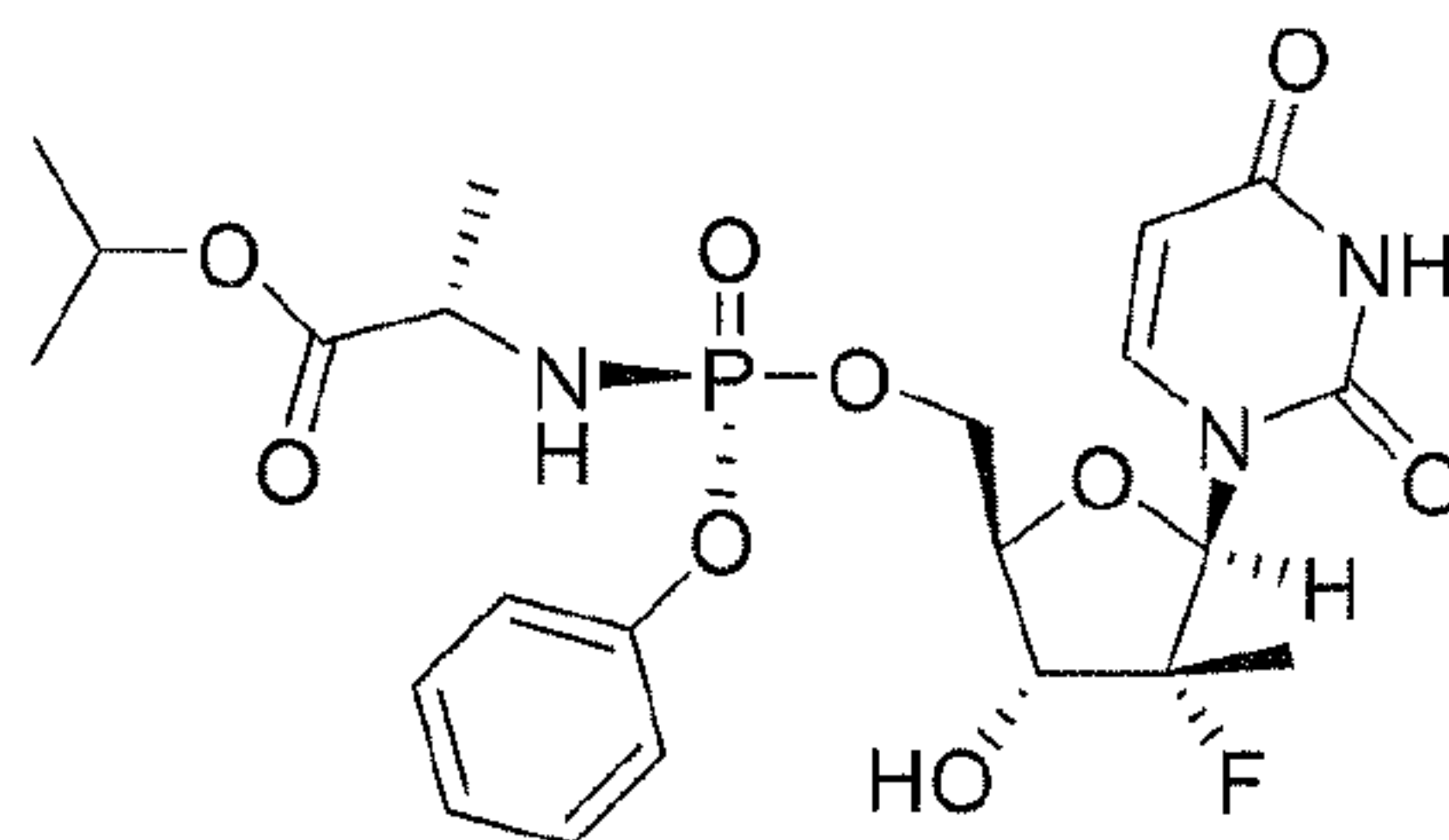
Compound 34
