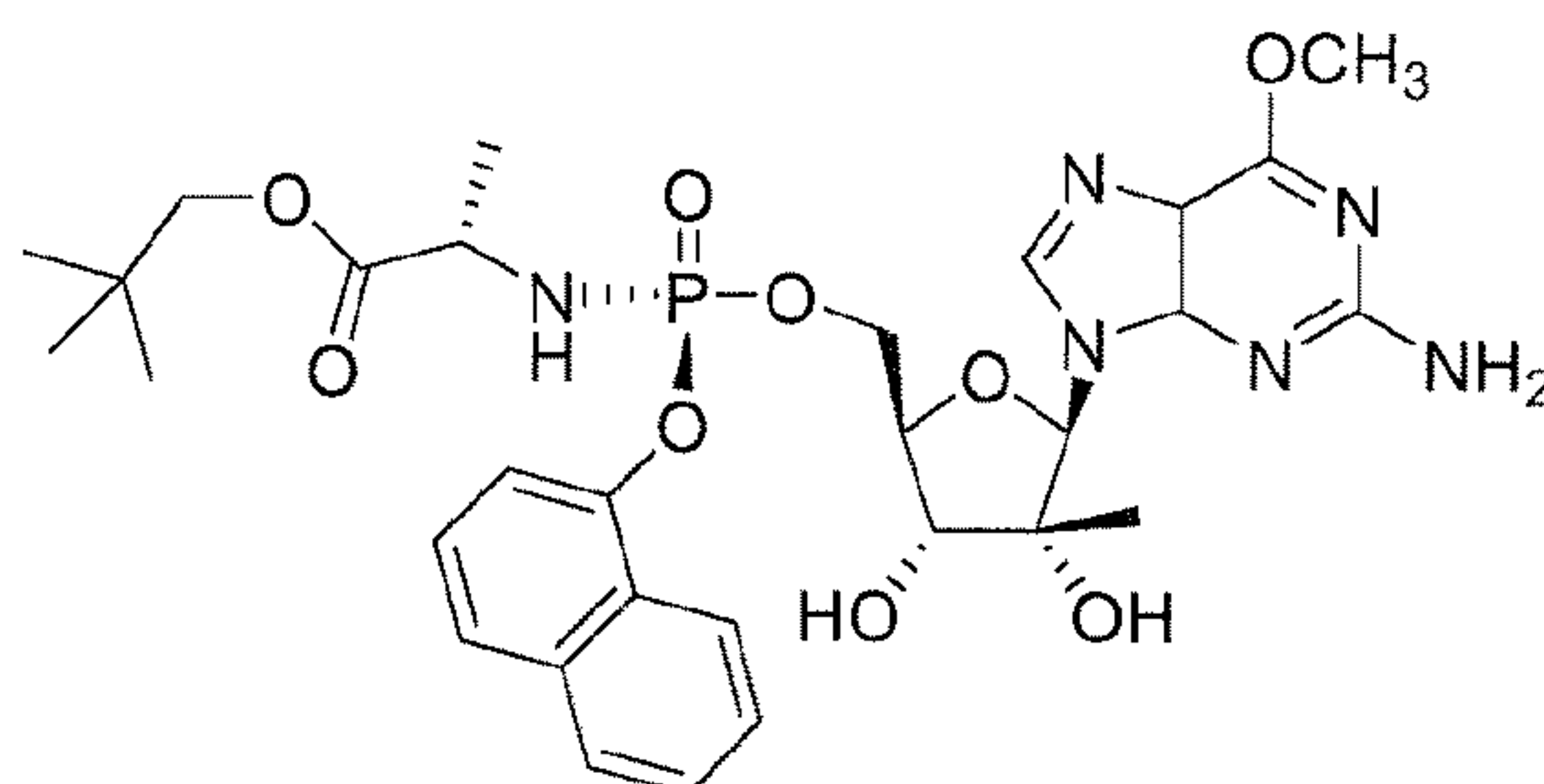
Compound 35
