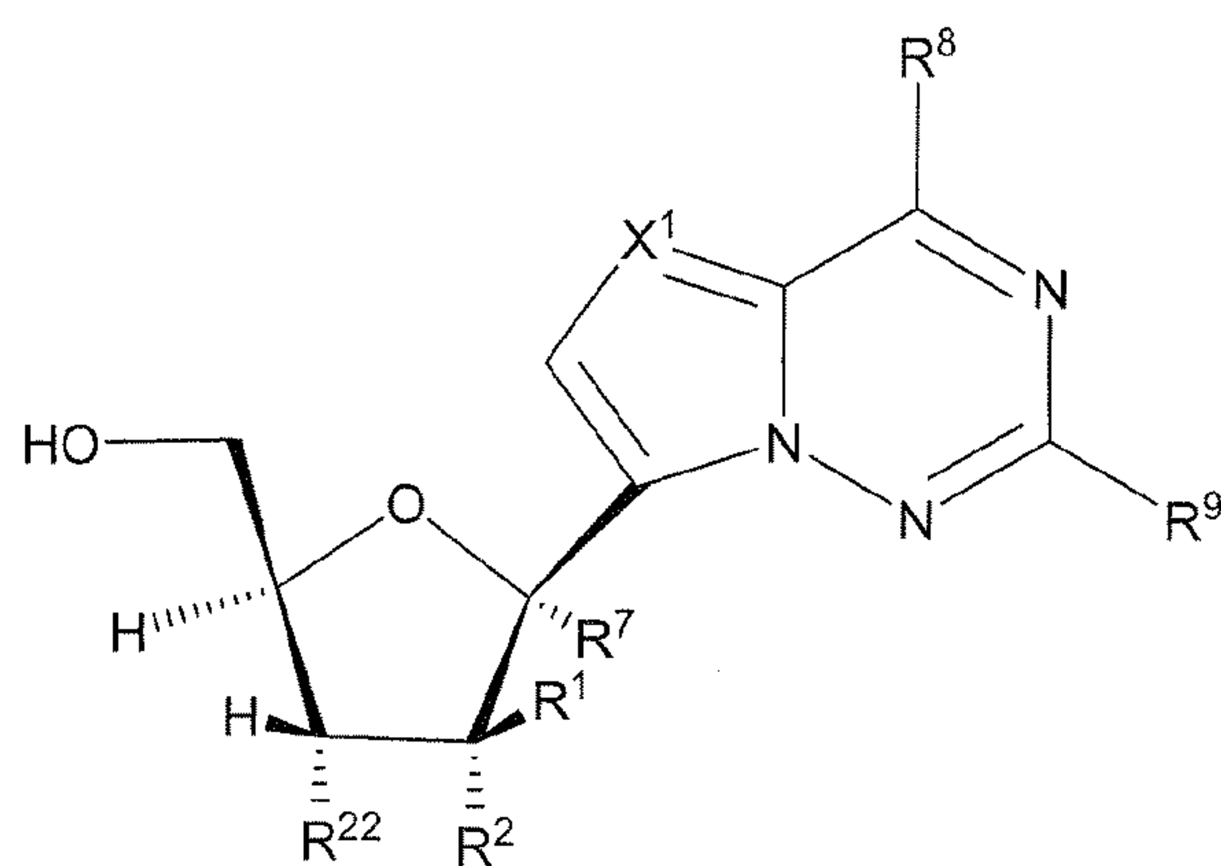
Formula VII
