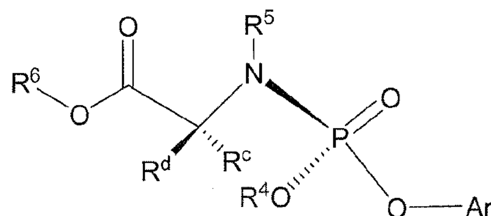
Formula IIIa
