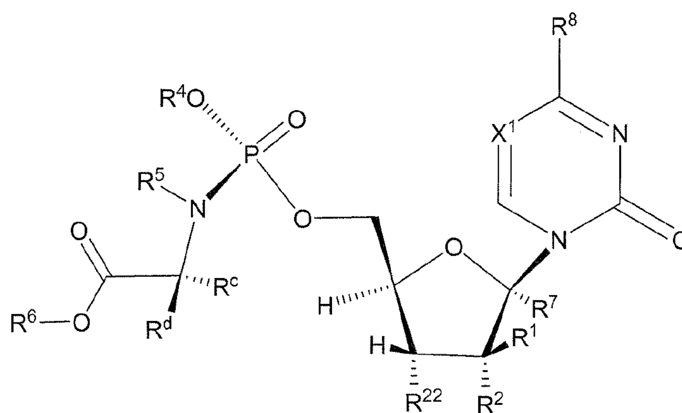
Formula XIIIb
