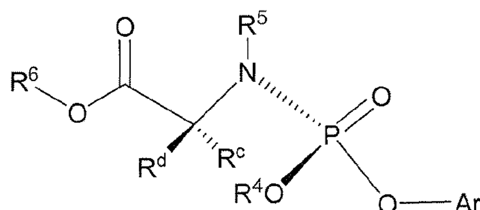
Formula IIIb
