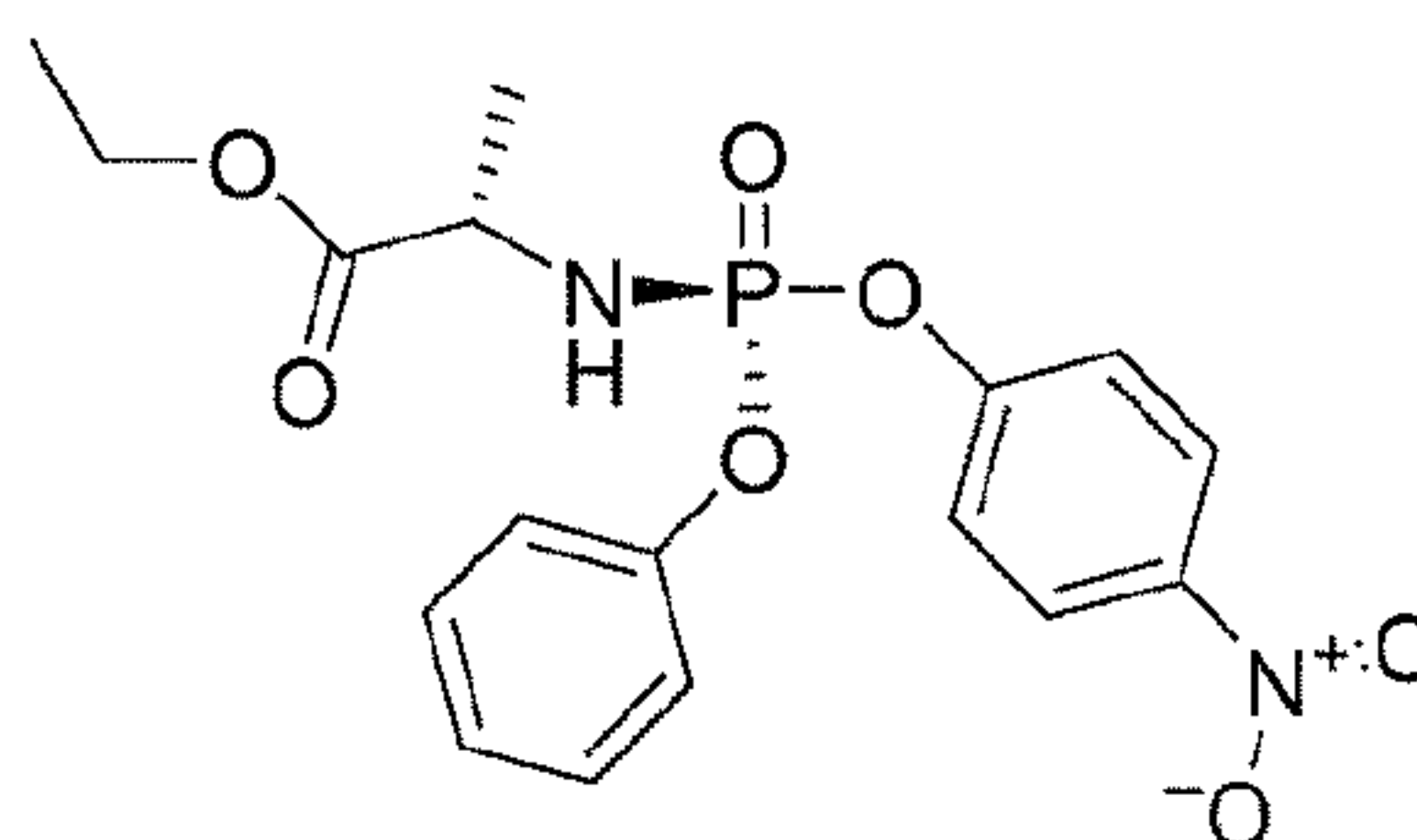
Compound 12
