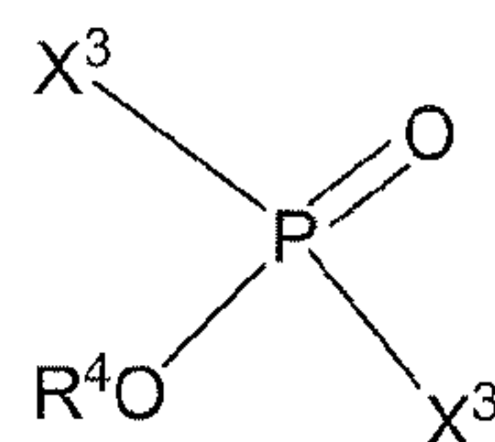
Formula X
