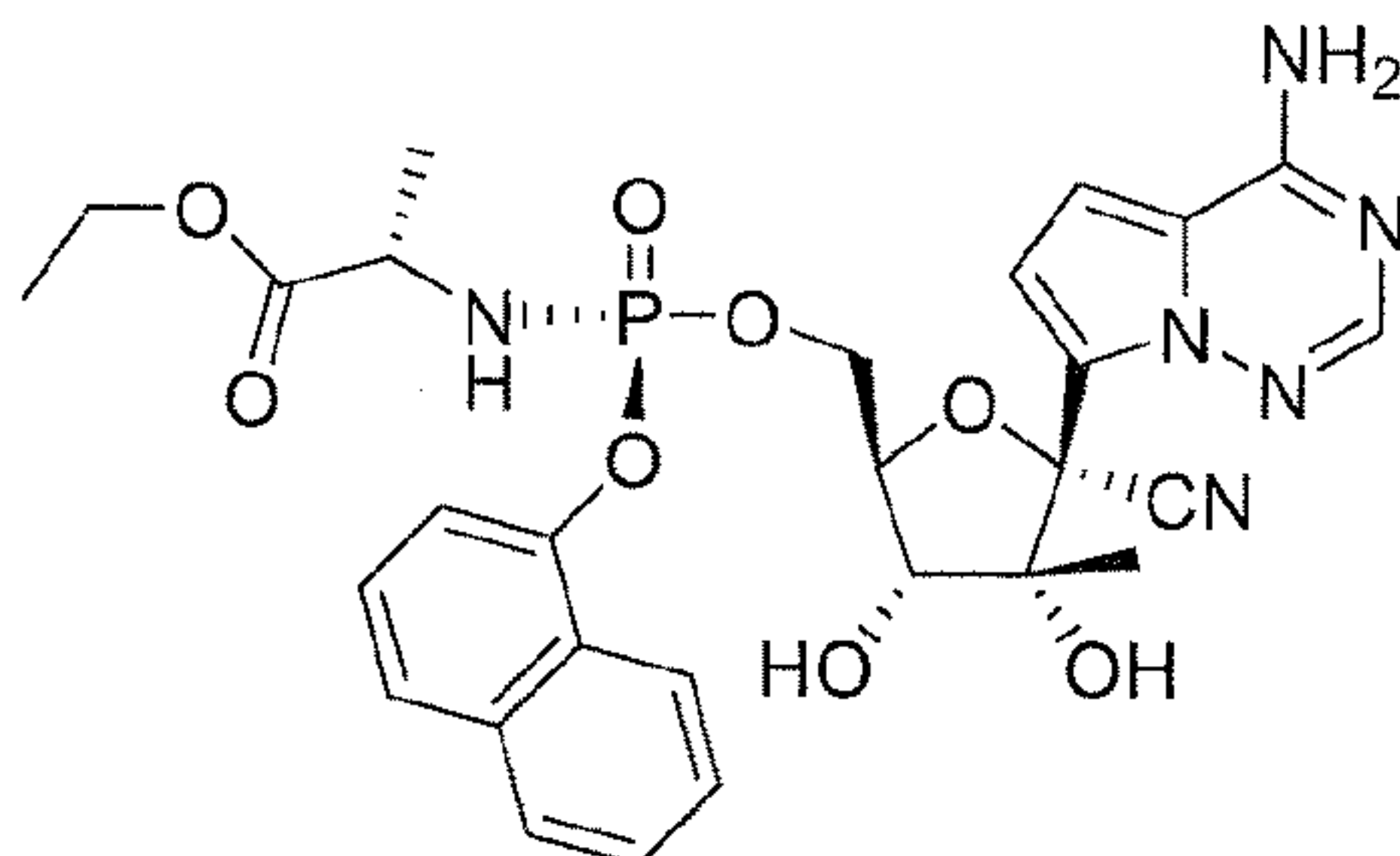
Compound 29
