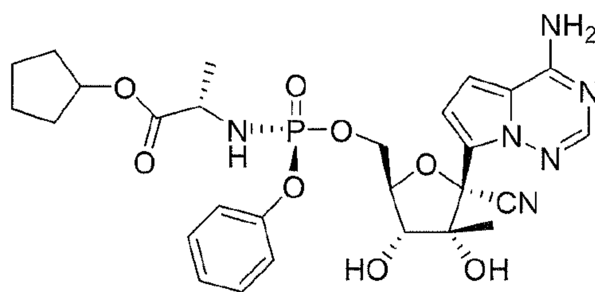
Compound 27
