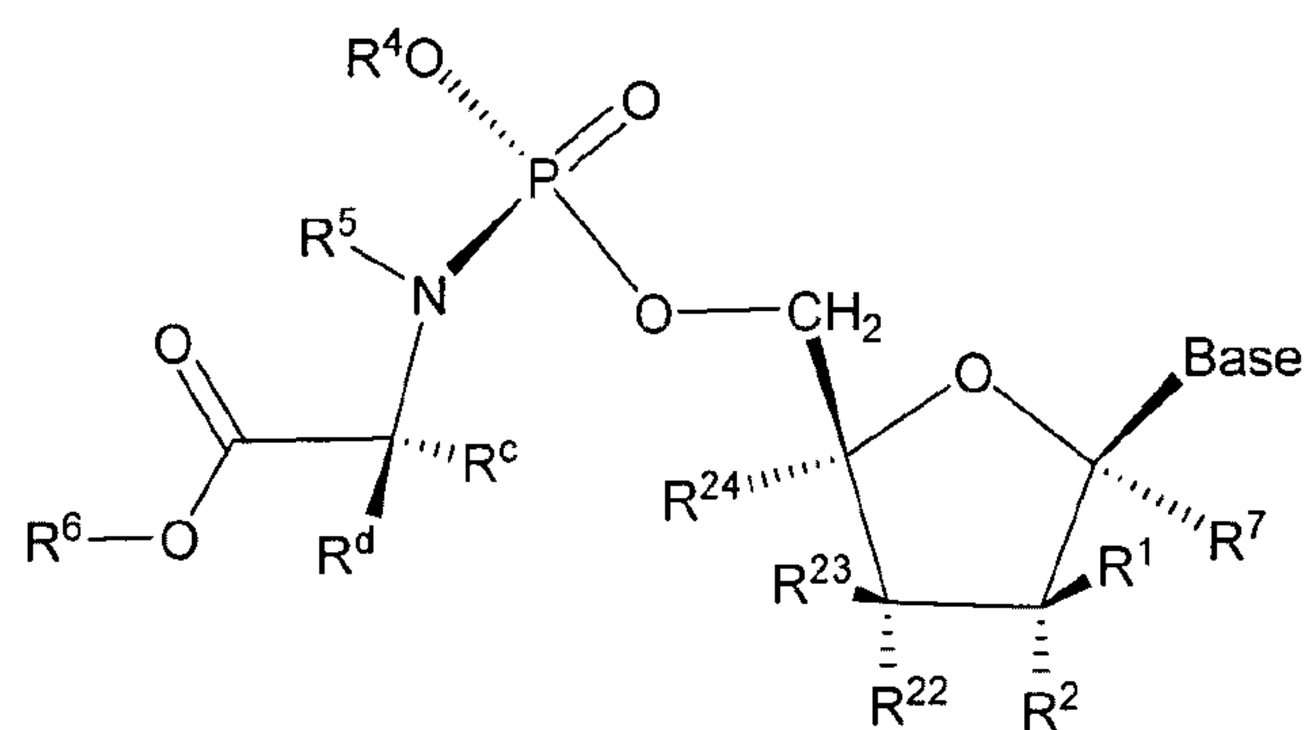
Formula IVb
