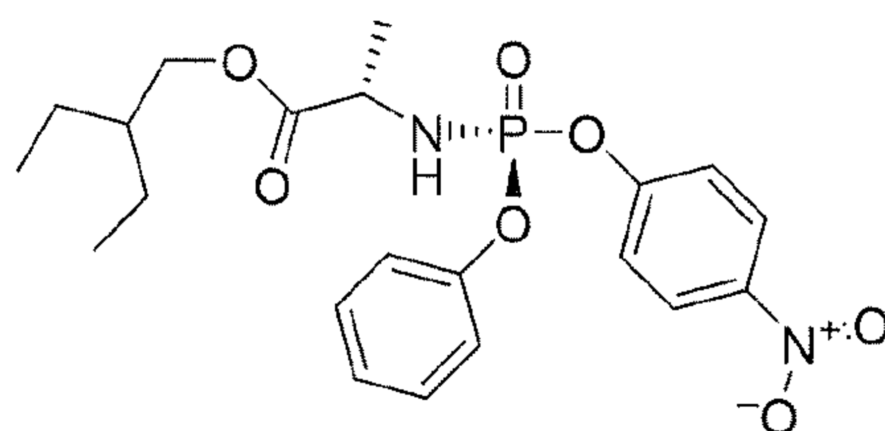
Compound 15
