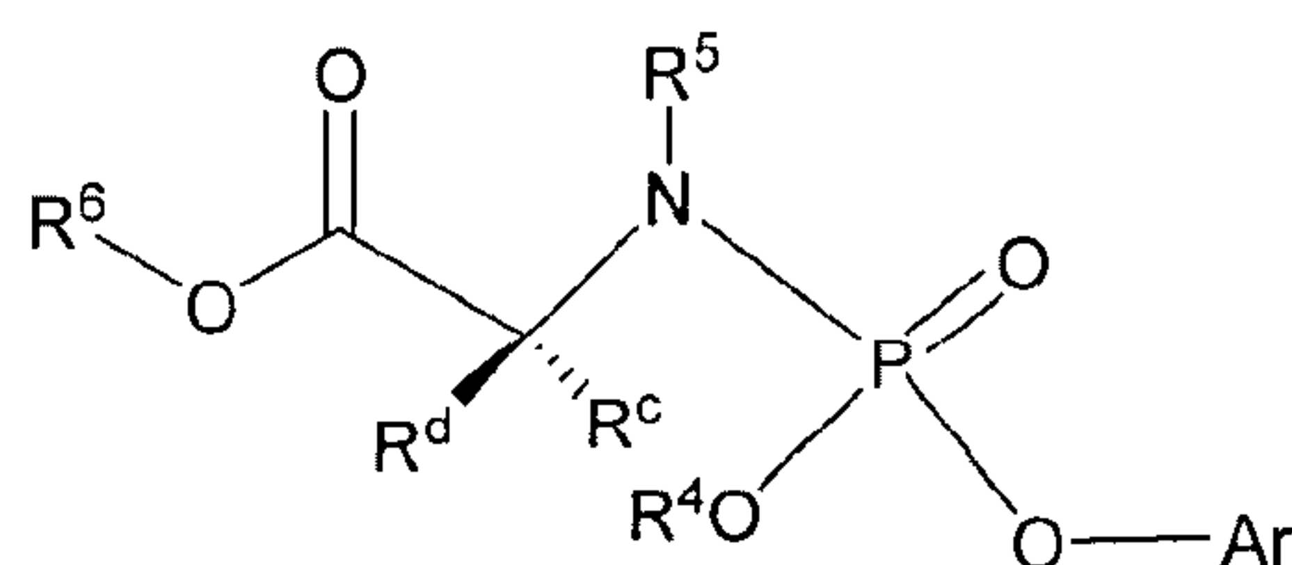
Formula VIII
