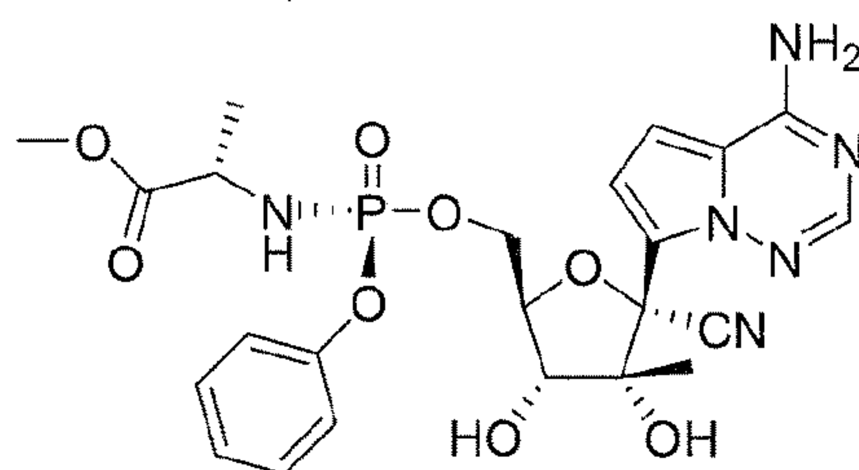
Compound 22
