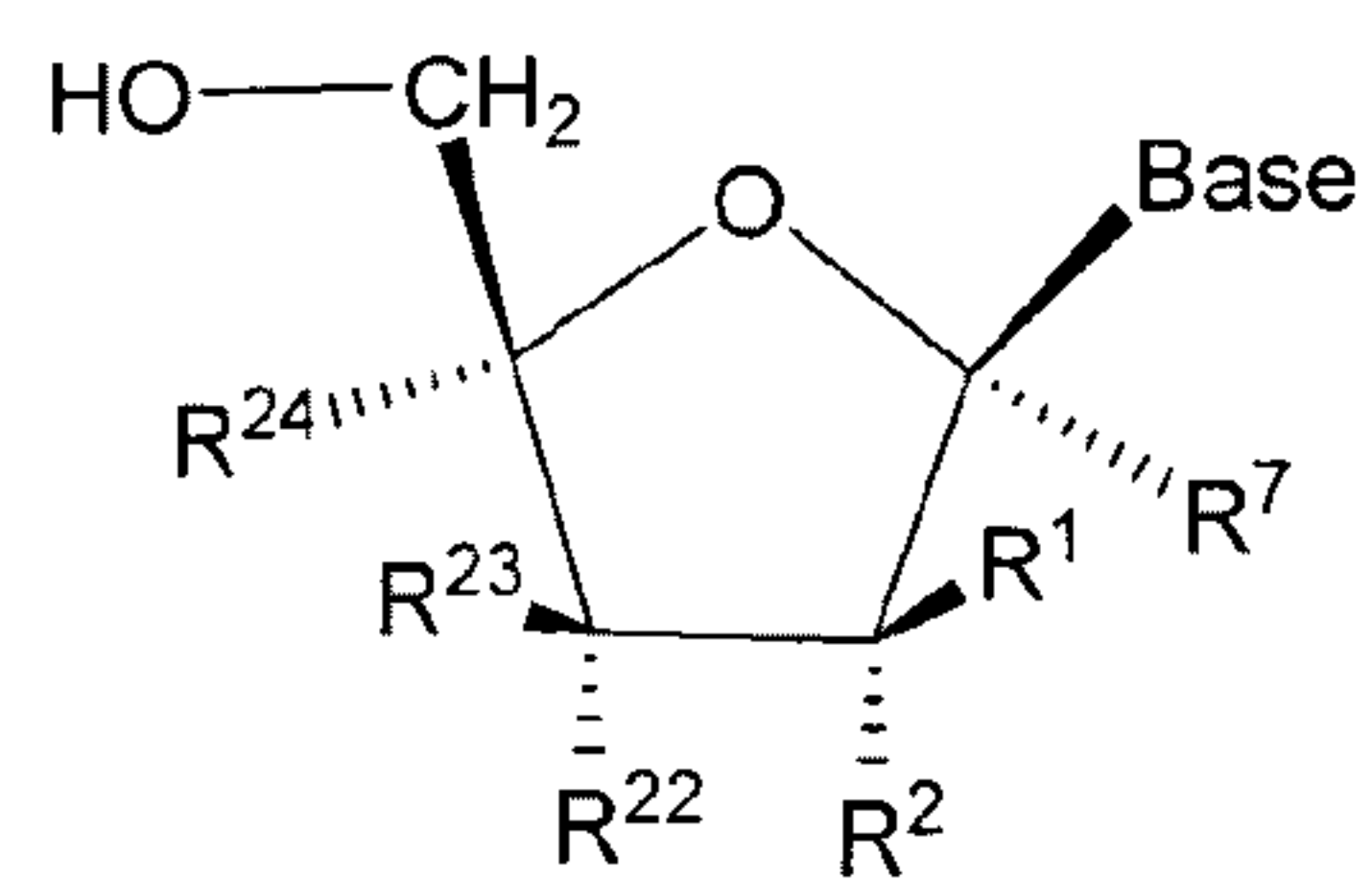
Formula V
