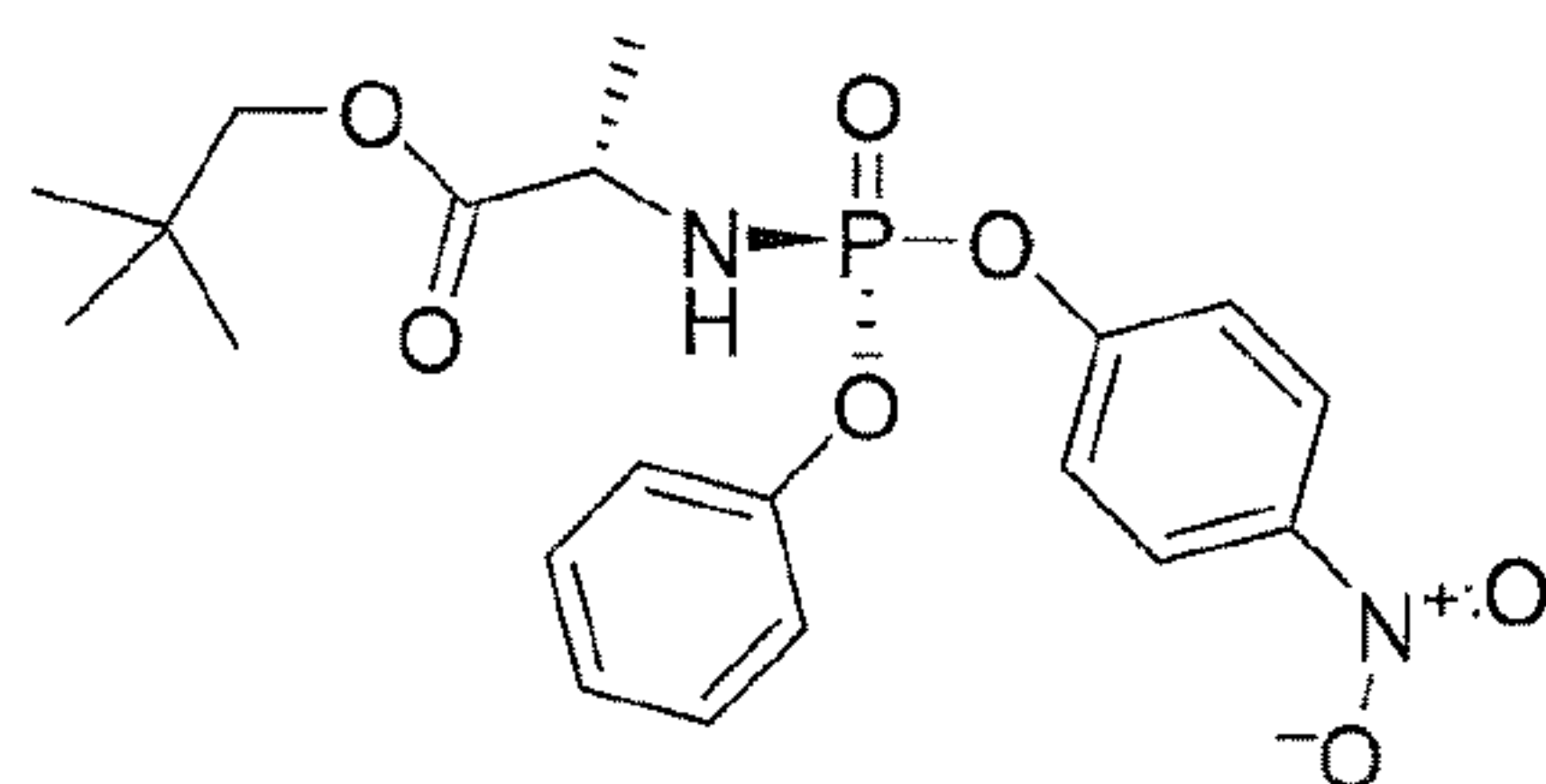
Compound 23
