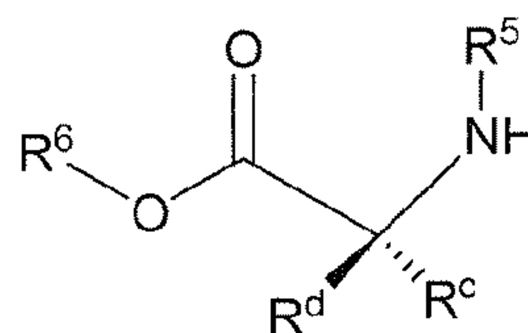
Formula IX
