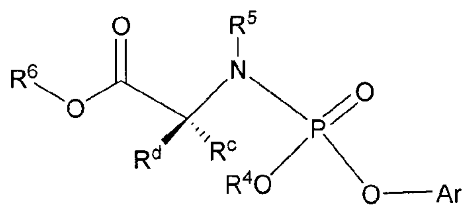
Formula VIII
