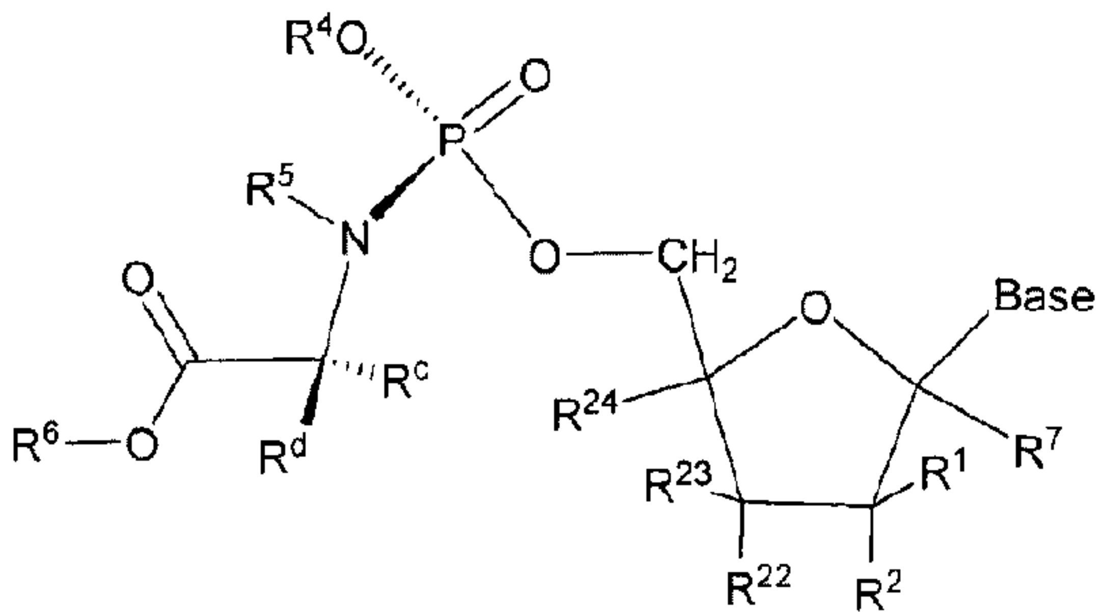
Formula Ib
