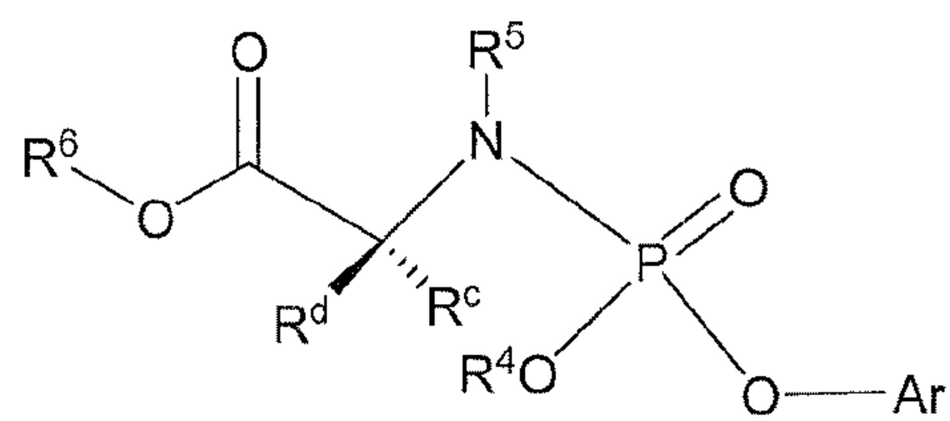
Formula VIII
