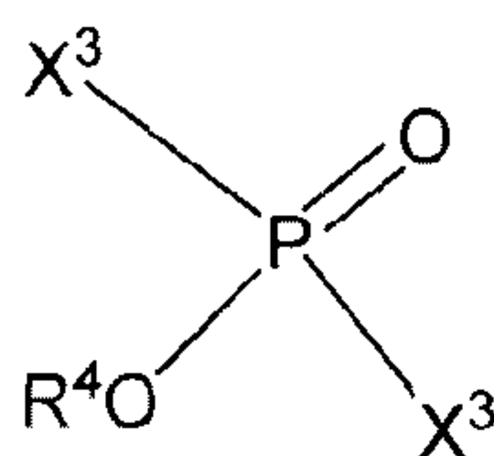
Formula X
