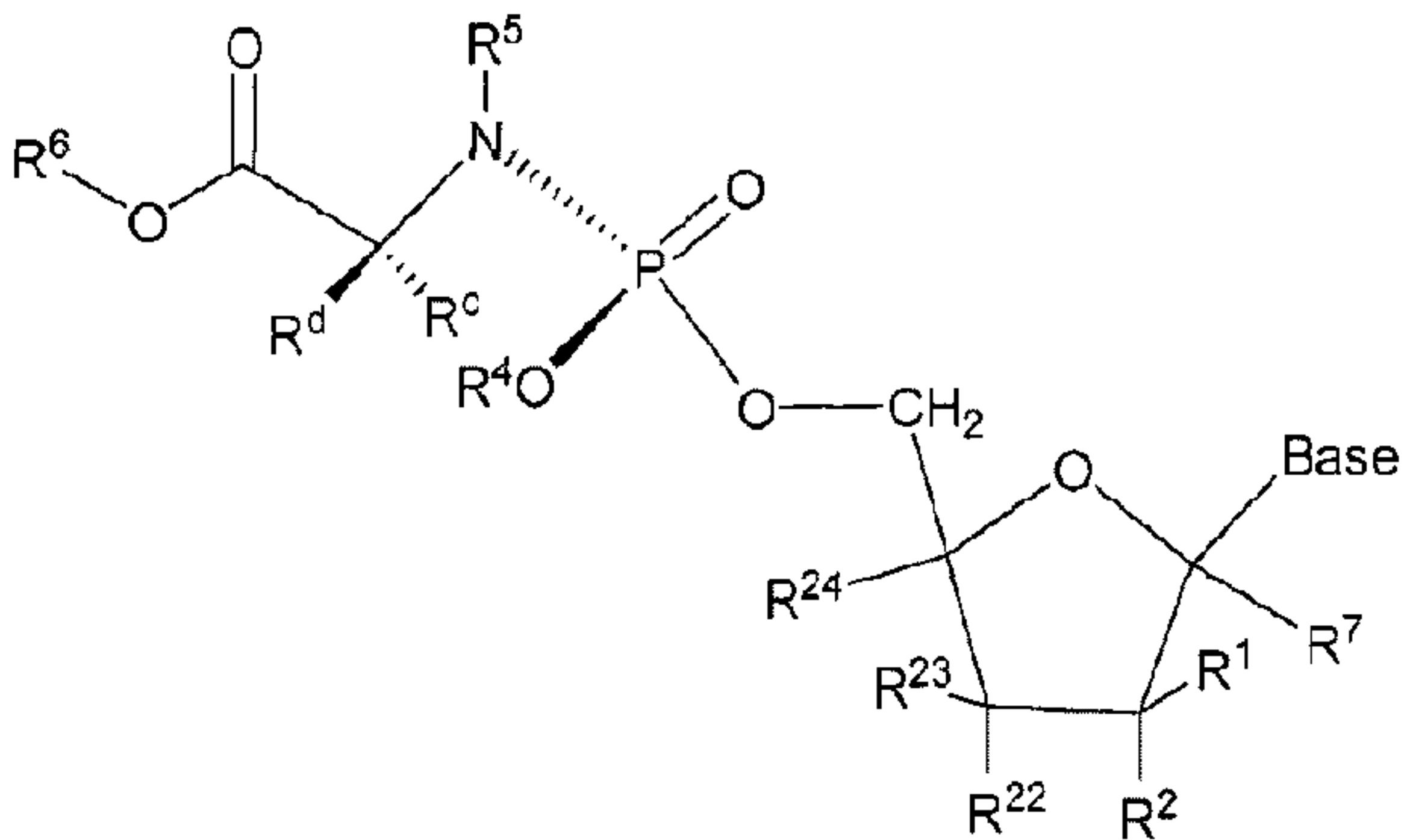
Formula Ia
