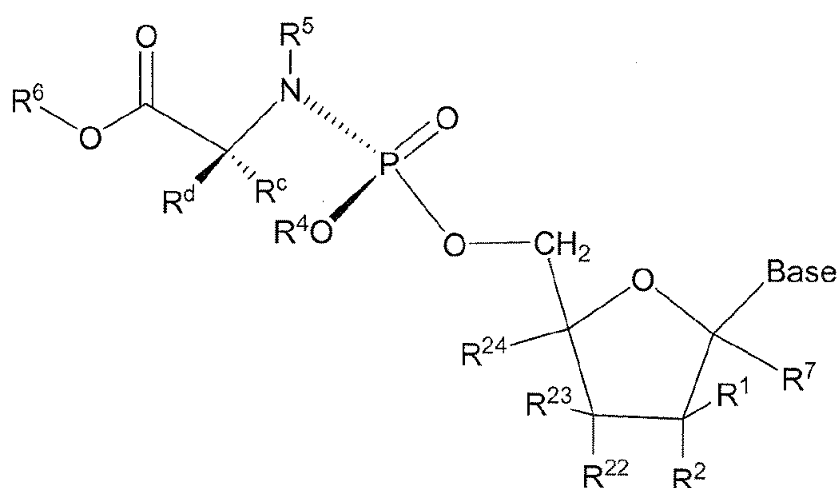
Formula Ia
