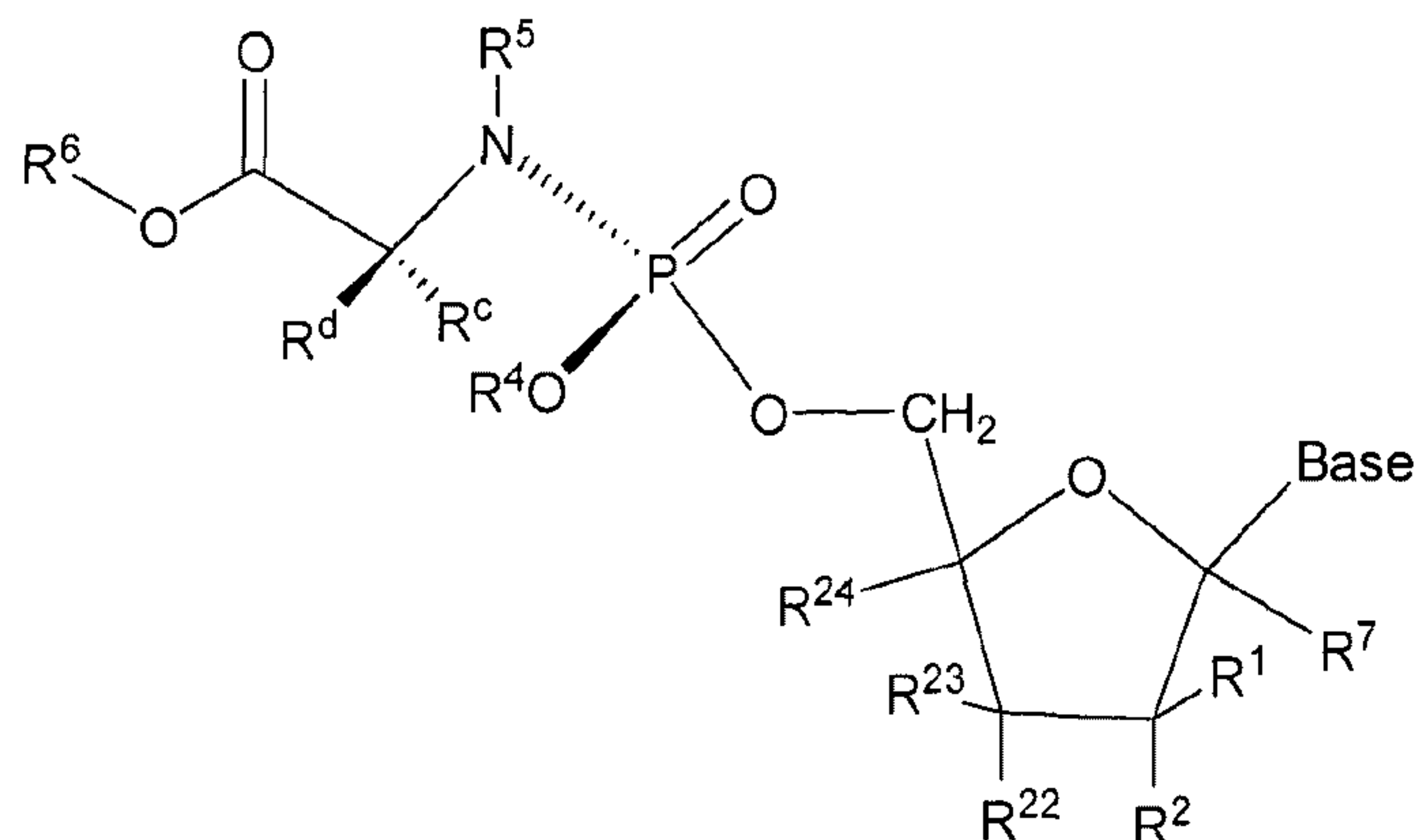
Formula Ia
