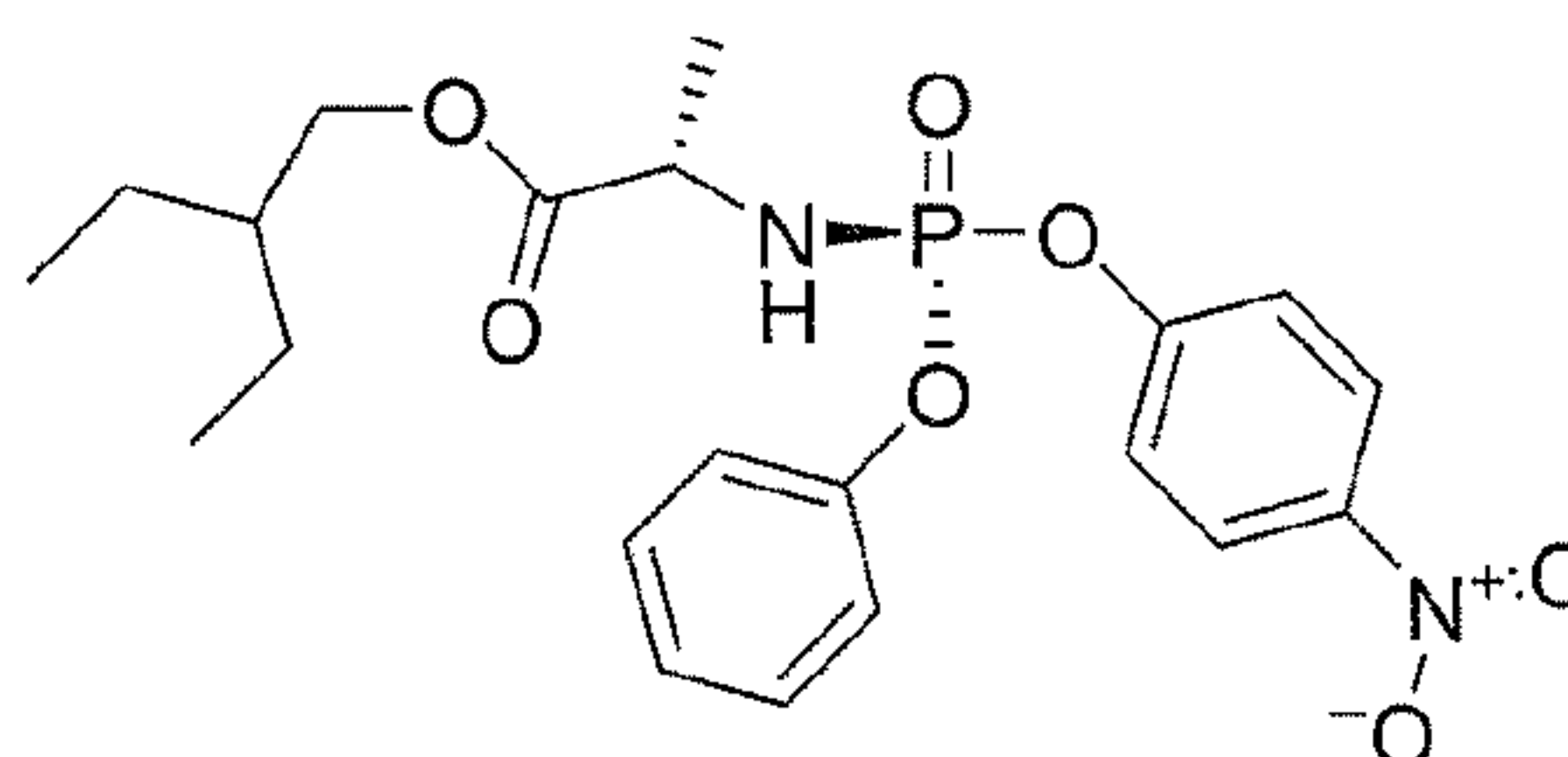
Compound 13
