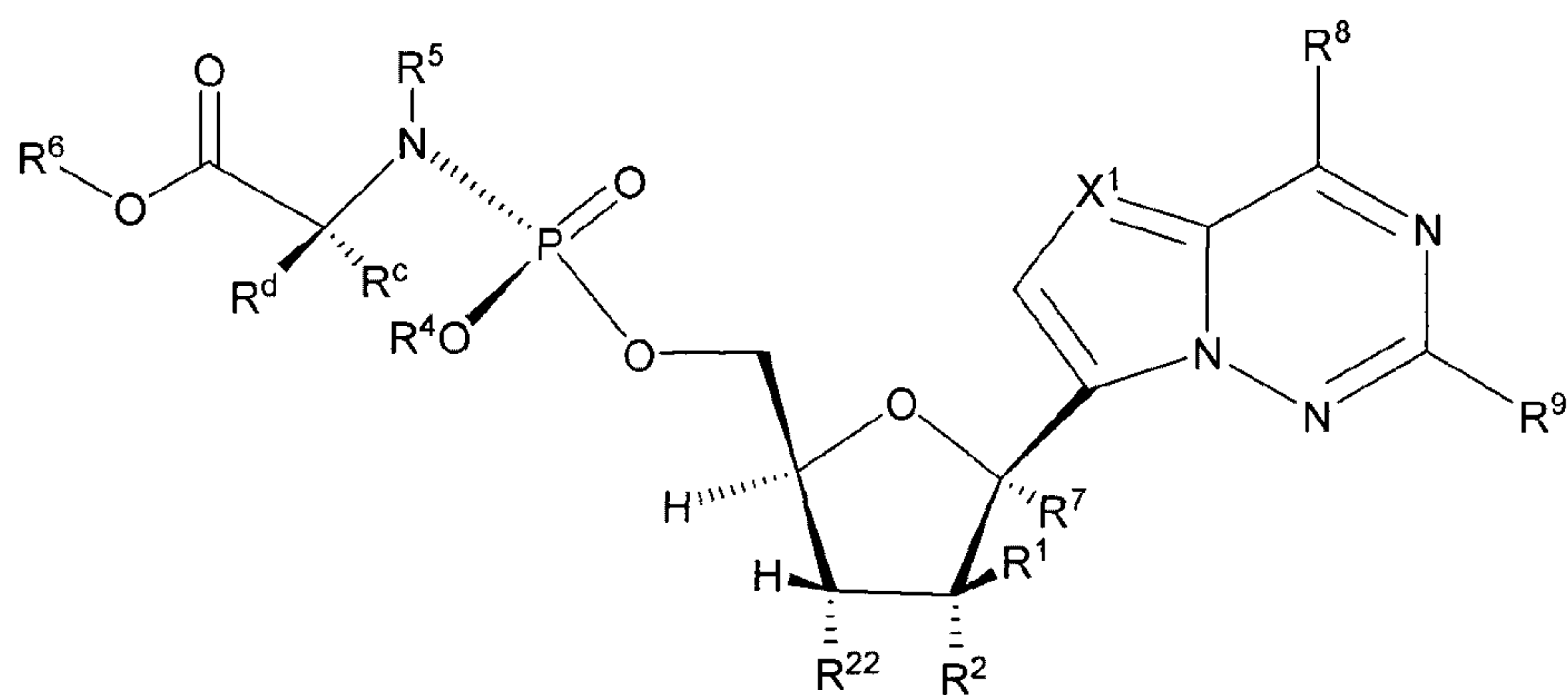
Formula VIa
