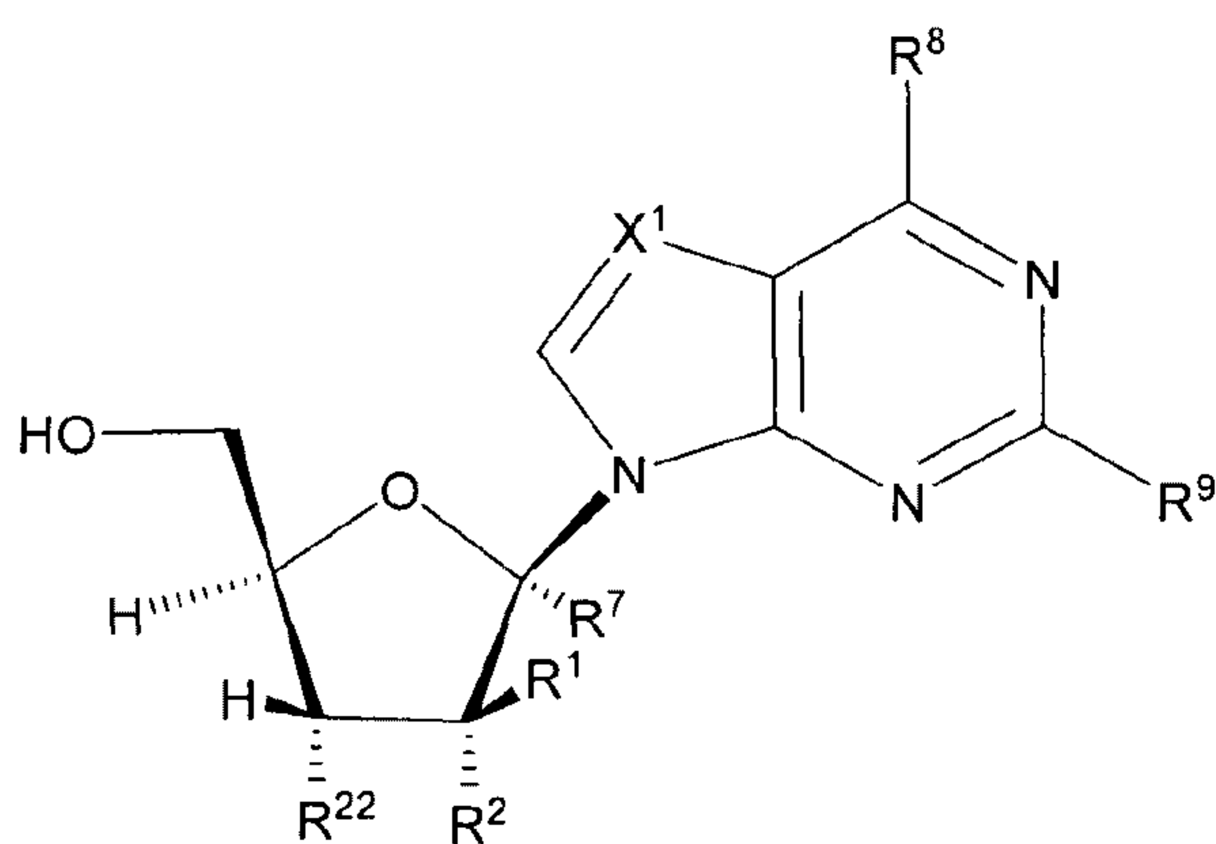
Formula XII
