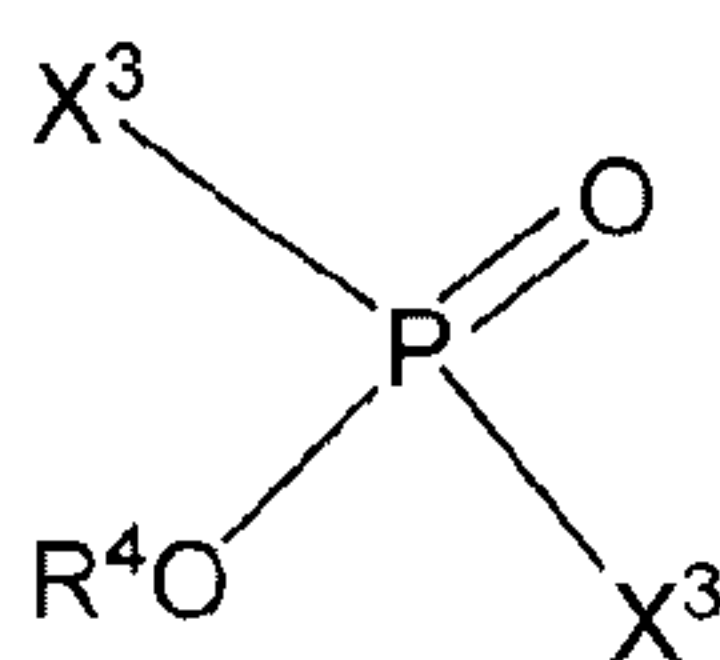
Formula X
