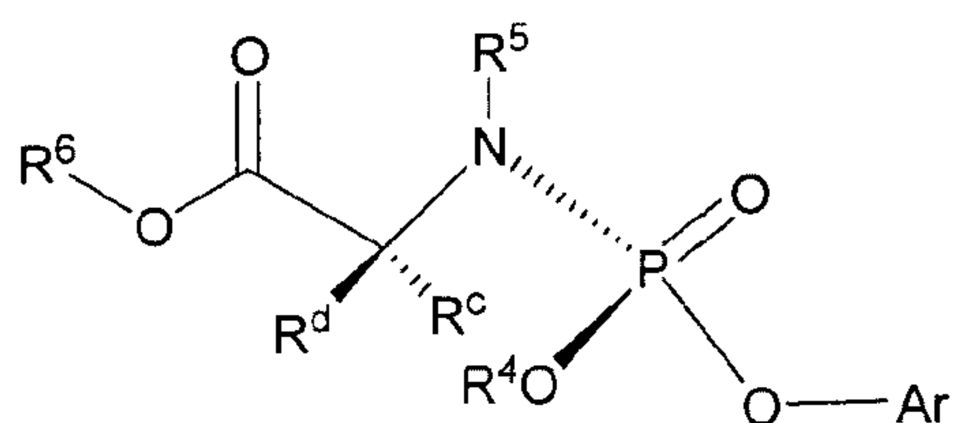
Formula IIIb
