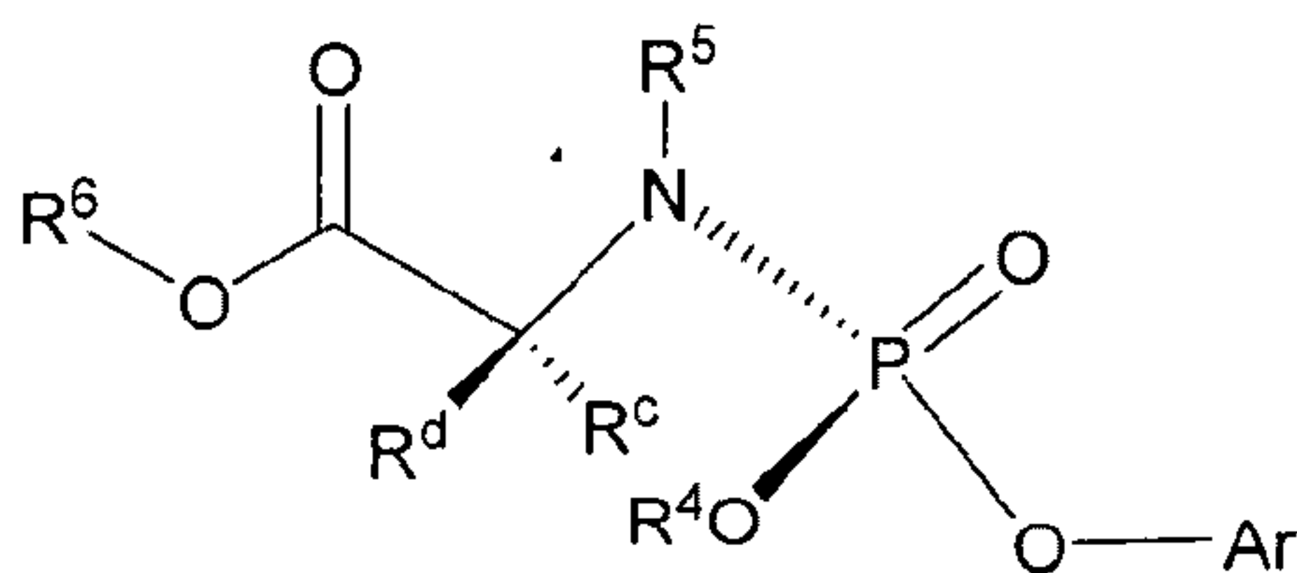
Formula IIIb
