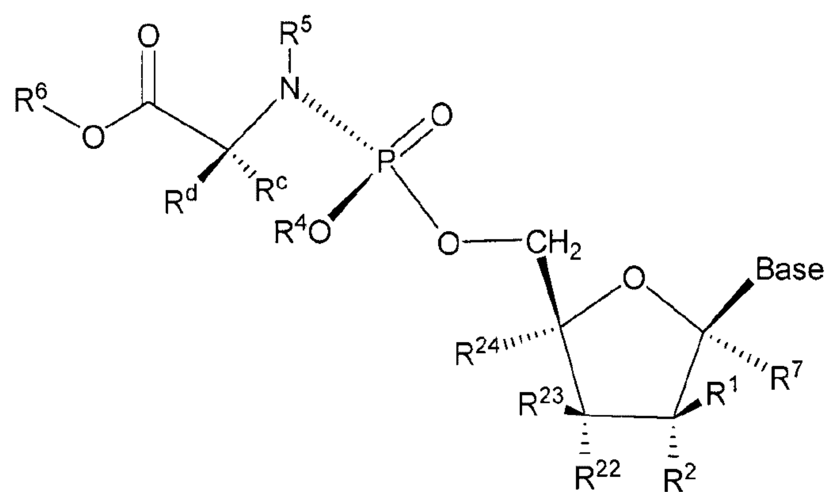
Formula IVa
