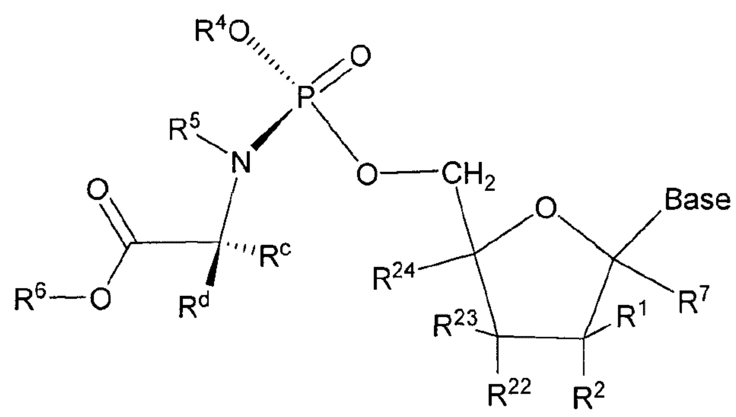
Formula Ib
