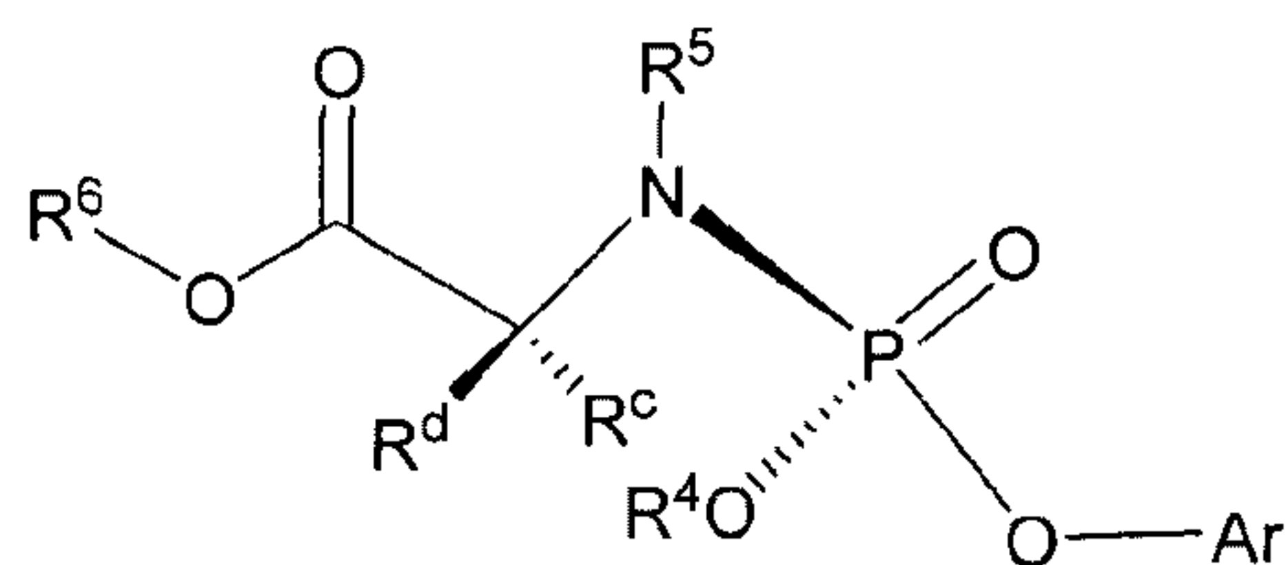
Formula IIIa
