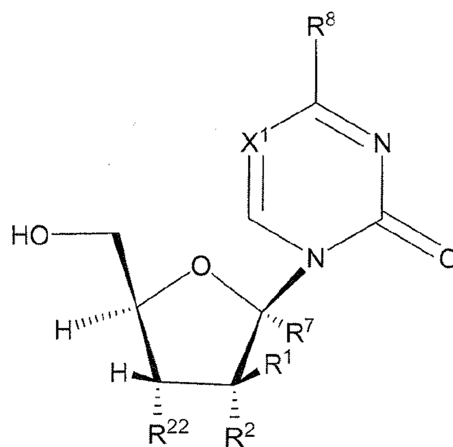
Formula XIV
