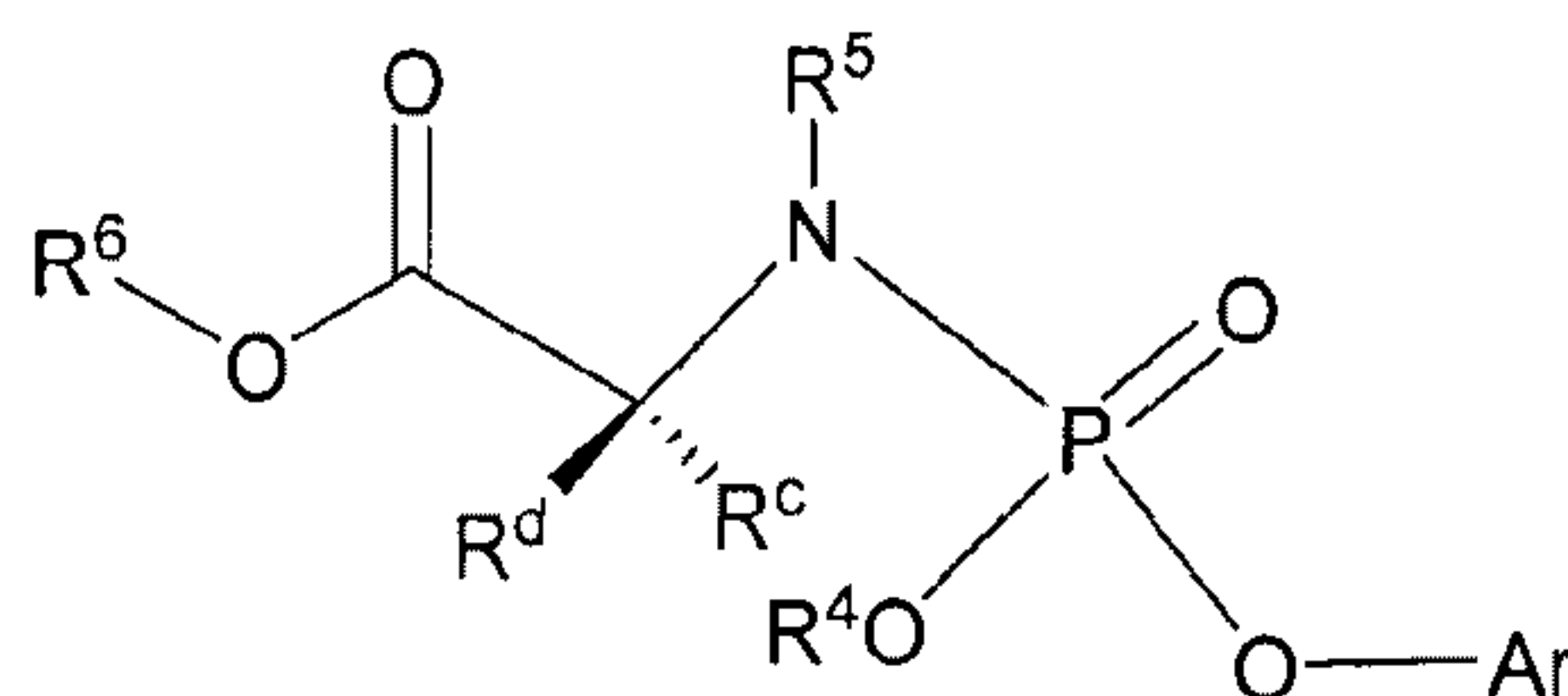
Formula VIII
