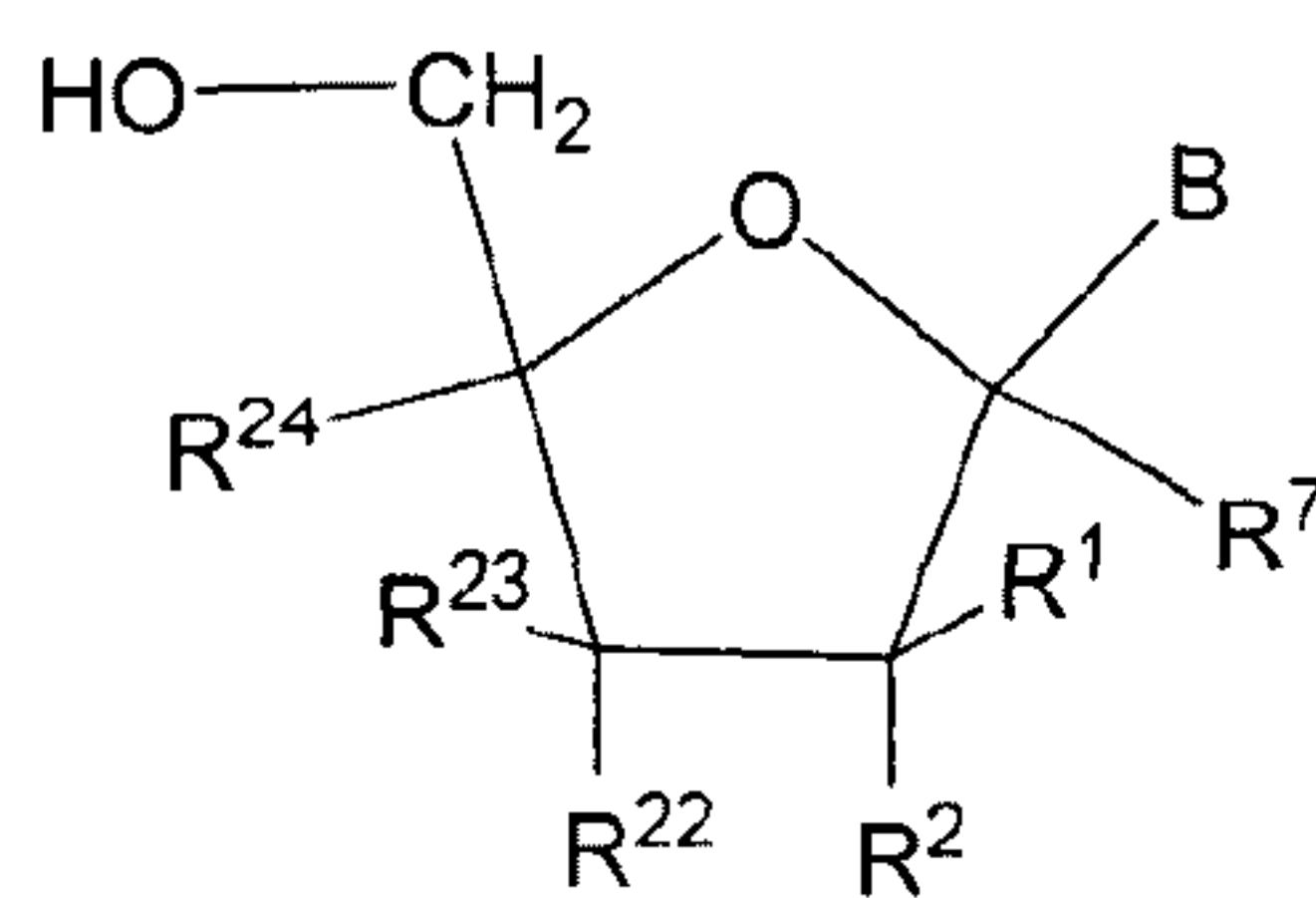
Formula II
