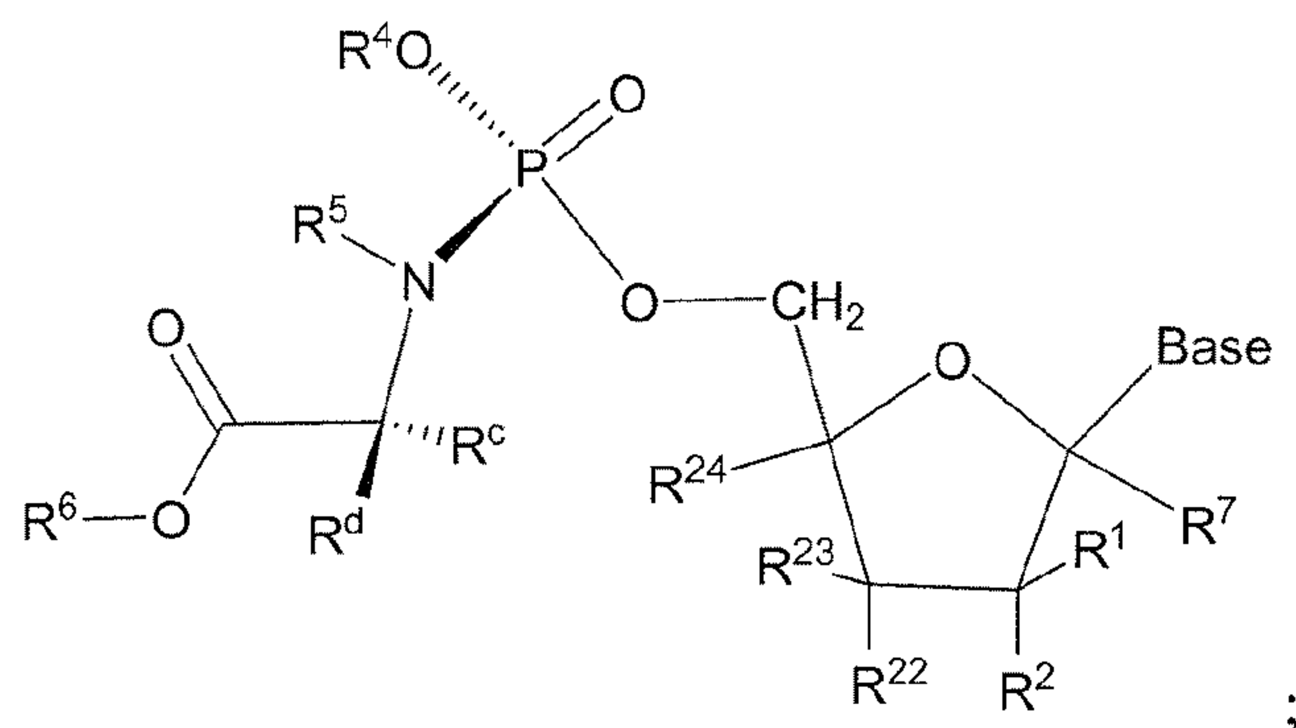
Formula Ib
