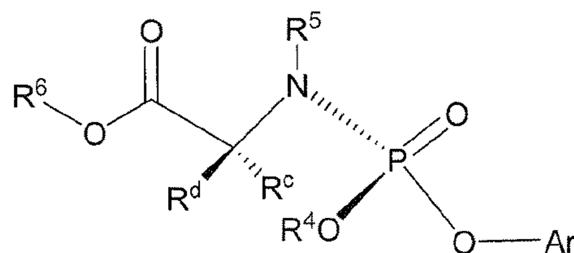
Formula IIIb
