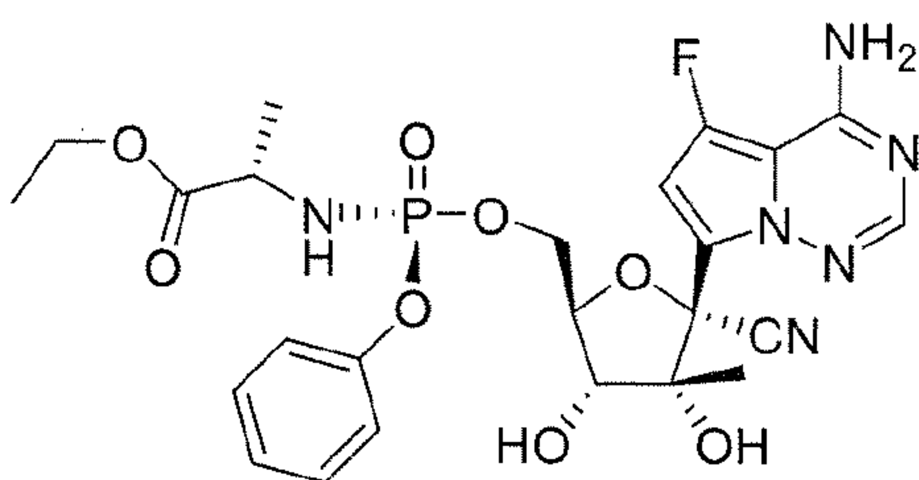
Compound 30
