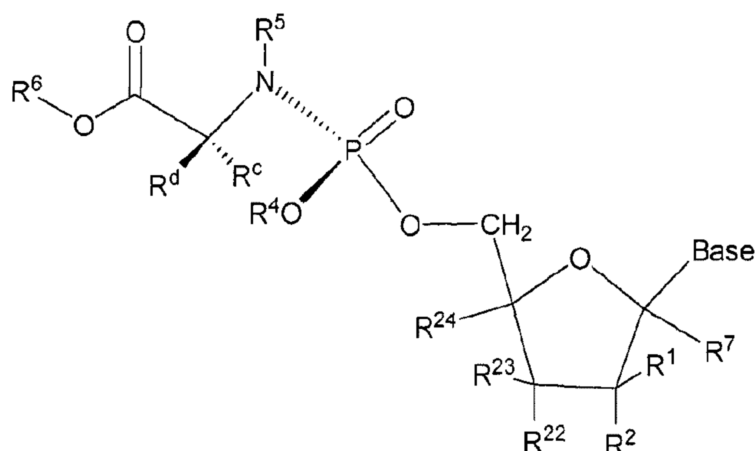
Formula Ia
