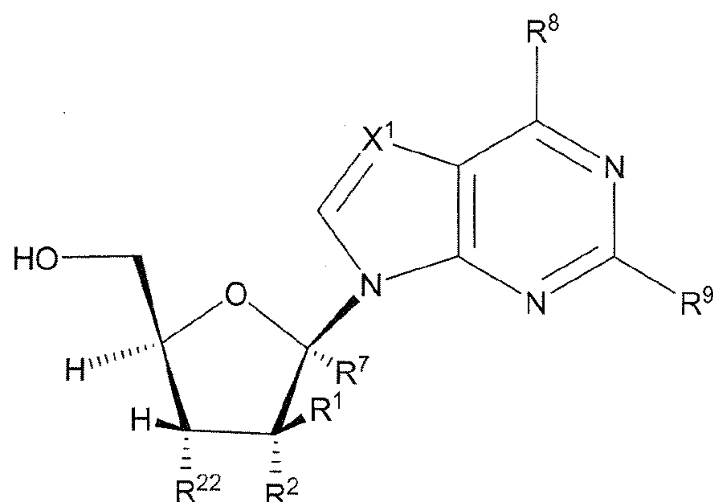
Formula XII
