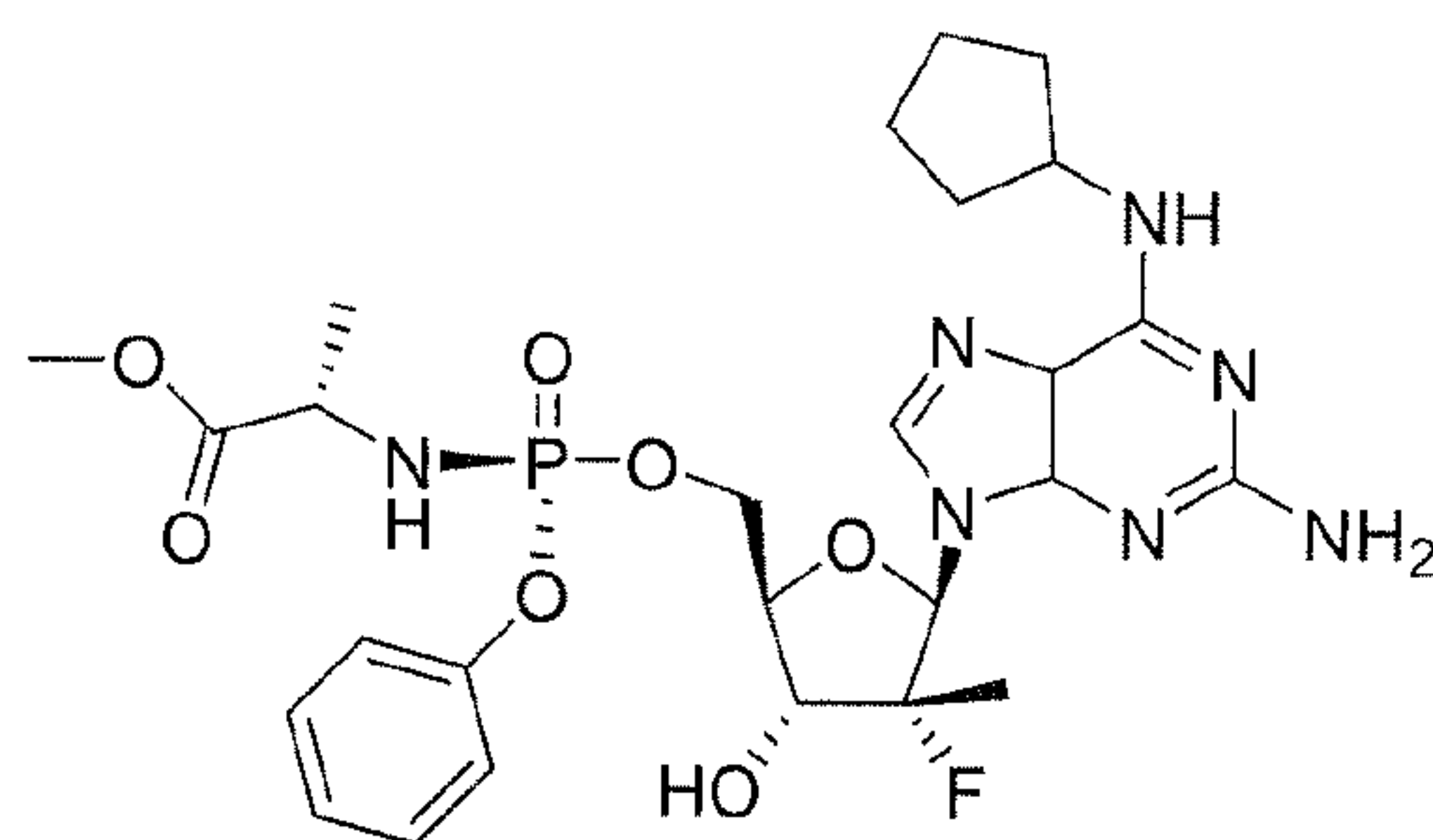
Compound 38
