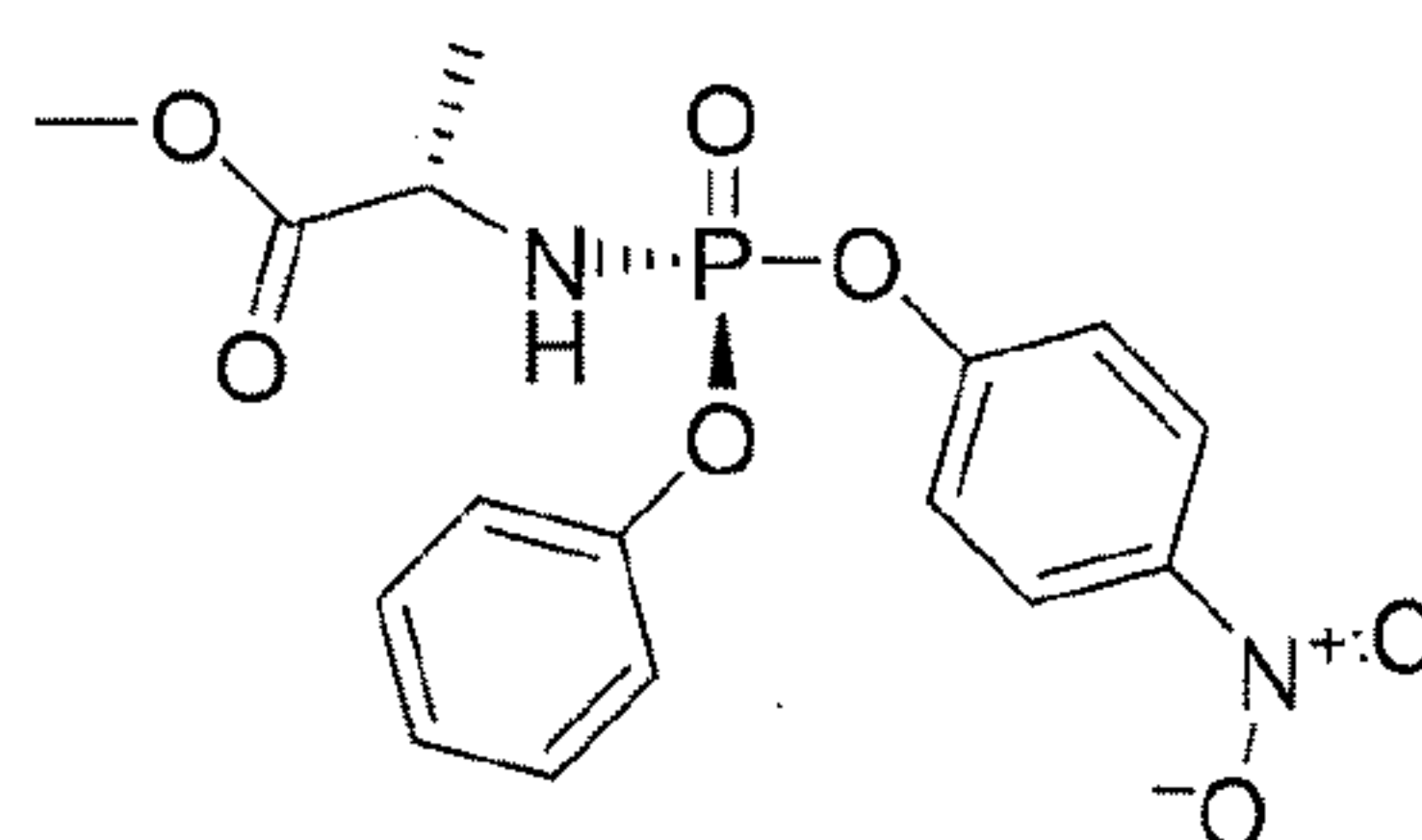
Compound 11
