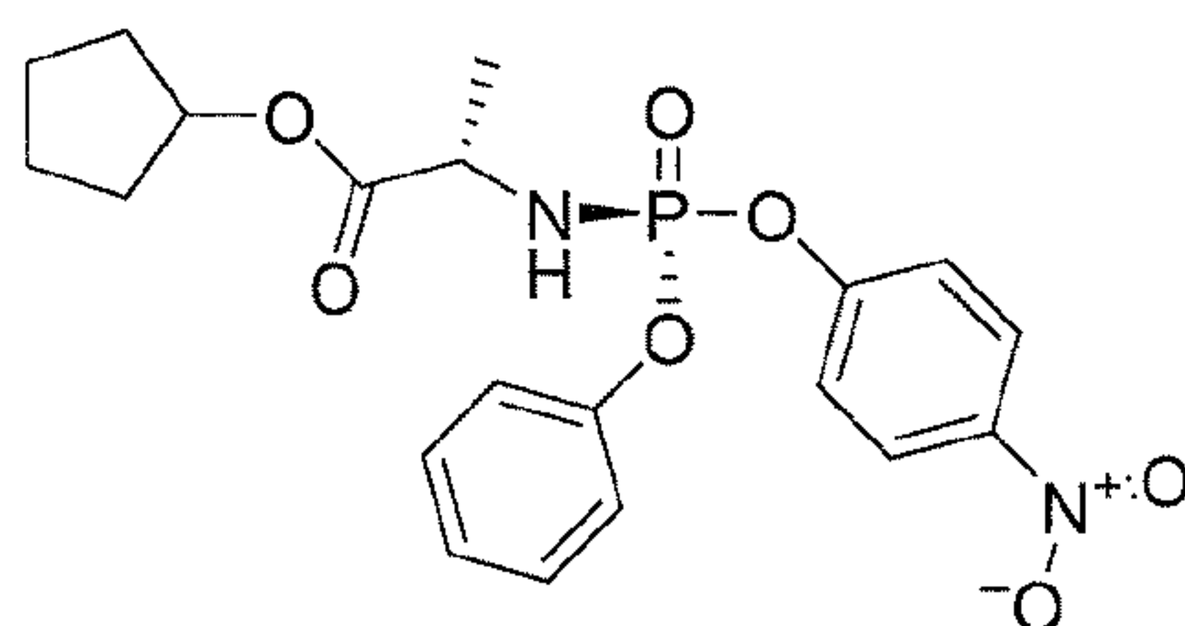
Compound 16
