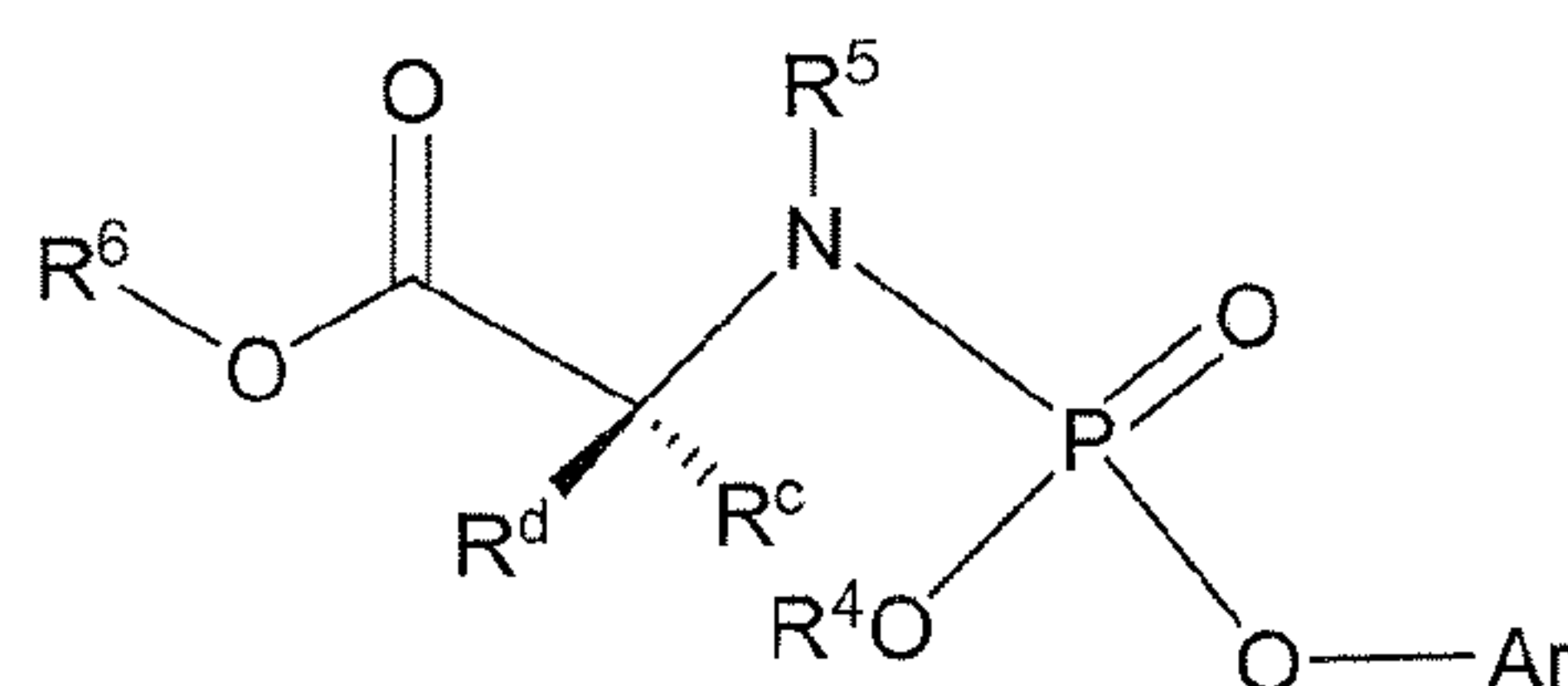
Formula VIII
