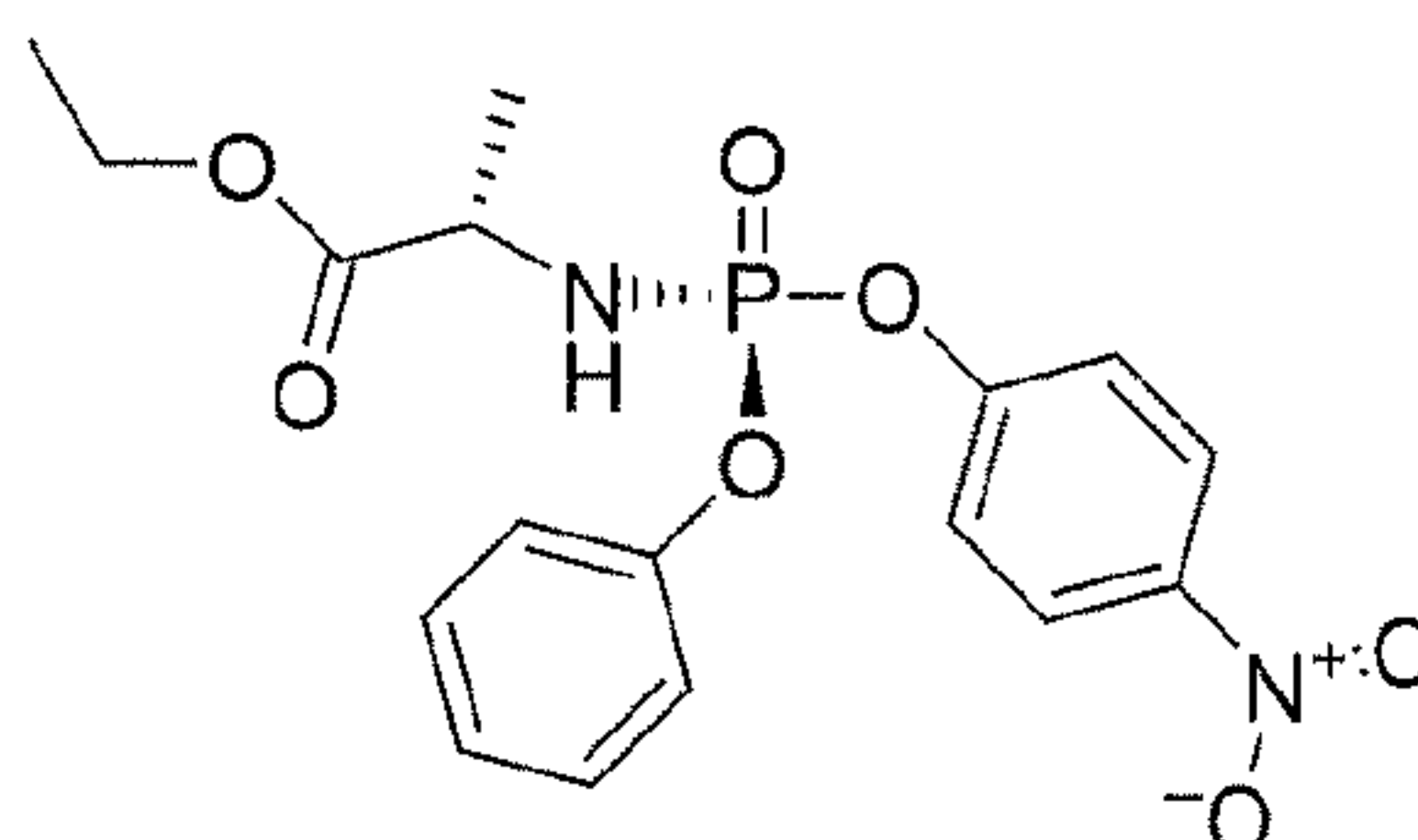
Compound 13
