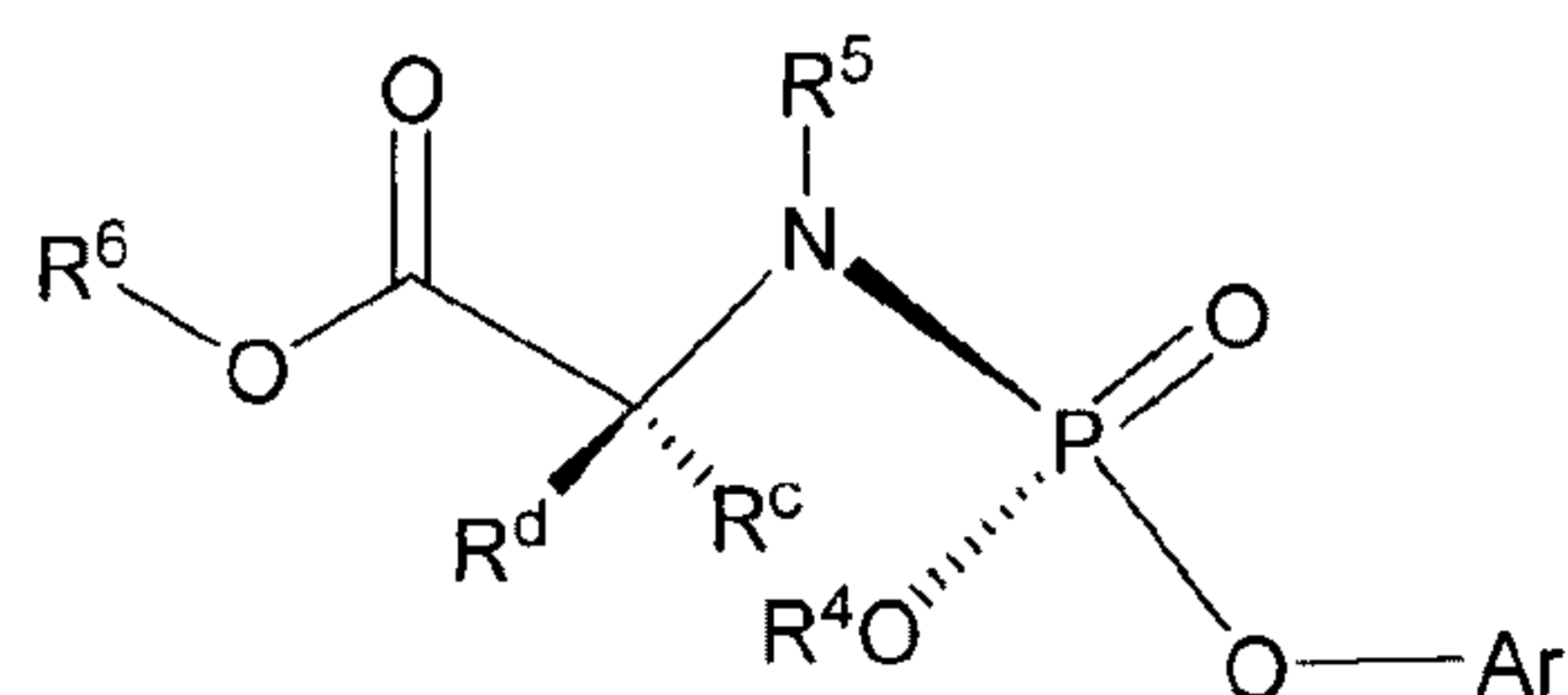
Formula IIIa
