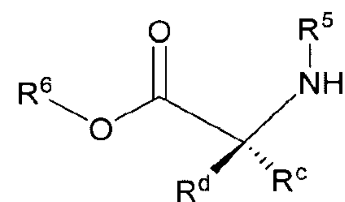
Formula IX
