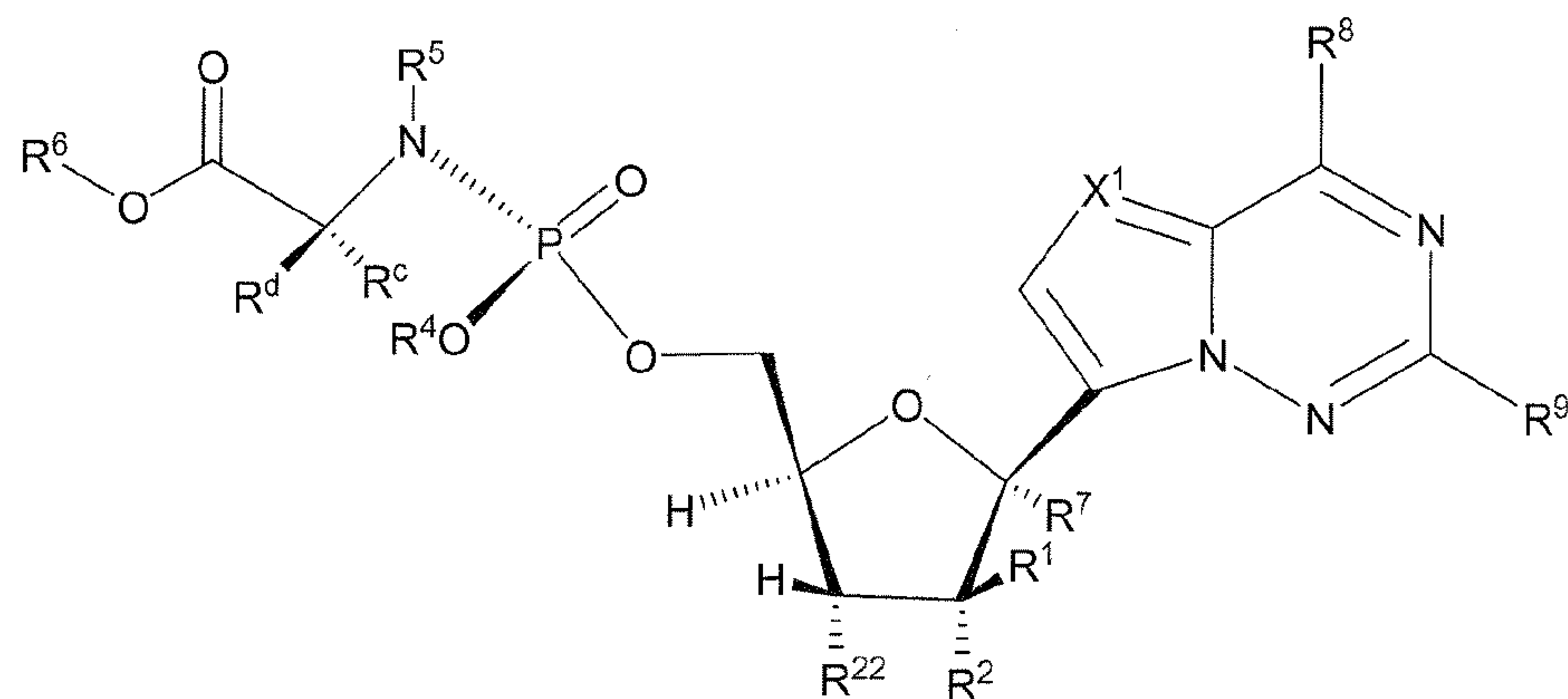
Formula VIa
