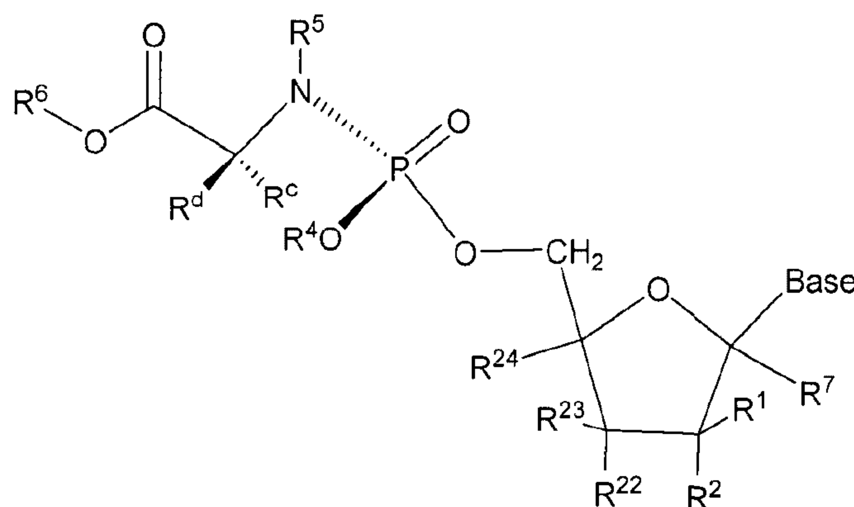
Formula Ia
