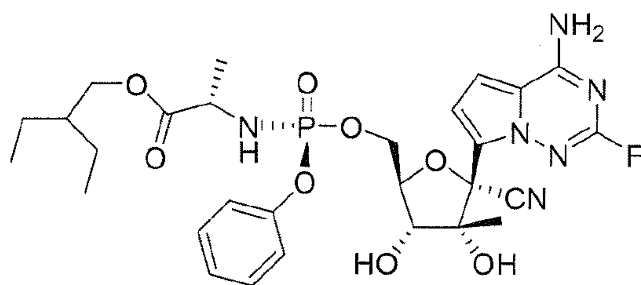
Compound 32
