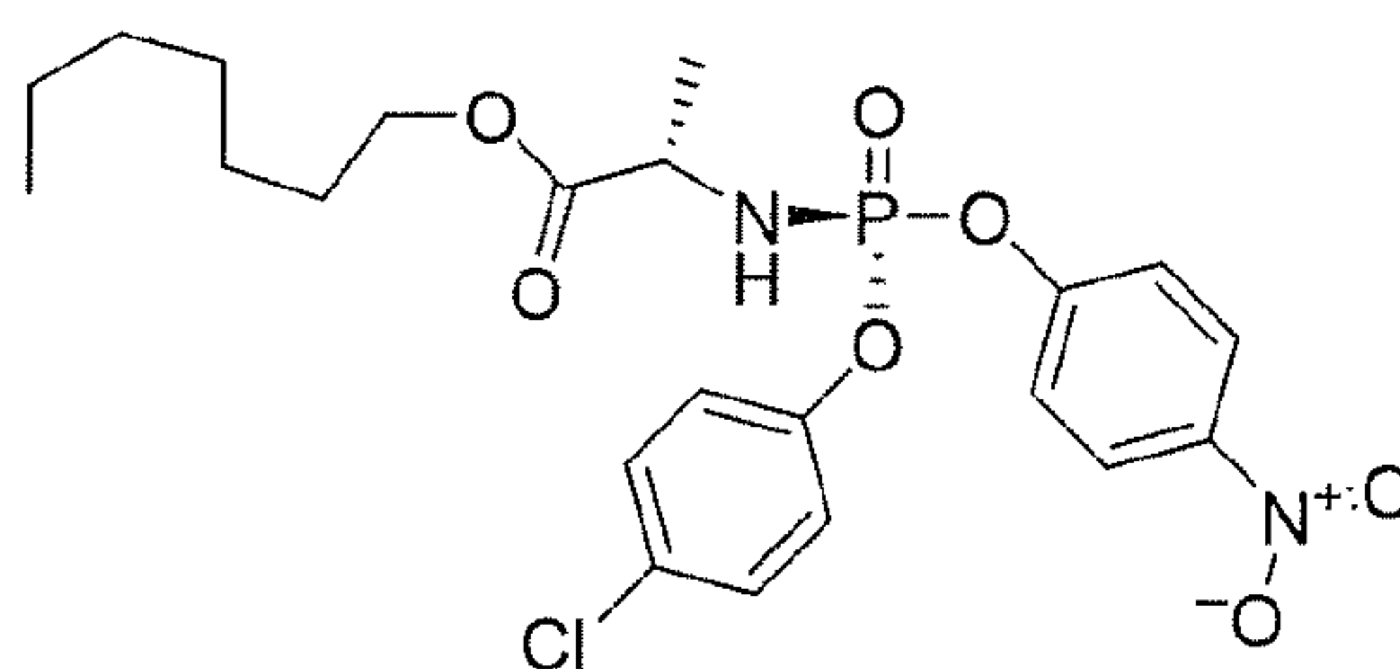
Compound 18
