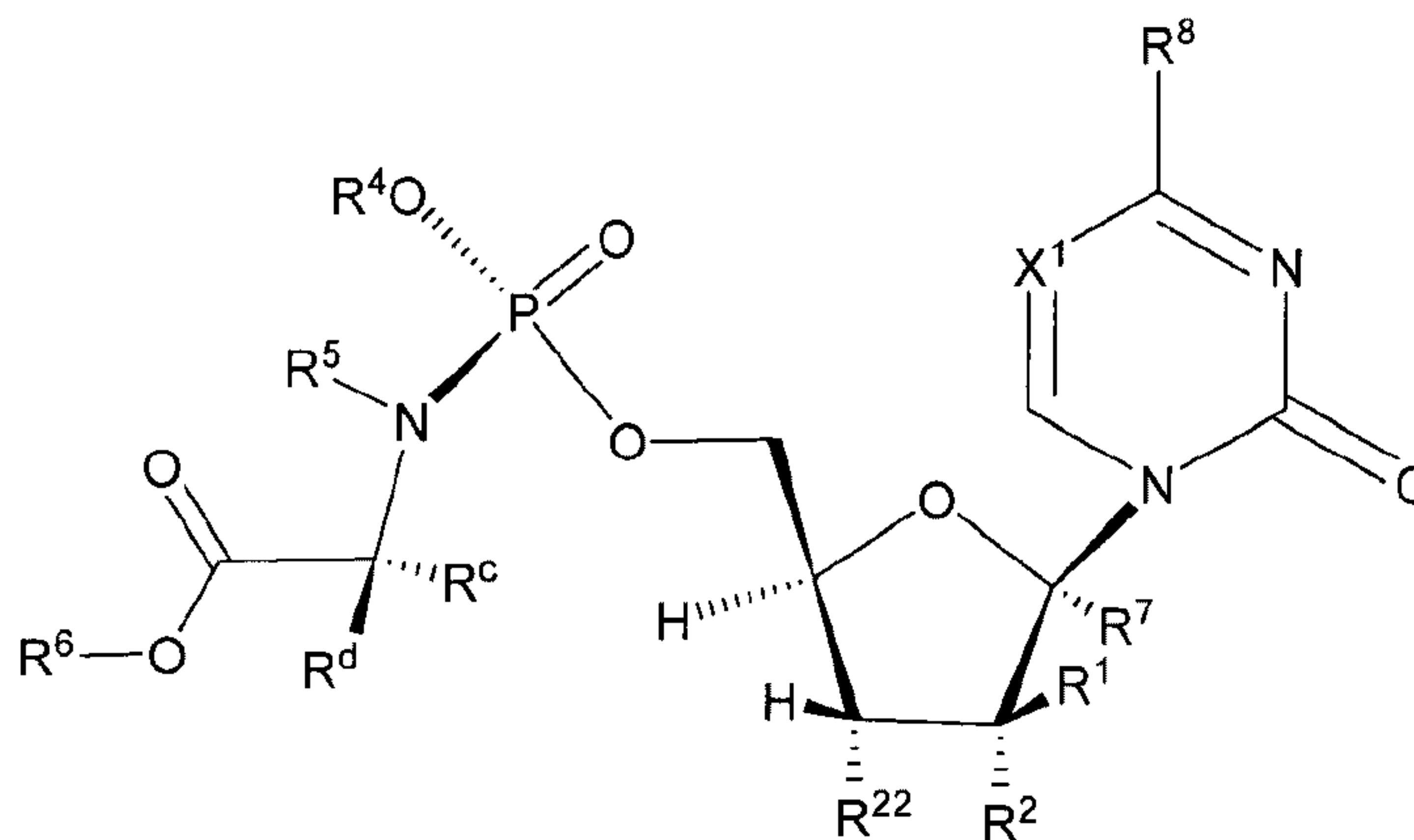
Formula XIIIb
