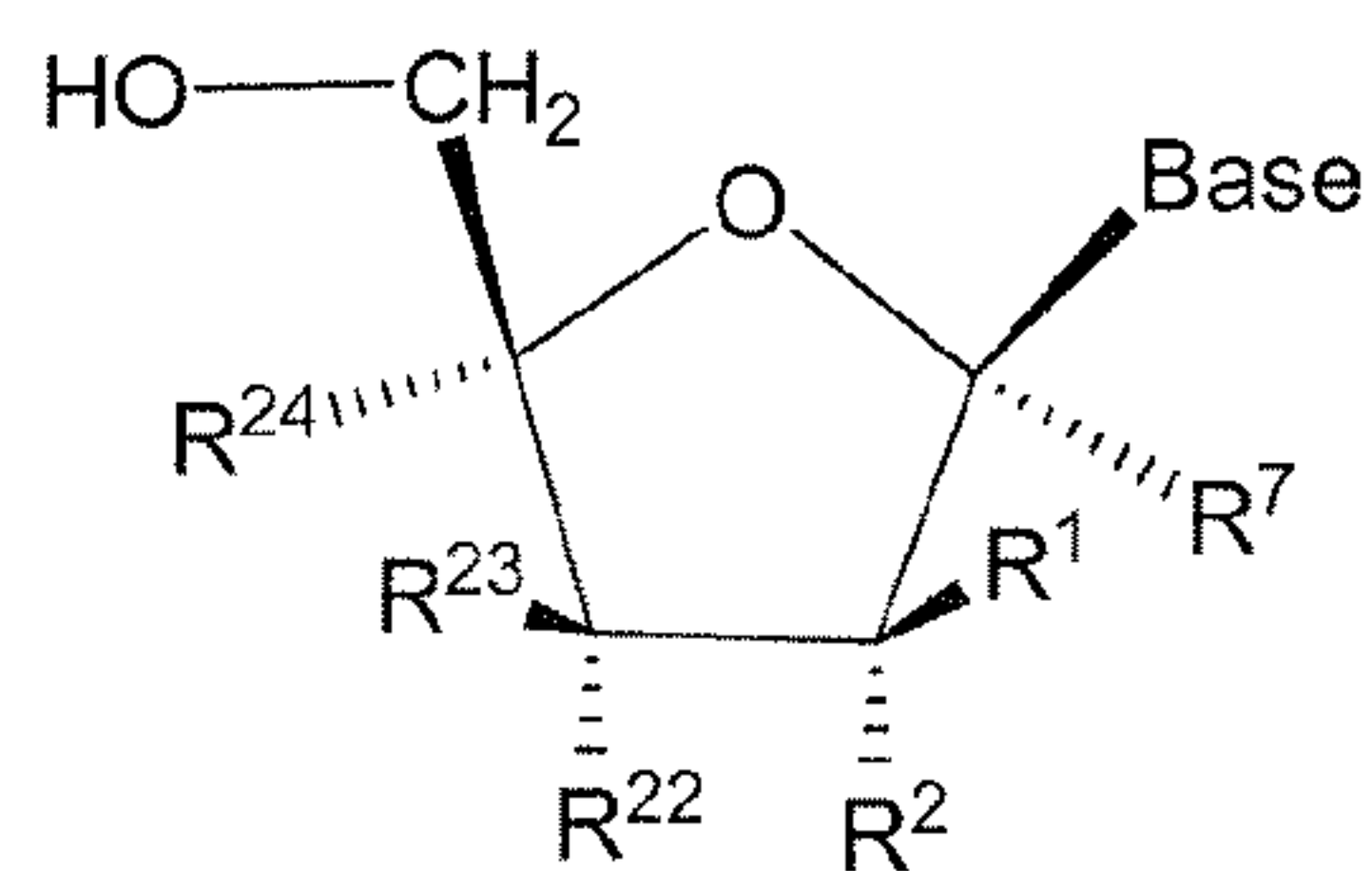
Formula V
