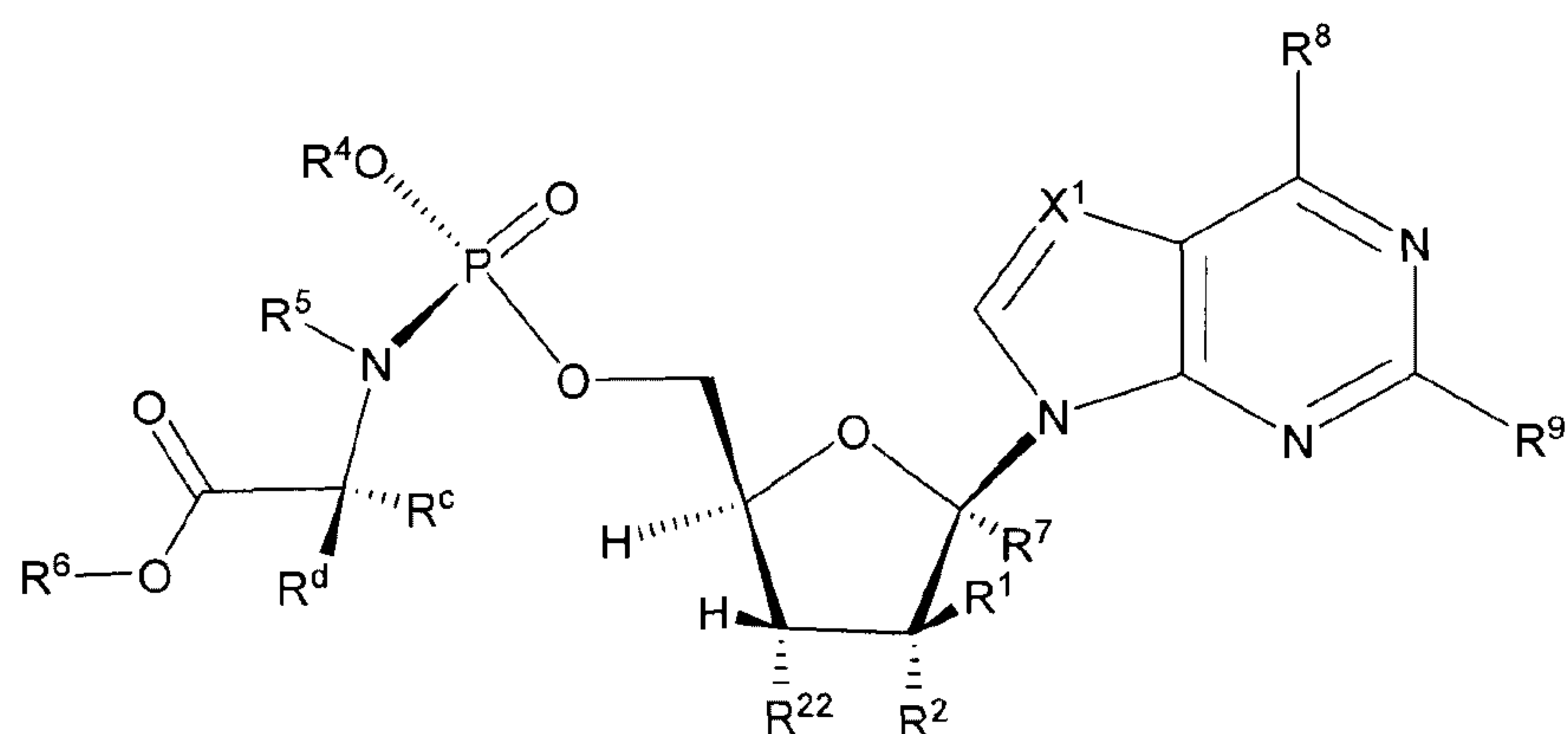
Formula XIb
