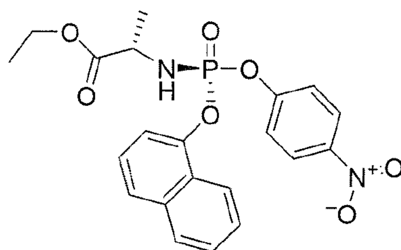
Compound 20
