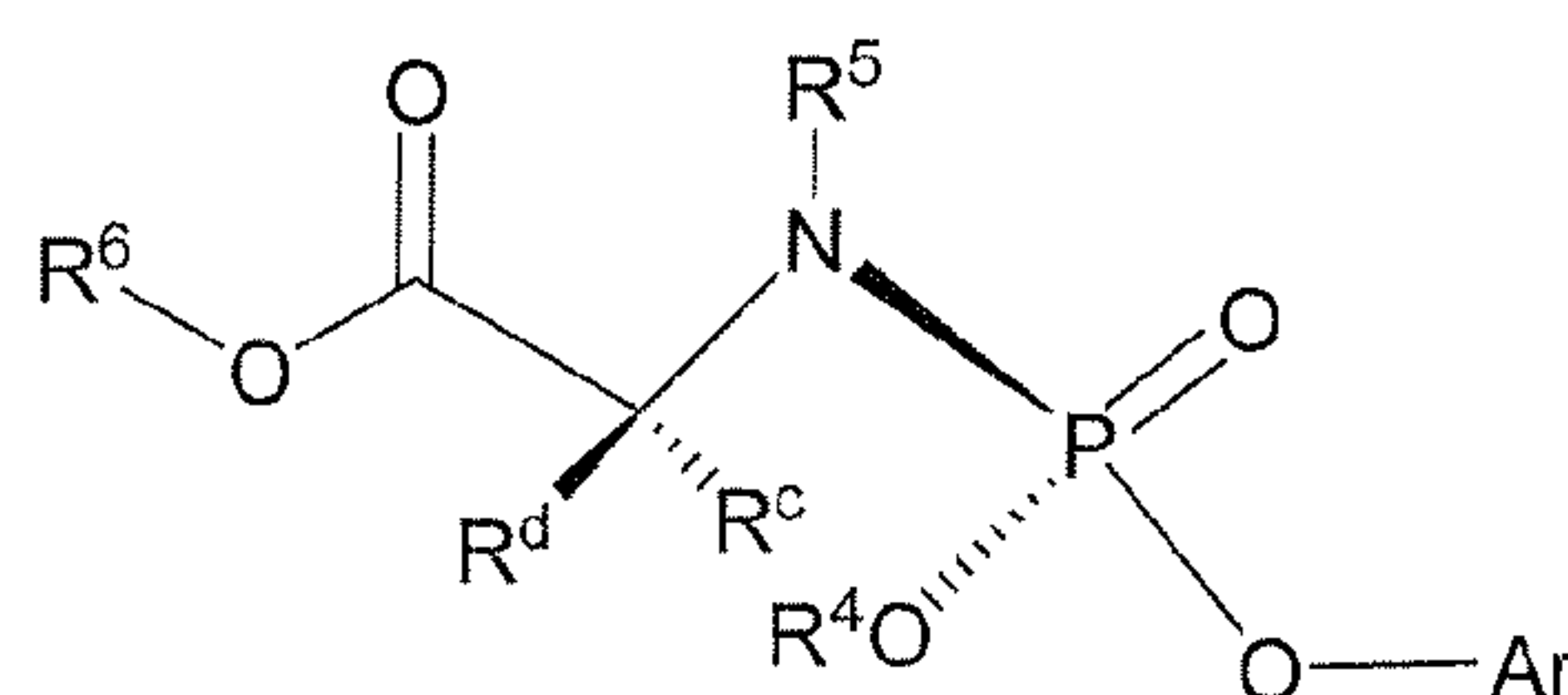
Formula IIIa
