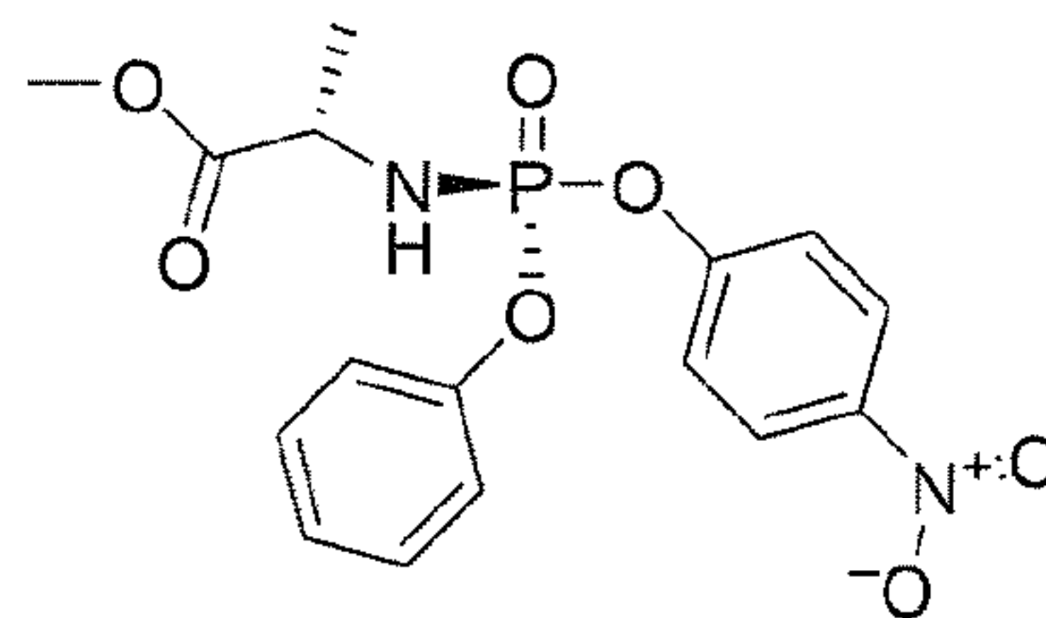
Compound 10
