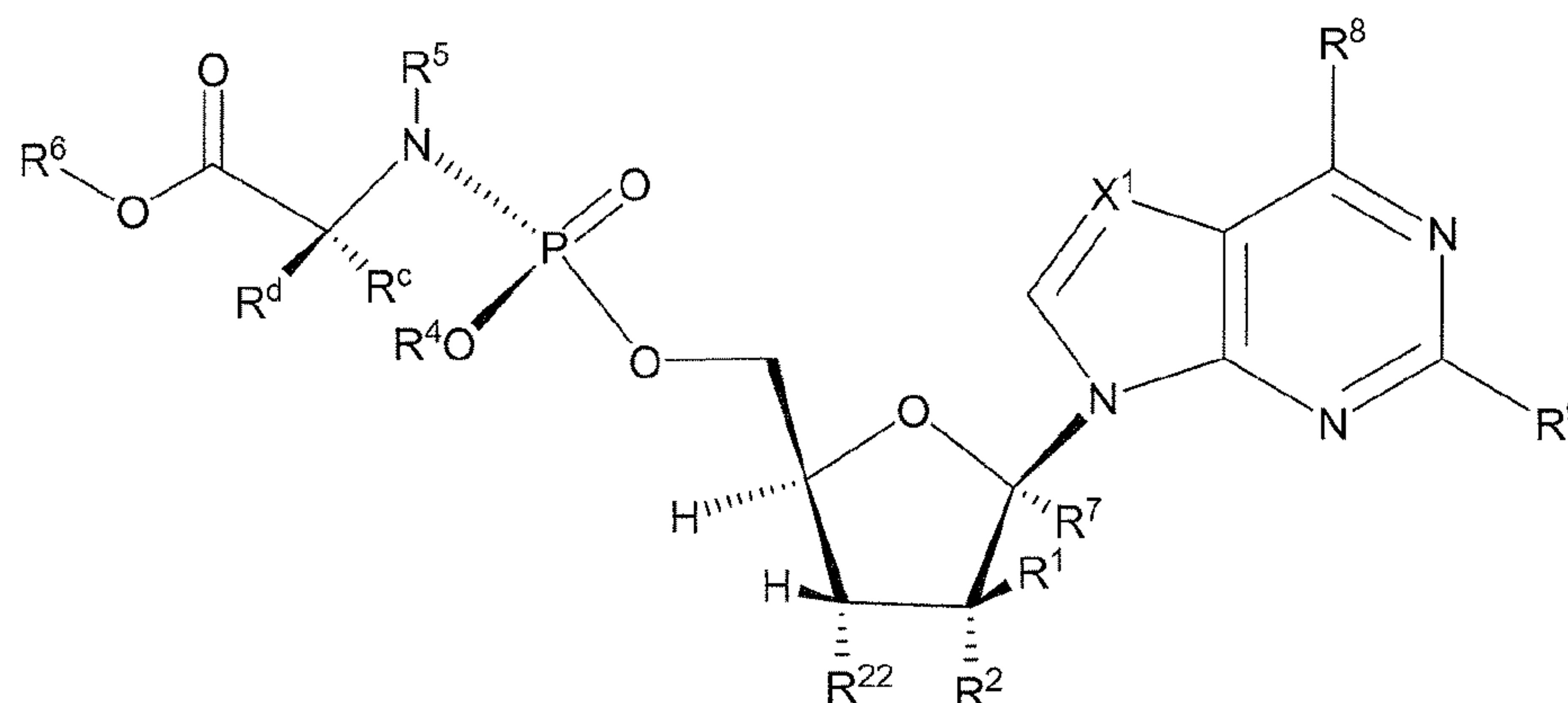
Formula XIa
