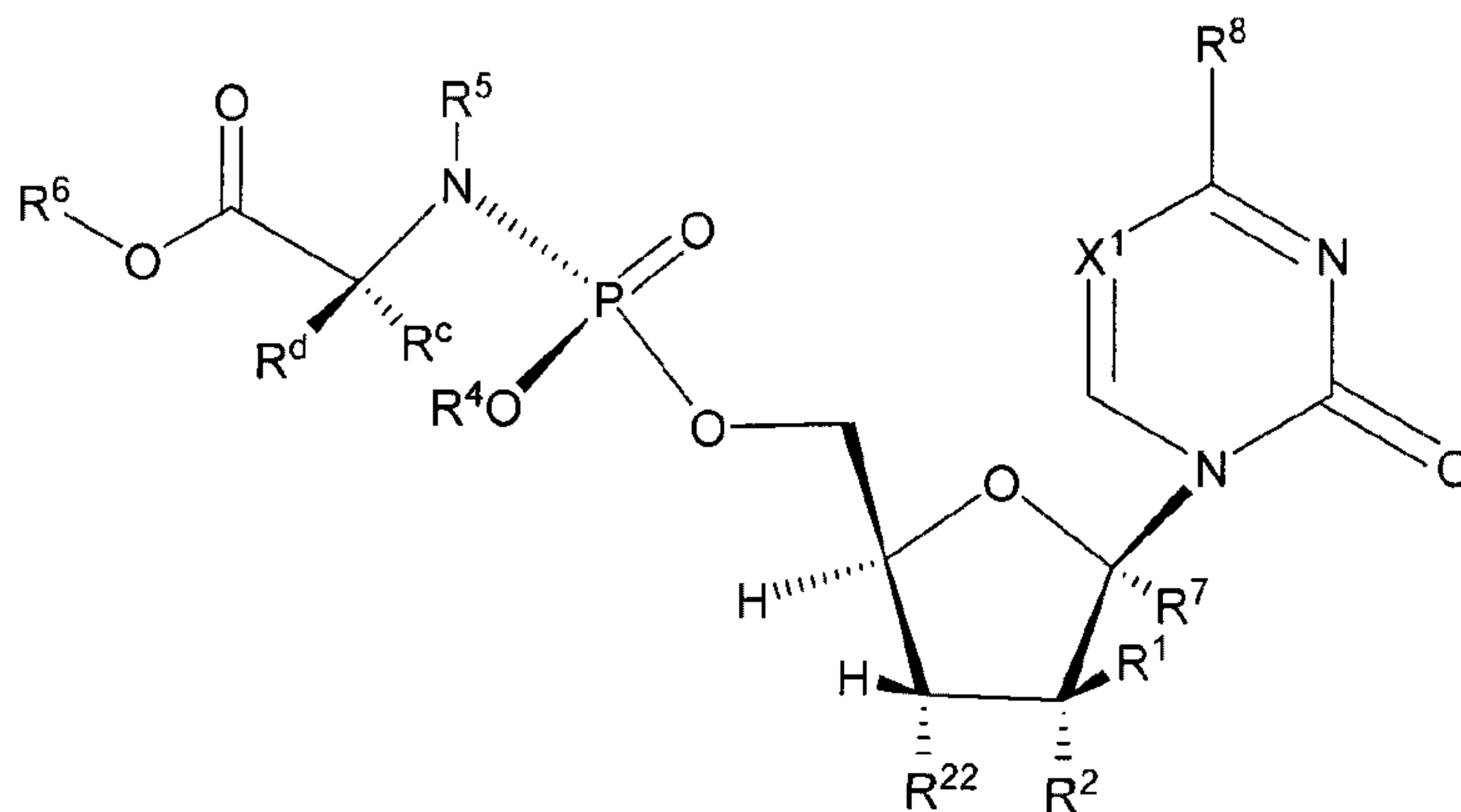
Formula XIIIa
