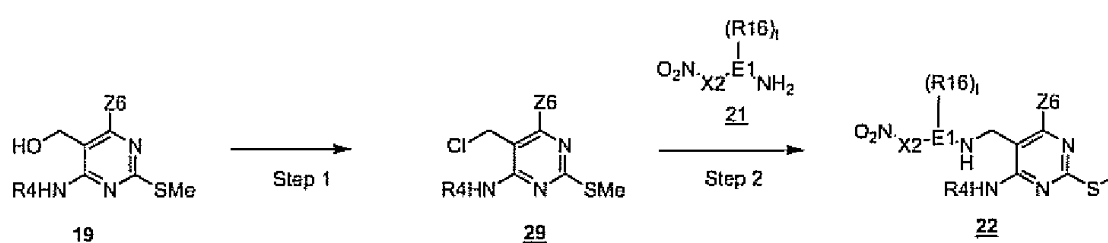
Scheme 4
