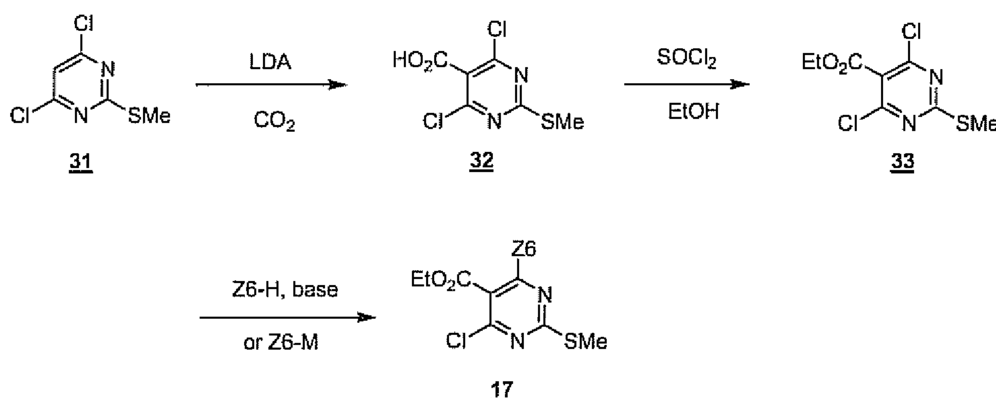
Scheme 5
