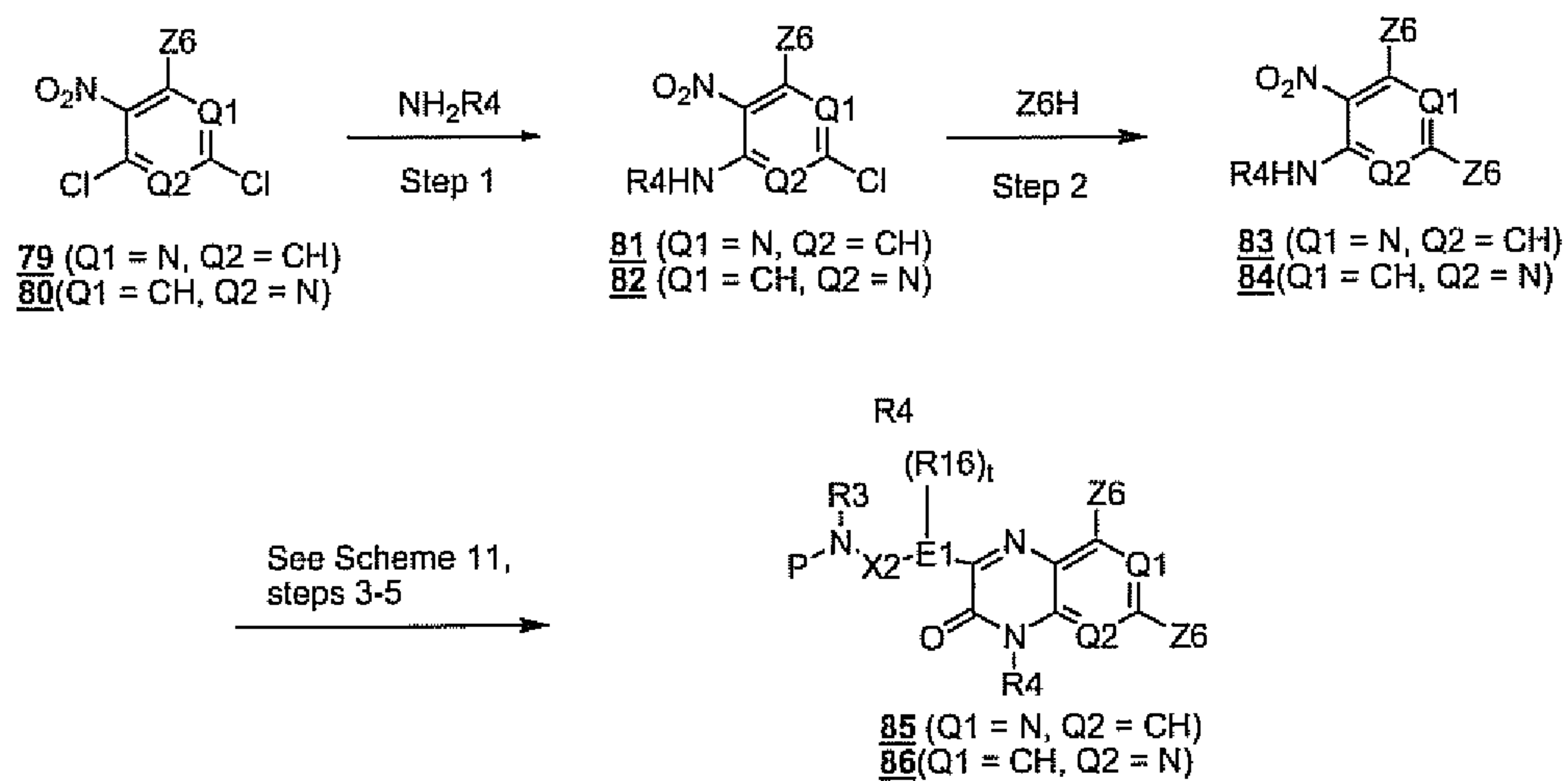
Scheme 12
