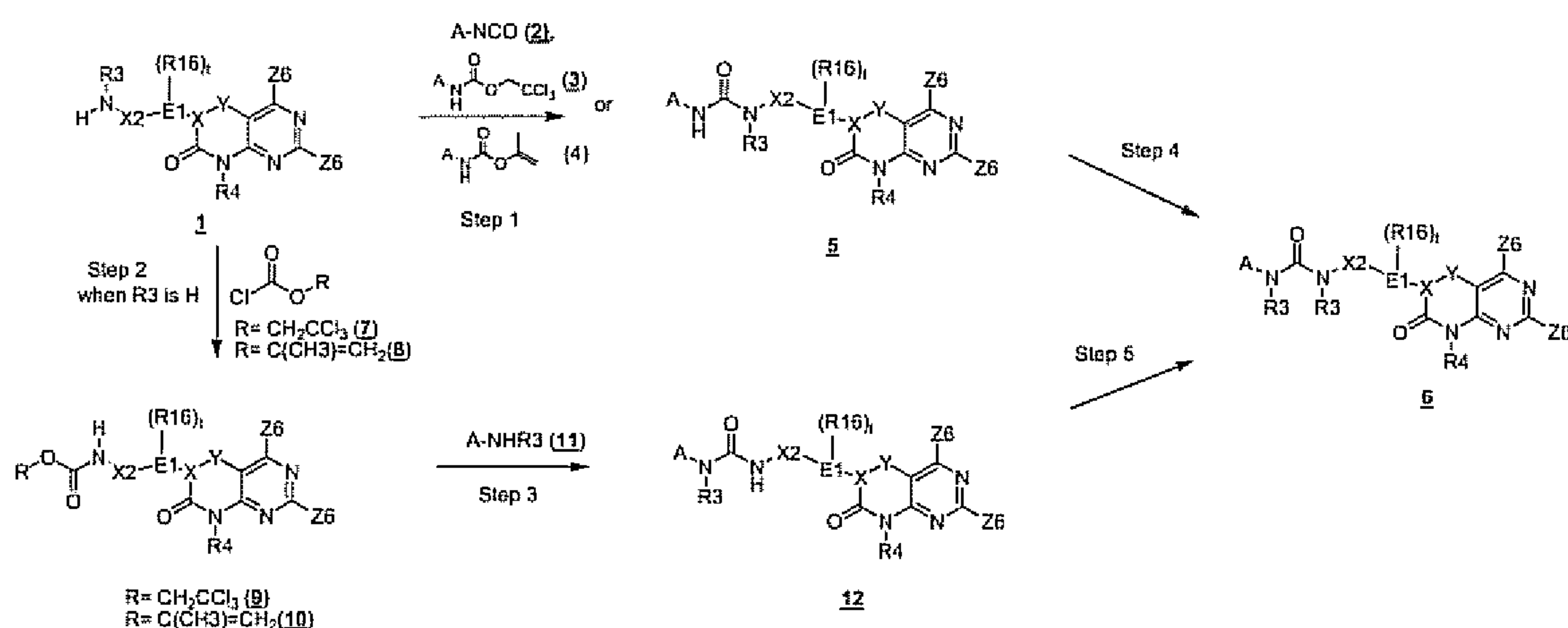
Scheme 1
