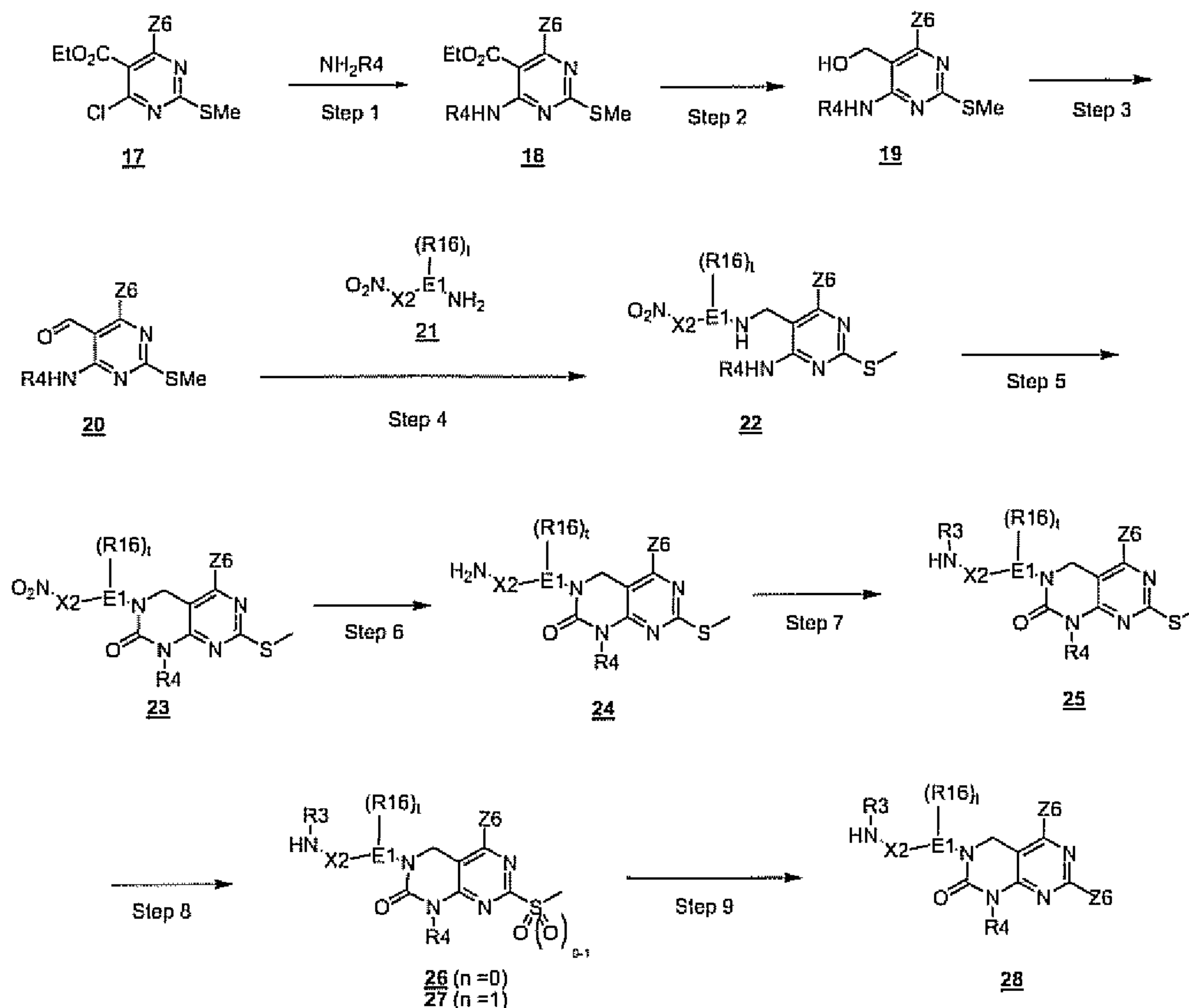
Scheme 3
