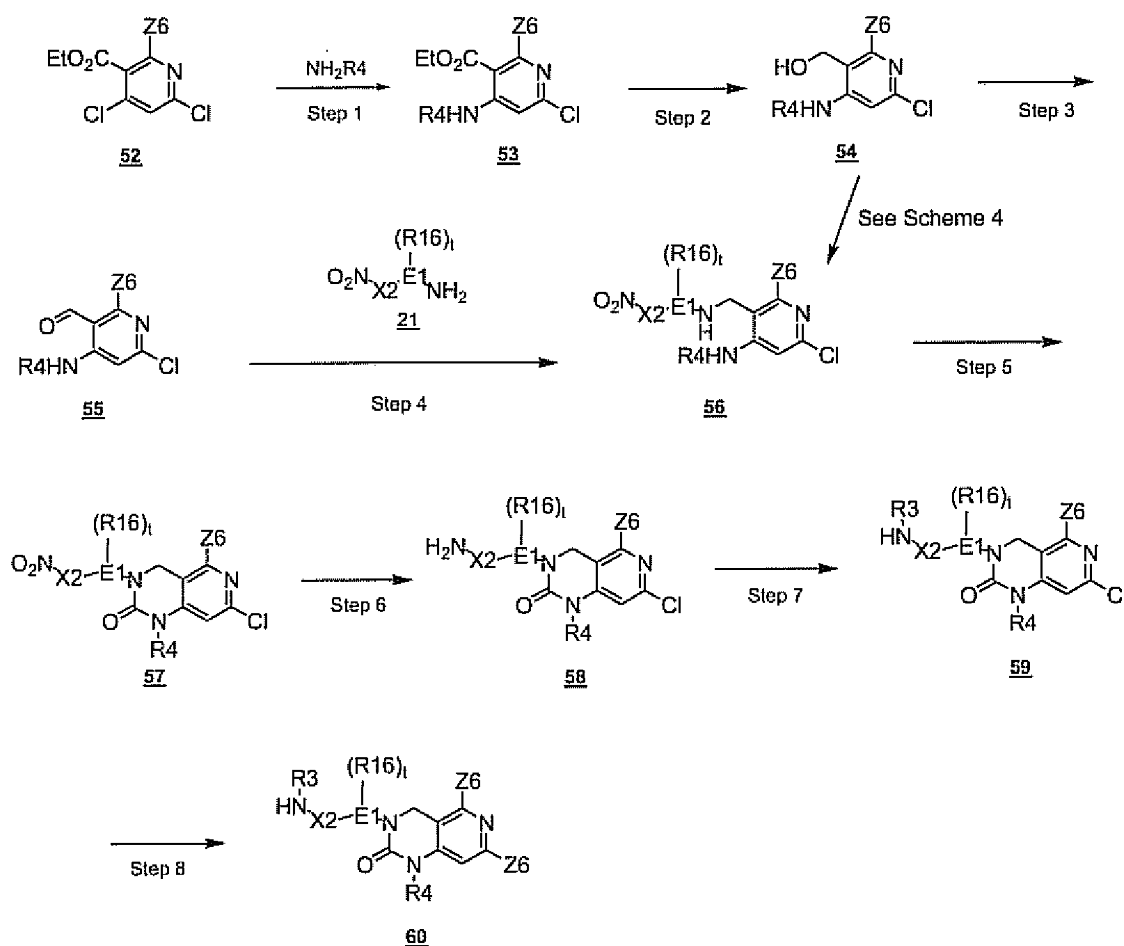
Scheme 8
