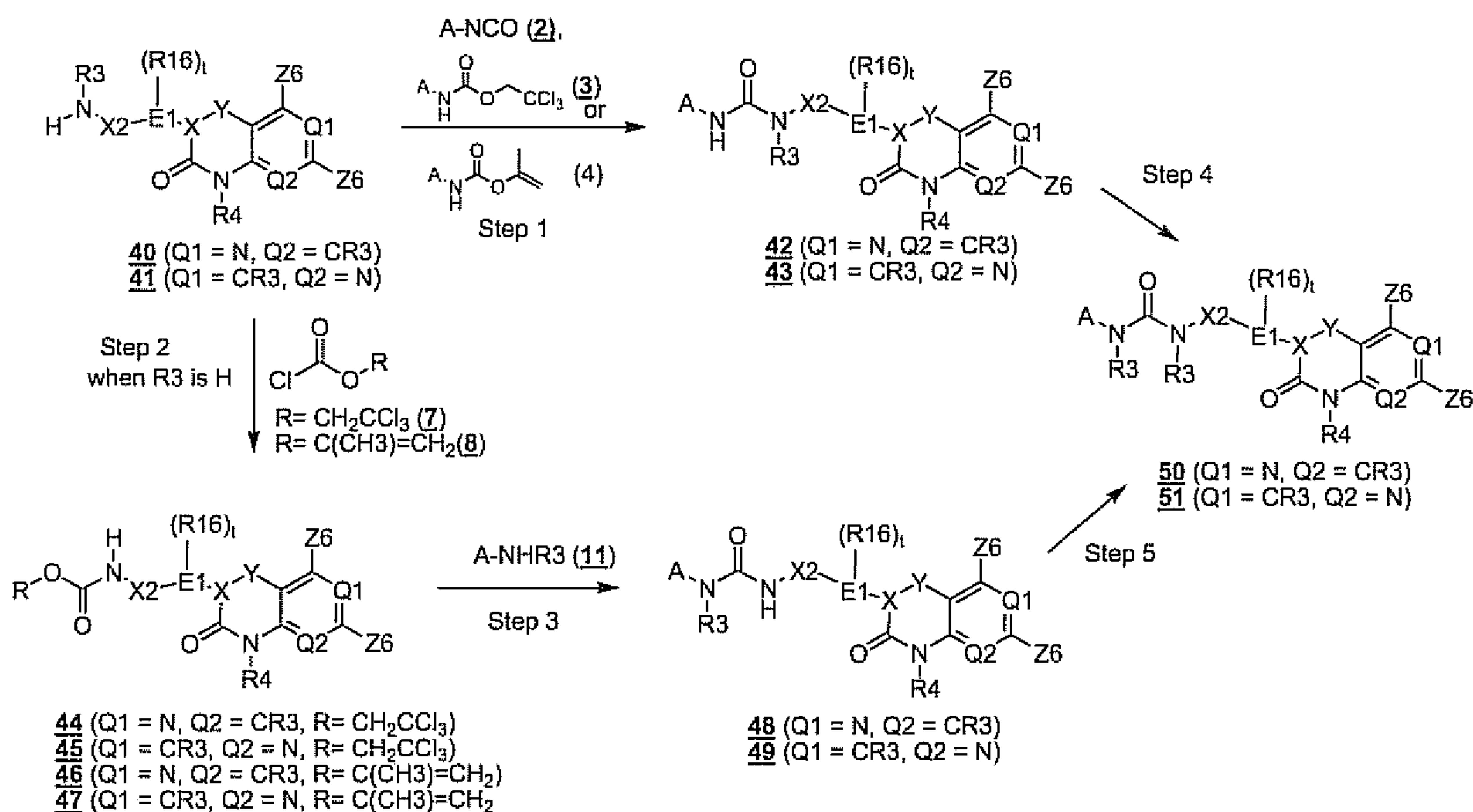
Scheme 7
