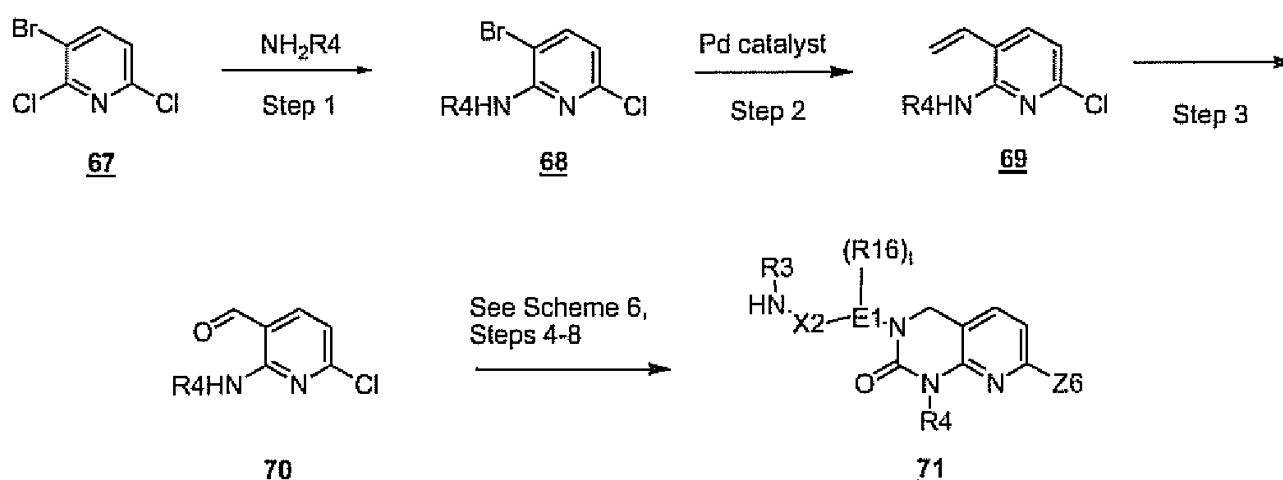
Scheme 10
