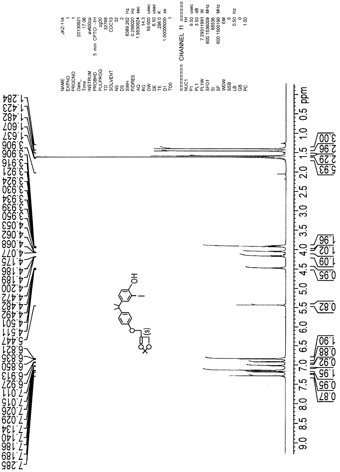
FIG.5A Compound iii-Cl, 1 H NMR
